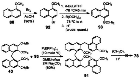
Scheme 3.18 Synthesis of uncyclized tetranaphthyl compound 91
