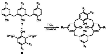
Scheme 1.3 Synthesis of calix[4]arenes via "3+1" fragment condensation
