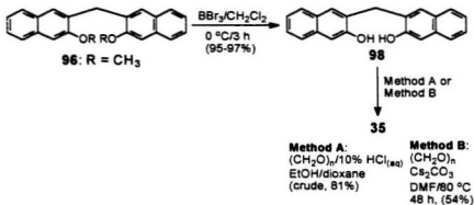
Scheme 3.25 Synthesis of "C-12" endo calix[4]naphthalene 35
