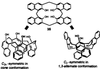
Figure 3.1 Different conformation of 35
