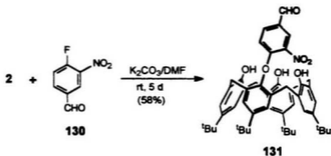
Scheme 5.2 Synthesis of monoaryl ether compound 131
