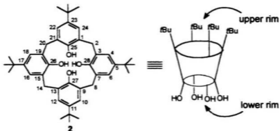
Figure 1.1 Nomenclature of calix[4]arene
