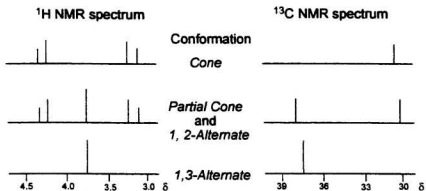
Figure 1.3 ^1\text{H} NMR and ^{13}\text{C} NMR spectral patterns of the methylene groups of calixarenes
