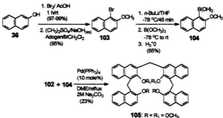
Scheme 3.22 Synthesis of uncyclized tetraphthyl compound 105 using Pd(0)-catalyzed conditions afforded 105 in low yield (23%) (Scheme 3.22).
