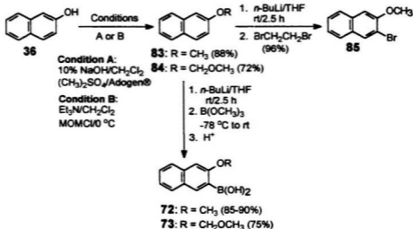
Scheme 3.13 Ortho metallation of 2-naphthol derivatives ( 83 and 84 ) preferential substitution at the C-3 position. Biehl et al. 58 have shown that treating 83 with n -BuLi in diethyl ether followed by the addition of electrophiles DMF or TMSCl afforded ortho substituted products. In our hands, a more convenient approach was found by treating 83 with n -BuLi in THF instead of diethyl ether and stirring for 2.5 h at room temperature, followed by the addition of trimethyl borate or 1,2-dibromoethane at -78 °C to afford the ortho substituted (C-3) products 72 or 85 , respectively. Thus, ortho metallation of 83 with 1.25 equivalents of n -BuLi and 1,2-dibromoethane in THF afforded 3-bromo-2-methoxynaphthalene 85 in 96% yield (Scheme 3.13). When the ortho metallation conditions were employed with either 83 or 84 , followed by treatment with trimethyl borate, the corresponding boronic acid derivatives 72 and 73 were obtained in 85-90% and 75% yields, respectively
