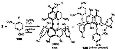
Scheme 5.5 Synthesis of di-O-aryl compound 133 and 138 using Ullmann aryl ether-forming conditions
