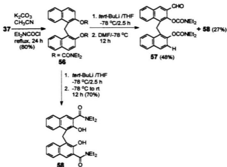
Scheme 3.8 Double ortho metallation of compound 56
