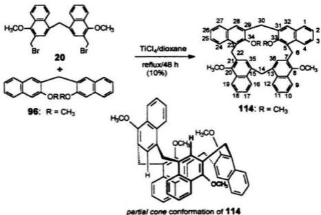
Scheme 3.29 Synthesis of endo/exo calix[4]naphthalene 114
