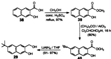
Scheme 2.1 Synthesis of intermediate 29
