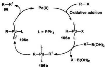
Scheme 3.23 A proposed mechanism for the Pd(0)-catalyzed coupling of 72 and 74
