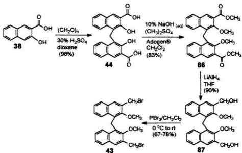
Scheme 3.14 Synthesis of compound 43
