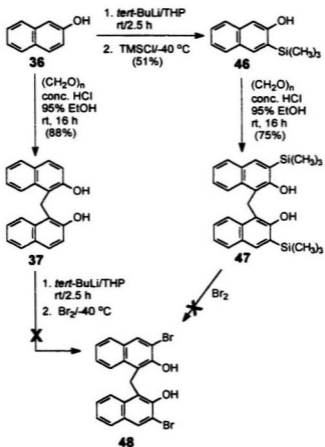
Scheme 3.4 Attempted synthesis of compound 48
