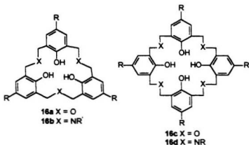
Figure 1.5 Other examples of calixarenes
