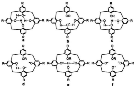
Figure 2.3 Mono, dianions and trianions of calix[4]arenes
