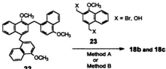
Scheme 1.9 Synthesis of 18b-18c via "3+1" fragment condensation
