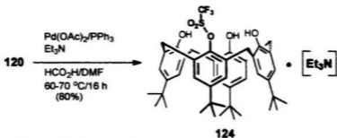
Scheme 4.5 Attempted reactions to replace triflates in 120
