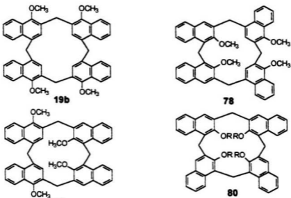
Figure 3.2 Different isomers of calix[4]naphthalenes ( 19b , 78-80 )
