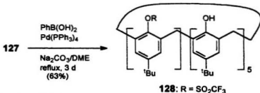
Scheme 4.9 Attempted reactions to replace triflates in 127
