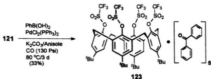
Scheme 4.4 Pd(0)-catalyzed carbonylation reactions between 121 and phenylboronic acid
