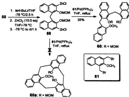
Scheme 3.9 Attempted coupling of 59 and 61 using Negishi conditions
