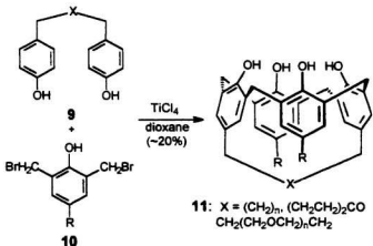
Scheme 1.4 Synthesis of calix[4]arenes via "2+2" fragment condensation
