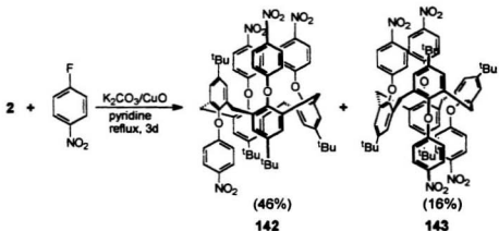
Scheme 5.7 Synthesis of tetra-O-aryl compounds 142 and 143 using Ullmann aryl ether-forming conditions
