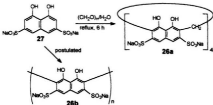
Scheme 1.11 Synthesis of sulfonatocalix[4]naphthalene ( 26a )
