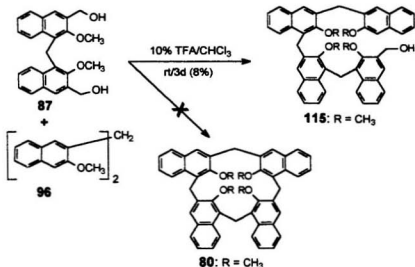
Scheme 3.30 Attempted synthesis of compound 80
