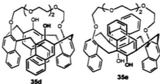
Figure 1.7 An example of calixcrown derivative of 35
