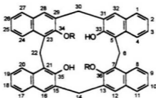
113d: R = Ethyl
