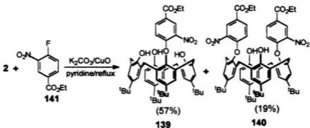
Scheme 5.6 Synthesis of compounds 139 and 140
