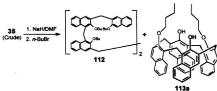
Scheme 3.26 Synthesis of n -butyl ether derivative of 35
