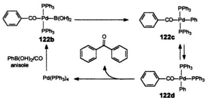
Scheme 4.3 A proposed mechanism for the synthesis of benzophenone during the coupling reactions of 118 and phenylboronic acid
