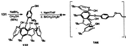
Scheme 5.8 Attempts to form double calixarenes 144
