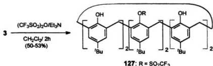
Scheme 4.8 Synthesis of tert -butylcalix[6]arene triflates ( 127 )
