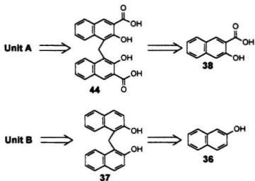
Scheme 3.2 Retrosynthetic analysis of Unit A and Unit B
