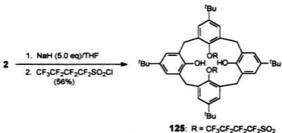
Scheme 4.6 Synthesis of tert -butylcalix[4]arene nonaflates ( 125 )
