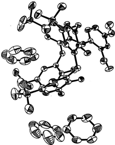
Figure 5.3 X-ray crystal structure of 131
