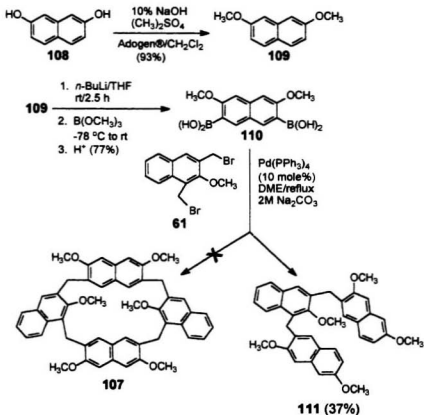
Scheme 3.24 Attempted cyclization of 61 and 110
