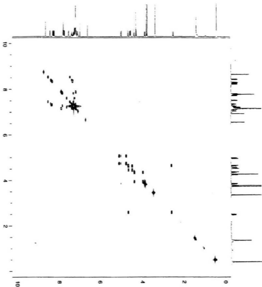
Figure 3.6 ^1\text{H} COSY spectrum of compound 114
