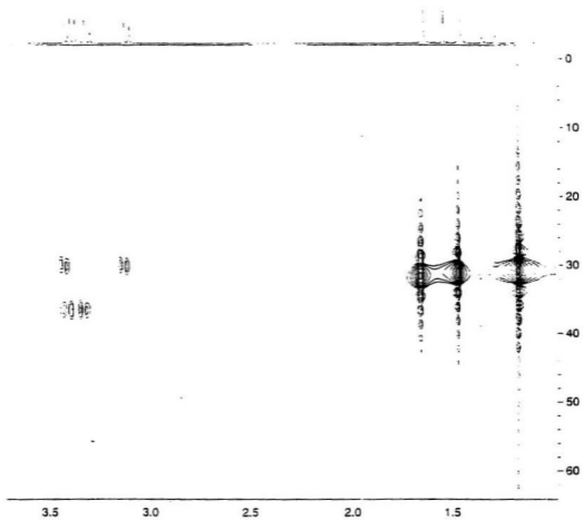
Figure 5.5 ^1\text{H} COSY spectrum of the methylene region of compound 142
