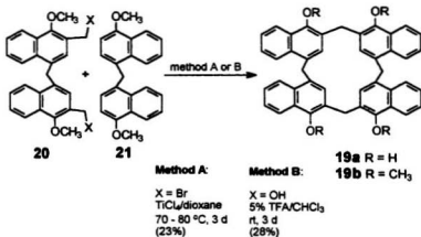
Scheme 1.8 Synthesis of exo calix[4]naphthalenes via "2+2" fragment condensation
