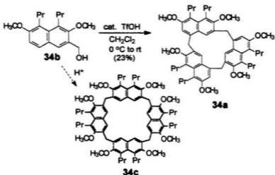
Scheme 1.14 Synthesis of cyclic trimer containing naphthalene rings
