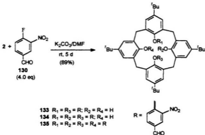
Scheme 5.3 Attempts to form tetra-O-aryl ether derivatives of 2
