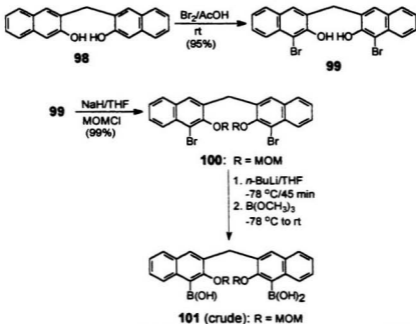
Scheme 3.20 Synthesis of bis(naphthalene)boronic acid 101
