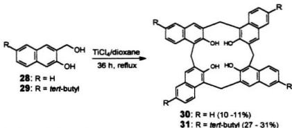
Scheme 1.12 Synthesis of endo calix[4]naphthalenes ( 30-31 )
