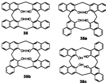
Figure 1.6 Isomers of endo calix[4]naphthalenes
