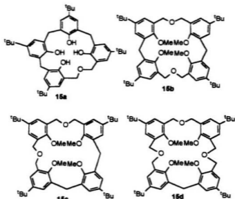
Figure 1.4 Examples of homooxalixarenes
