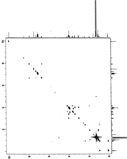
Figure 5.6 ^1\text{H} COSY spectrum of compound 145
