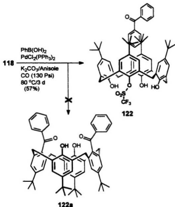
Scheme 4.2 Attempted synthesis of 122a via Pd(0)-catalyzed carbonylation reactions
