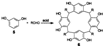
Scheme 1.2 Synthesis of calixresorcin[4]arenes
