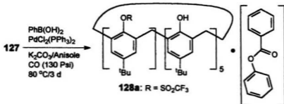
Scheme 4.10 Pd(0)-catalyzed carbonylation reactions between 127 and phenylboronic acid
