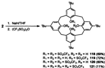
Scheme 4.1 Synthesis of tert -butylcalix[4]arene triflates (118-121)
