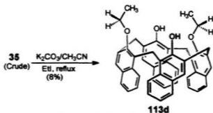
Scheme 3.28 Synthesis of ethyl ether derivatives of 35
