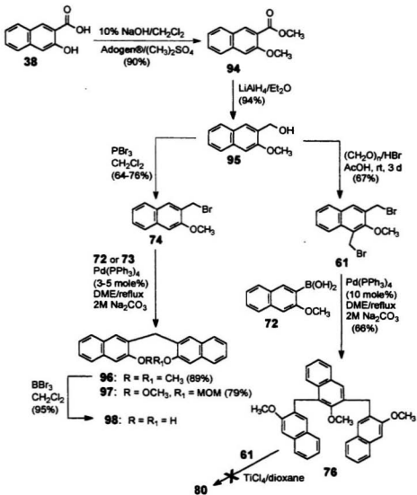
Scheme 3.19
