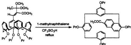
Scheme 1.13 Synthesis of naphthalene-containing calix[4]arene
