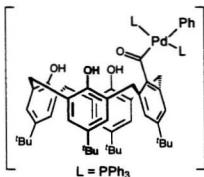
Figure 4.3 A putative square-planar intermediate during carbonylation reactions of calixarene triflate and phenylboronic acid
