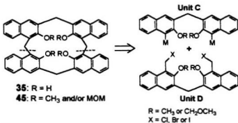
Scheme 3.3 Alternative retrosynthetic route of 35
