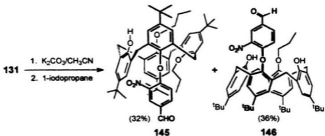
Scheme 5.9 Synthesis of propyl ether derivatives of 131
