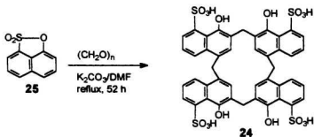
Scheme 1.10 Synthesis of peri -tetrasulfonatocalix[4]naphthalene (24)
