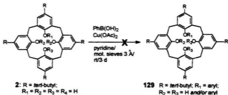
Scheme 5.1 Attempts to form phenyl ethers using Cu(II)acetate-promoted conditions
