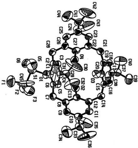
Figure 4.1 X-ray crystal structure of 119
