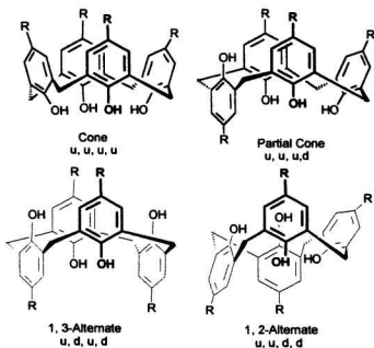
Figure 1.2 Conformation of calix[4]arenes
