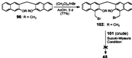
Scheme 3.21 Attempted coupling of 101 and 102 using Suzuki-Miyaura Pd(0)-catalyzed conditions
