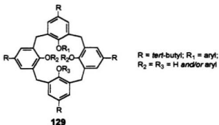
Figure 5.1 Lower rim aryl ether derivatives of calixarenes
