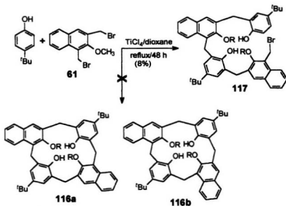
Scheme 3.31 Attempted synthesis of compound 116a-b
