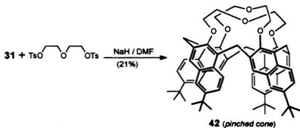
Scheme 2.4 Synthesis of tert -butylcalix[4]naphthalene-1,3-crown
