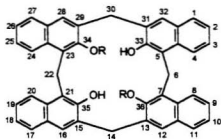
113c: R = isopropyl
