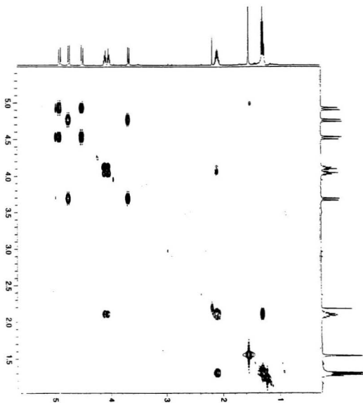
Figure 3.3 ^1\text{H} COSY spectrum of the methylene region of 113b
