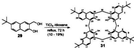
Scheme 2.2 Synthesis of endo calix[4]naphthalene ( 31 )
