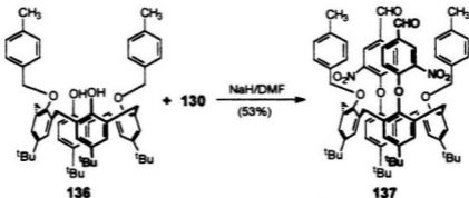
Scheme 5.4 Synthesis of di-O-benzyl-di-O-aryl compound 137
