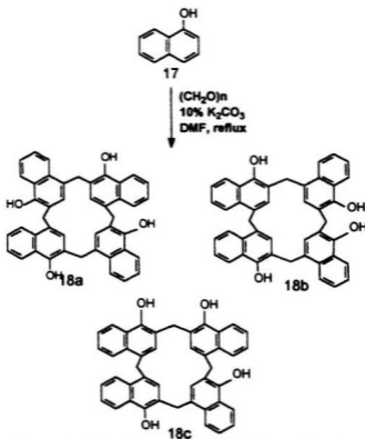
Scheme 1.7 A 'One-pot' synthesis of exo calix[4]-naphthalene (18a-18c)
