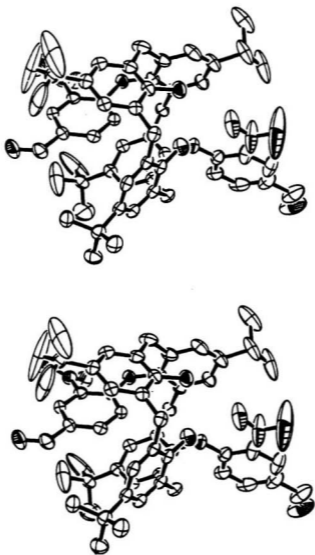
Figure 5.4 Stereoview X-ray crystal structure of compound 138
