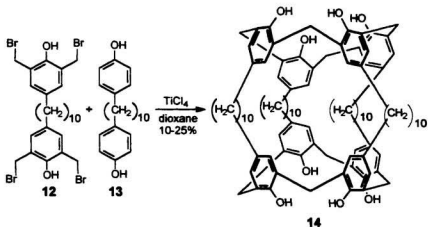
Scheme 1.5 Synthesis of tetra-linked double calix[4]arenes
