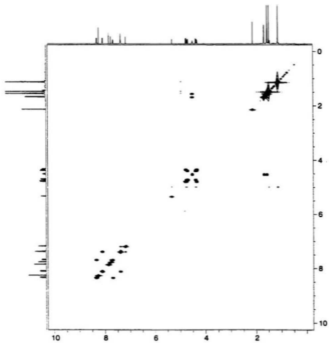
Figure 2.5 ^1\text{H} COSY spectrum of compound 41b
