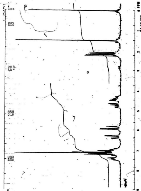
Figure 2.1: The ^1\text{H} FT NMR spectrum of trans-1,2-dihydroxy-1,2-dihydronaphthalene
