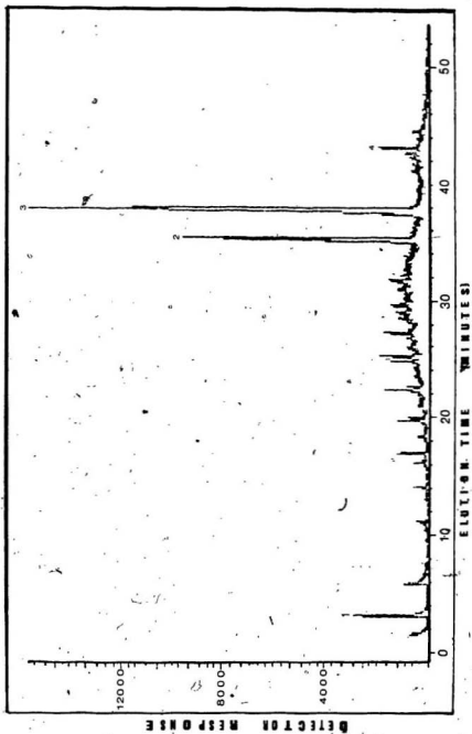
Figure A.3: GC-mass spectrum of the NOS fraction of PBCO
