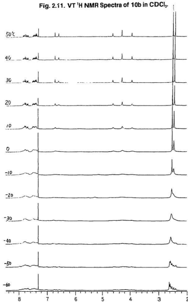
Fig. 2.11. VT ^1\text{H} NMR Spectra of 10b in \text{CDCl}_3 .
