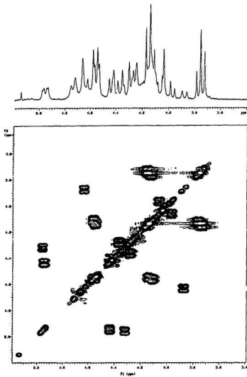
Fig. 2.8. HH COSY Spectrum of Methylene in 10a at -50 °C in \text{CDCl}_3 .
