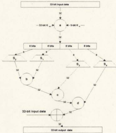
Figure 4.10: The Generic Round Function Module
