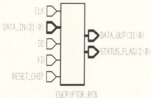
Figure 4.7: A Component Interface of RC6 Encrytor
