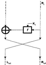
Figure 2.4: A Basic Feistel Structure
