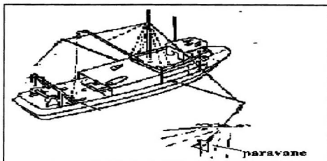
FIGURE 5.7: PARAVANE STABILIZER IN DEPLOYED POSITION.
