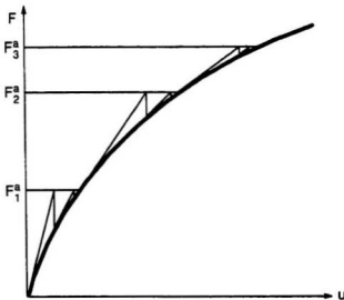
Figure 3.5 Incremental Newton-Raphson procedure
