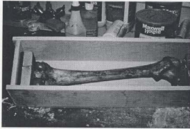
Figure 4.6 - Femur held in scanning orientation between custom made load platens. The purpose of the plywood box is to embed the femur in plaster for subsequent sectioning.
