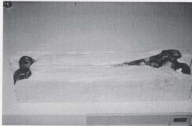
Figure 4.7 - Femur embedded in plaster in scan / load orientation. The sides of the plaster block are parallel to the load axis.
