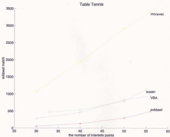
Figure 5.4 Comparison using sub-block matching as the benchmark
