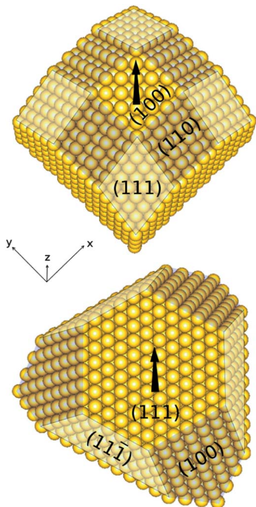
Fig. 7 The 4-fold and 6-fold symmetries observed in spin coated colloidal crystals arise from Bragg reflections from different faces of an fcc structure. With the z direction corresponding to the “top” view of spin coated structures, fcc structures with (100) and (111) faces parallel to the substrate give rise to 4- and 6-arm patterns respectively. The global 4 or 6 arm symmetry is believed to arise from Bragg reflections from light incident at oblique angles. In particular, the 4-fold symmetry of the (111) and (110) planes (top) leads to the 4 arm patterns, and the 3-fold symmetry of the (11 \bar{1} ) and (100) planes (bottom) leads to the 6 arm patterns; see text.
