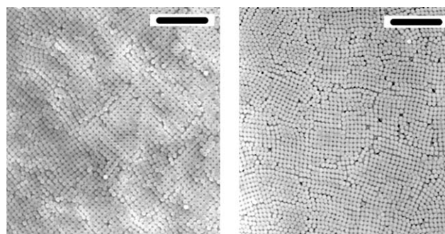
Fig. 8 Scanning electron micrographs in the absence and in the presence of an electric field, left and right respectively. 22 Field strength 0.95 kV mm -1 and frequency 3 kHz. Left: the dominant domain orientation at zero field (obtained via individual particle tracking methods that are optimized for crowded particle features 43 ) is along the radial direction, which is about 45° from the vertical. Right: the dominant domain orientation is along the field direction (vertical) and not in the radial direction (which is 49° from vertical). The scale bars are 5 μm (reprinted from, Langmuir , 2012, 28 , 3067–3070. Copyright 2012 American Chemical Society).
