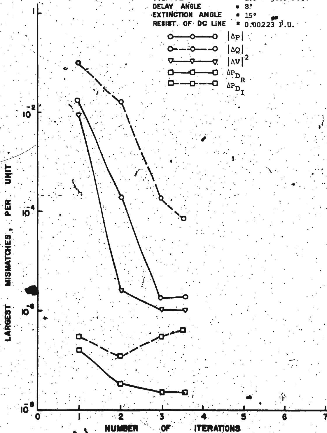
FIGURE 4.20 Convergence Characteristics of Test System C (Alpha-M.Q.S.O.N.R. Method)
