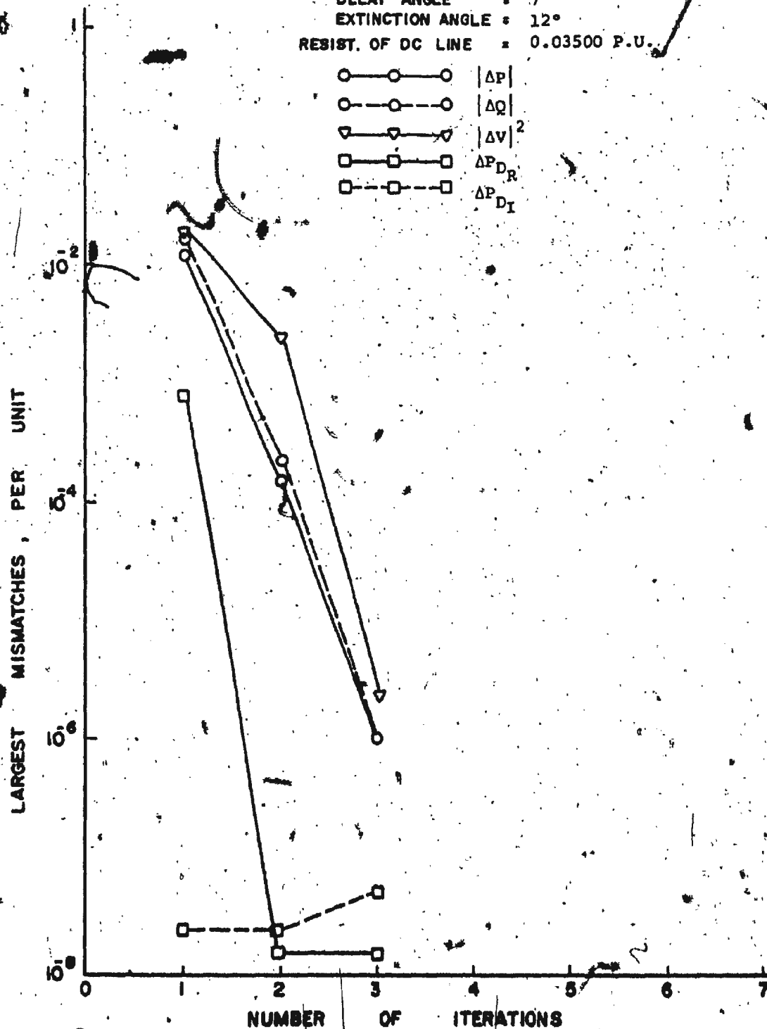
FIGURE 4.7 Convergence Characteristics of Test System R (N.R. Method)
