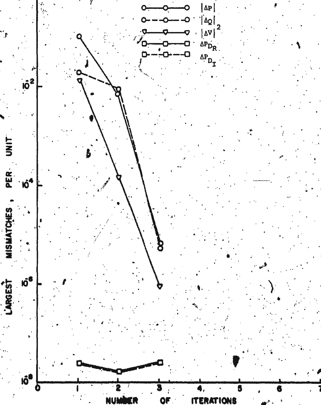
FIGURE 4.11 Convergence Characteristics of Test System D (N.R. Method)
