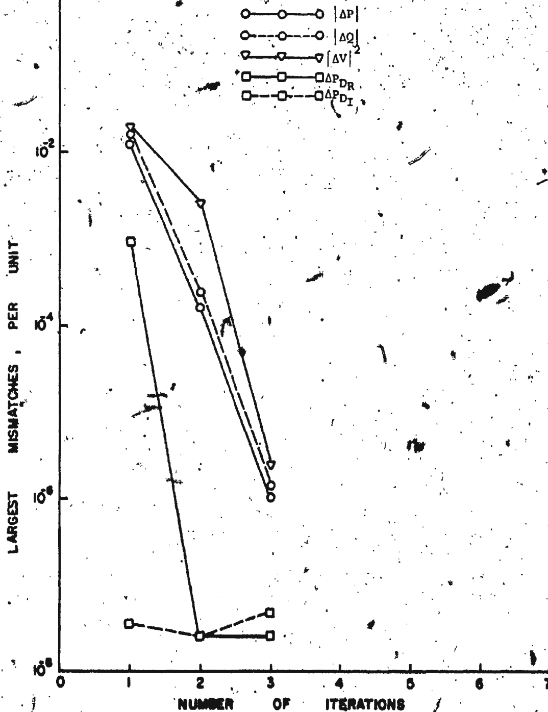
FIGURE 4.8 Convergence Characteristics of Test System B (N.R. Method)
