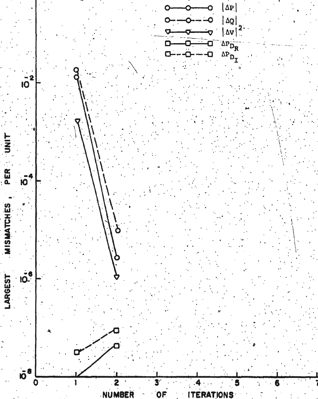
FIGURE 4.21 Convergence Characteristics of Test System D (Alpha-M.Q.S.O.N.R. Method)
