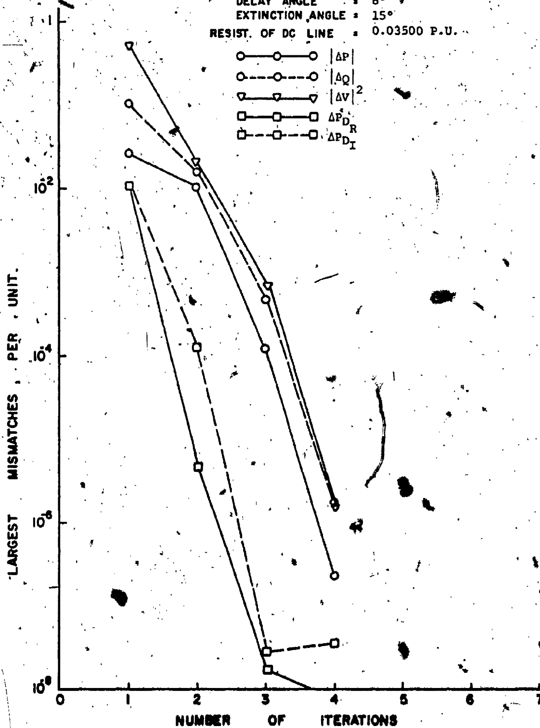
FIGURE 4.6 Convergence Characteristics of Test System B (N.R. Method)
