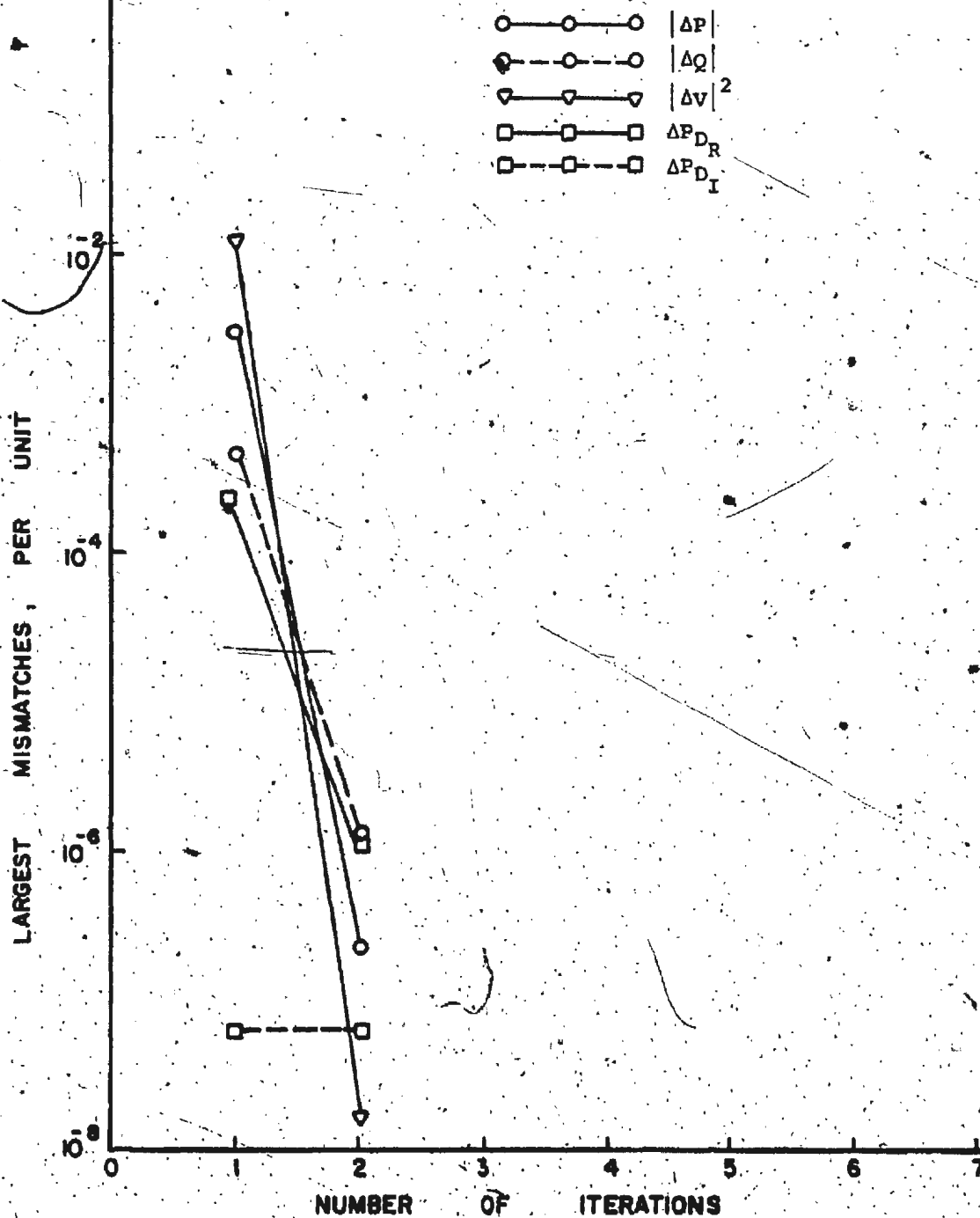
FIGURE 4.19 Convergence Characteristics of Test System B (Alpha-M.Q.S.O.N.R. Method)
