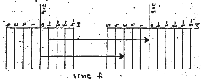
Fig. 2.5. Energy level diagram of ^{13}\text{CH}_3\text{F} . The transitions shown are for the lines a, b, c, d, e and f of Fig. 2.4.
