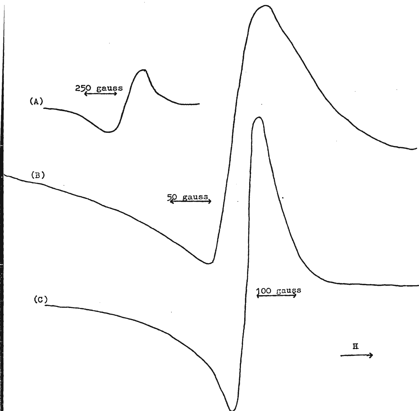
Figure IX. Comparison of (A) e.s.r. spectrum of experimental dimer signal due to copper(II) malate at 77^{\circ}\text{K}^{80} with the e.s.r. spectra of (B) copper(II) phenylsulfoxyacetate 3/2 hydrate and (C) copper(II) phenylsulfoxyacetate monohydrate at x-band frequency in methanol at -30^{\circ}\text{C} .
