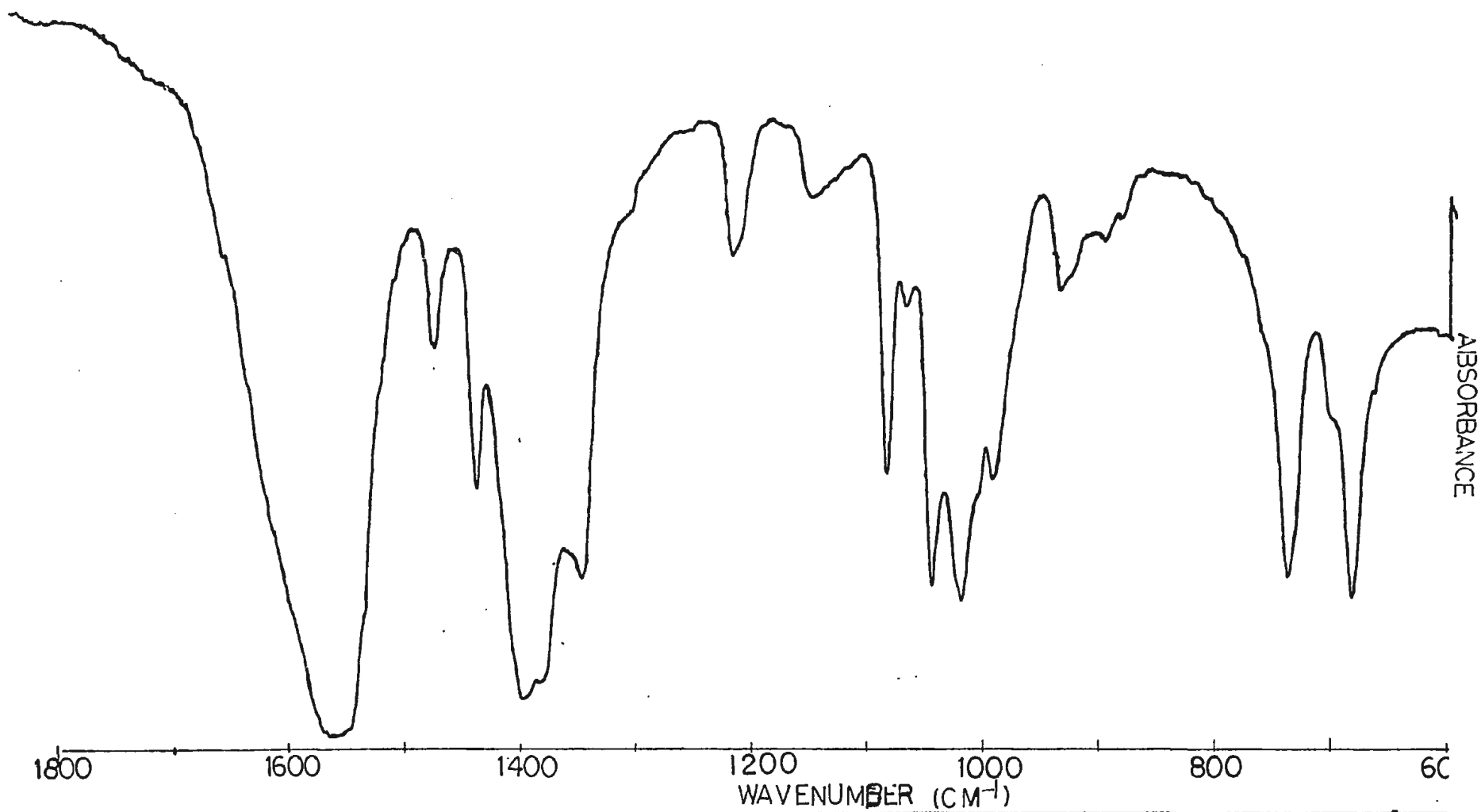
Figure IVa. I.r. spectrum (1800-600 cm -1 ) of simple salt (C 6 H 5 SOCH 2 CO 2 )Cd·2H 2 O.
