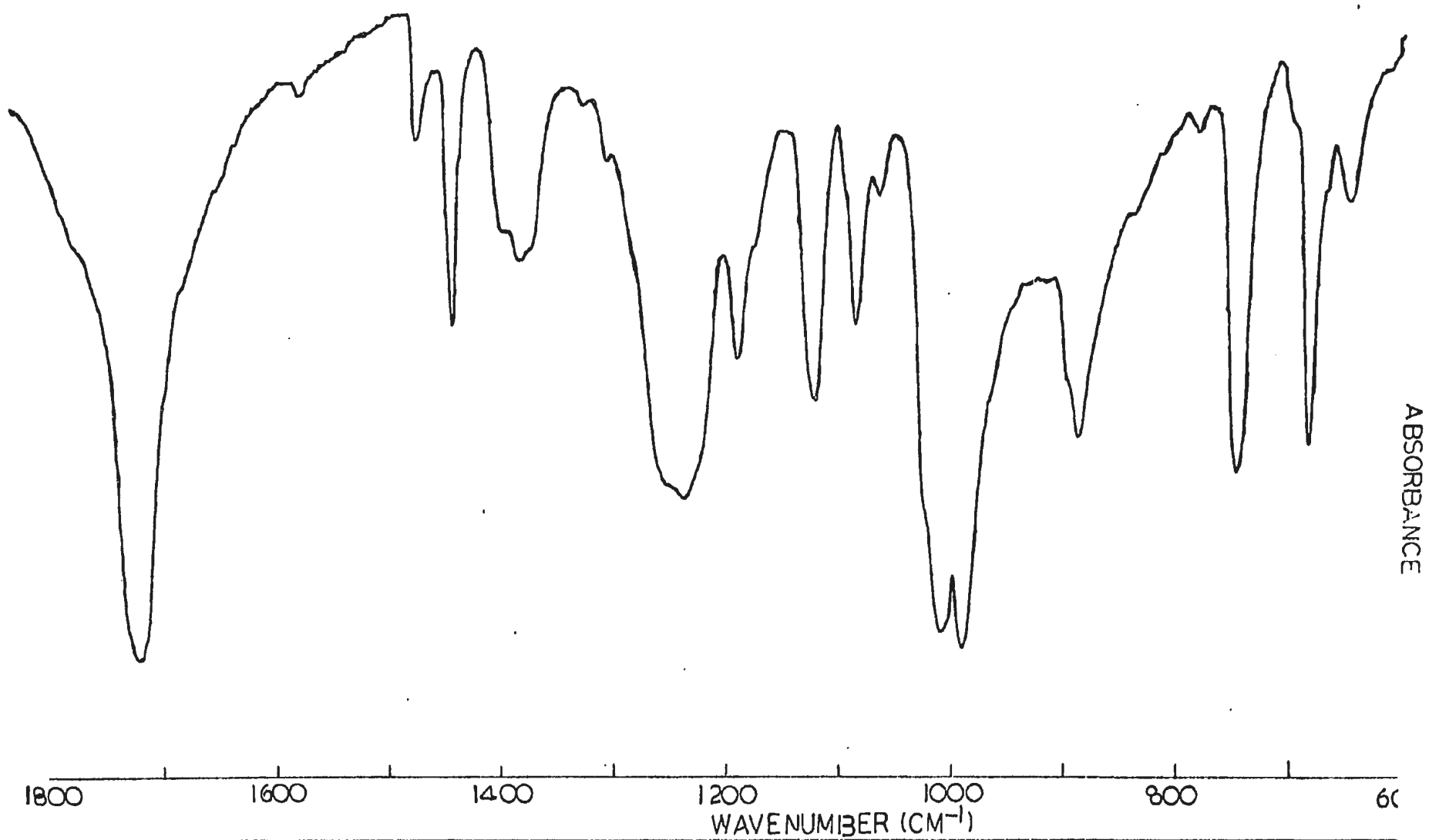
Figure Ib. I.r. spectrum ( 1800\text{--}600\text{ cm}^{-1} ) of phenylsulfoxyacetic acid. in KBr disc.
