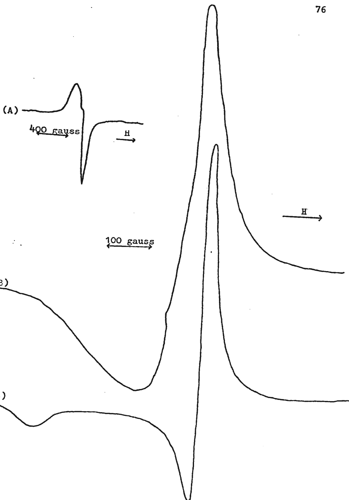
Figure VIII. Comparison of e.s.r. spectrum of (A) copper(II) citrate at PH = 4 at room temperature 76 with e.s.r. spectra of powdered samples of (B) copper(II) phenylsulfoxyacetate 3/2 hydrate and (C) copper(II) phenylsulfoxyacetate monohydrate at x-band frequency at room temperature.
