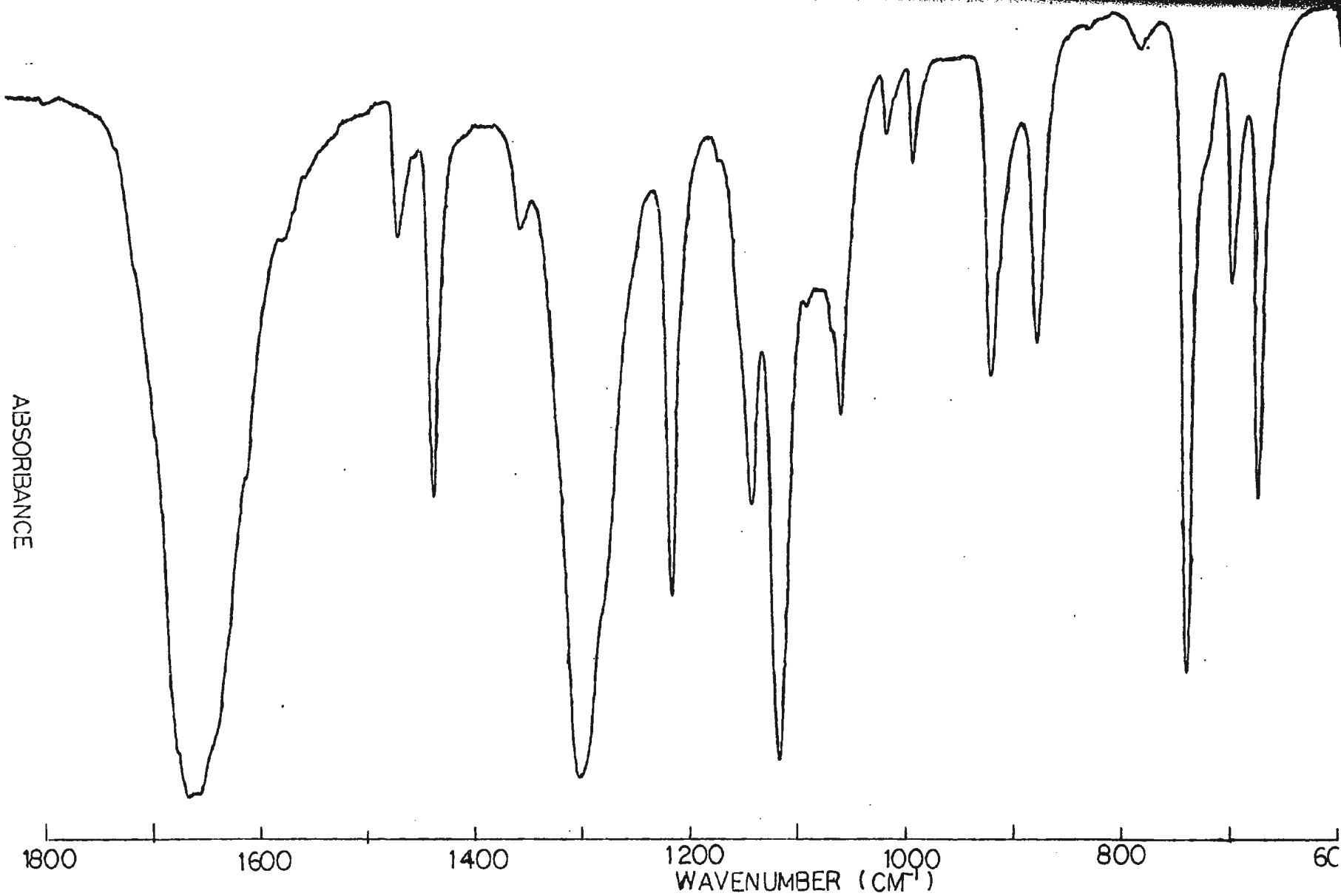
Figure IIb. I.r. spectrum (1800-600 \text{cm}^{-1} ) of chelated \text{H}(\text{Pt}(\text{C}_6\text{H}_5\text{SOCH}_2\text{CO}_2)\text{Cl}_2) in KBr disc
