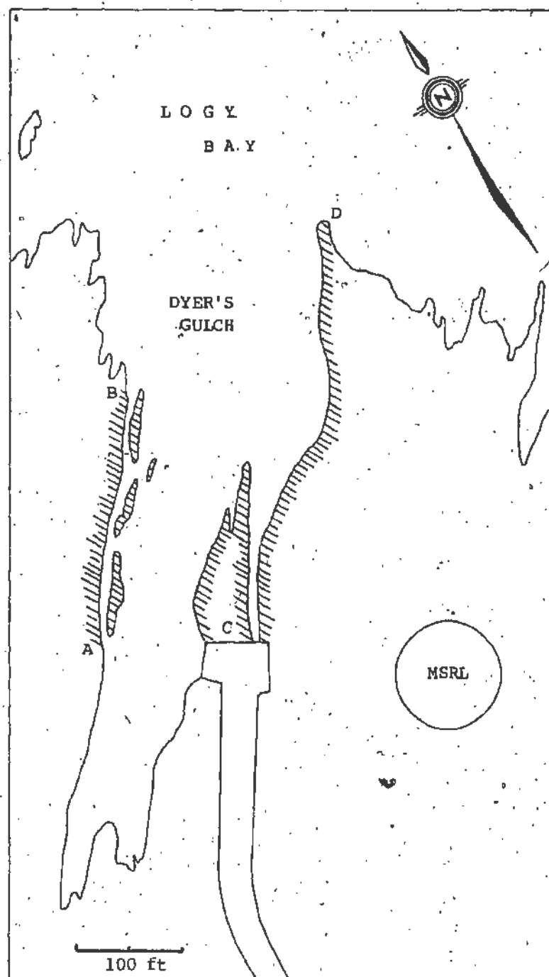
FIGURE 2: LOCATION OF STUDY AREAS (SHADED) IN DYER'S GULCH, LOGY BAY, NEWFOUNDLAND.
