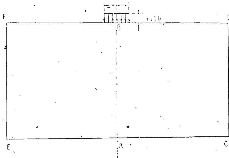
Figure 3.7.3. Finite element model for an ice sheet under partially distributed load.
