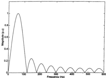
Figure 3.2: Frequency response of full cycle Fourier algorithm
