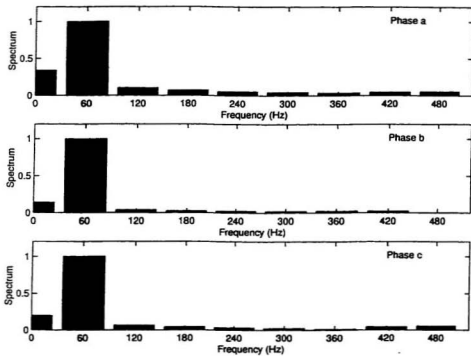
Figure 5.7(b): Frequency spectrum of phase currents for a three-phase fault at 60% of the line
