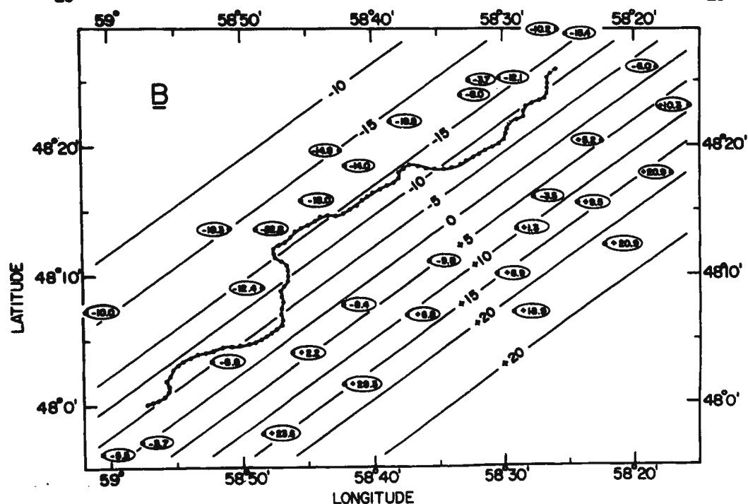
Figure 3.5.1 (B) Plot of traverse between distances 69 km and 142 km from Port-aux-Basques. Heavy dots with ovals show Dominion Observatory stations with Bouguer anomalies. Anomaly contours, with 5 mgal spacing, have been drawn on the basis of these and other Dominion Observatory values. (A) g_B , observed anomaly profile; g_C , regional gravity pattern obtained from contours (Figure 3.5.1(B); g_R , residual gravity profile.
