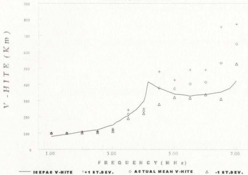
Figure 3.1: Ionograms based on Ionosondes and ICEPAC for Manitoba on March 1993 at 13.7 LT[34]
