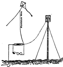
Figure 2.6: The Temporary receiving antenna used at Signal Hill for the Tranatlantic tests[1]
