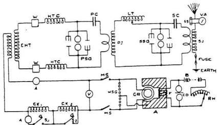
A, Alternator Frame; CR, Alternator Collector Rings; B, Battery; Rb, Rheostat; CD, Carbon Duc Protector across Field Windings; F, Alternator Field Windings; WSG, Wurtz Spark Gap Protector across Armature; MS, Main Switch; V, Voltmeter; A, Ammeter; CK1, CK2, Signalling Coiling Coils; S1, S2, Signalling Switches; EHT, Transformer 2000-20,000 volt ratio; HTC, High Tension Inductance; WW, Wurtz Arrestors; PC, Primary Condenser; PSG, Primary Spark Gap fitted with Condenser Protector; PJ, Primary Jigger; LT, Adjustable Tuning Inductance; SC, Secondary Condenser; SSG, Secondary Spark Gap with Protectors; SJ, Secondary Jigger; VA, Aerial Ammeter with SS Ammeter Sheath.
