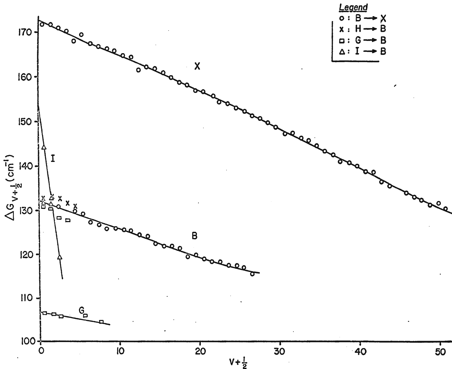
Fig.7. Mean \Delta G curves of observed states of diatomic bismuth ( plotted against v + \frac{1}{2} )
