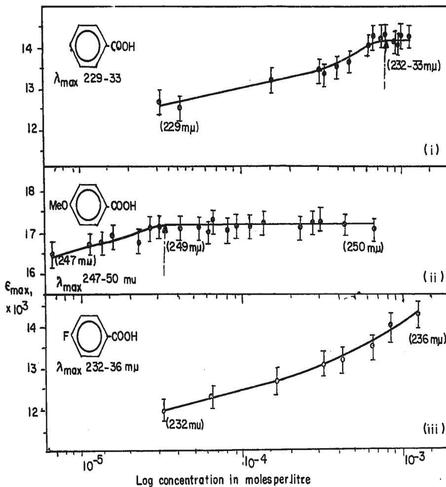
Fig. XI The variation of \epsilon_{\max} on changing the concentration for (i) benzoic acid in cyclohexane solution, (ii) anisic acid in cyclohexane solution containing 5% ether, and (iii) p-fluorobenzoic acid in cyclohexane solution.
