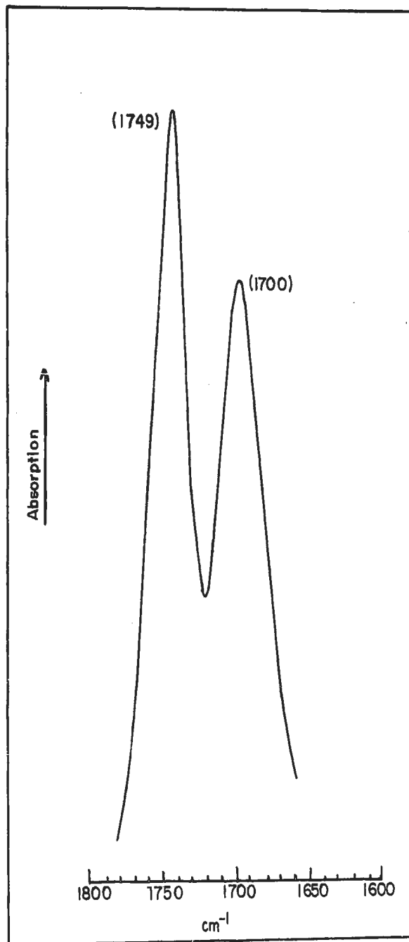
Fig. XVII The infrared carbonyl stretching bands in carbon tetrachloride solution at a concentration of ca. 3.5 \times 10^{-2} moles/litre for o -methoxybenzoic acid. Values of \nu_{\max} are given in brackets.
