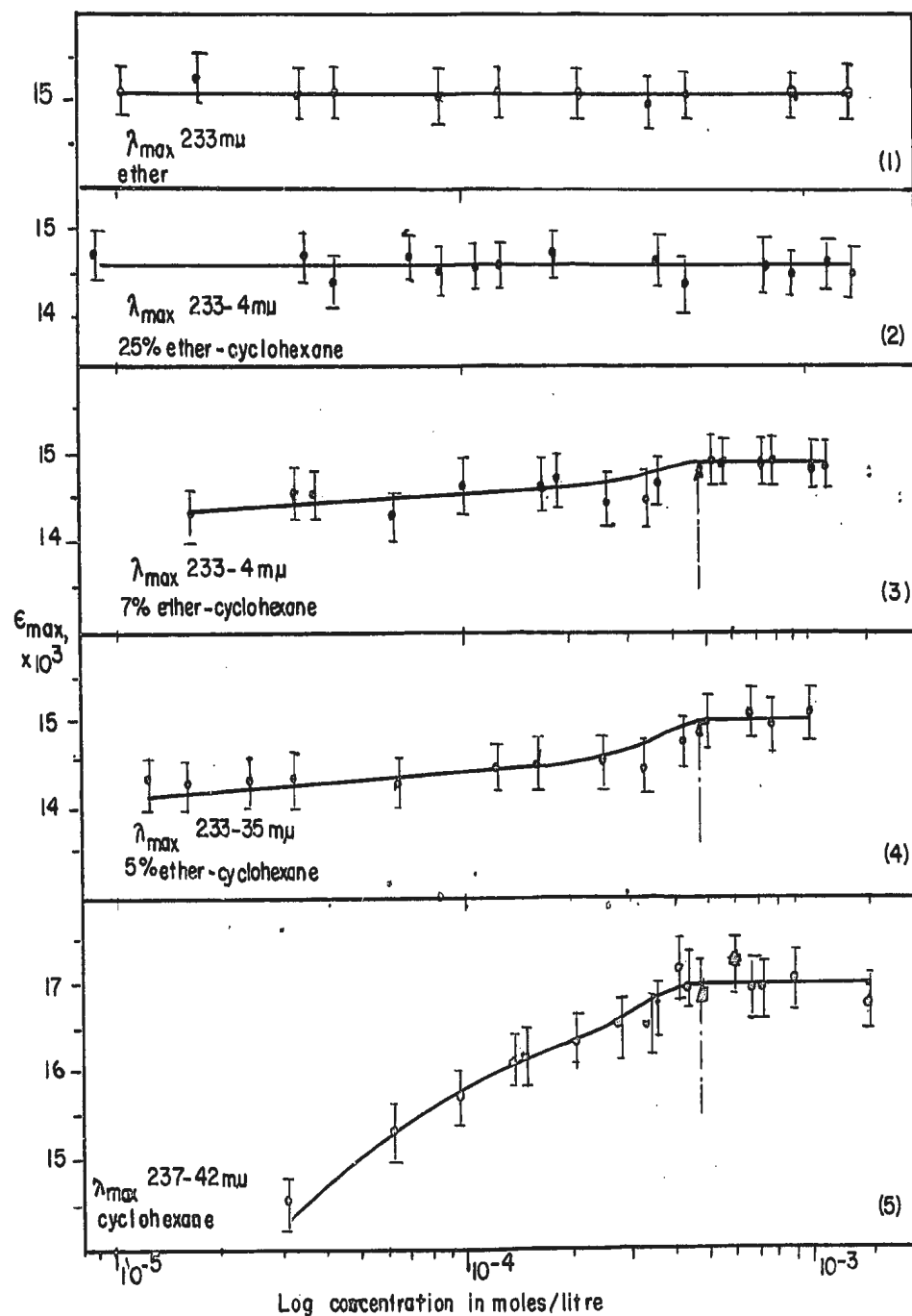
Fig. VIII The variation of \epsilon_{\max} on changing the concentration of acid for p-toluic acid in (1) ether solution, (2) cyclohexane solution containing 25% ether, (3) cyclohexane solution containing 7% ether, (4) cyclohexane solution containing 5% ether, and (5) cyclohexane solution.
