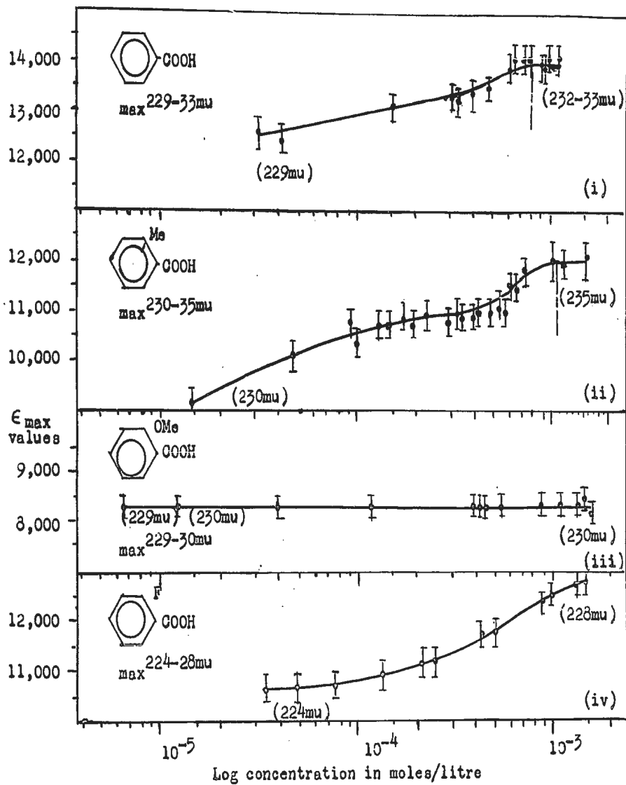
Fig. XV. The variation of \epsilon_{\max} on changing the solute concentration in cyclohexane solution for (i) benzoic acid, (ii) o-toluic acid, (iii) o-methoxybenzoic acid, and (iv) o-fluorobenzoic acid.
