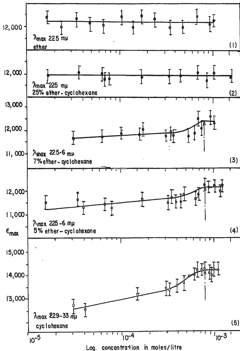
Fig. VII The variation of \epsilon_{\max} on changing the concentration of acid for benzoic acid in (1) ether solution (2) cyclohexane solution containing 25% ether, (3) cyclohexane solution containing 7% ether, (4) cyclohexane solution containing 5% ether, and (5) cyclohexane solution.
