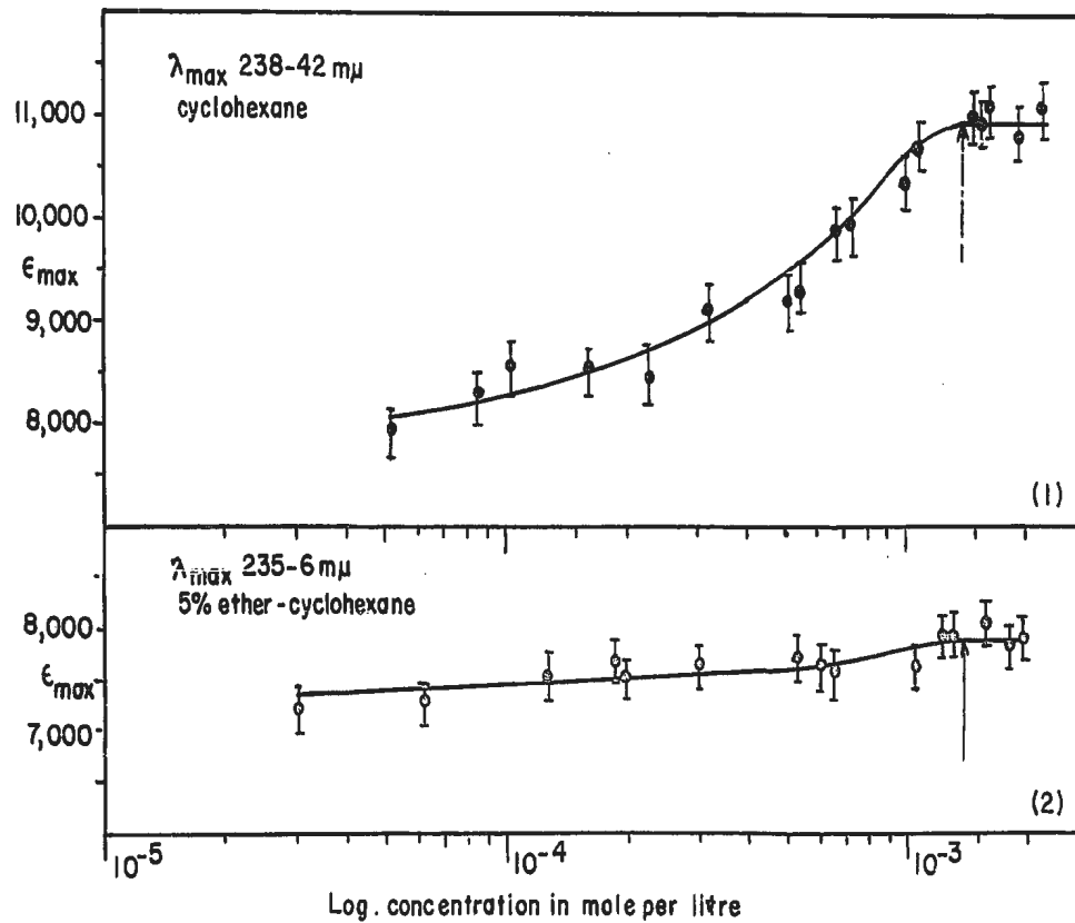
Fig. X The variation of \epsilon_{\max} on changing the concentration of acid for salicylic acid in (1) cyclohexane, and (2) cyclohexane solution containing 5% ether.
