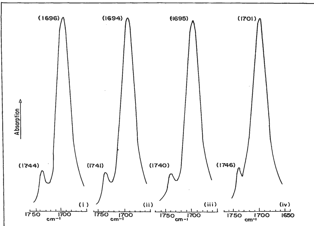
Fig. XIV. The infrared carbonyl stretching bands in \text{CCl}_4 solution at a concentration of ca. 3.5 \times 10^{-2} \text{ M} of (i) Benzoic, (ii) m-toluic, (iii) m-methoxybenzoic, and (iv) m-fluorobenzoic acid. Values of \nu_{\max} are given in brackets.
