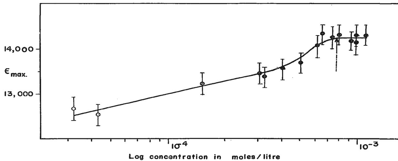
Fig. V Plot of maximal absorption against solute concentration for benzoic acid.
