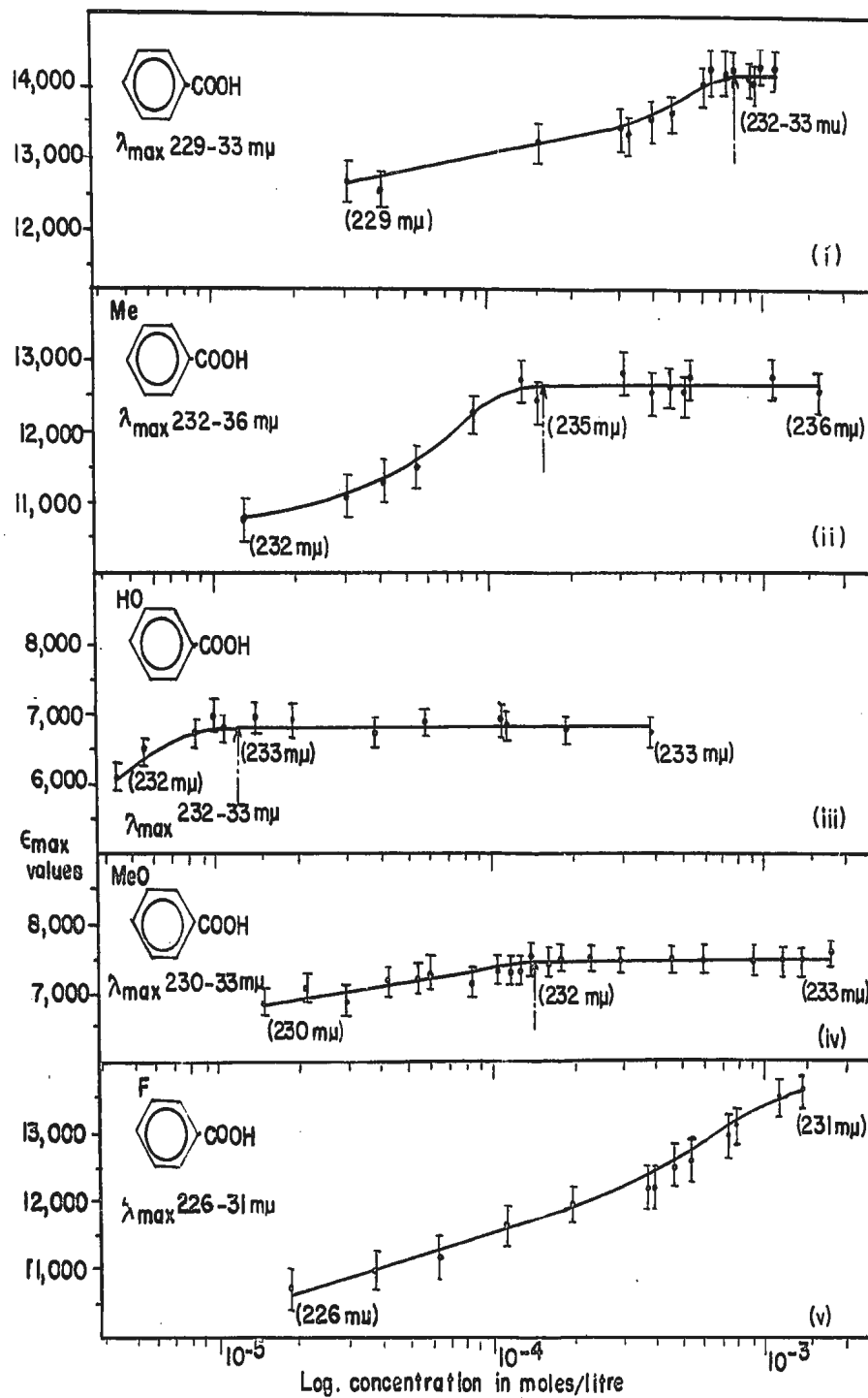
Fig. XIII The variation of \epsilon_{\max} on changing the solute concentration of (i) benzoic acid in cyclohexane solution, (ii) m -toluic acid in cyclohexane solution, (iii) m -hydroxybenzoic acid in cyclohexane containing 5% ether, (iv) m -methoxybenzoic acid in cyclohexane solution containing 5% ether, and (v) m -fluorobenzoic acid in cyclohexane solution.
