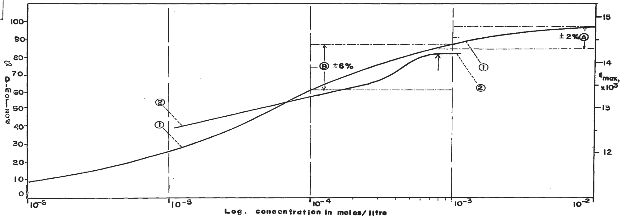
Fig. VI A plot of (1) calculated percentage of the total acid concentration in the dimerized form (theoretical curve) and (2) ultraviolet extinction coefficient, \epsilon_{\max} , (experimental curve) against log concentration for benzoic acid. Theoretical values were calculated from K = [D] / [M]^2 assuming K = \text{ca. } 1.6 \times 10^4 (cf. p.18).
