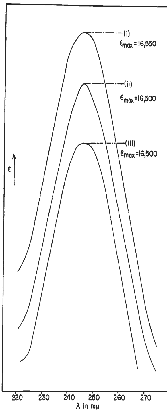
Fig. II The B-band of diphenyl in cyclohexane (bands shifted vertically for clarity)
