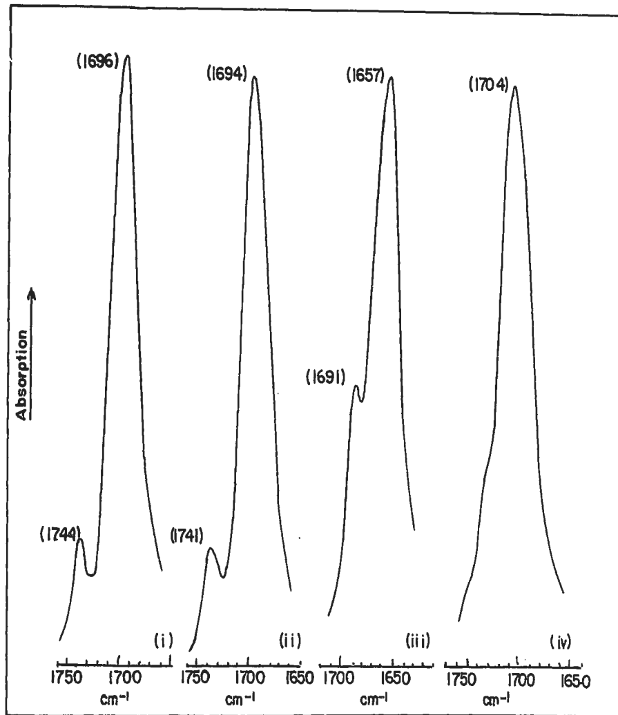
Fig. XVI The infrared carbonyl stretching bands in carbon tetrachloride solution at a concentration of ca. 3.5 \times 10^{-2} moles/litre of (i) benzoic acid, (ii) o -toluic acid, (iii) salicylic acid, and (iv) o -fluorobenzoic acid. Values of \nu_{\max} are given in brackets.
