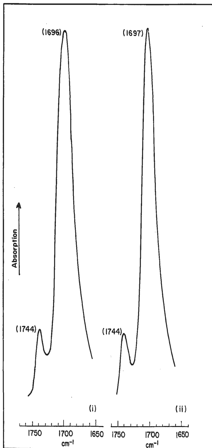
Fig. XII The infrared carbonyl stretching bands in carbon tetrachloride solution at a concentration of ca. 3.5 \times 10^{-2} moles/litre of (i) benzoic acid (ii) p-fluorobenzoic acid. Values of \nu_{\text{max}} are given in brackets.
