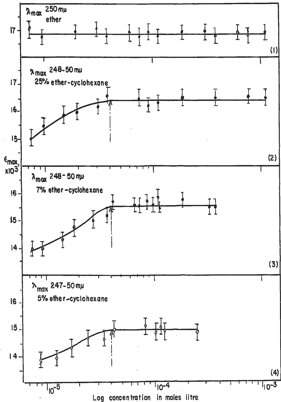
Fig. IX The variation of \epsilon_{max} on changing the solute concentration for p-hydroxybenzoic acid in (1) ether solution, (2) cyclohexane solution containing 25% ether, (3) cyclohexane solution containing 7% ether, and (4) cyclohexane solution containing 5% ether.
