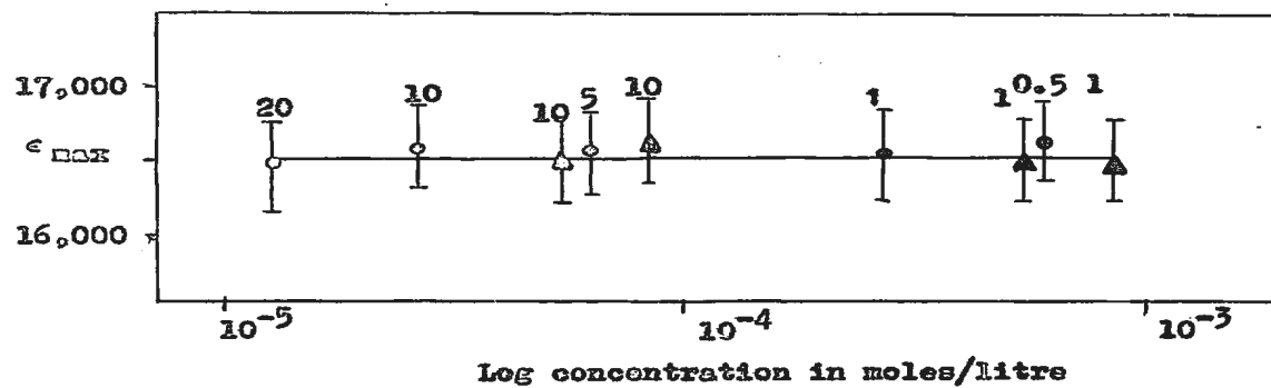
Fig. III Plot of \epsilon_{\text{MAX}} vs. log concentration for diphenyl in cyclohexane. The number above each point is the cell length in mm. Values obtained using pure cyclohexane in the solvent cell are given as ●, while those obtained with a solution of diphenyl in cyclohexane in the solvent cell are shown as ▲.
