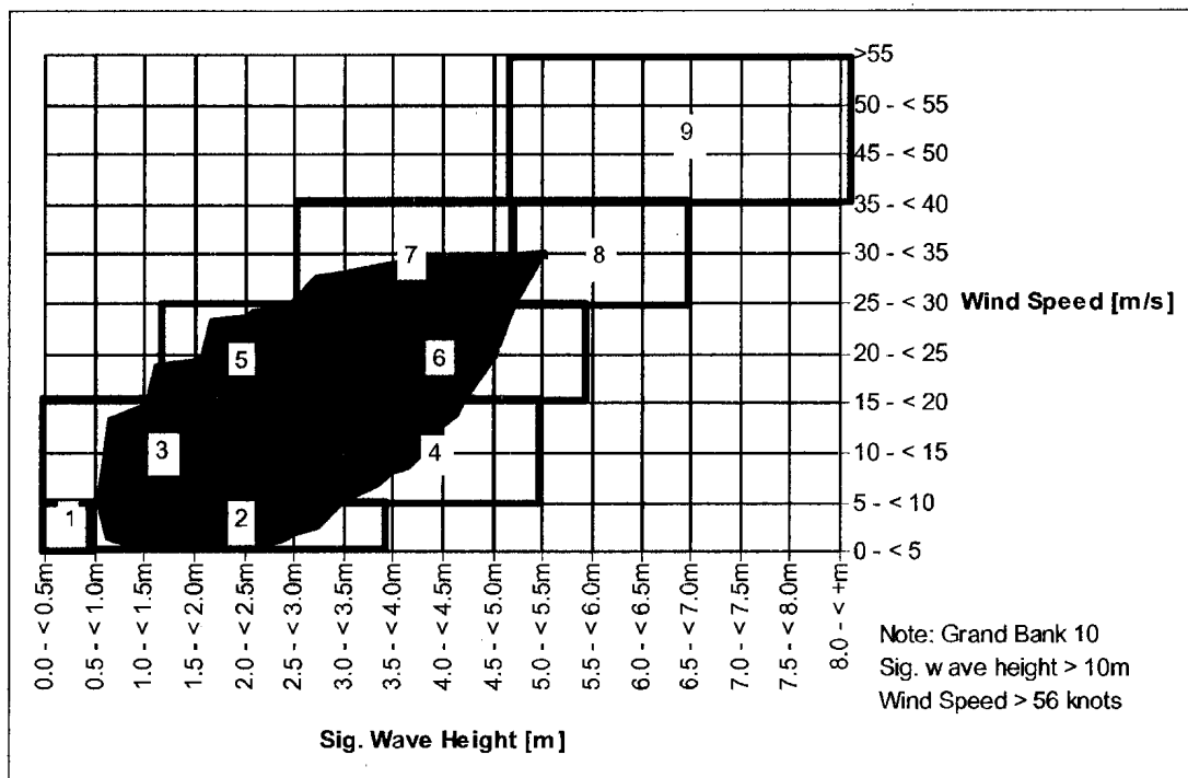
Figure 2.17: Grand Banks scale (significant wave height & wind speed)
