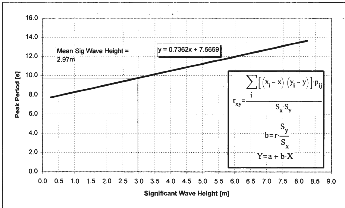
Figure 2.16: Peak period versus significant wave height model
