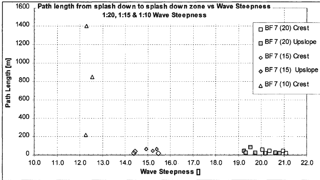
Figure 4.41: Path length from splash down to splash down zone versus wave steepness
