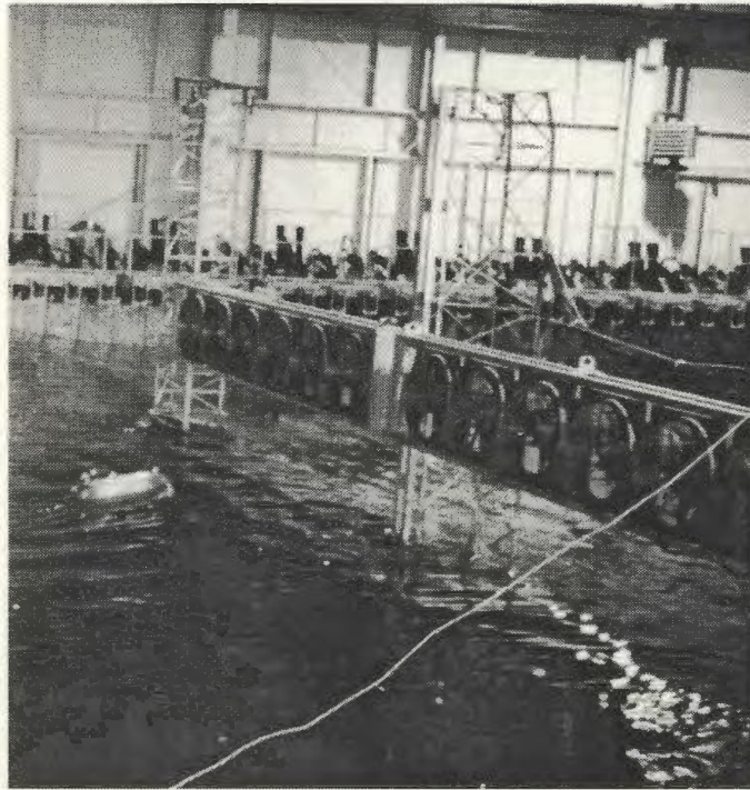
Figure 5.7: Original wind machine setup for tests reported in 2002
