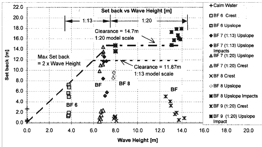
Figure 4.2: Set back versus wave height (perpendicular orientation)
