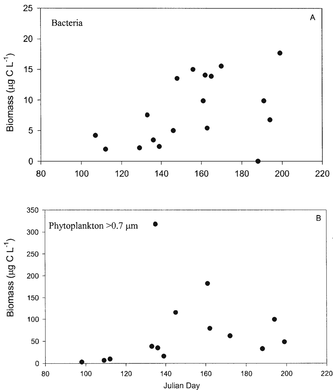
Figure 3.3 Bacteria and total chlorophyll a (>0.7µm) biomass, in the North Water Polynya at stations where dilution experiments were conducted from April through July, 1998
