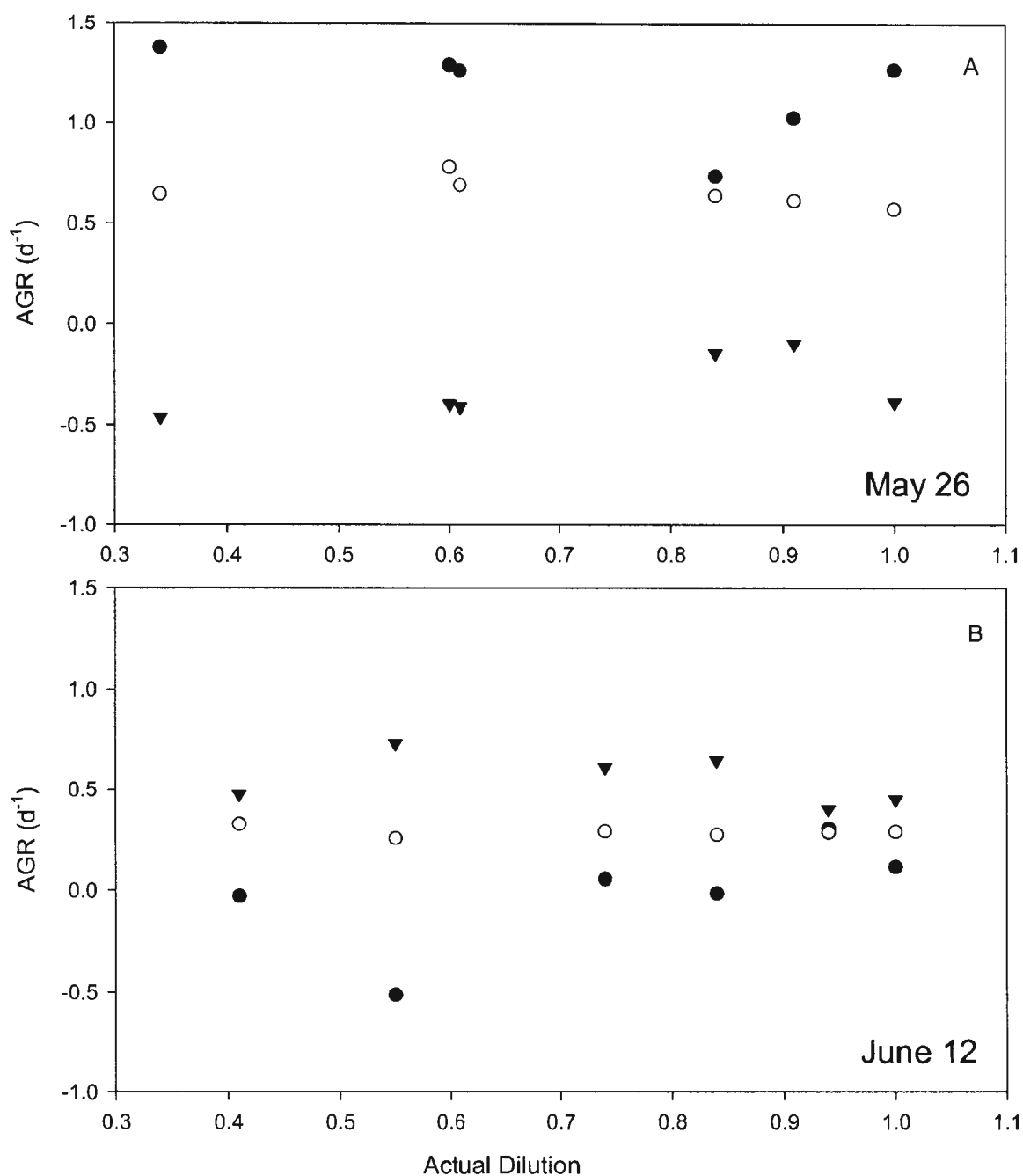
Figure 3.7 Two representative dilution plots of bacteria in the North Water Polynya in 1998. Three size classes are presented in each graph : small (<0.5 \mu\text{m} ) closed circles; medium (0.5 - 1.0 \mu\text{m} ) open circles; and large (>1.0 \mu\text{m} ) closed triangles. Growth and grazing mortality for each size class are calculated from the regression between apparent growth rate (AGR) and actual dilution.
