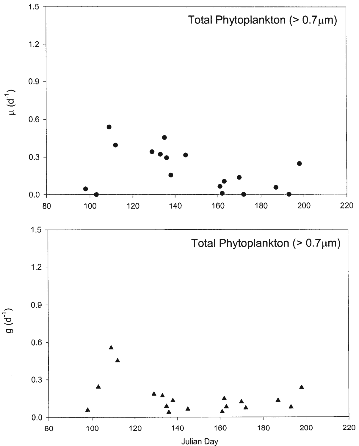
Figure 2.3 Phytoplankton (> 0.7 \mu\text{m} ) growth ( \mu ) and grazing mortality ( g ) rates measured in the North Water Polynya from April 8 through July 17, 1998.
