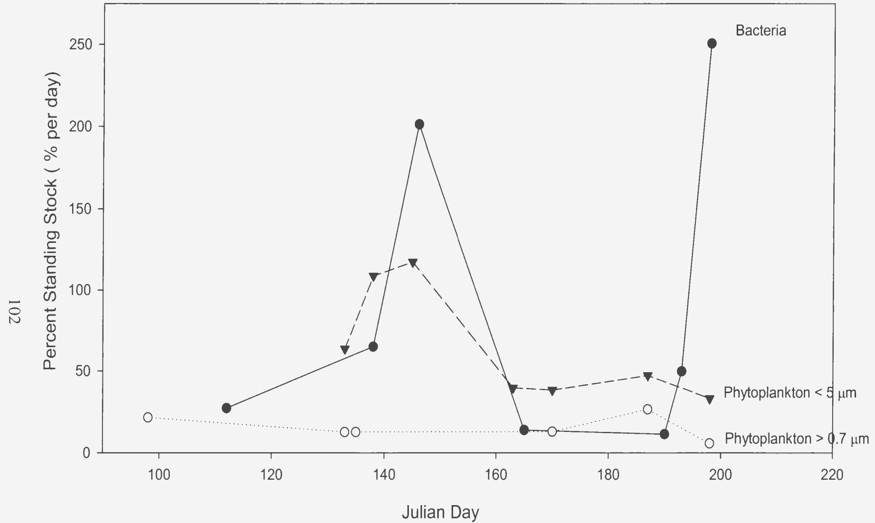
Figure 2.22 Calculated percent standing stock consumed of the various prey types - phytoplankton ( >0.7 \mu\text{m} , >5 \mu\text{m} , <5 \mu\text{m} ) and bacteria, throughout the North Water Polynya as the study progressed from April to July, 1998.
