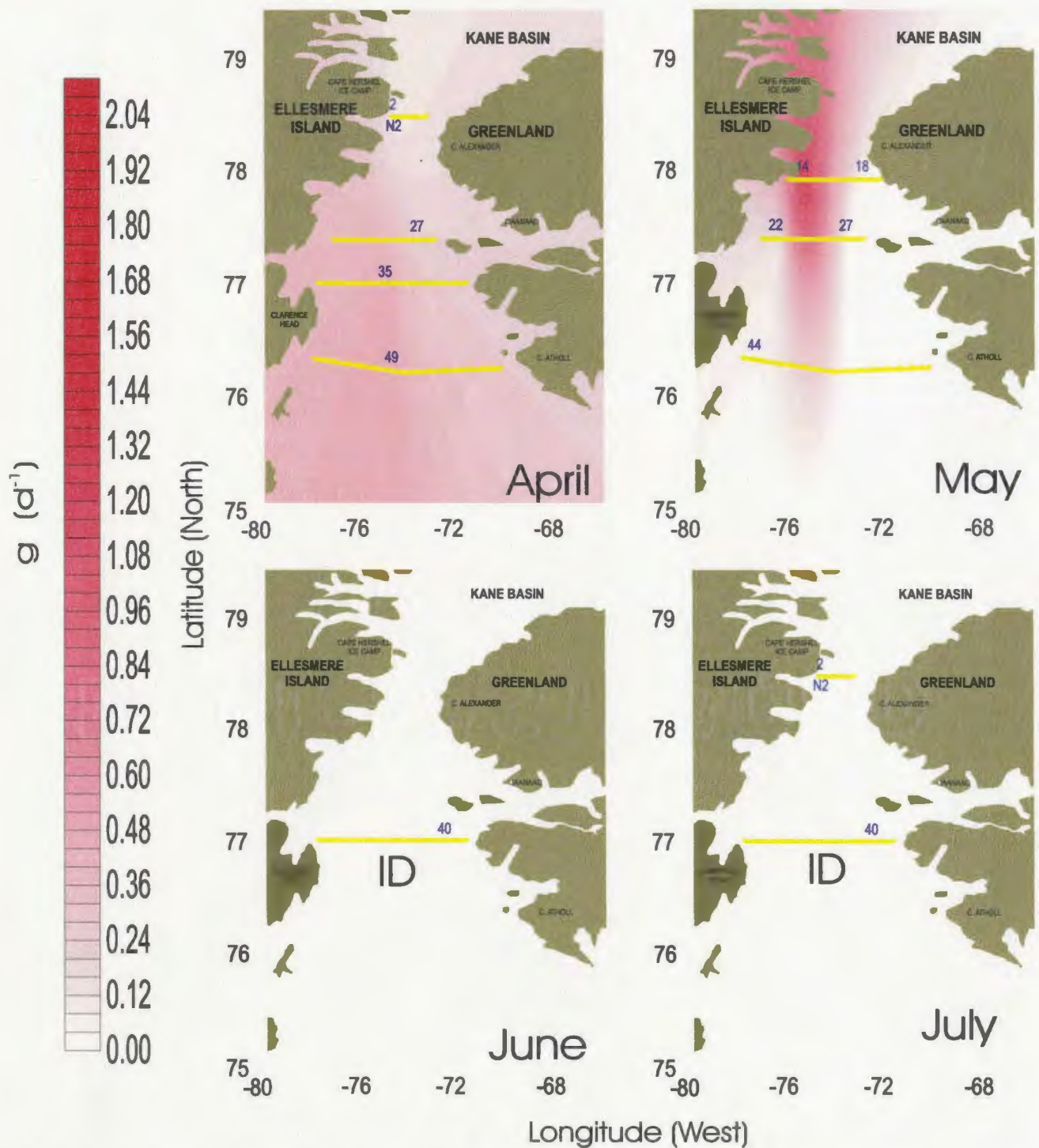
Fig.2.14 Spatial trends in grazing mortality ( g ) of large phytoplankton ( >5 \mu m ) throughout the North Water Polynya during April, May, June and July, 1998.
