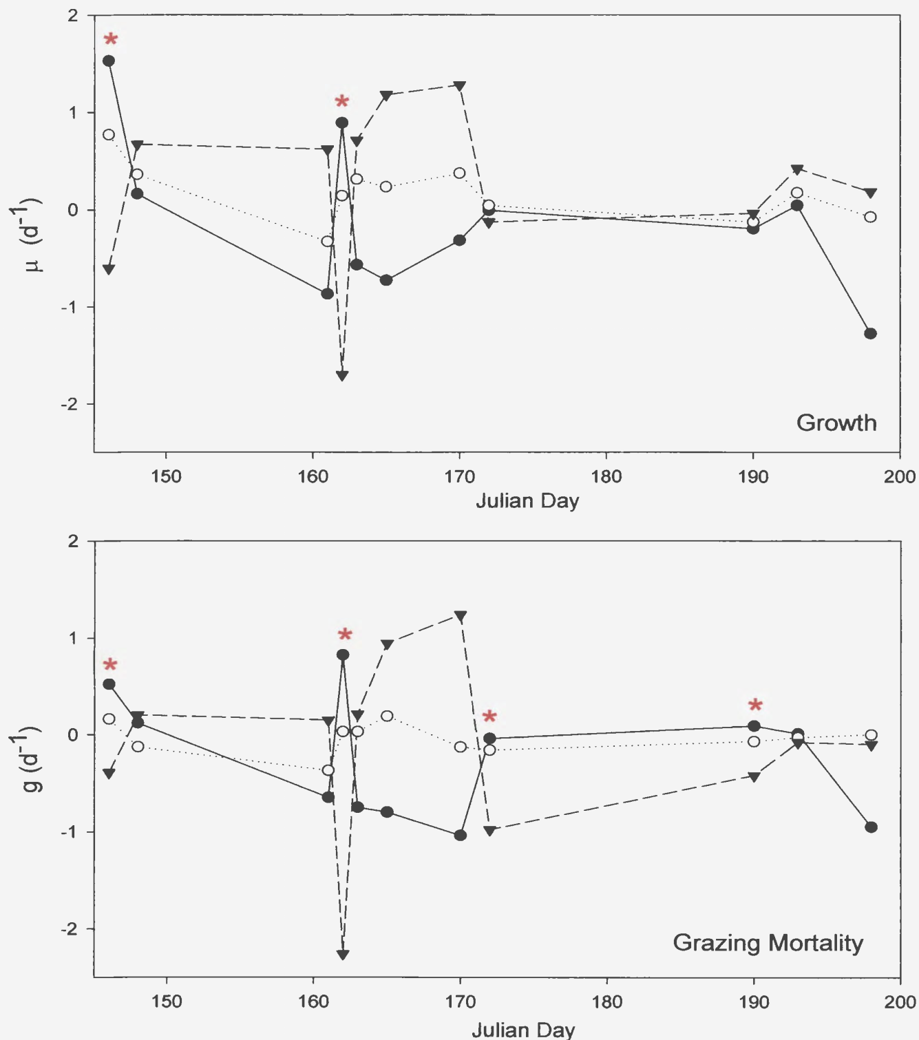
Figure 3.8 Rates of growth ( \mu ) and grazing mortality rates ( g ) for three size classes of bacteria (Small <5 \mu m , closed circles; Medium 0.5 - 1.0 \mu m , open circles; Large > 1.0 \mu m , closed triangles) measured in the North Water Polynya from May to July, 1998. Asterisks ( * ) represents experiments of interest which are discussed in the text.
