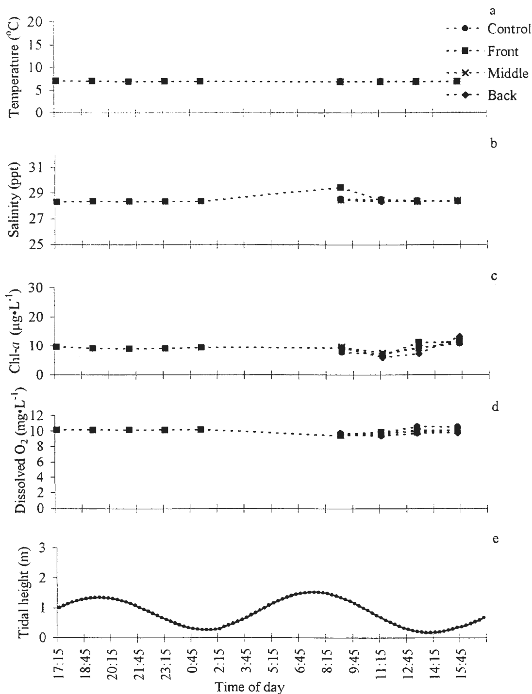
Appendix 4.12: Short-term environmental (tidal) data collected at Reach Run, Nov. 4-5, 1998; measured at the control station and three lines in the front, middle and back of the farm at 3.5 m depth with a CTD, a) temperature, b) salinity, c) chlorophyll-a, d) dissolved oxygen e) tidal height at time of sampling.
