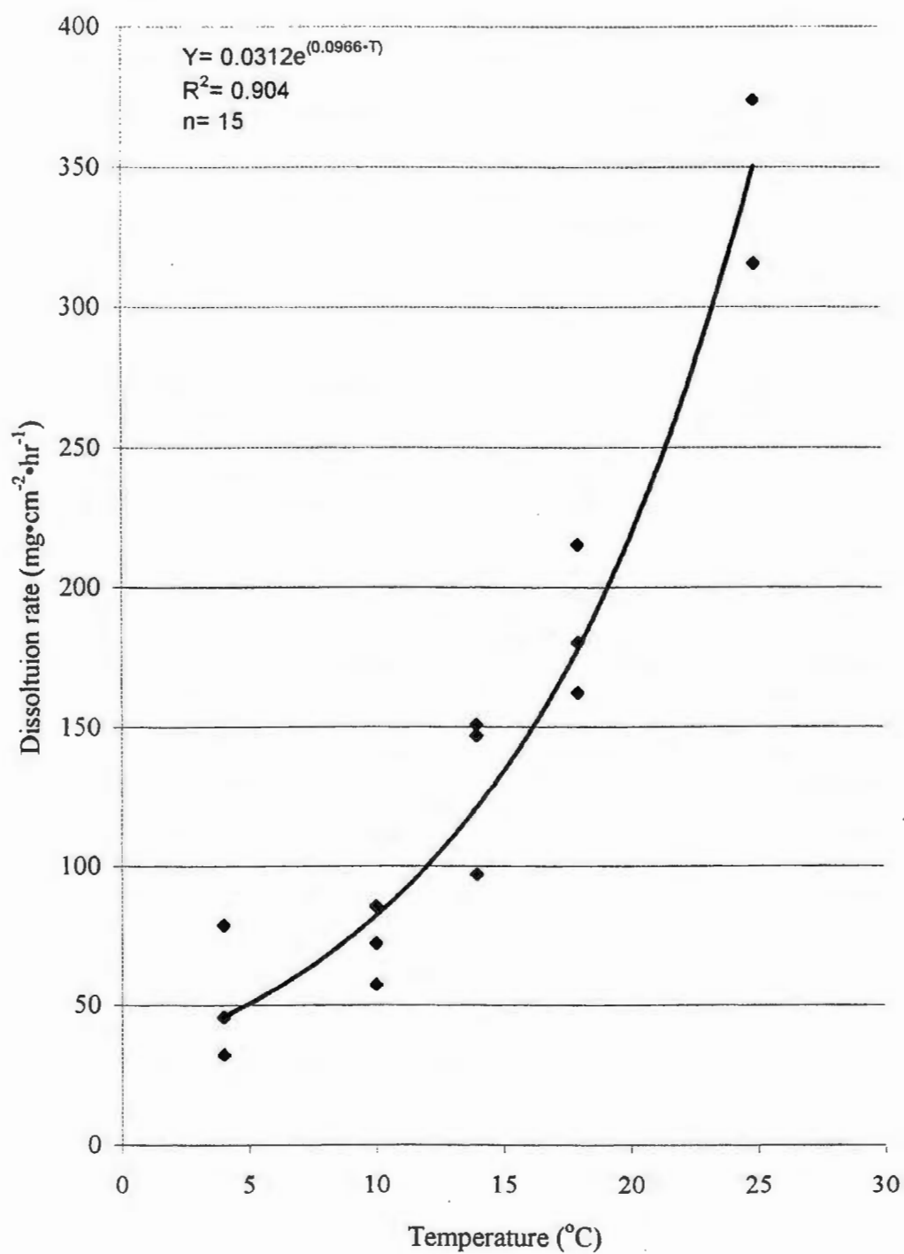
Appendix 1.1: The effects of temperature on dissolution of plaster cylinders. Dissolution based on weight of loss of dry cylinders per unit surface area per hour.
