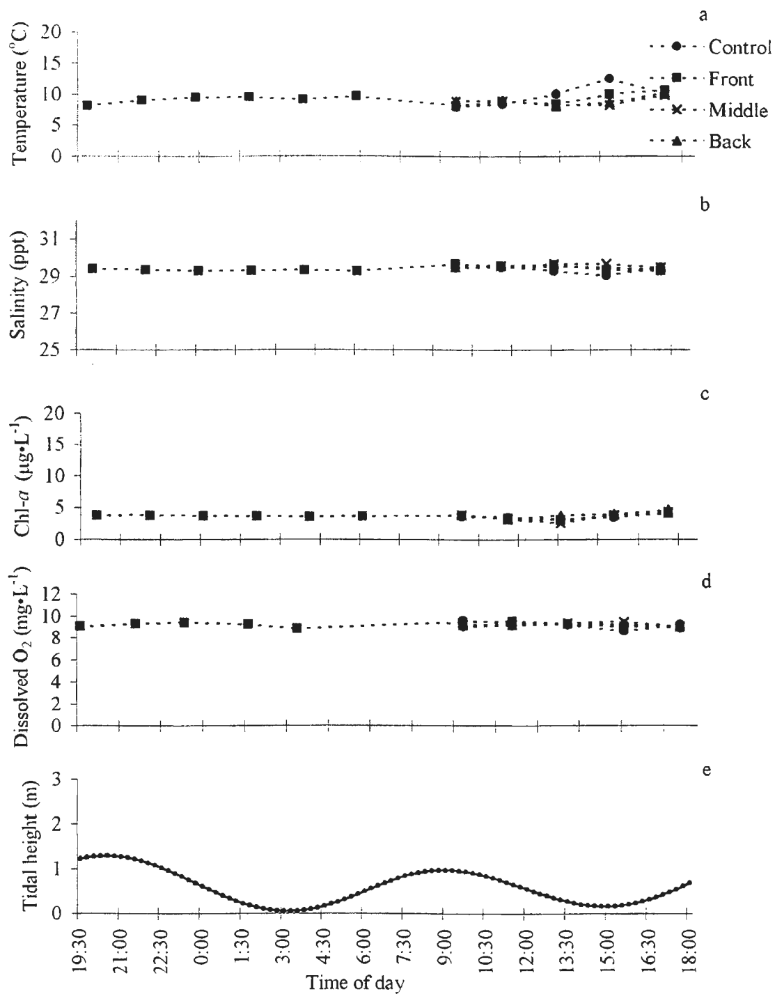
Appendix 4.14: Short-term environmental (tidal) data collected at Big Island, June 25-26, 1998; measured at the control station and three lines in the front, middle and back of the farm at 3.5 m depth with a CTD, a) temperature, b) salinity, c) chlorophyll-a, d) dissolved oxygen e) tidal height at time of sampling.
