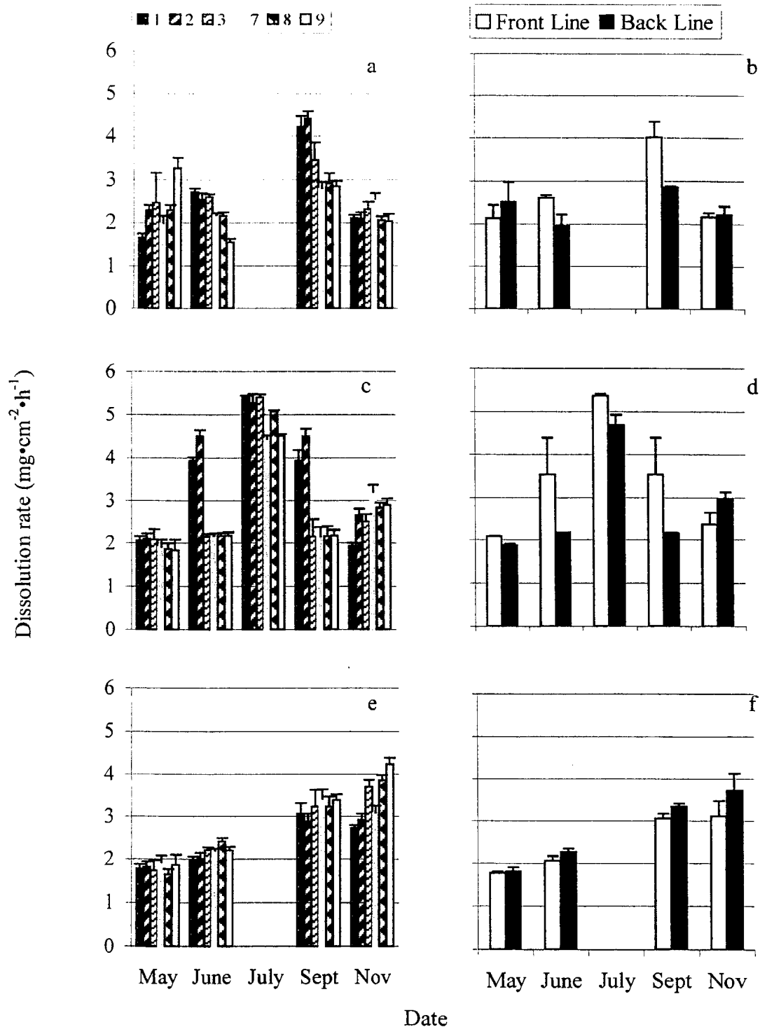
Figure 8. Seasonal dissolution rates (mg·cm -2 ·h -1 ) of cylinders placed at 3.5 m (a, c, e) at stations 1-3 and 7-9 in a) Burnt Arm c) Reach Run and e) Big Island. Experimental longline averages at 3.5 m (b, d, f) in b) Burnt Arm, d) Reach Run and f) Big Island (n=5, error bars= standard error).
