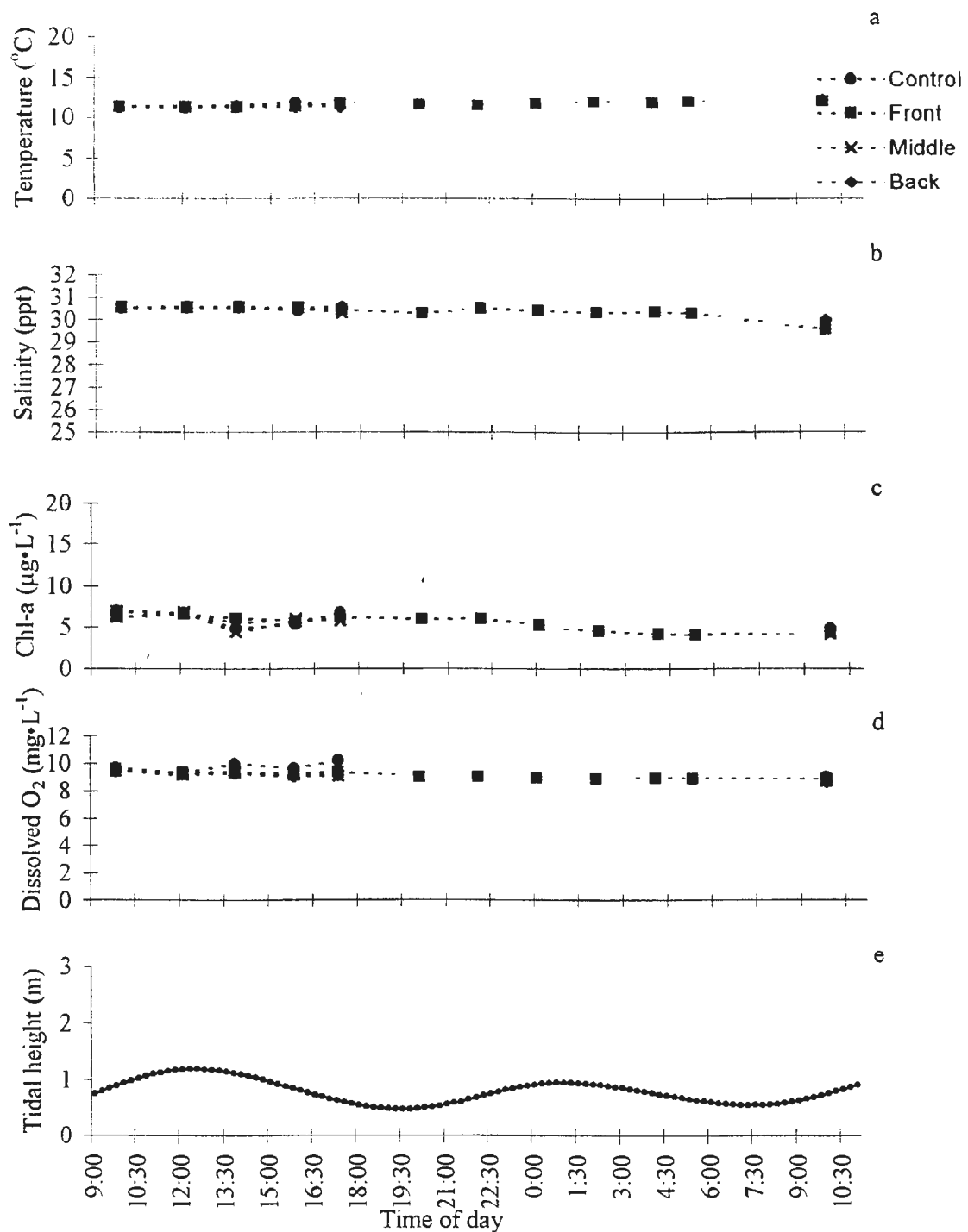
Appendix 4.4: Short-term environmental (tidal) data collected at Burnt Arm, Sept. 13-14, 1998; measured at the control station and three lines in the front, middle and back of the farm at 3.5 m depth with a CTD, a) temperature, b) salinity, c) chlorophyll-a, d) dissolved oxygen e) tidal height at time of sampling.
