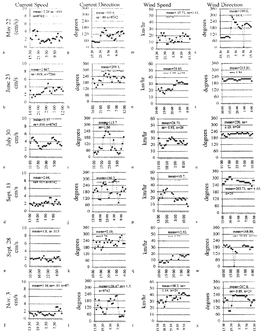
Appendix 5.1: Hourly current speed a)-f) and current direction g)-l) measured with an S4 current meter in Burnt Arm, Notre Dame Bay, NL (station 2) on May 22, June 23, July 30, Sept. 13, Sept. 28 and Nov. 3, respectively; Hourly wind speed m)-r) and direction s)-x) collected in the Twillingate, NL on the above dates (source Environment Canada, Twillingate, NL, n= 3 per point ).
