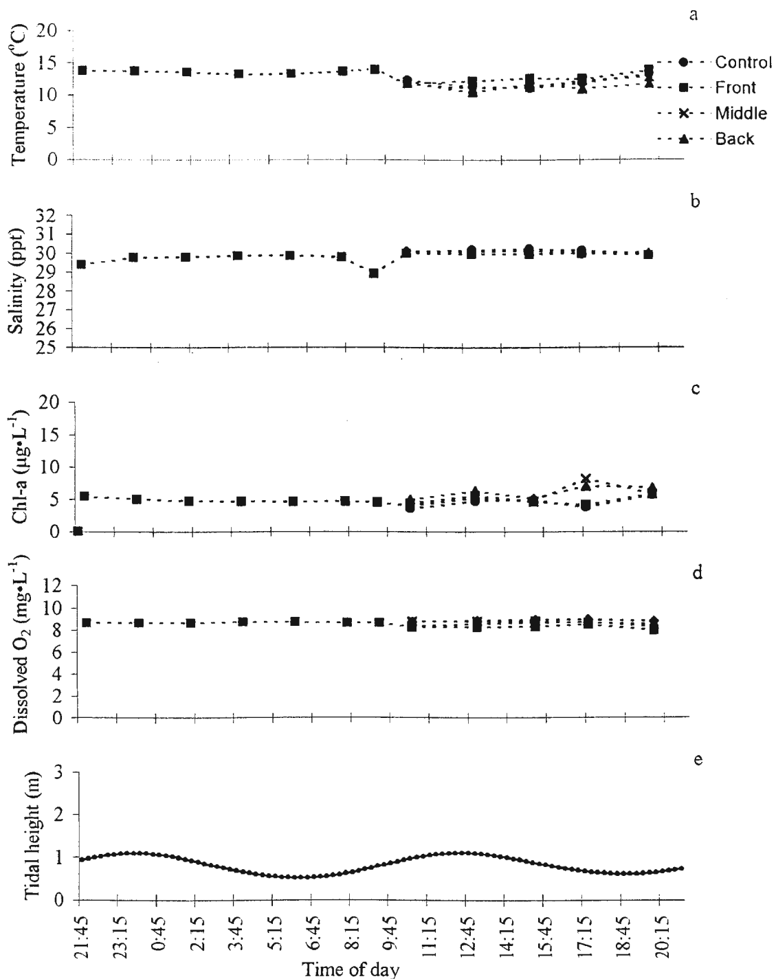
Appendix 4.3: Short-term environmental (tidal) data collected at Burnt Arm, July 30-31, 1998; measured at the control station and three lines in the front, middle and back of the farm at 3.5 m depth with a CTD, a) temperature, b) salinity, c) chlorophyll-a, d) dissolved oxygen e) tidal height at time of sampling.
