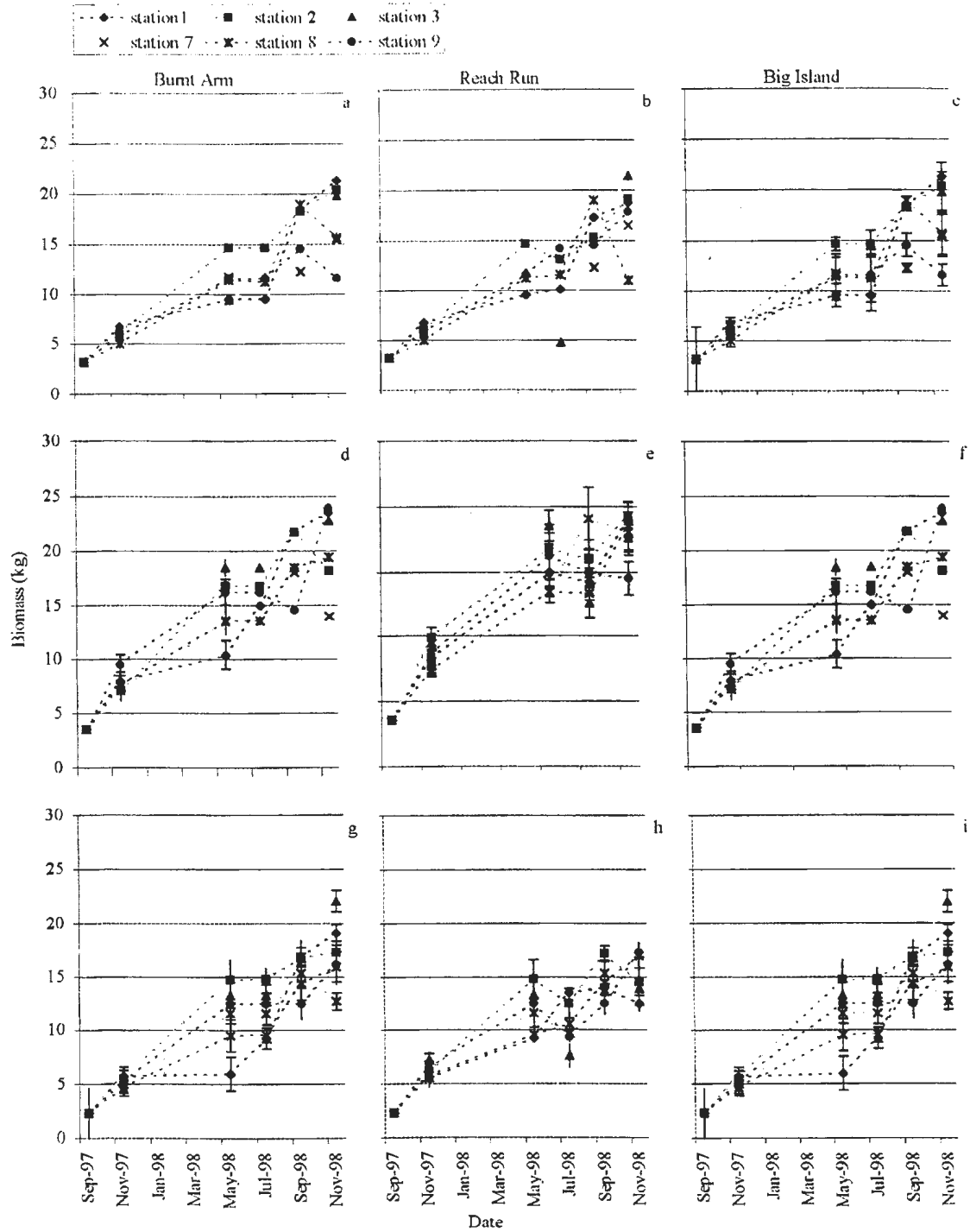
Figure 12.1: Summary of increasing biomass by sock weight (kg) of Reach Run mussels (a-c); Burnt Arm mussels (d-f); Big Island mussels (g-i) transplanted to Burnt Arm (column 1), Reach Run (column 2) and Big Island (column 3), respectively (n= 2, error bars= standard error).
