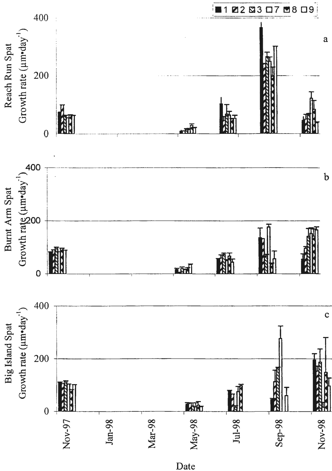
Figure 11.3. Average growth rate ( \mu\text{m}\cdot\text{d}^{-1} ) per station for Reach Run spat (a), Burnt Arm spat (b) and Big Island spat (c), transplanted to Big Island ( n=100 mussels, error bars= standard error).
