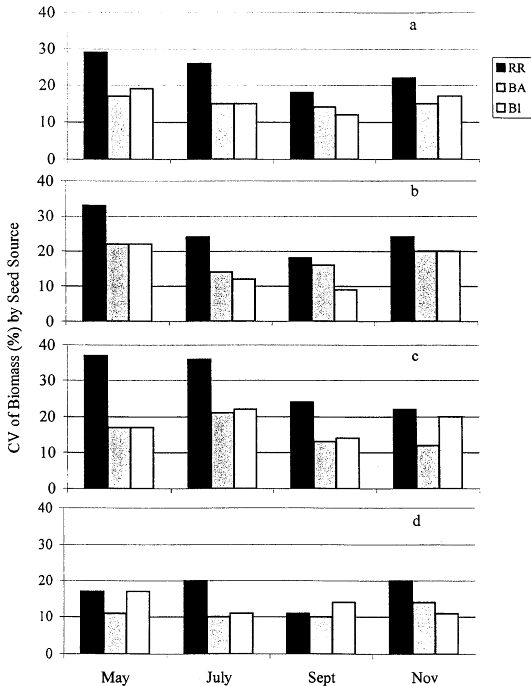
Figure 13.1. Coefficient of variation ( CV = \text{standard deviation} \cdot \text{mean}^{-1} ) of mussel biomass by seed source at a) all three sites, at sample stations at b) Burnt Arm, c) Reach Run, and d) Big Island.
