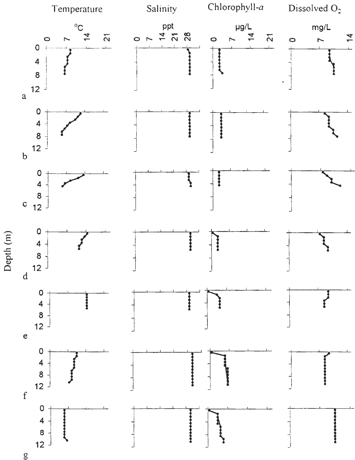
Figure 6.3. Vertical depth profiles of environmental data averaged from all 10 static at Big Island on a) May 30, b) June 26, c) July 8, d) August 5, e) September 3, f) October 2 and g) November 8, 1998.
