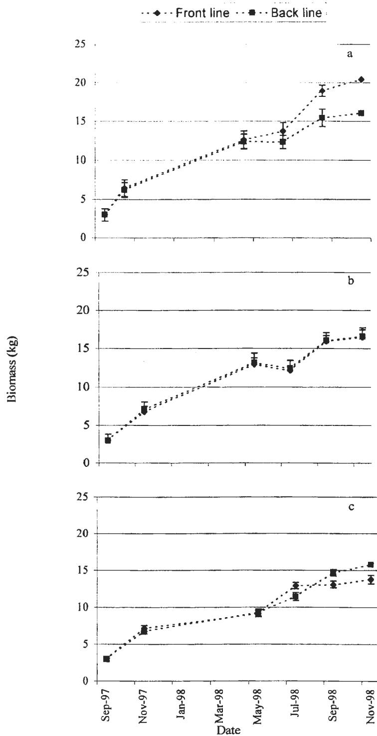
Figure 12.2. Summary of yield of all mussels grown at a) Burnt Arm, b) Reach Run and c) Big Island on the front and back longline of the experimental area (error bars= standard error, n=18).
