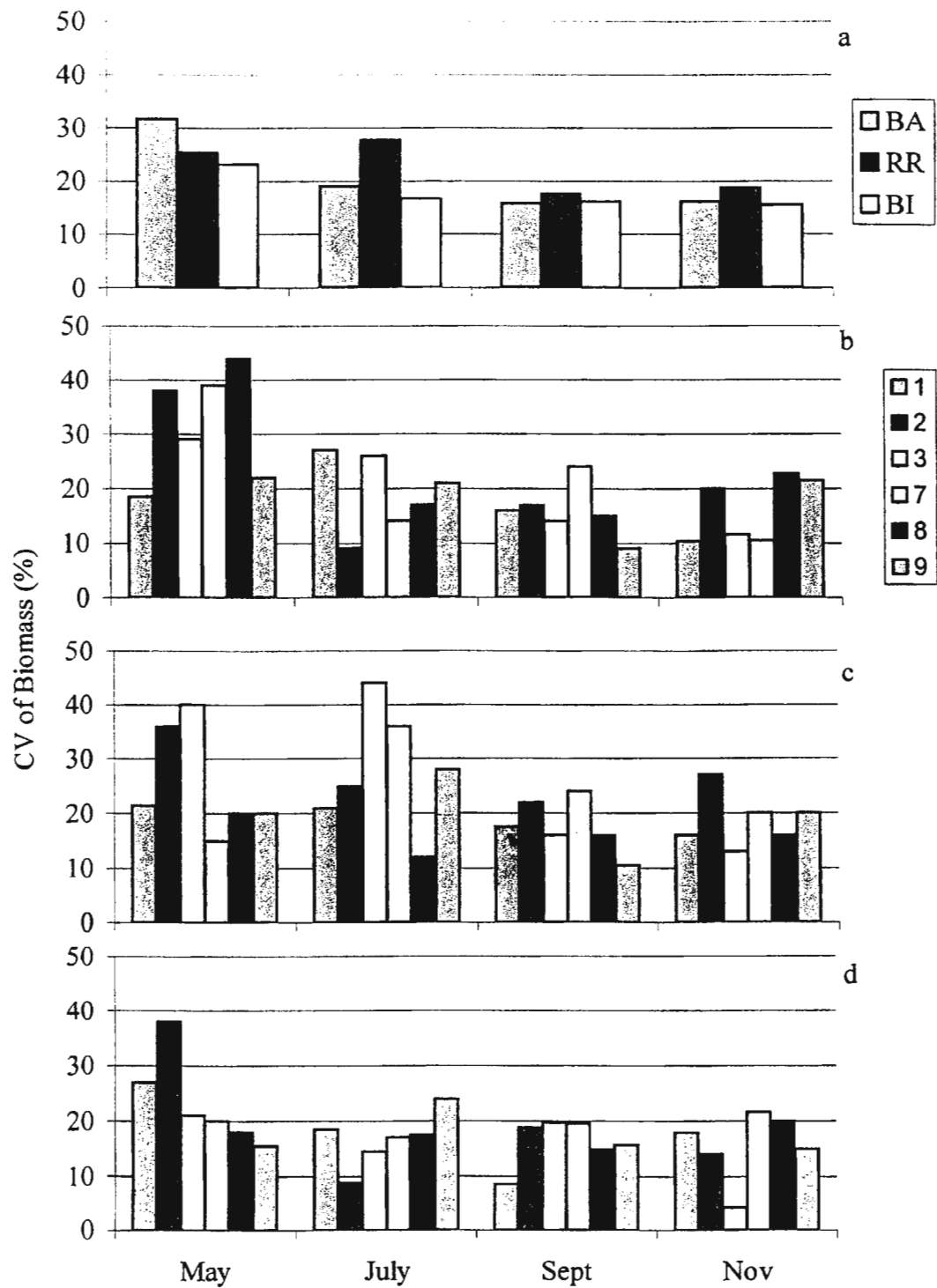
Figure 13. Coefficient of variation ( CV = \text{standard deviation} \cdot \text{mean}^{-1} ) of mussel biomass at a) all three sites, at sample stations at b) Burnt Arm, c) Reach Run, and d) Big Island.
