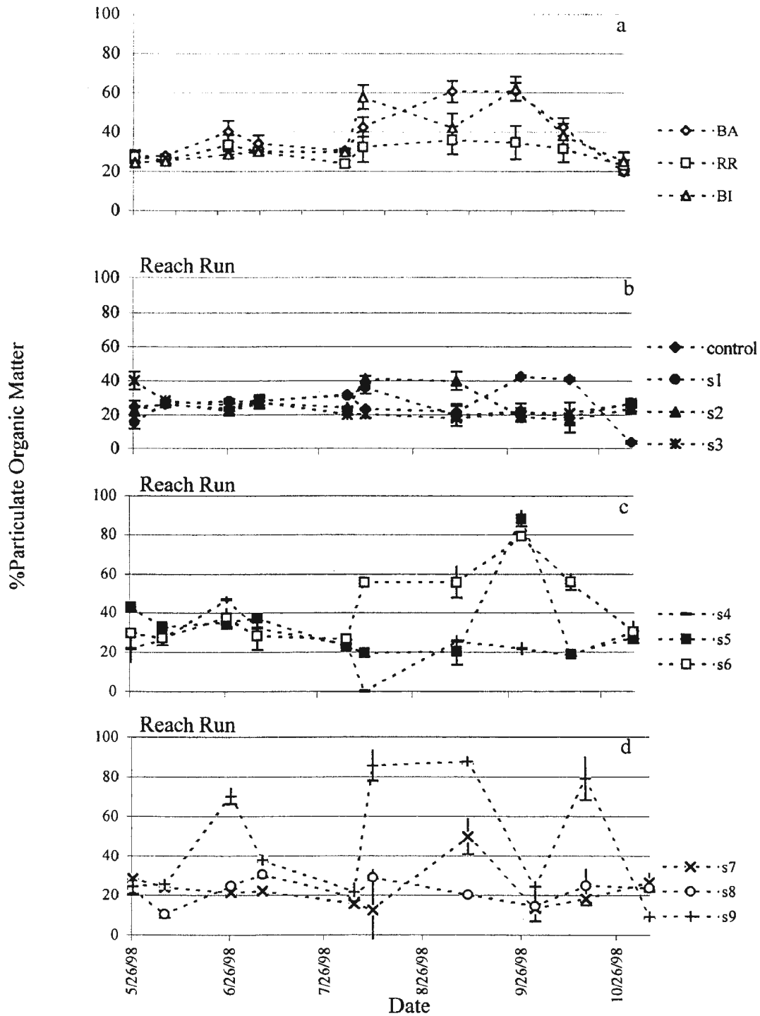
Figure 7.2. a) Percent POM averaged over all stations at Burnt Arm (BA), Reach Run (RR) and Big Island (BI) at 3.5 m, %POM in Reach Run at station b) control, 1, 2 and 3 c) 4, 5 and 6 and d) 7, 8 and 9, respectively (error bars= standard error).
