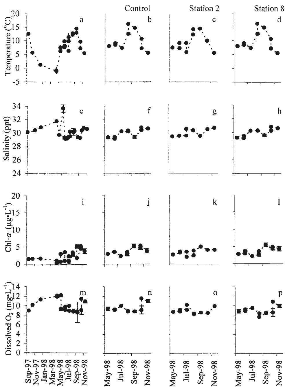
Figure 5.3. Environmental data collected at Big Island, Sept. 1997 – Nov. 1998 at 3.5 m. Column 1 represents data collected in this study as well as another NAIA sponsored study, column 2 represents data from this study collected at the control station located at the outside each farm, column 3 represents data collected at station 2, positioned at the front of each farm, column 4 represents data collected at station 8 positioned at the back of each farm. Each row represents temperature, salinity, chlorophyll- a and dissolved oxygen, respectively (n= 3-5 per point, error bars= standard error).
