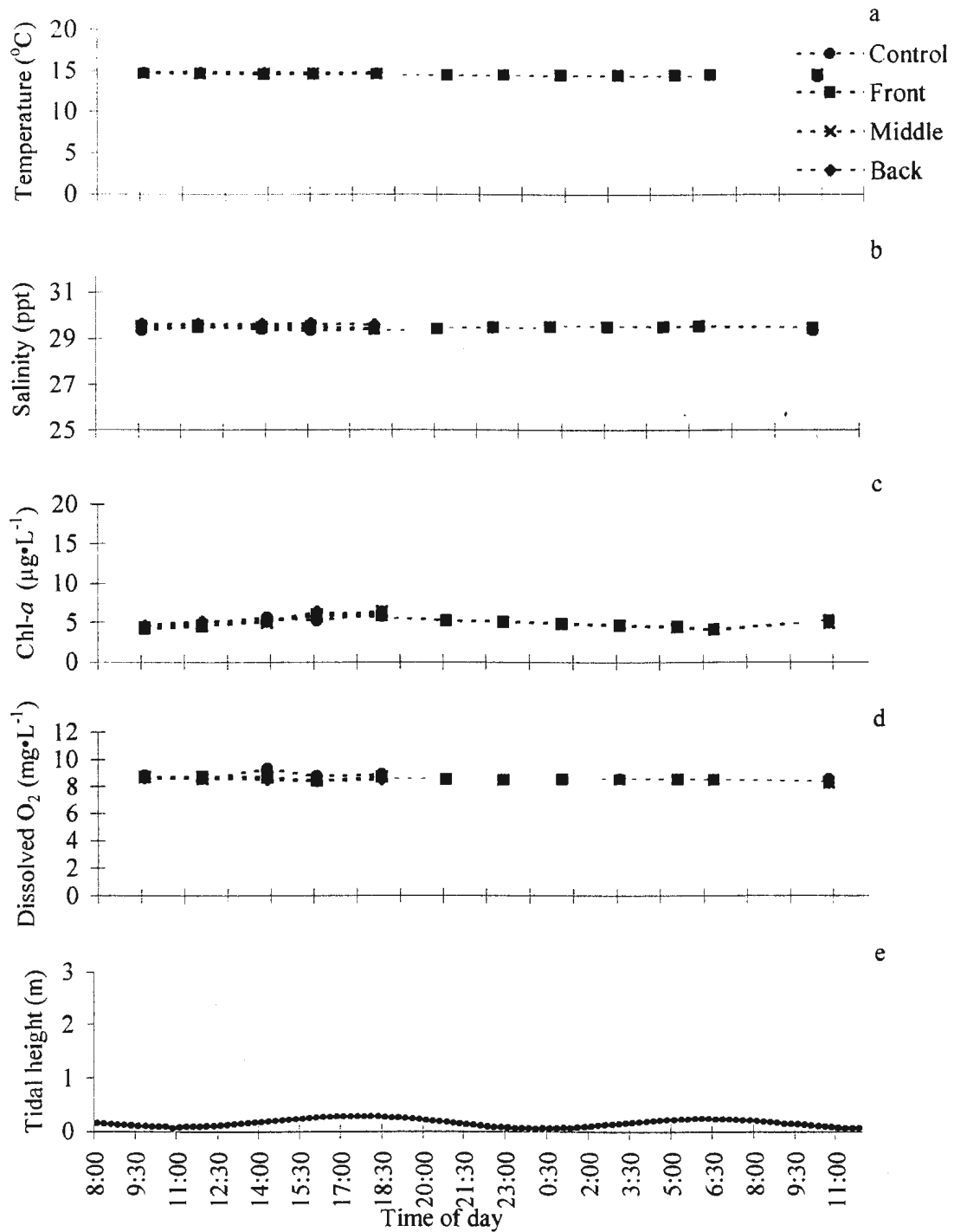
Appendix 4.16: Short-term environmental (tidal) data collected at Big Island, Sept. 3-4, 1998; measured at the control station and three lines in the front, middle and back of the farm at 3.5 m depth with a CTD, a) temperature, b) salinity, c) chlorophyll-a, d) dissolved oxygen e) tidal height at time of sampling.
