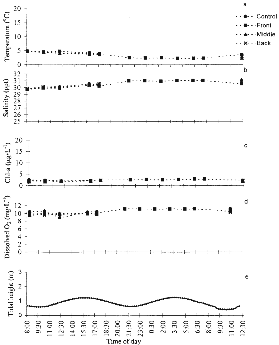
Appendix 4.1: Short-term environmental (tidal) data collected at Burnt Arm, May 21-22, 1998; measured at the control station and three lines in the front, middle and back of the farm at 3.5 m depth with a CTD, a) temperature, b) salinity, c) chlorophyll-a, d) dissolved oxygen e) tidal height at time of sampling.
