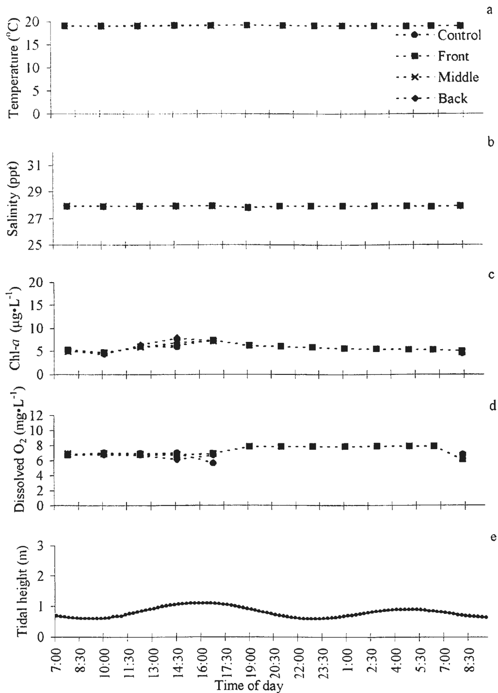
Appendix 4.9: Short-term environmental (tidal) data collected at Reach Run, Aug. 3-4, 1998; measured at the control station and three lines in the front, middle and back of the farm at 3.5 m depth with a CTD, a) temperature, b) salinity, c) chlorophyll-a, d) dissolved oxygen e) tidal height at time of sampling.
