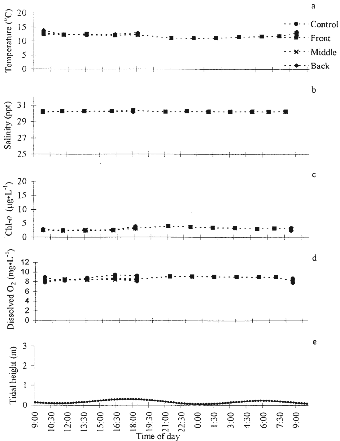
Appendix 4.15: Short-term environmental (tidal) data collected at Big Island, Aug. 4-5, 1998; measured at the control station and three lines in the front, middle and back of the farm at 3.5 m depth with a CTD, a) temperature, b) salinity, c) chlorophyll-a, d) dissolved oxygen e) tidal height at time of sampling.
