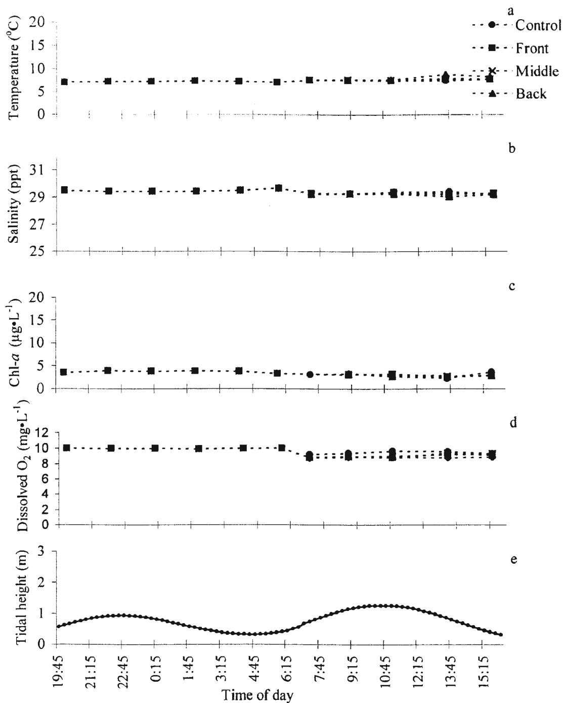
Appendix 4.13: Short-term environmental (tidal) data collected at Big Island, May 28-29, 1998; measured at the control station and three lines in the front, middle and back of the farm at 3.5 m depth with a CTD, a) temperature, b) salinity, c) chlorophyll- a , d) dissolved oxygen e) tidal height at time of sampling.
