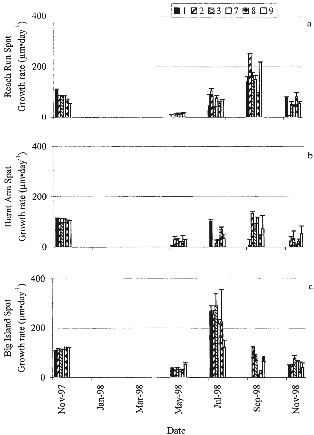
Figure 11.2. Average growth rate ( \mu\text{m}\cdot\text{d}^{-1} ) per station for Reach Run spat (a), Burnt Arm spat (b) and Big Island spat (c), transplanted to Reach Run ( n=100 mussels, error bars= standard error).
