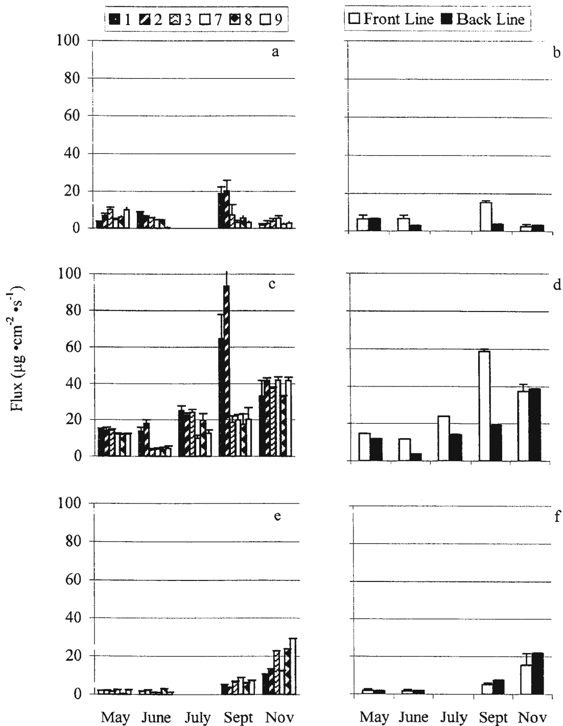
Figure 10. a), c) and e) Flux ( \mu\text{g} \cdot \text{cm}^{-2} \cdot \text{s}^{-1} ) at 3.5 m, stations 1-3 and 7-9 calculated using data from dissolution cylinders and chlorophyll- a concentrations in a) Burnt Arm, c) Reach Run and e) Big Island, (n= 5, error bars= standard error). Experimental long line averages at 3.5 m (b, d, f), in b) Burnt Arm, d) Reach Run and f) Big Island (n= 15, error bars= standard error).
