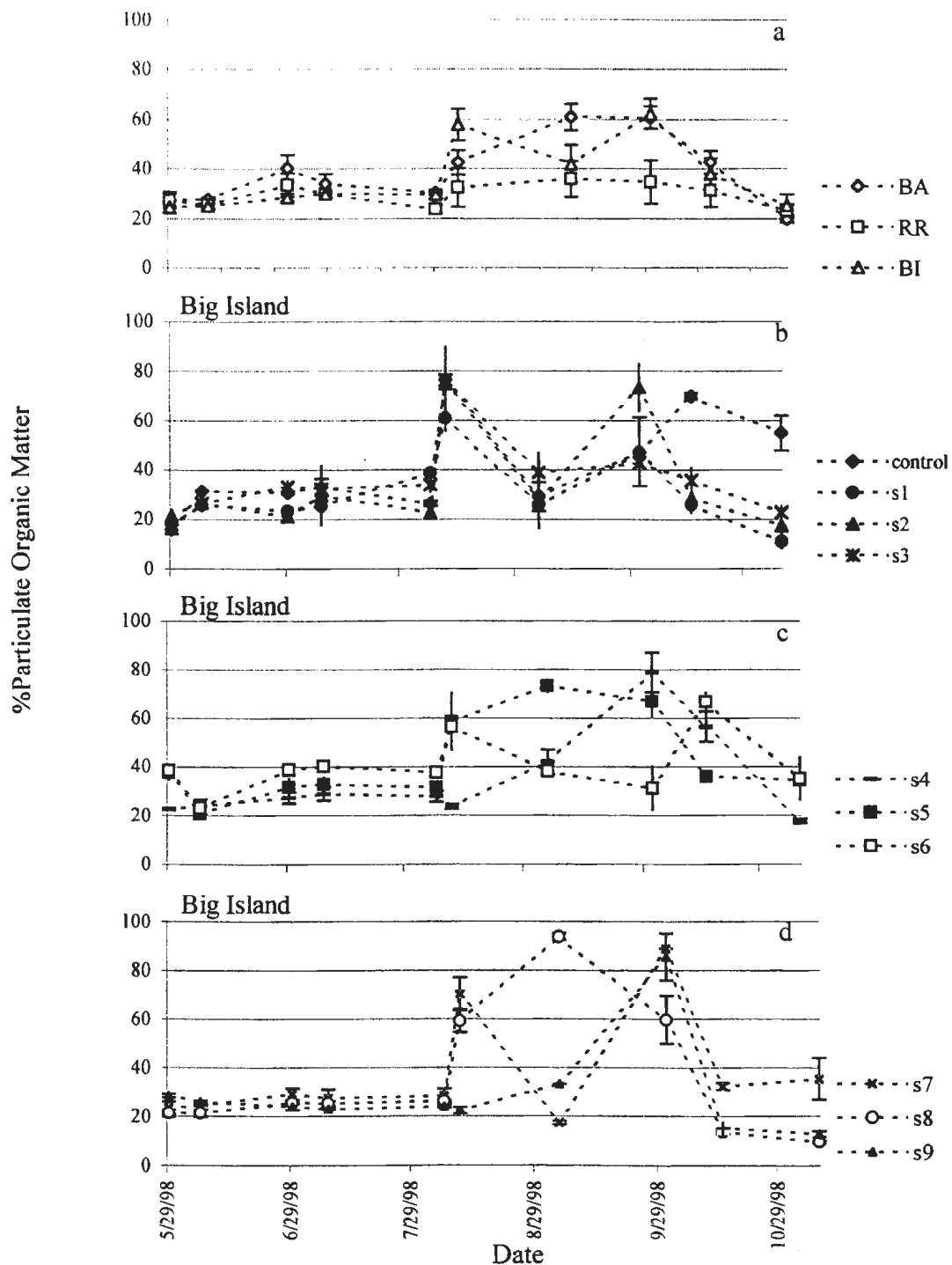
Figure 7.3. a) Percent POM averaged over all stations at Burnt Arm (BA), Reach Run (RR) and Big Island (BI) at 3.5 m, %POM in Big Island at station b) control, 1, 2 and 3 c) 4, 5 and 6 and d) 7, 8 and 9, respectively (error bars= standard error).
