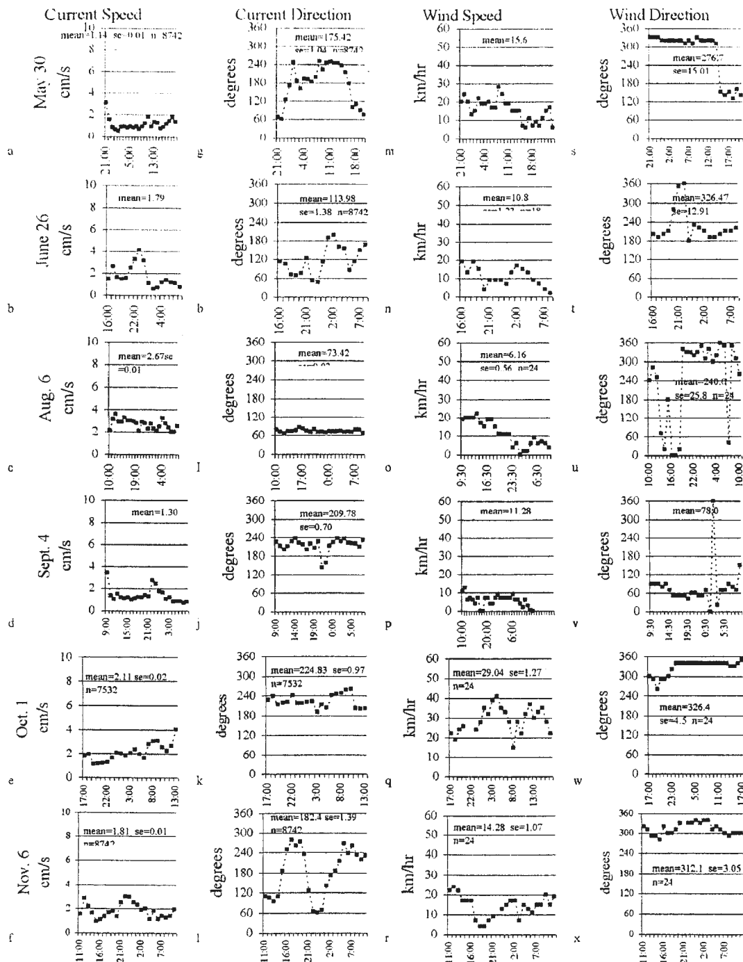
Appendix 5.3: Hourly current speed a)-f) and current direction g)-l) measured with an S4 current meter near Big Island, Notre Dame Bay, NL (station 2) on May 30, June 26, Aug. 6, Sept. 4, Oct. 1 and Nov. 6th, respectively; Hourly wind speed m)-r) and direction s)-x) collected in the Twillingate, NL on the above dates (source Environment Canada, Twillingate, NL, n= 3 per point).
