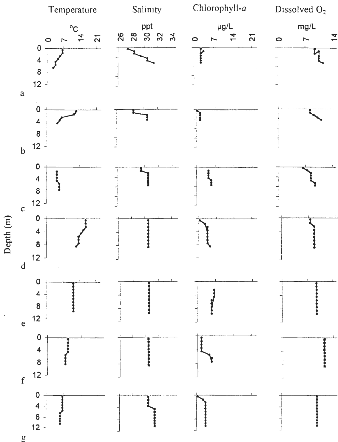
Figure 6.1. Vertical depth profiles of environmental data averaged from all 10 static at Burnt Arm on a) May 21, b) June 23, c) July 04, d) August 10, e) September 13, f) October 17 and g) November 30, 1998.
