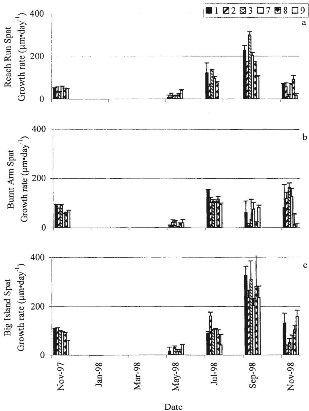
Figure 11.1. Average growth rate ( \mu\text{m}\cdot\text{d}^{-1} ) per station for Reach Run spat (a), Burnt Arm spat (b) and Big Island spat (c), transplanted to Burnt Arm ( n=100 mussels, error bars= standard error).
