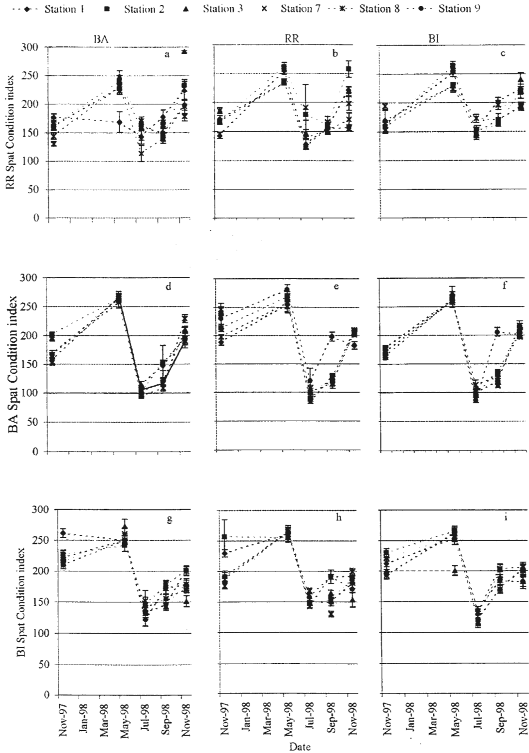
Figure 15. Condition indices of Reach Run mussels (a-c), Burnt Arm mussels (d-f), Big Island mussels (g-i) transplanted to Burnt Arm (column 1), Reach Run (column 2) and Big Island (column 3), respectively (error bars= standard error, n=30).
