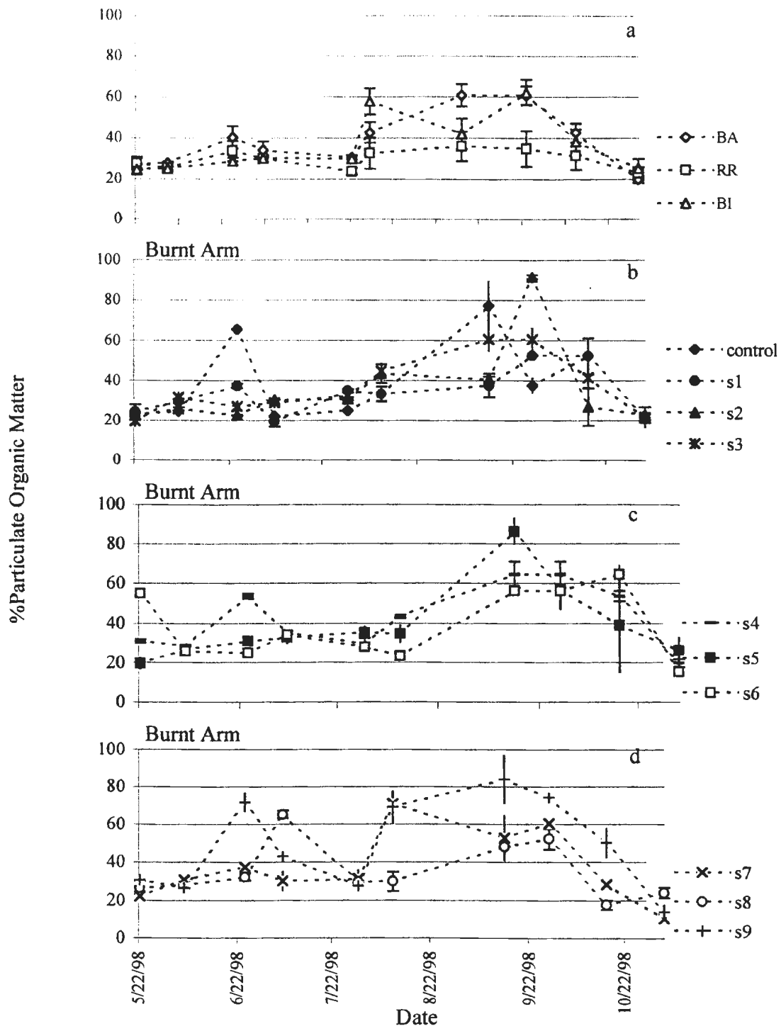
Figure 7.1. a) Percent POM averaged over all stations at Burnt Arm (BA), Reach Run (RR) and Big Island (BI) at 3.5 m, %POM in Burnt Arm at station b) control, 1, 2 and 3 c) 4, 5 and 6 and d) 7, 8 and 9, respectively (error bars= standard error).
