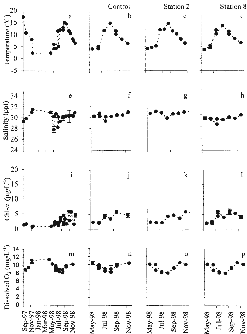
Figure 5.1. Seasonal environmental data collected at Burnt Arm, Sept. 1997 – Nov. 1998 at 3.5 m. Column 1 represents data collected in this study as well as another NAIA sponsored study, column 2 represents data from this study collected at the control station located at the outside each farm, column 3 represents data collected at station 2, positioned at the front of each farm, column 4 represents data collected at station 8 positioned at the back of each farm. Each row represents temperature, salinity, chlorophyll- a and dissolved oxygen, respectively ( n = 3-5 per point, error bars = standard error).
