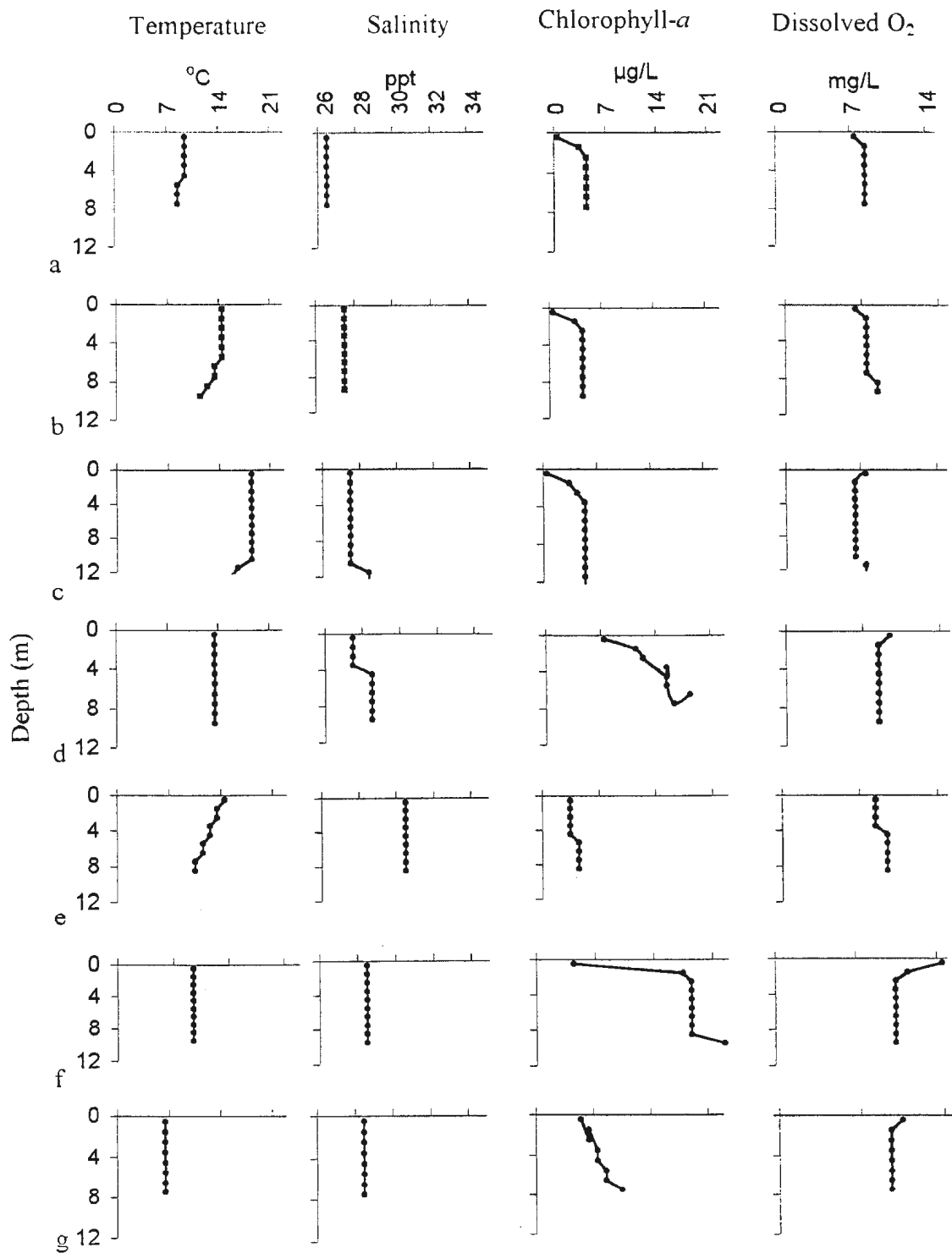
Figure 6.2. Vertical depth profiles of environmental data averaged from all 10 static at Reach Run on a) May 25, b) June 25, c) July 06, d) August 8, e) September 08, f) October 16 and g) November 05, 1998.
