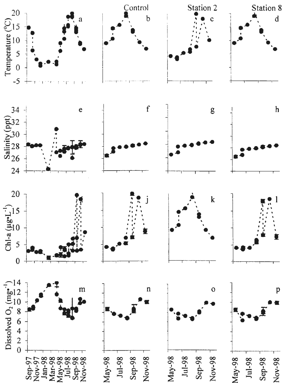
Figure 5.2. Seasonal environmental data collected at Reach Run, Sept. 1997 – Nov. 1998 at 3.5 m. Column 1 represents data collected in this study as well as another NAIA sponsored study, column 2 represents data from this study collected at the control station located at the outside each farm, column 3 represents data collected at station 2, positioned at the front of each farm, column 4 represents data collected at station 8 positioned at the back of each farm. Each row represents temperature, salinity, chlorophyll- a and dissolved oxygen, respectively ( n = 3-5 per point, error bars = standard error).
