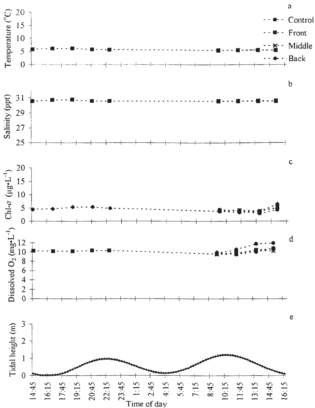
Appendix 4.18: Short-term environmental (tidal) data collected at Big Island, Nov. 7-8, 1998; measured at the control station and three lines in the front, middle and back of the farm at 3.5 m depth with a CTD, a) temperature, b) salinity, c) chlorophyll-a, d) dissolved oxygen e) tidal height at time of sampling.
