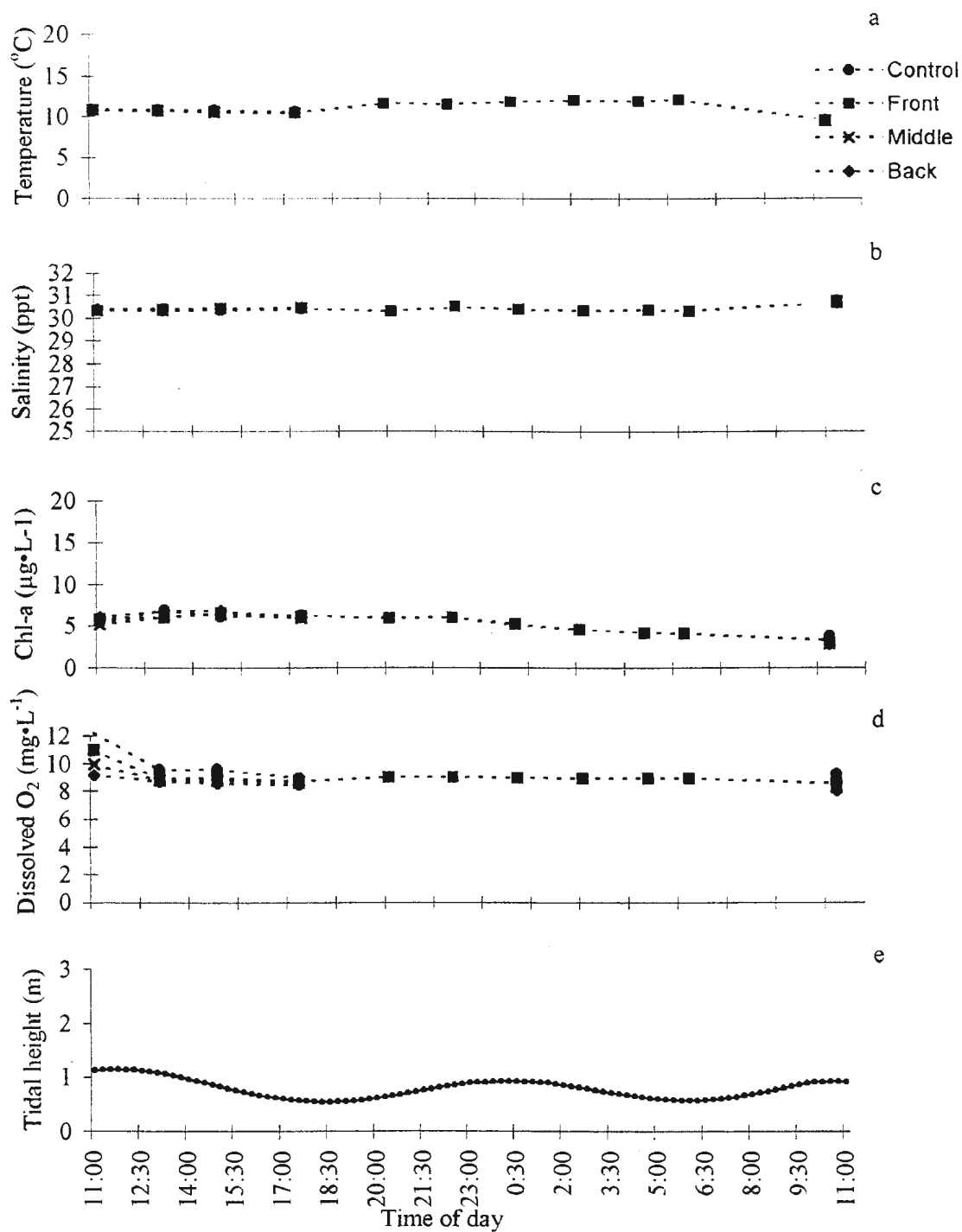
Appendix 4.5: Short-term environmental (tidal) data collected at Burnt Arm, Sept. 28-29, 1998; measured at the control station and three lines in the front, middle and back of the farm at 3.5 m depth with a CTD, a) temperature, b) salinity, c) chlorophyll-a, d) dissolved oxygen e) tidal height at time of sampling.
