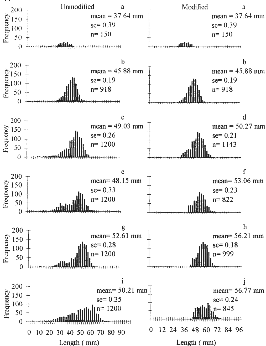
Appendix 2.4: Shell length frequency distributions of Burnt Arm spat transplanted in Reach Run measured a) Sept. 1997, b) Nov. 1997, c) May 1998, d) May 1998 modified, e) July 1998, f) July 1998 modified, g) Sept. 1998, h) Sept. 1998 modified i) Nov. 1998, j) Nov. 1998 modified (se= standard error, n= number of mussels, modified= data from secondary set removed).
