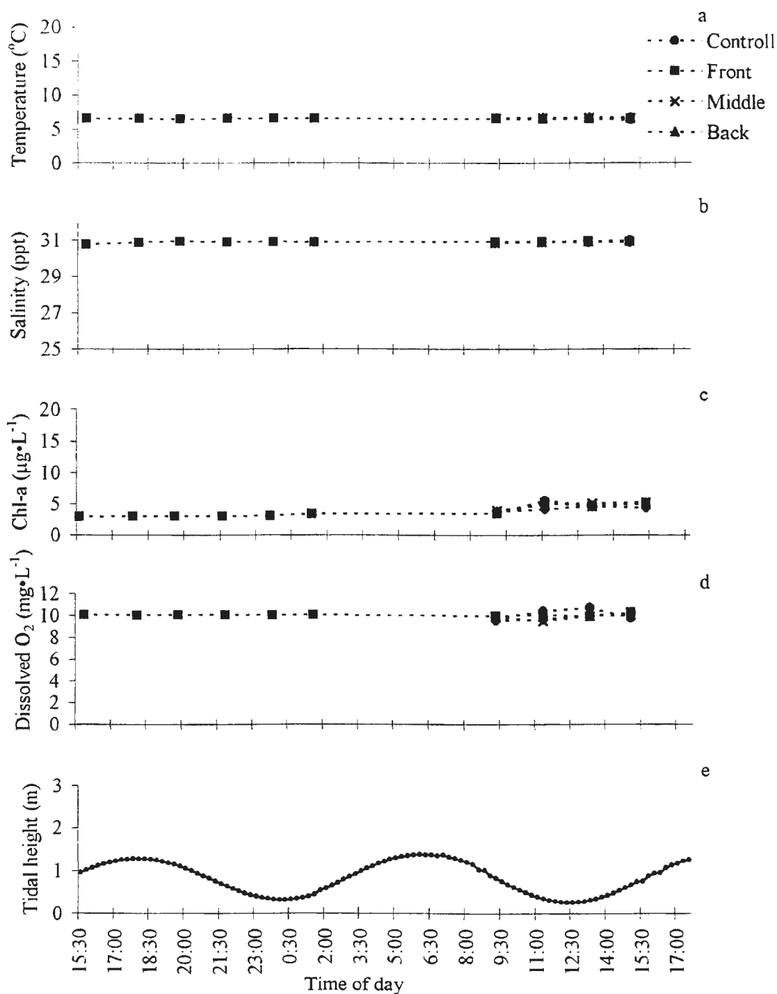
Appendix 4.6: Short-term environmental (tidal) data collected at Burnt Arm, Nov. 2-3, 1998; measured at the control station and three lines in the front, middle and back of the farm at 3.5 m depth with a CTD, a) temperature, b) salinity, c) chlorophyll-a, d) dissolved oxygen e) tidal height at time of sampling.
