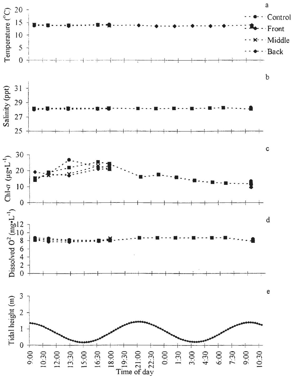
Appendix 4.10: Short-term environmental (tidal) data collected at Reach Run, Sept. 8-9, 1998; measured at the control station and three lines in the front, middle and back of the farm at 3.5 m depth with a CTD, a) temperature, b) salinity, c) chlorophyll-a, d) dissolved oxygen e) tidal height at time of sampling.
