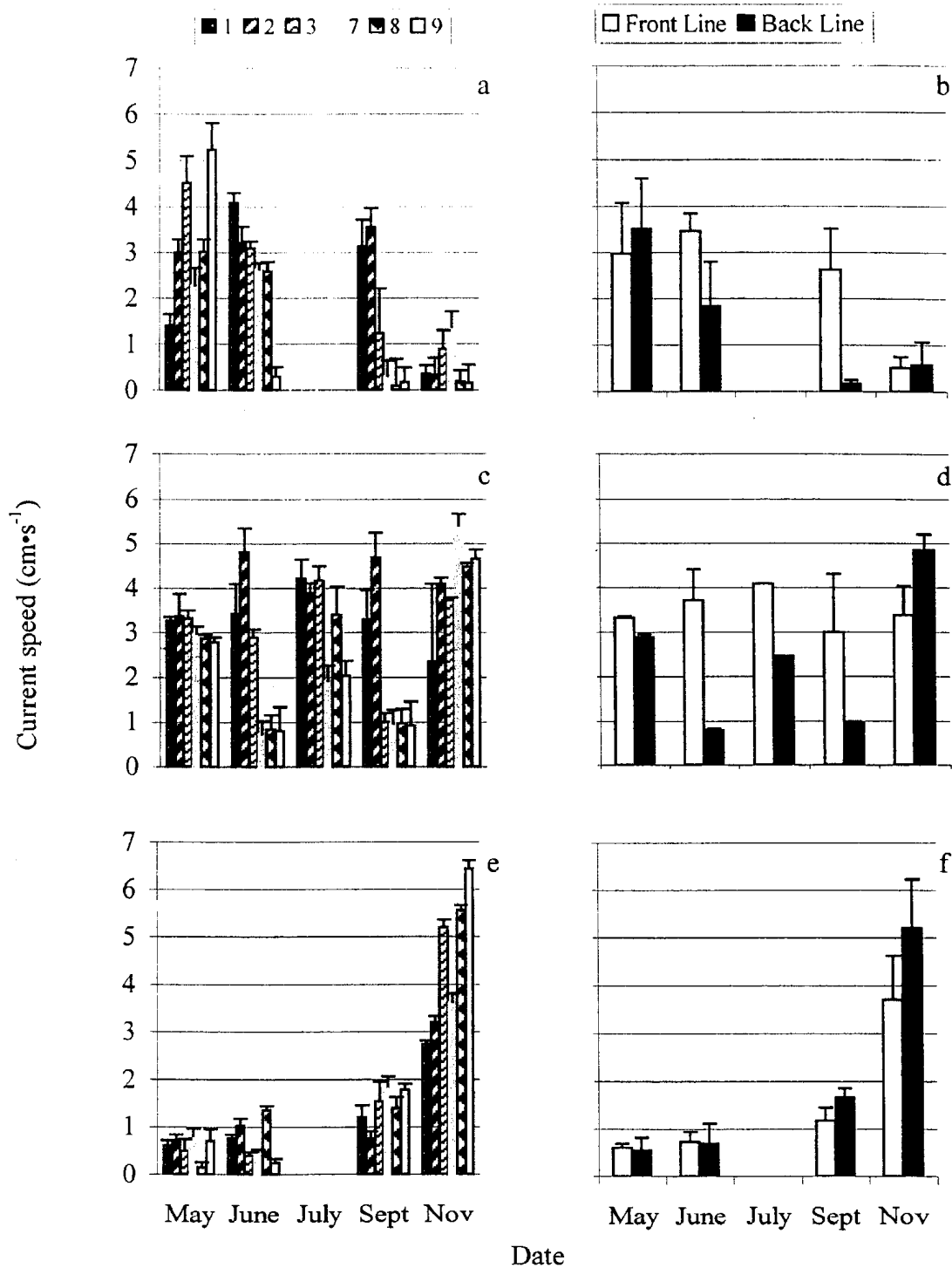
Figure 9. Relative current speed ( \text{cm} \cdot \text{s}^{-1} ) at 3.5 m (a, c, e) stations 1-3 and 7-9 measured with dissolution cylinders in a) Burnt Arm, c) Reach Run and e) Big Island, ( n=5 , error bars = standard error). Experimental long line averages at 3.5 m (b, d, f), in b) Burnt Arm, d) Reach Run and f) Big Island ( n=15 , error bars = standard error).
