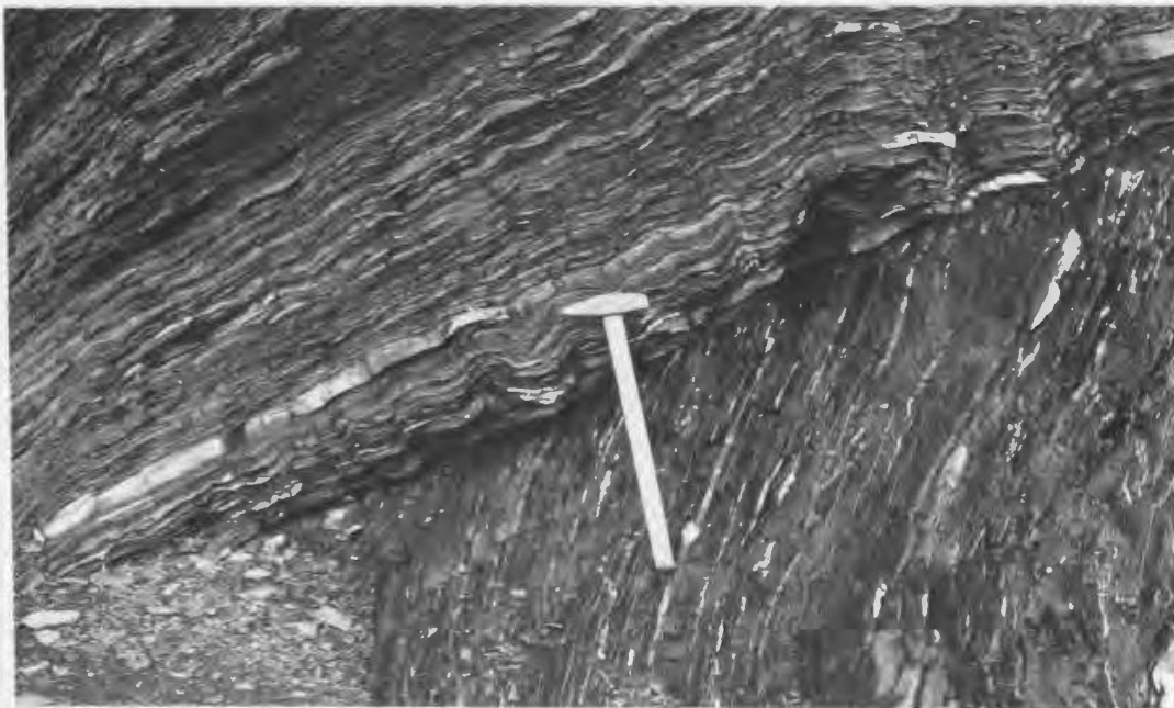
Fig.35. Small thrust, probably resulting from the faulting of a box shaped fold(fig.34.). Locality and horizon as in fig.34.
