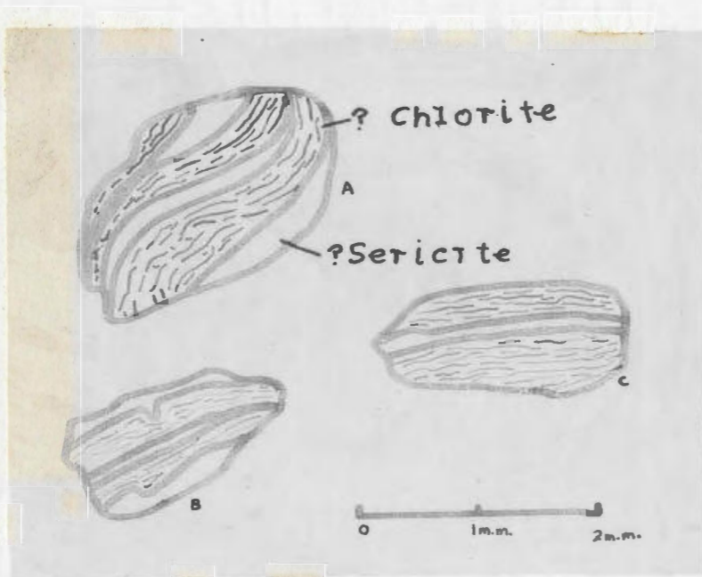
Fig.3. ?Chlorite-?Sericite intergrowths.
