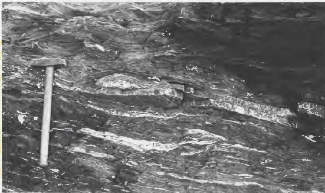
Fig.14. Bedding plane thrust repeating a thin dolomitic siltstone of the Middle Arm Point formation and folded shales near the head of the hammer. About 1 mile north of Middle Arm Point.
