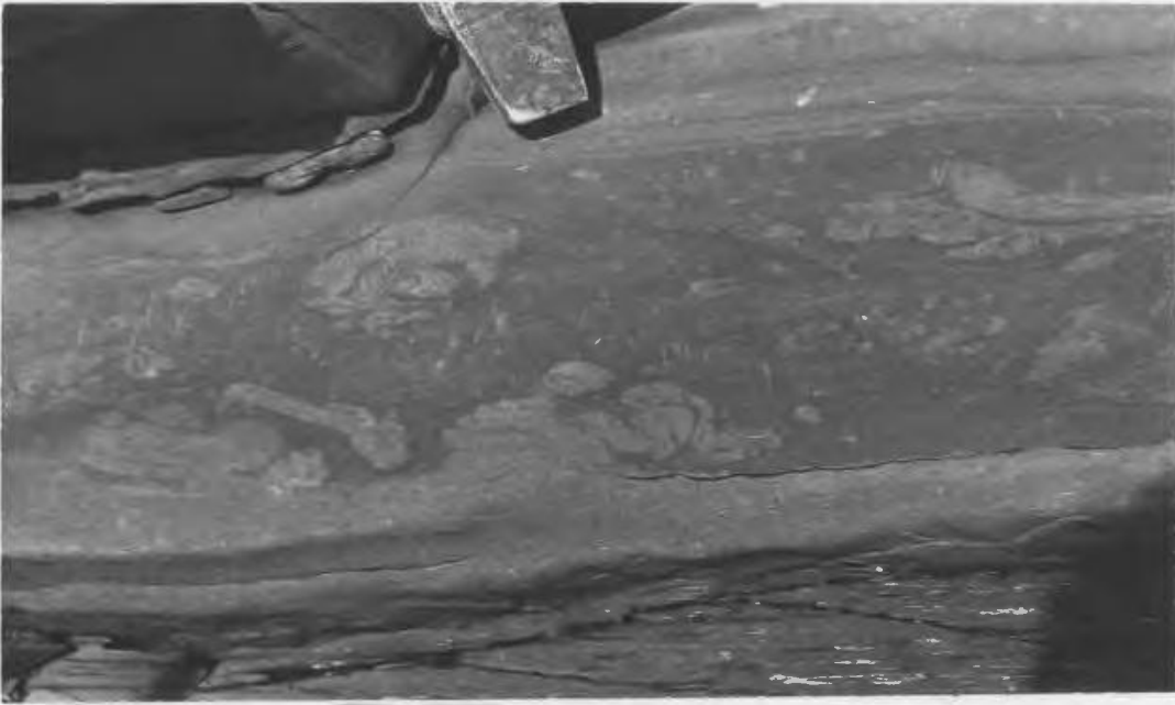
Fig.21. Ripple marks on the top surface of a dolomitic siltstone bed of the J.1. sequence just north of Lower Beach.
