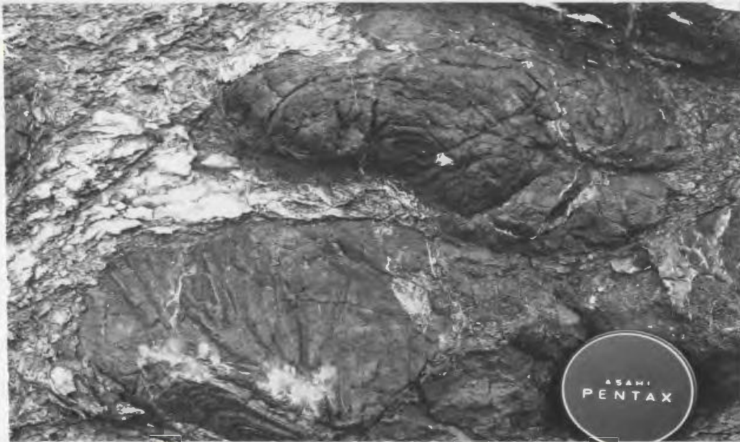
Fig.18. Pillowed volcanic flow with a calcite matrix from the volcanic horizon of the Woods Island formation just west of Tiheay Cove, Woods Island.
