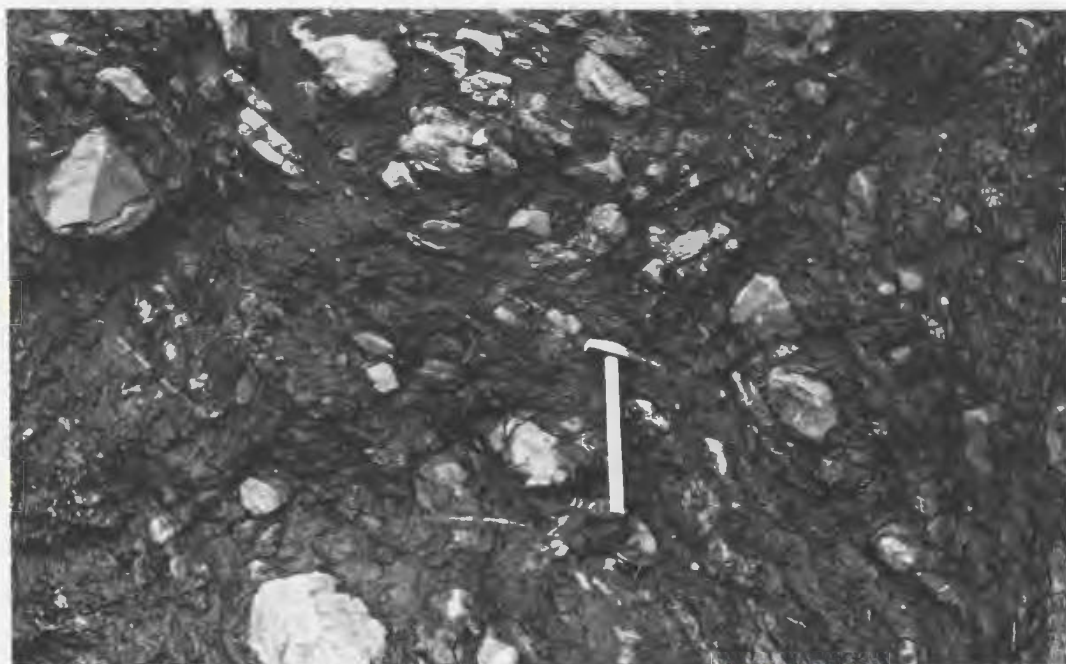
Fig.46. Chaotic deformation at Trenchman's Head. Most of the blocks are limestone and a crude stratification dipping towards the bottom right of the photograph can be detected.
