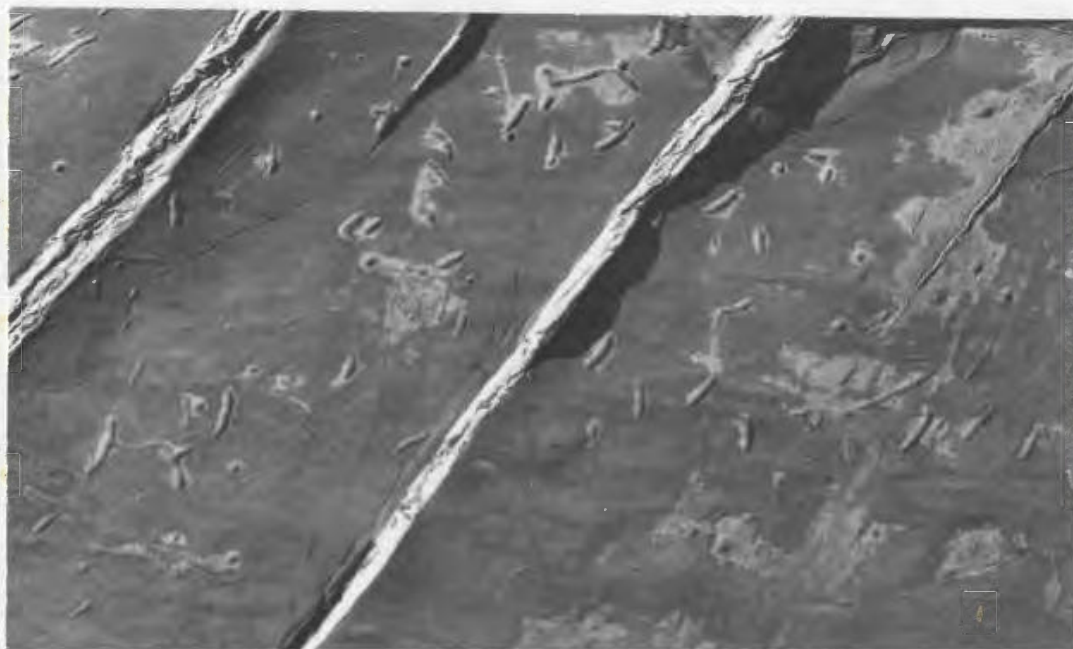
Fig.29. Simple trace fossils on the bottom of a dolomitic siltstone horizon. South-western shore of Eagle Island.
