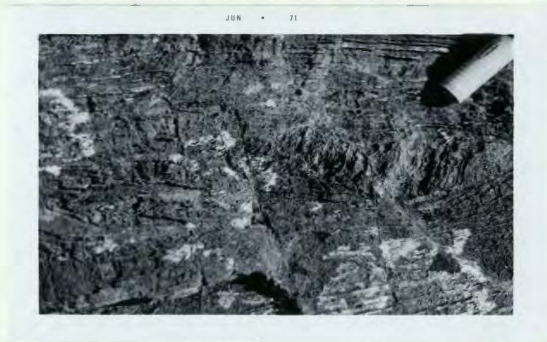
b: Augened ultramafic inclusions, Grassy Gulch. Note folding in inclusion on left.
