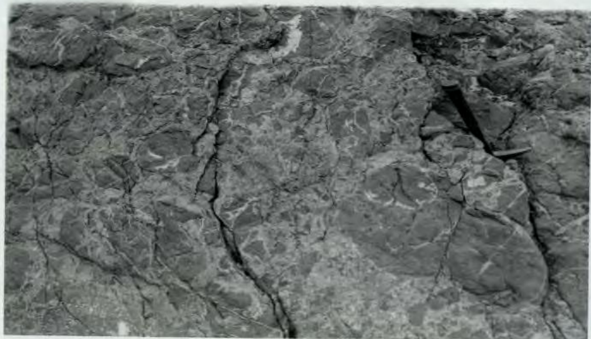
b: Pyroclastics at Bottle Cove. Prehnite and calcite abundant Batheau yielding lighter-color matrix.
