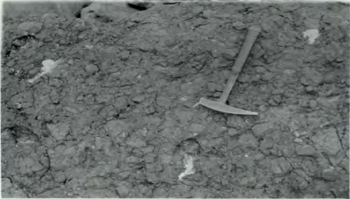
a: Pyroclastics at Bottle Cove Batheau
