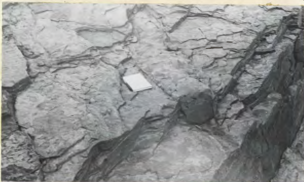
Plate. 3-21 Ribbon-like sandstone body in facies C. Note the sharp contact to the right of the note book. (Outer Cove Member of the St. John's Formation, Outer Cove).
