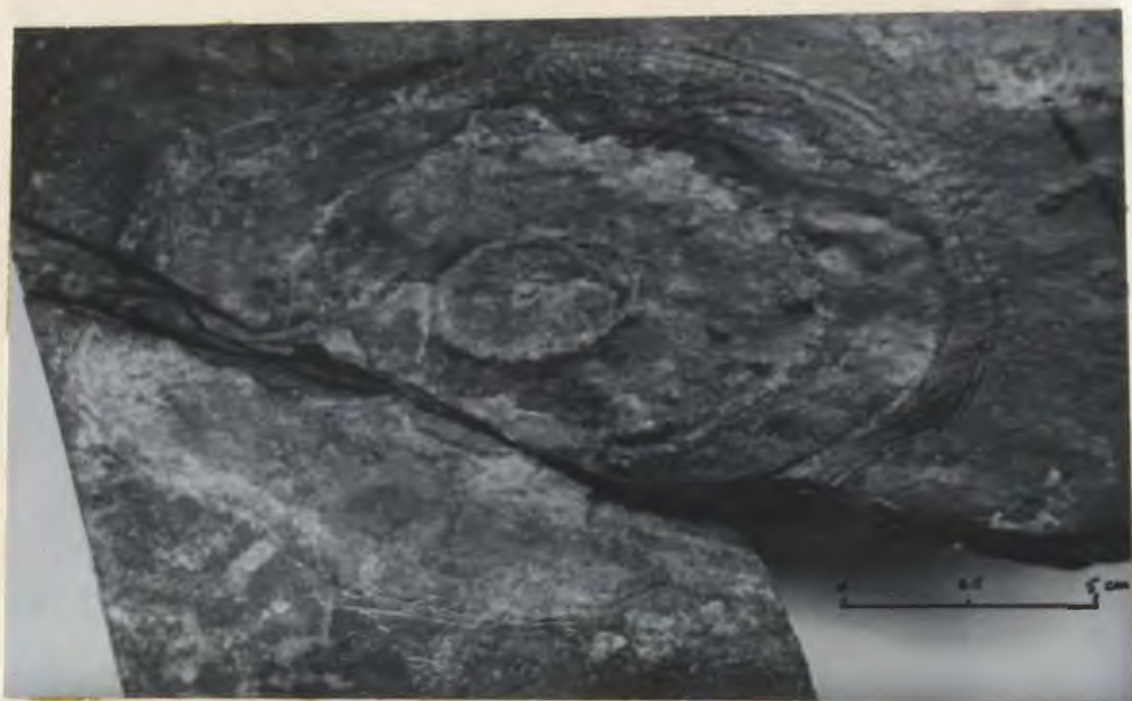
Plate. 4-8- The largest Type 5 marking showing concentric rings. Top surface of black shale. Outer Cove Member of the St. John's Formation, Ferryland.
