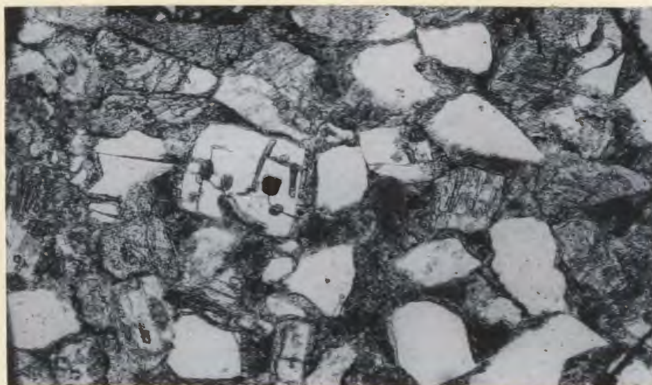
Plate. 3-32- Tuffaceous sandstone in facies A. Note the fractured volcanic quartz (light) and strongly altered plagioclase (turbid). X 40, transmitted light. (Aquaforte Harbour)
