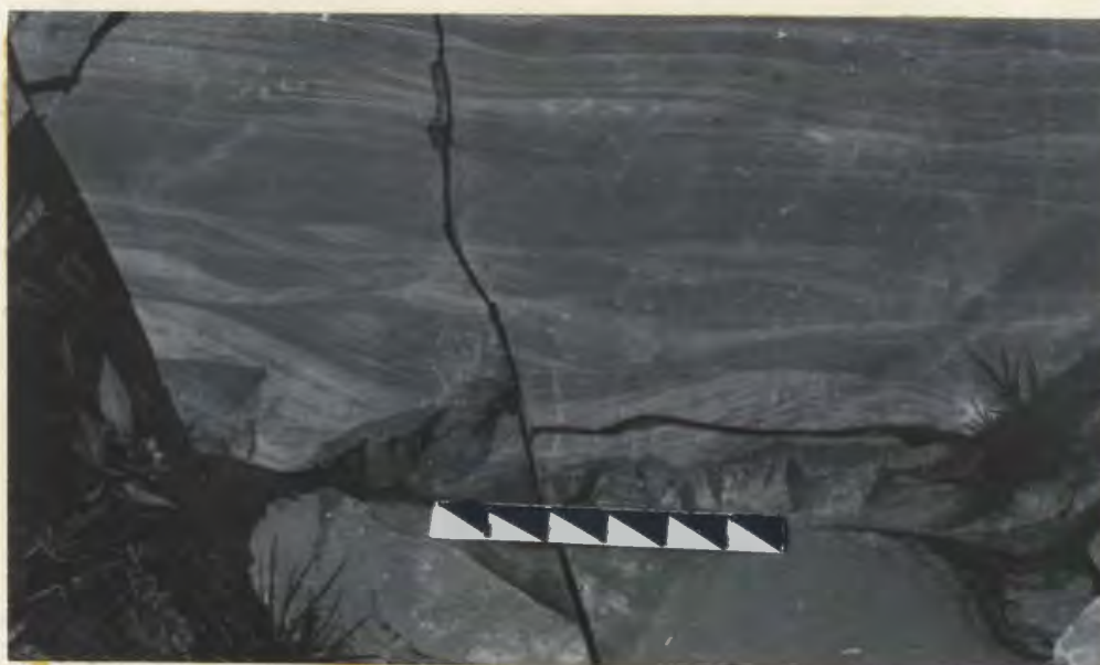
Plate. 3-38 Cosets of ripple-drift cross lamination in the very fine-grained sandstone the Gibbett Hill Formation. Scale in inch. (Calvert Bay).
