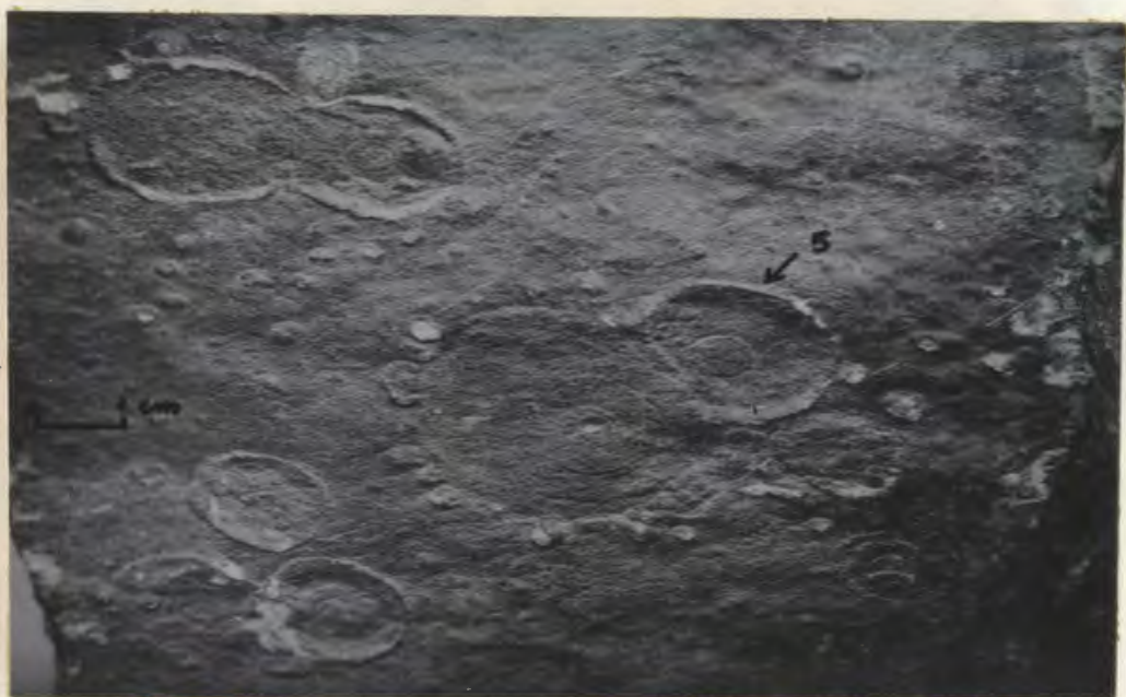
Plate. 4-7- Type 1 and Type 5 markings. Note the overlap of Type 5 markings. Lower surface of the sandstone bed. (Outer Cove Member of the St. John's Formation, Ferryland)
