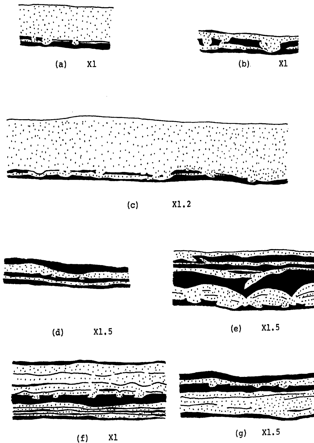
Fig. 4-3. Internal structures of surface markings in the St. John's Formation. Sandstone in stipples, black shale in black.
