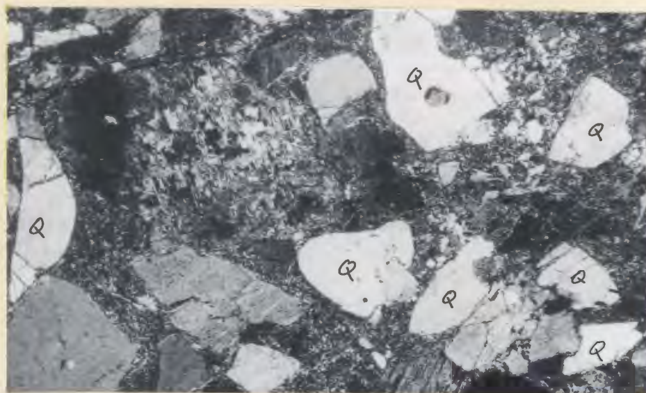
Plate, 3-50- Tuffaceous sandstone showing volcanic quartz (Q) and feldspar. Note the fractured quartz and feldspar. X 40, cross nicols.
