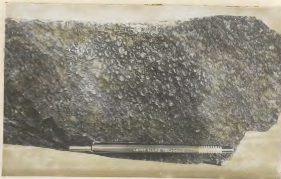
Plate. 4-5- Type 4 markings showing the longitudinal groove and radial line. Note the preferred orientation of the markings. Lower surface of sandstone bed. Outer Cove Member of the St. John's Formation. Ferryland.
