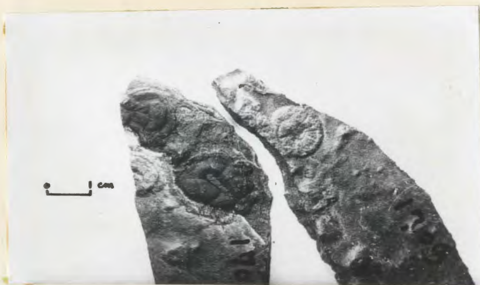
Plate. 4-4- Type 3 markings showing radial lines and concave central pit with marginal ring. Lower surface of sandstone bed. Outer Cove Member of the St. John's Formation, Ferryland.
