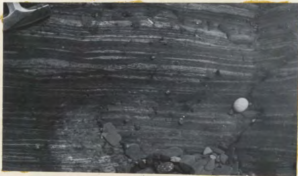
Plate. 3-12 Facies C (interbedded sandstone and shale) of the Outer Cove Member of the St. John's Formation. Note the lenticular sandstone bed just under the hammer. (Ferryland)
