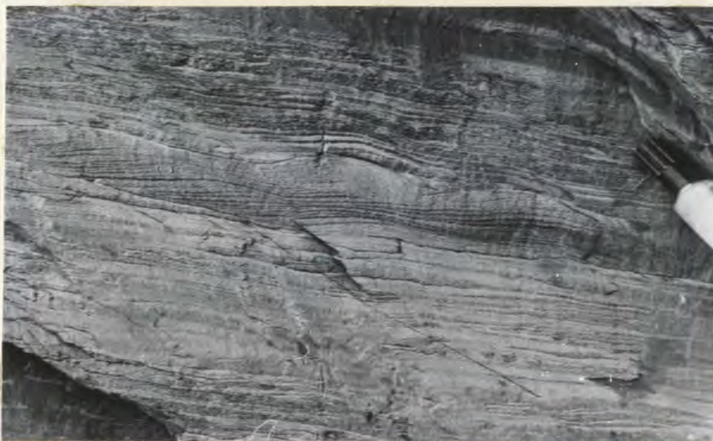
Plate. 3-13 Solitary set of ripple-drift cross laminations in Facies C. Current from north (right) to south (left). (Outer Cove Member of the St. John's Formation, Ferryland).
