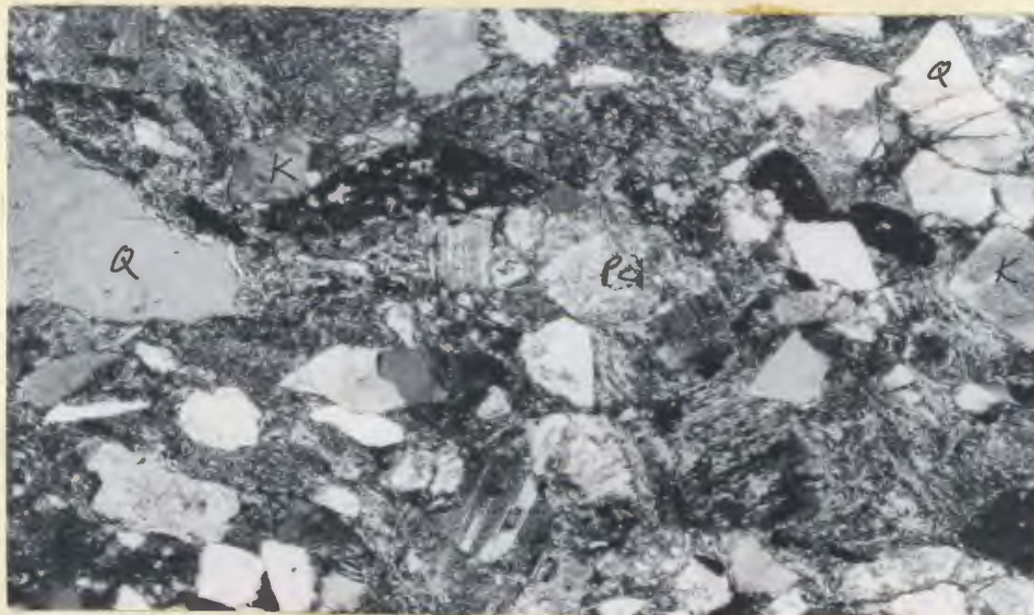
Plate. 3-29- Tuffaceous sandstone in facies C, showing volcanic quartz (Q), K-feldspar (K), and sodic plagioclase (Pc). (Outer Cove Member of the St. John's Formation, Ferryland) X 40, transmitted light.
