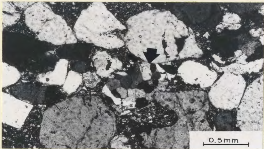
FIGURE 44. Detrital metaquartzite fragment. (X nicols) Sample BI-65a, Ochre Cove Formation.
