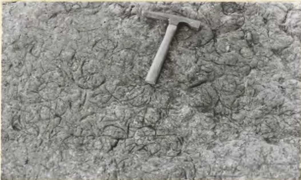
FIGURE 29a. "Scribbling" grazing traces; Freshwater Cove, Bell Island. Hammer is 28 cm long.
