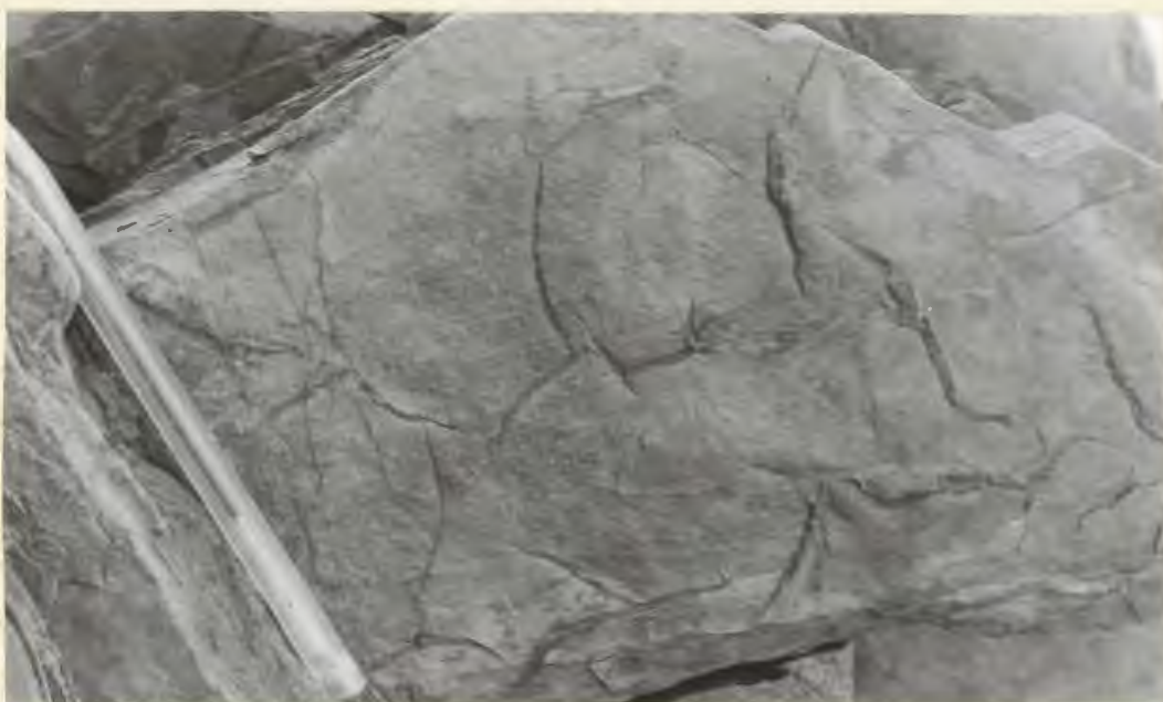
FIGURE 22. Mudcracks; between the ore docks, Bell Island. Pen is 13 cm long.
