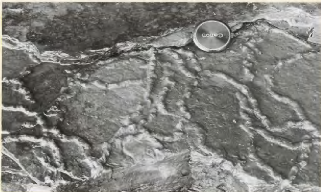
FIGURE 29b. Ichnofossil of unknown affinity, possibly a grazing trace; top of bed at Freshwater cove, Bell Island.
