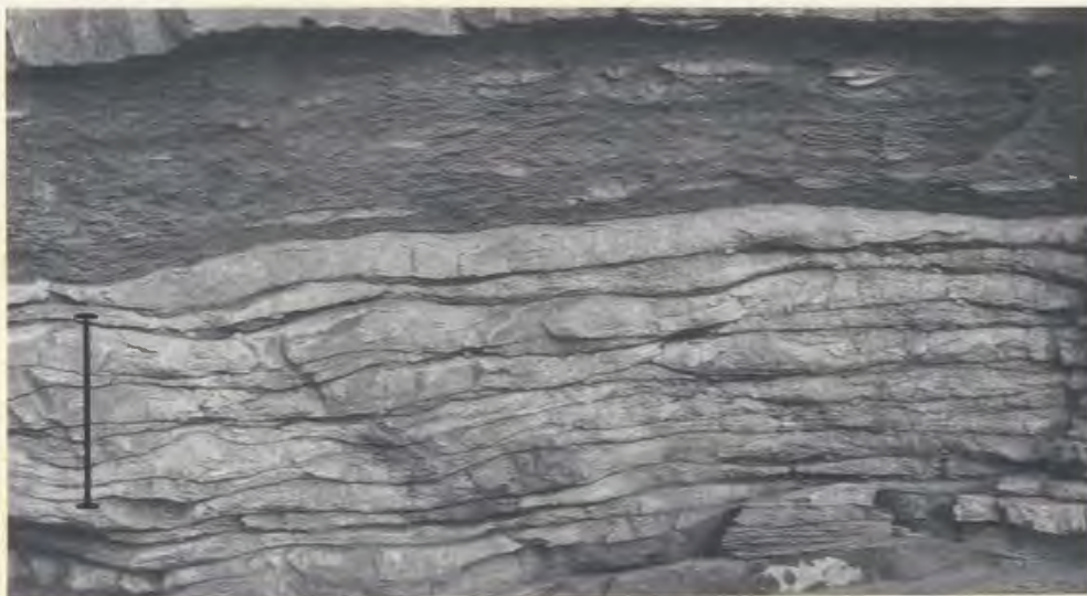
FIGURE 12. Mud-draped flaser-bedded sandstone overlain by starved ripples; The Beach, Bell Island. Bar represents 10 cm.
