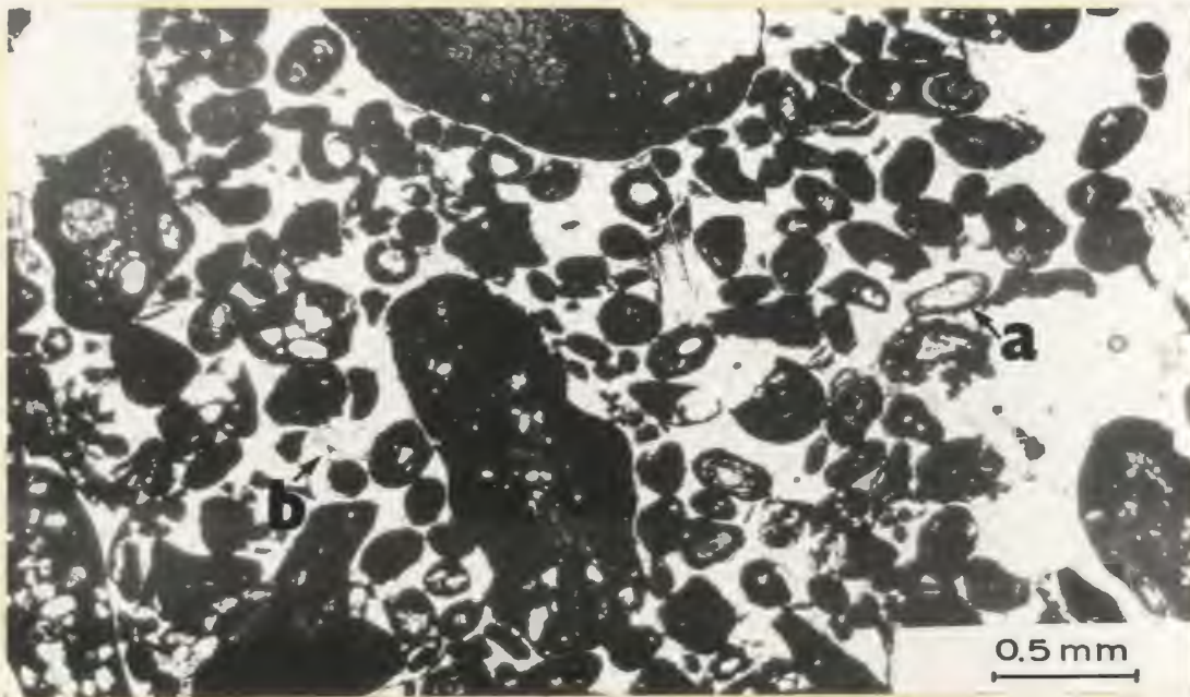
FIGURE 48. Pyrite Member. (a) Pyritized oolite with chamosite core; (b) unpyritized chamosite oolite. Sample BI-74, Powers Steps Formation.
