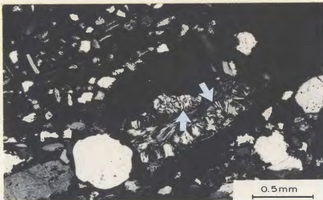
FIGURE 41. Spherulitic rhyolite fragment. Note radial structure (arrows). (X nicols) Sample N243h.
