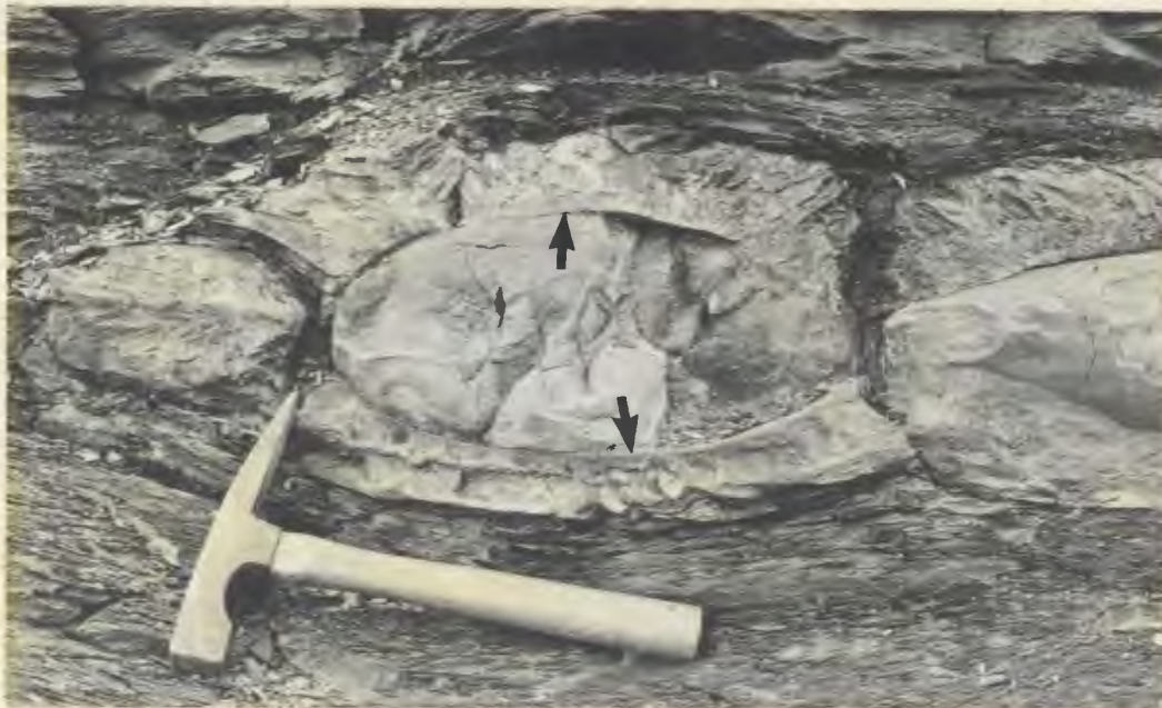
FIGURE 4b. Septarian nodules surrounded by cone-in-cone structure (arrows). Hammer is 28 cm long.
