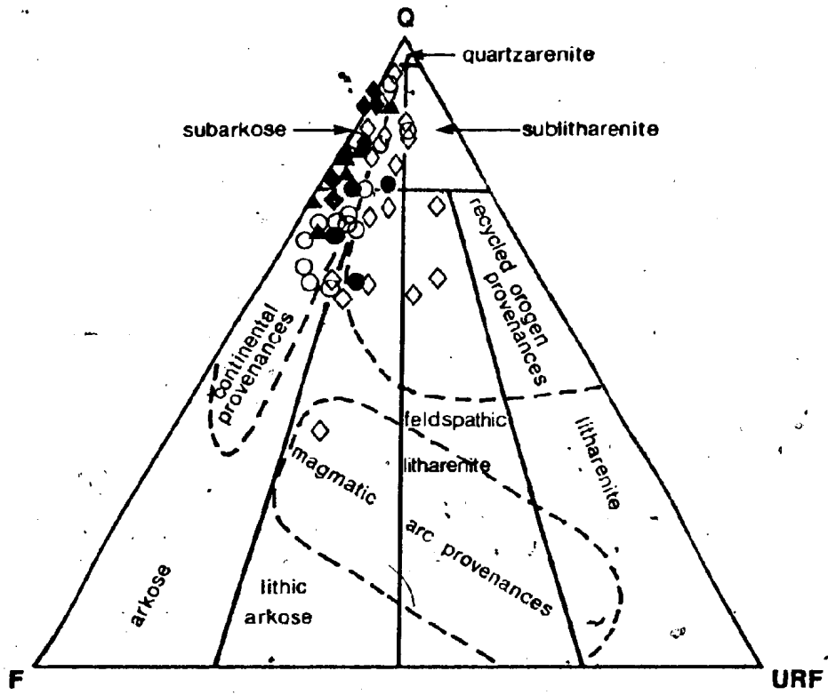
after Folk (1968) and Dickinson & Suczek (1979) Sandstone Compositions
