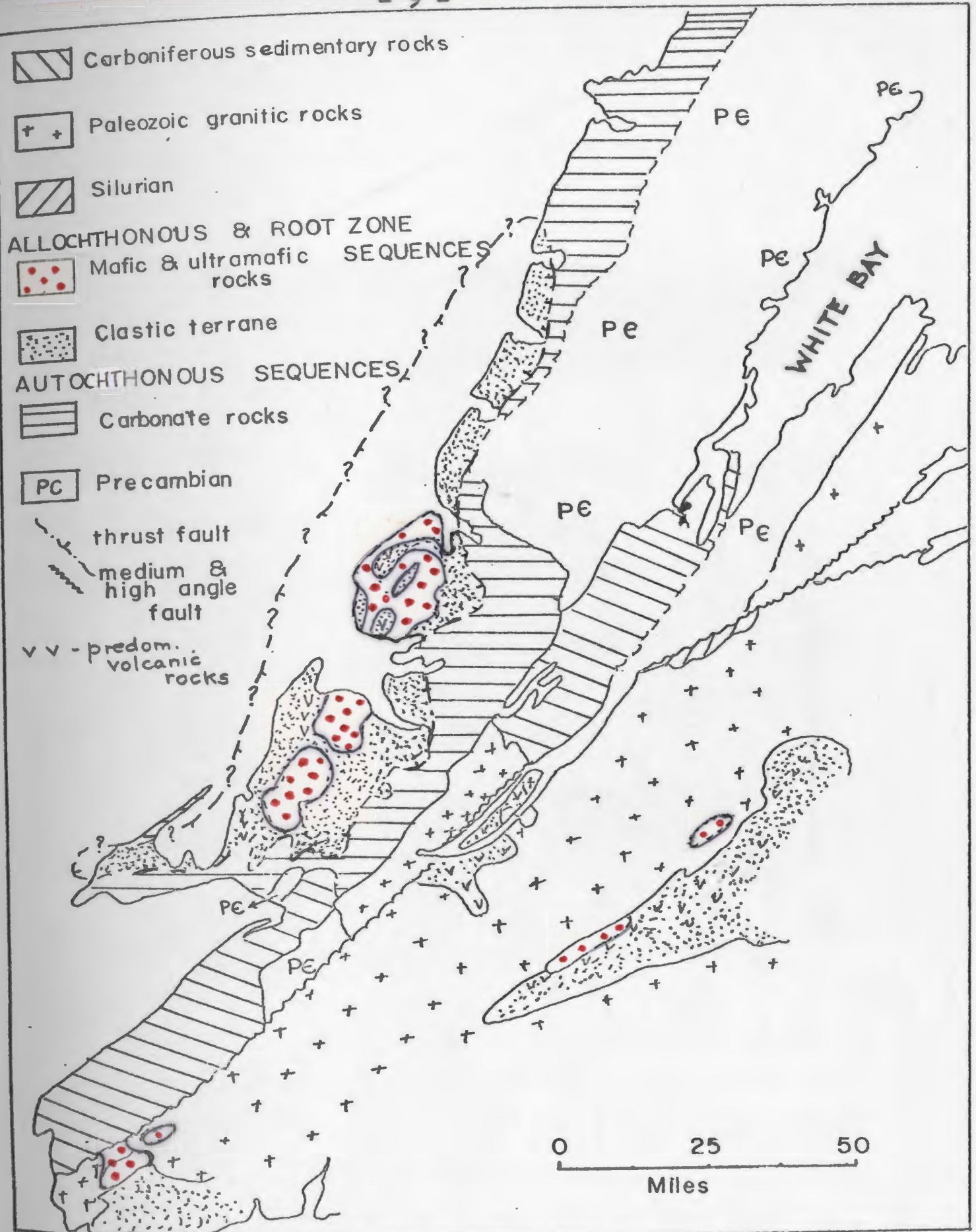
Fig. 4 Generalised Geology of Western Newfoundland, showing proposed Klippen (after Rodgers and Neale, 1963)
