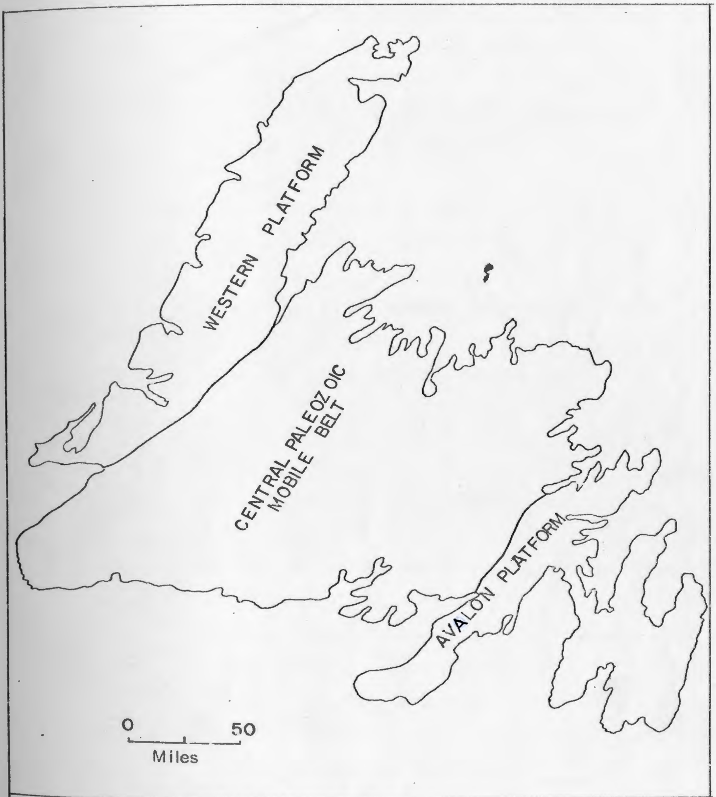
Fig.3 Major Geologic Provinces of Newfoundland Appalachians ( after Williams, 1969)
