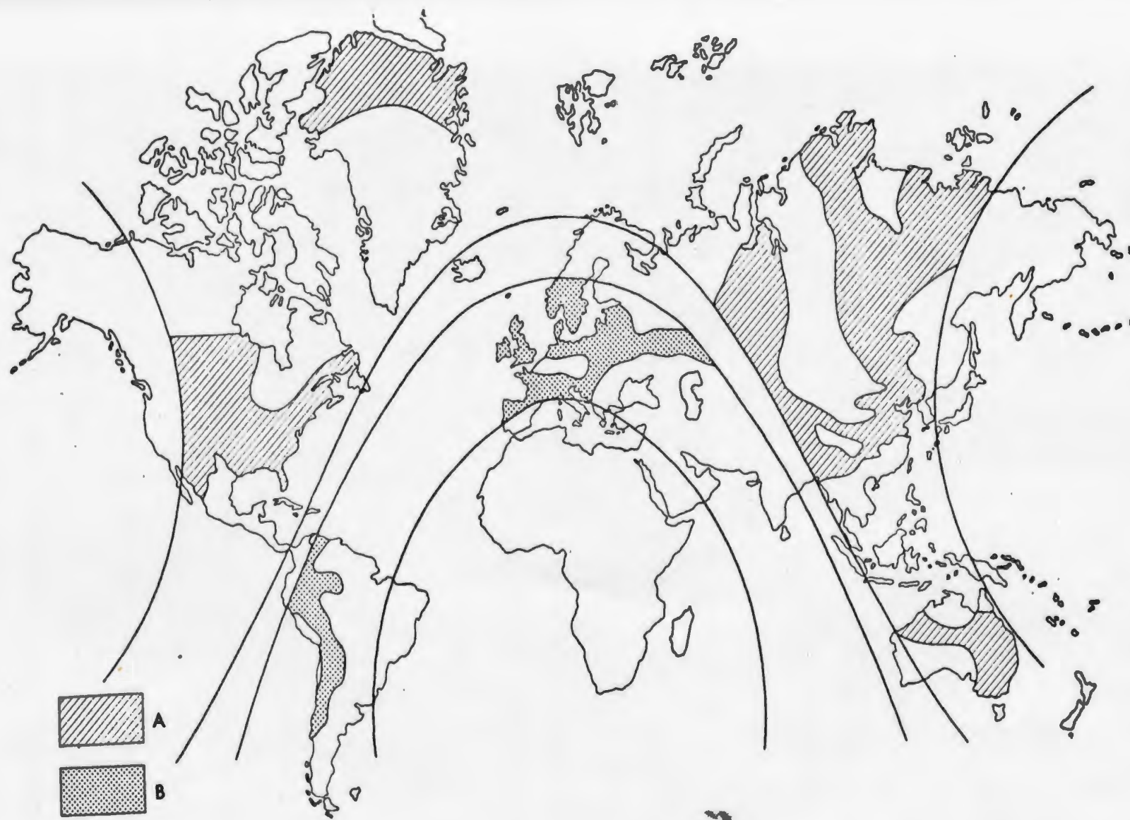
PLATE 36 Broad pattern of distribution of Ordovician faunas : A, northern hemisphere assemblage; B, southern hemisphere assemblage ( From Fell, 1968)
