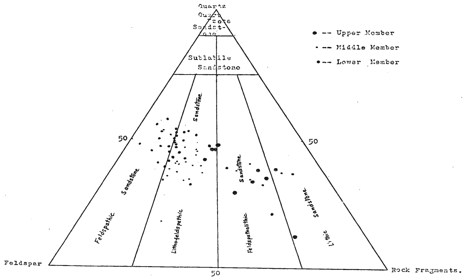
Fig.3-21 Detail composition of sandstones from the Signal Hill Formation.
