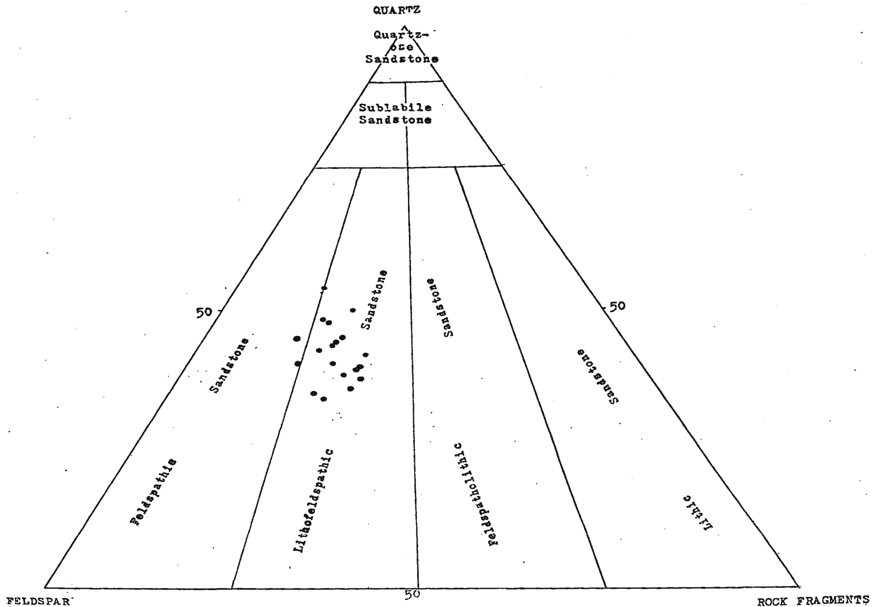
Fig.4-9. - Detail composition of sandstones from the Blackhead Formation.
