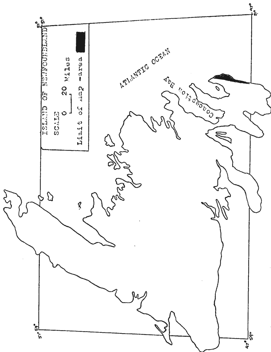
Figure 1-1. Index map showing location of map-area.
