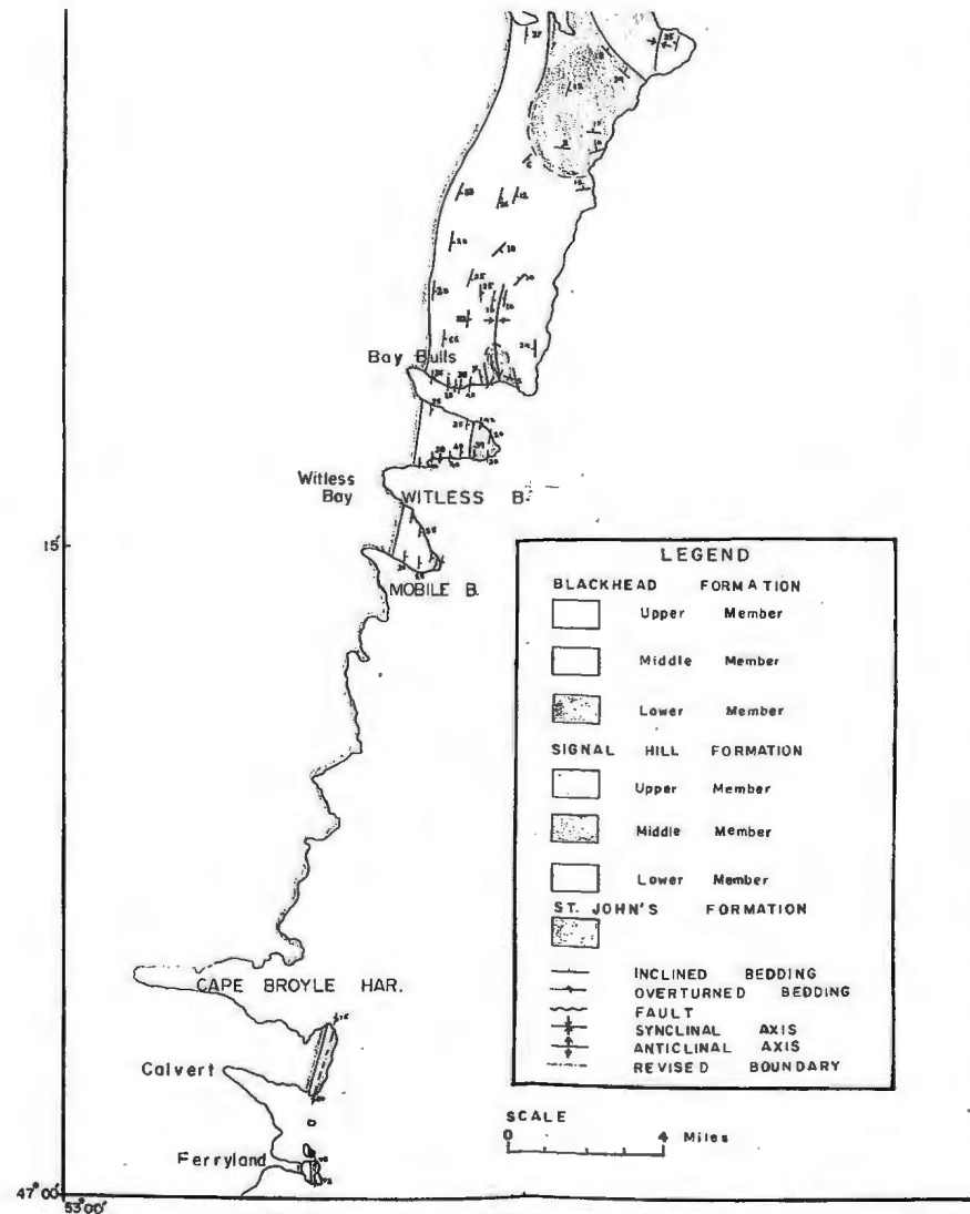
FIGURE 2-1 GEOLOGICAL MAP OF THESIS AREA A (Based on Rose 1952)
