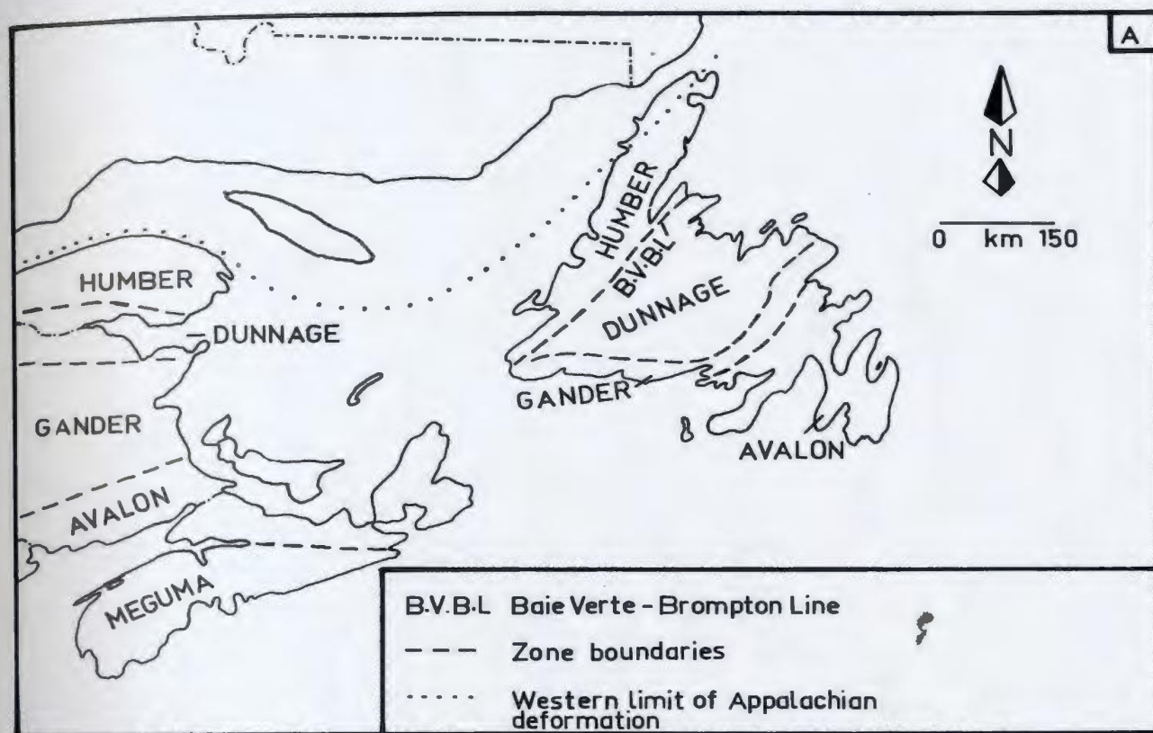
Figure 2.1 (A) The distribution of tectono-stratigraphic zones in the northern Appalachians.
