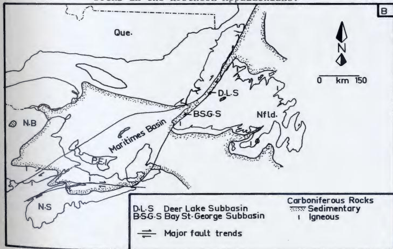
(B) Extent of the Upper Paleozoic Maritimes Basin and the distribution of Carboniferous sediments and igneous rocks in the northern Appalachians.
