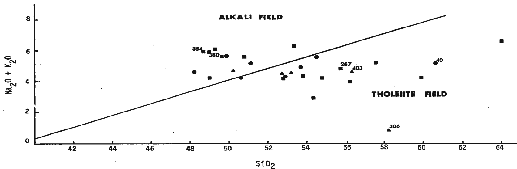
Figure 5.11. (after MacDonald and Katsura, 1964). Total alkalis vs. \text{SiO}_2
