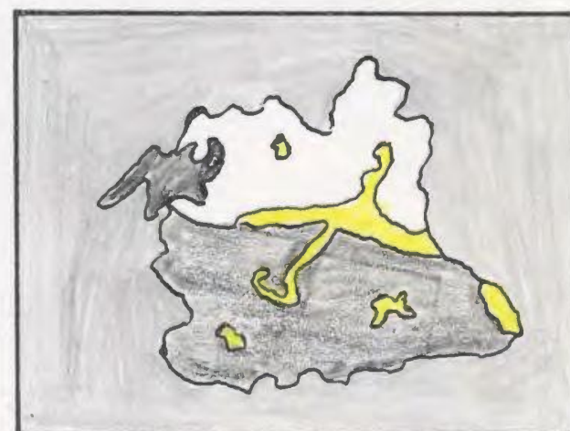
Figure 6.5 (x20) Shows relationship between pyrite (white), chalcopyrite (yellow) and sphalerite (black). Gangue (grey).
