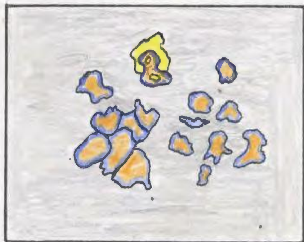
Figure 6.4 (x10) Pyrrhotite (orange) being altered to marcasite (blue) along margins and fractures. Chalcopyrite (yellow). Gangue (grey).
