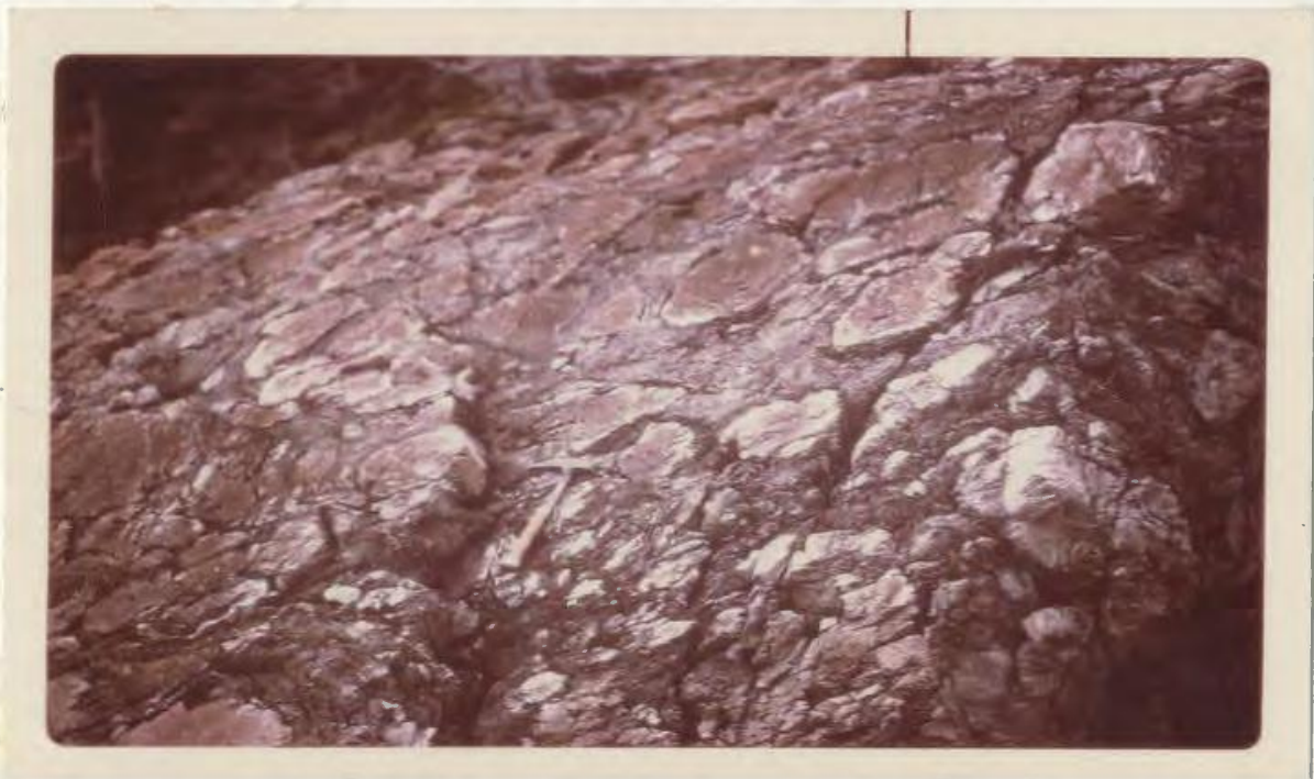
Plate 2. Pillow-Breccia developed in the LOWER BASALT Member. Northern end of Stag Island.
