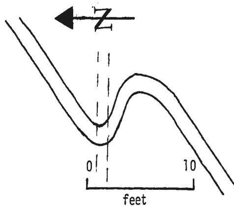
Figure 4.1. Fold noted near Red Point, west coast of Long Island.
