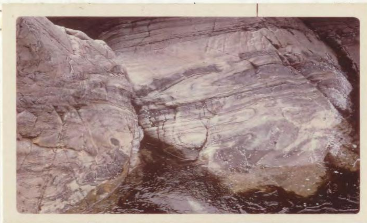
Plate 11. Slump folded tuffs of the PYROCLASTIC Member. This particular horizon occurs intercalated between andesite pillow lavas, Shagg Cliff, Wild Bight.
