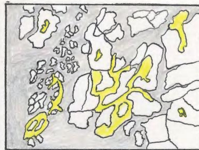
Figure 6.3 (x10) Anhedra, subhedra and massive pyrite (white). Crushed pyrite zone on the left. Chalcopyrite (yellow). Gangue (grey).
