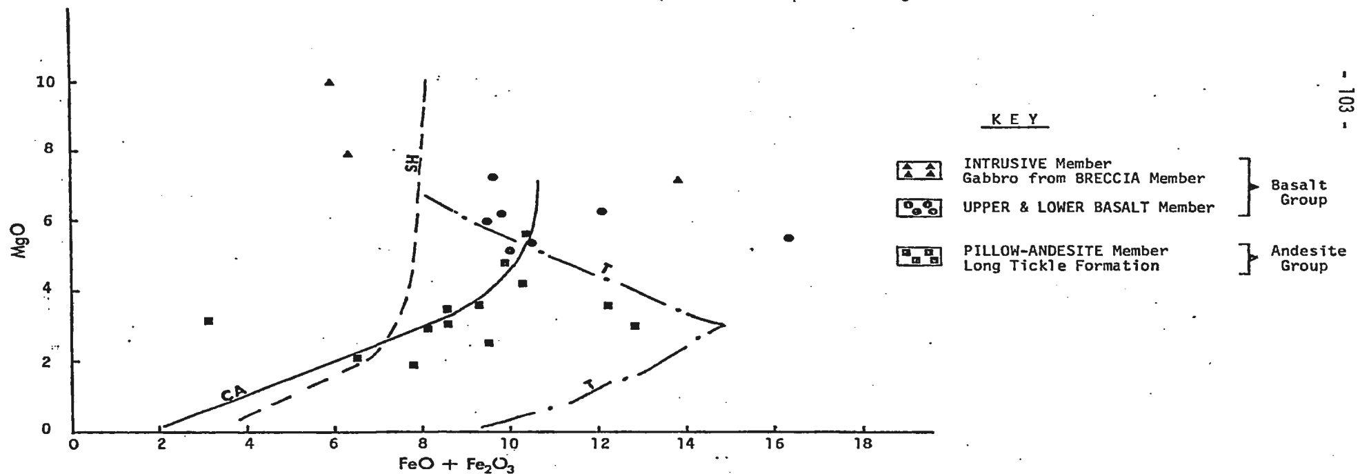
Figure 5.8. (after Willmott, 1972). Total Fe vs. MgO. CA = calc-alkaline association; SH = Shoshonite association, T = tholeiitic association. Note that the ANDESITE GROUP plots along the Ca-trend; whereas the BASALT GROUP has a scatter roughly paralleling the T-trend.
