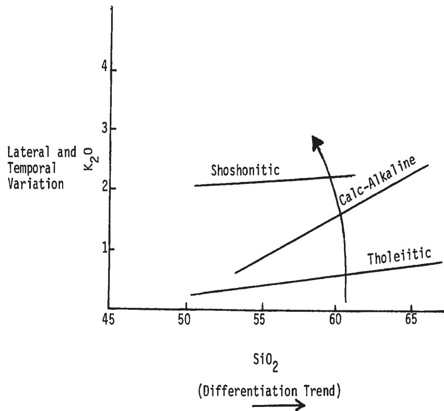
Figure 1.3. Lateral and Temporal Variation in the K_2O content of island arc andesitic rocks. 2 (After Jakes & White, 1972.)
