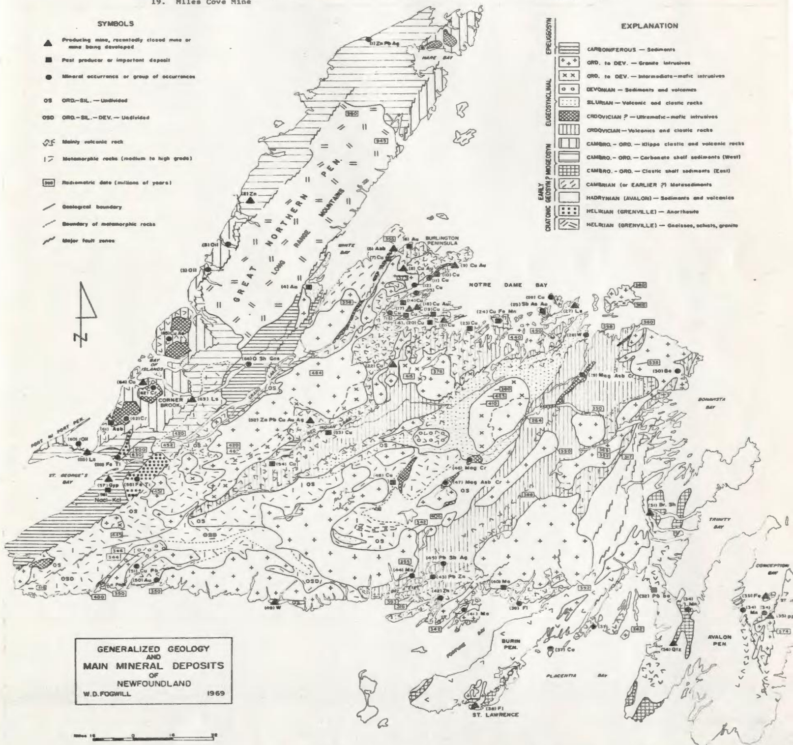
Figure 6.1 (after Fogwill, 1969). Generalized geology and 66 mineral deposits and occurrences of Newfoundland.
