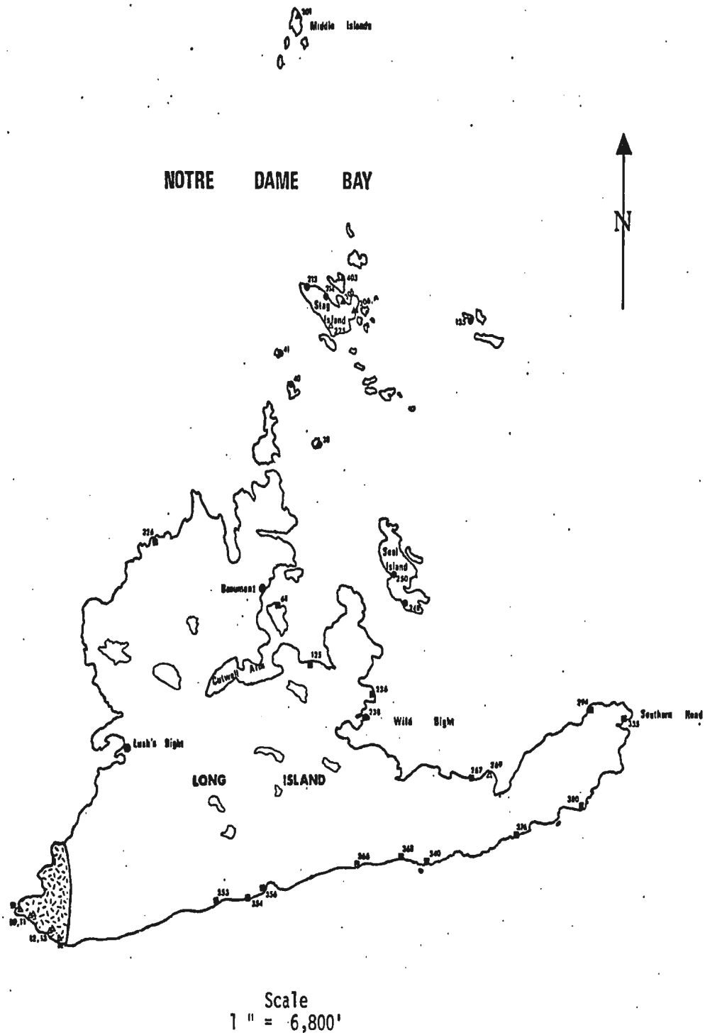
Figure 5.2. Sample location map. Solid symbols represent analyses given in Table 5.2; open symbols represent analyses of intrusive rocks given in Table A-II, Appendix II.
