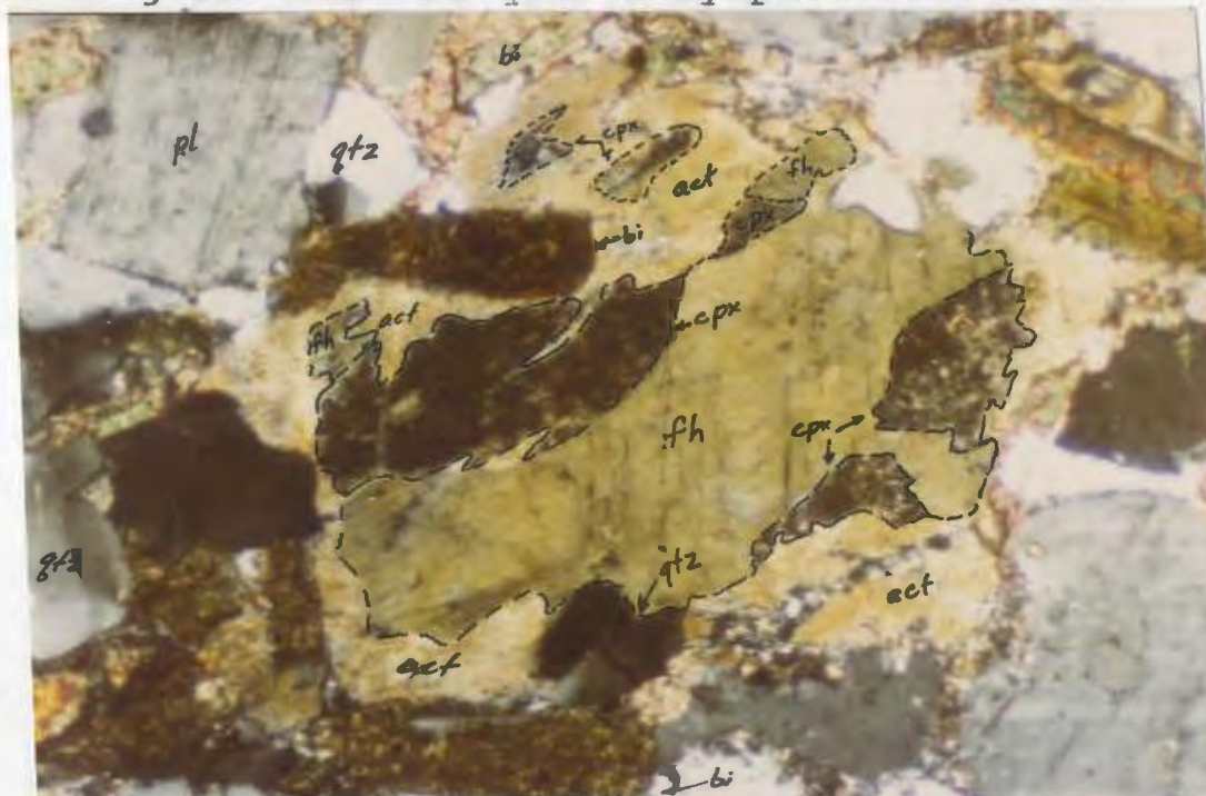
7b. Progressive transformation: ferrohastingsite → clinopyroxene (hedenbigite?) → actinolite in ferrodiiorite. (X 60)
