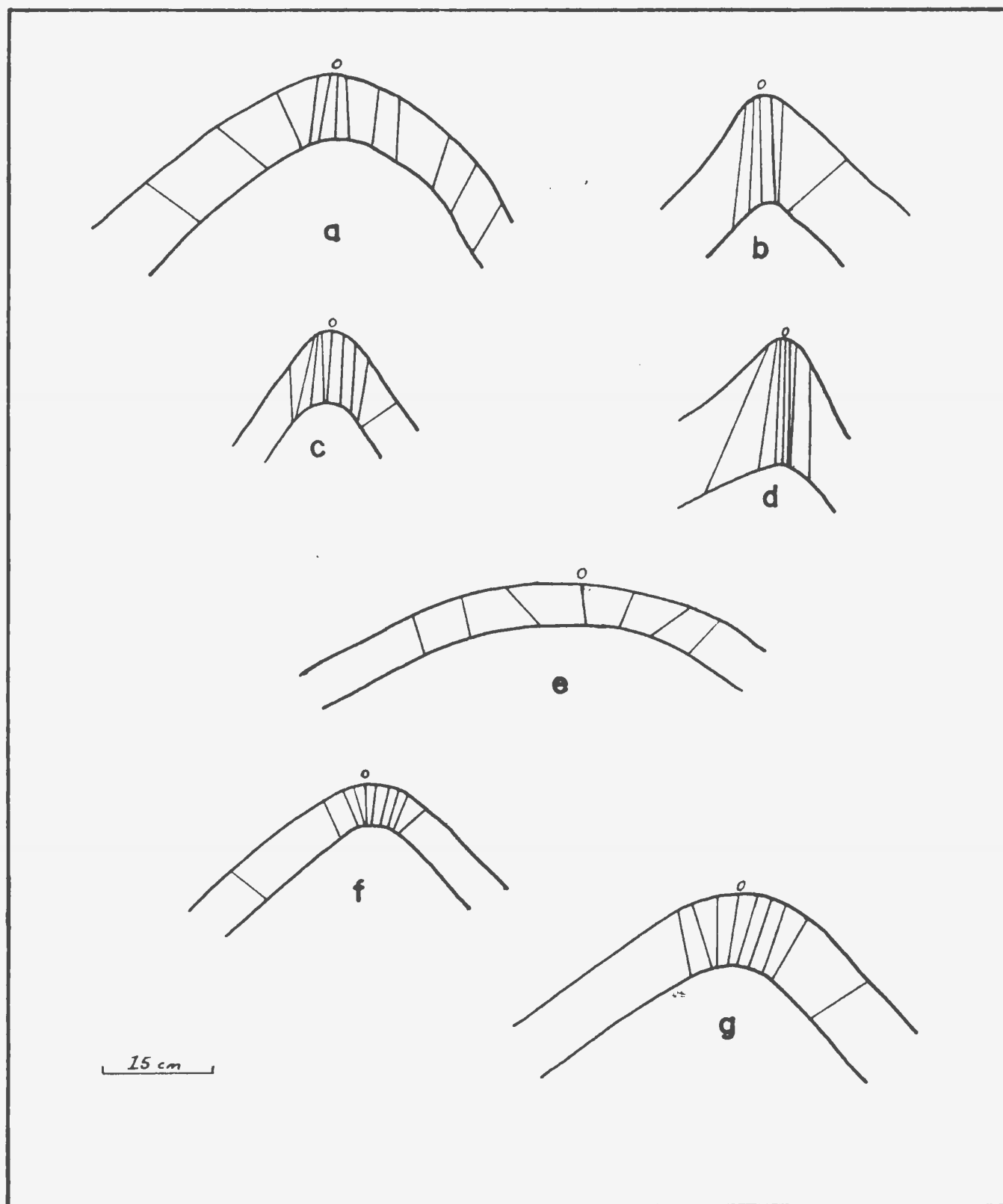
Figure 18. Dip isogons at 10^\circ intervals for approximate profile views of layer folded by F_{1+2} folds. Various localities north and west of Jerusalem Harbour.
