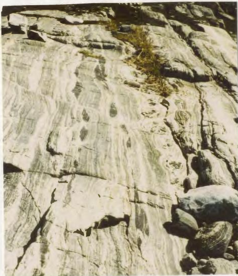
1a. Typical grey, migmatitic Uivak gneisses on south shore of Iterungnek Fiord.
