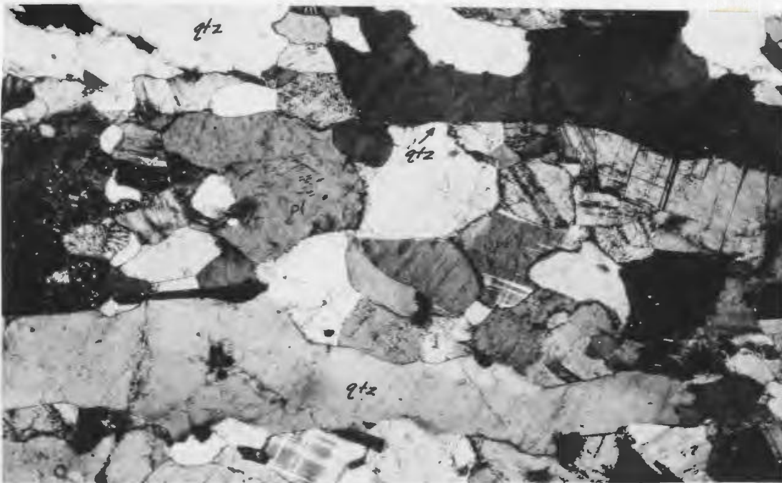
3b. Foliation in section parallel to the mineral streaking lineation, which in this case is defined by elongate quartz. (X 15)
