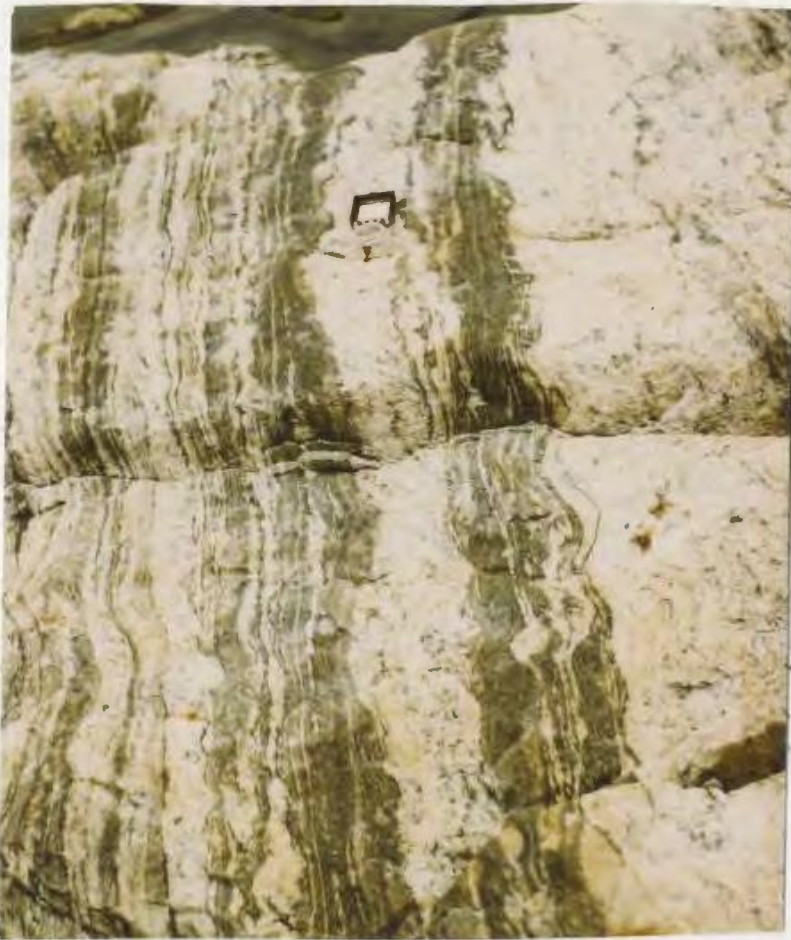
20a. Development of Iterungnek gneiss by lit-par-lit injection into Uivak gneiss.
