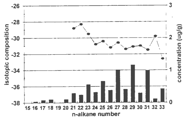
Conception Bay 30 cm sediment n-alkanes
