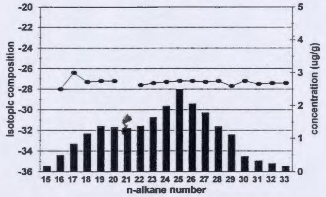
Late bloom n-alkanes
