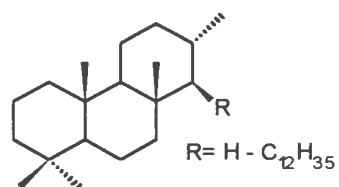
k. tricyclic terpane skeleton
