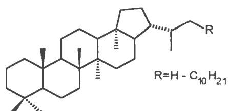
i. hopane skeleton
