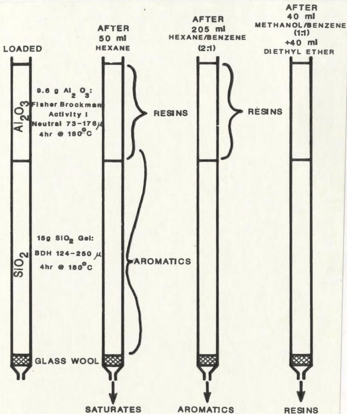
Figure 3-2: Liquid chromatography - schematic
