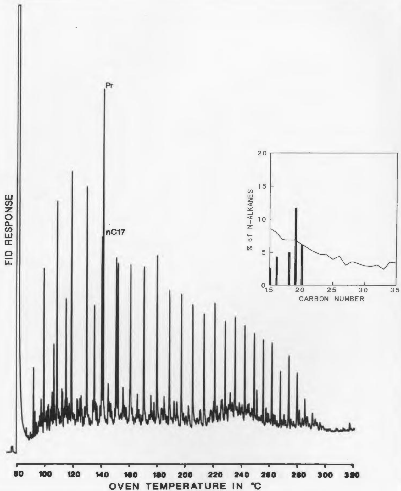
Figure C-25: Saturates, 3.2m
