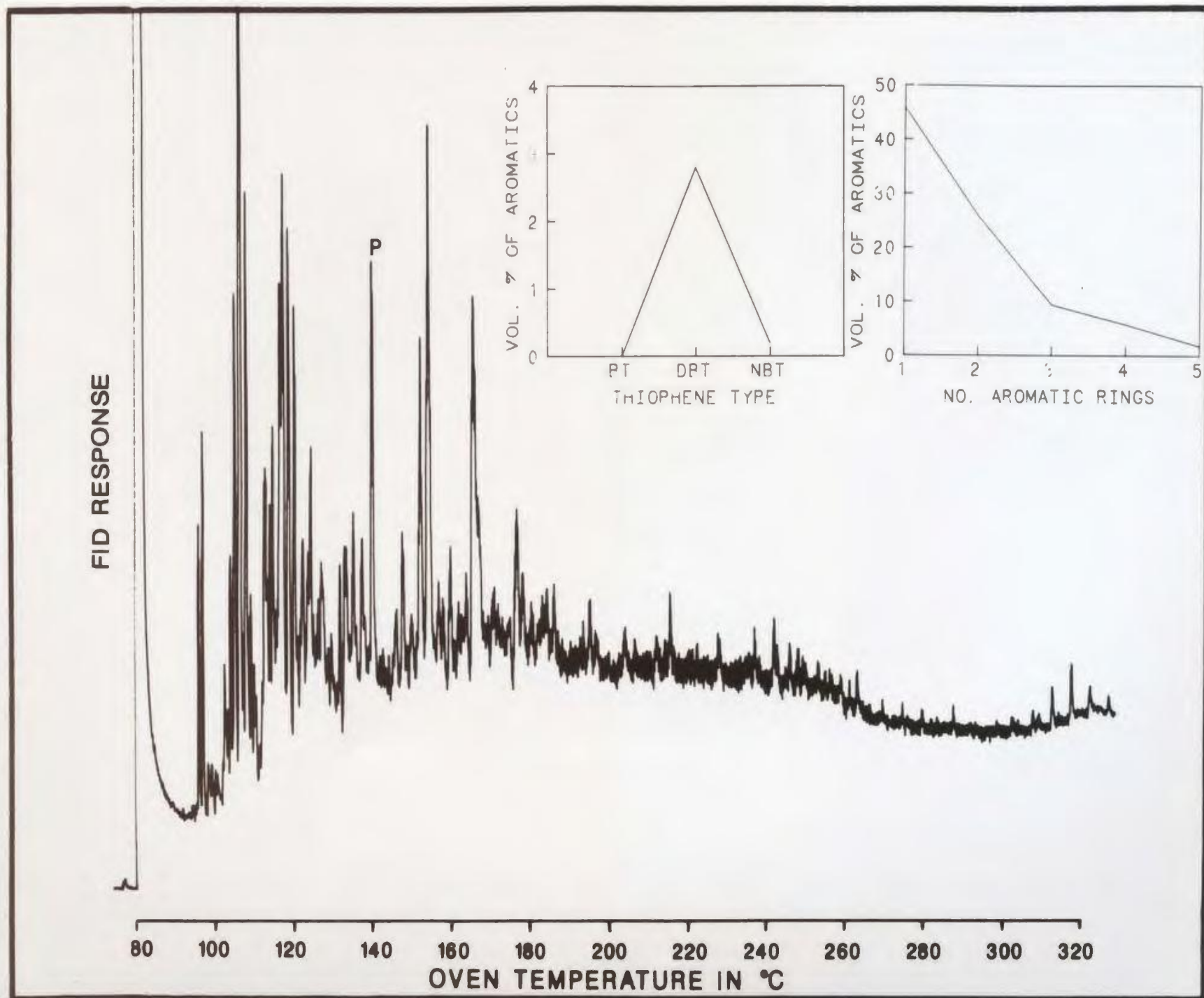
Figure C-46: Aromatics, 15.8m
