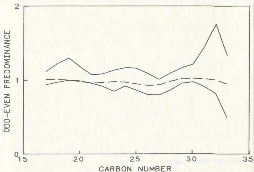
Figure 5-18: Composite OEP envelope: all bitumens (dashed line is reservoir oil)
