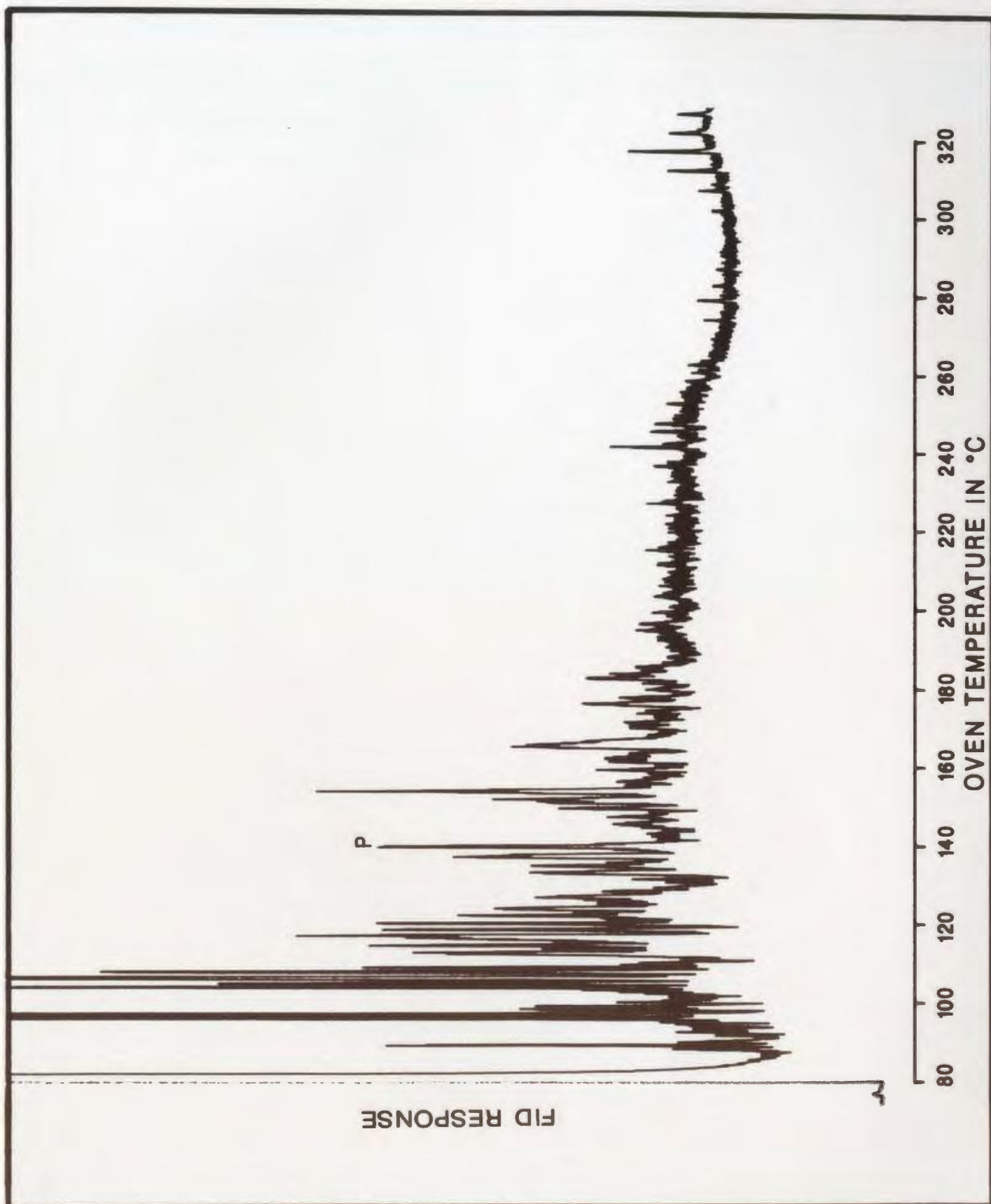
Figure C-39: Aromatics, 37.7m
