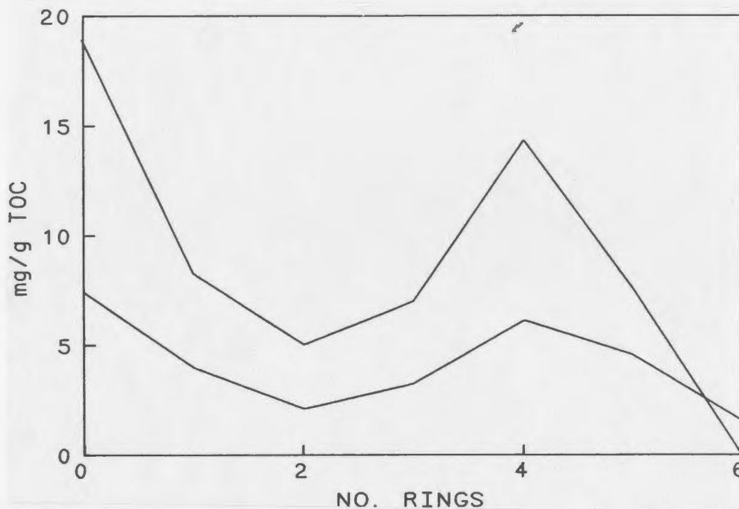
Figure 5-27: Carbon-normalized saturates distributions (Upper curve = 10.5m)
