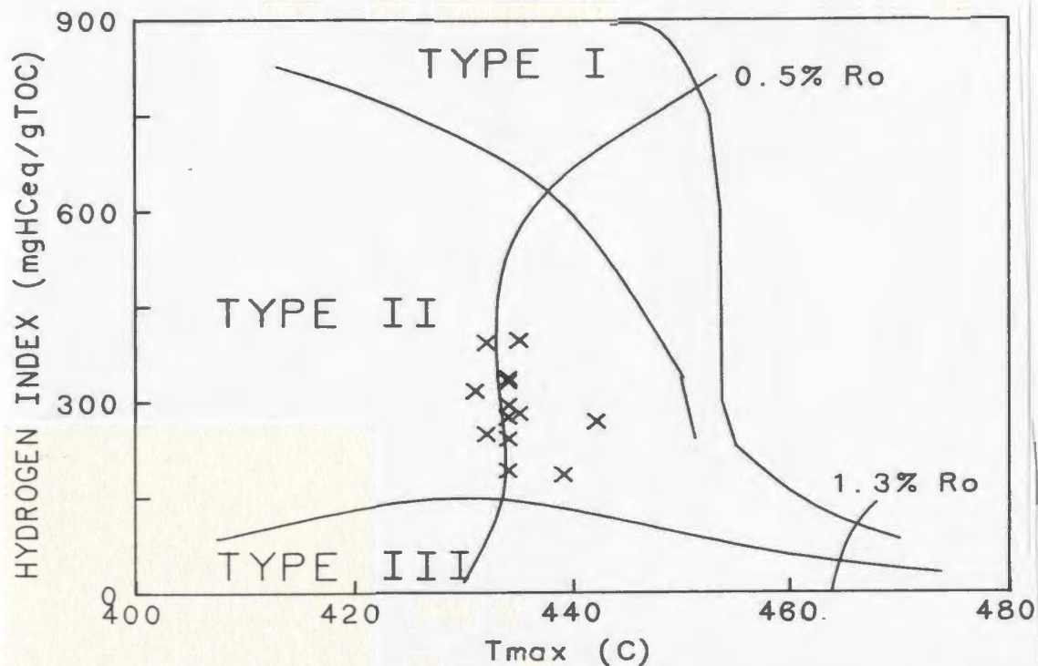
Figure 5-13: Rock-Eval HI vs. T_{\max}
