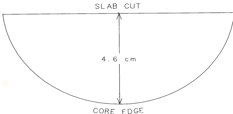
Figure A-1: Cross section of core
