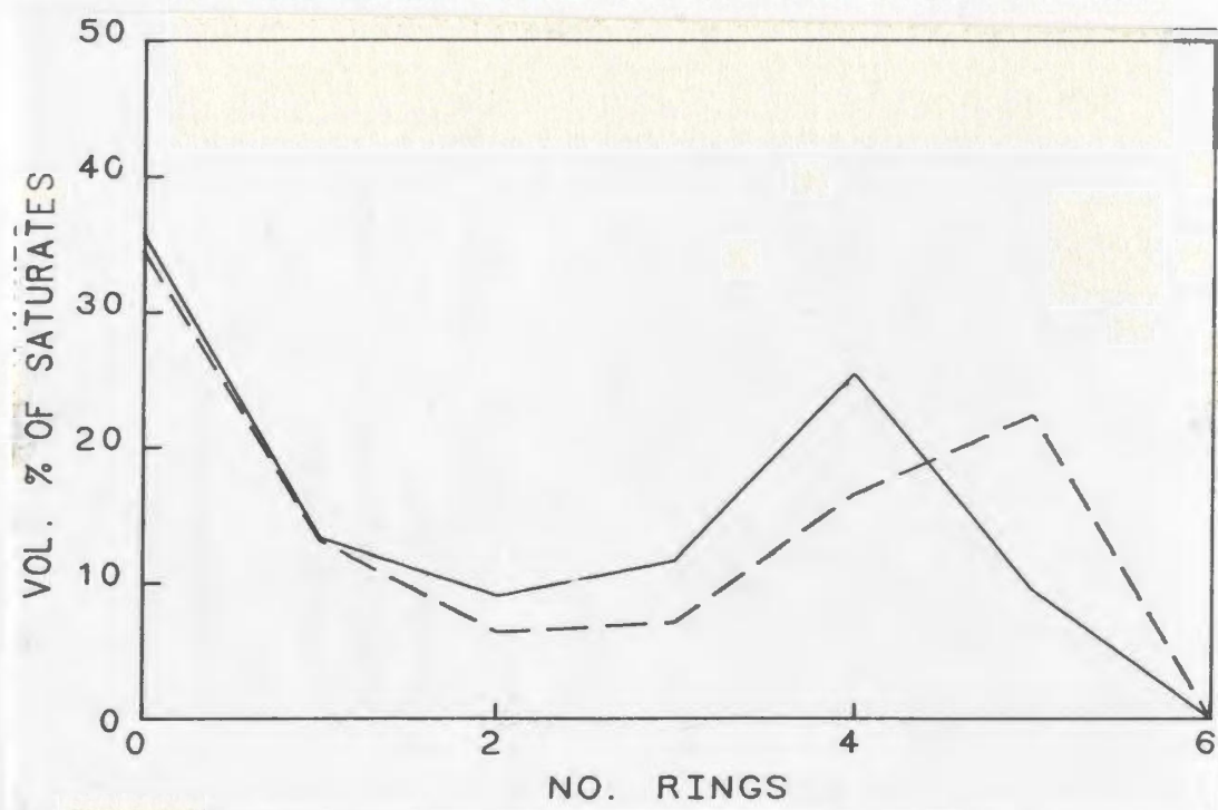
Figure 5-29: Distribution of expelled saturates, 12.4m (dashed line is reservoir oil)
