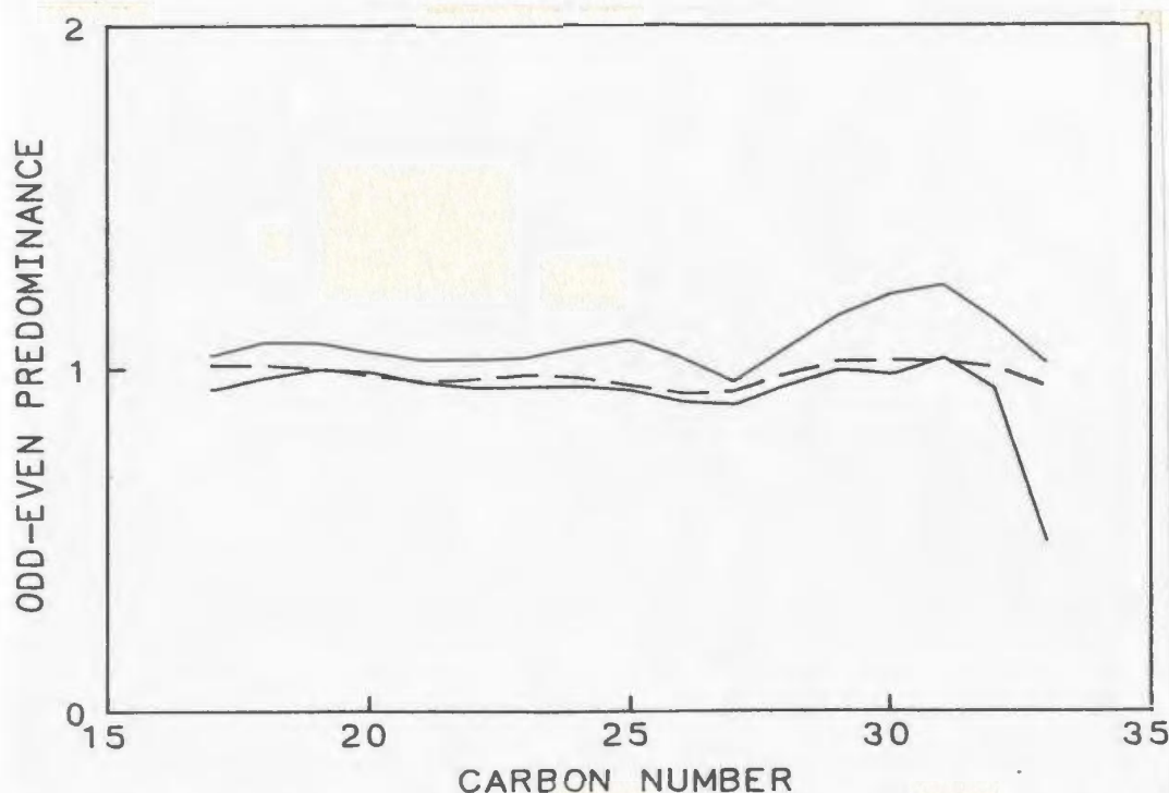
Figure 5-20: Composite OEP envelope: contaminated bitumens (dashed line is reservoir oil)
