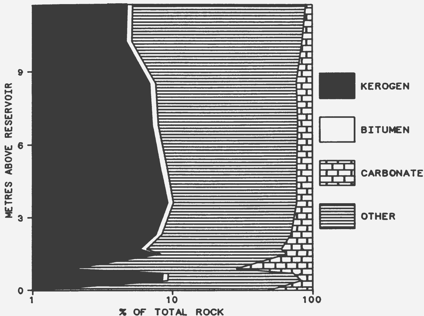
Figure 2-3: Litho-facies profile, L. Jurassic, France (after Vandenbroucke, 1972)
