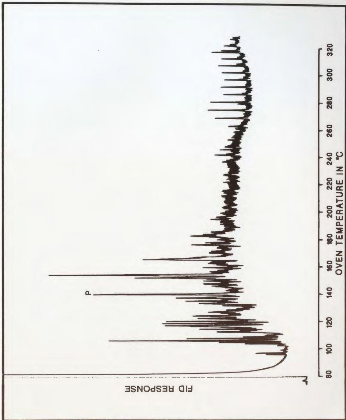
Figure C-44: Aromatics, 19.6m
