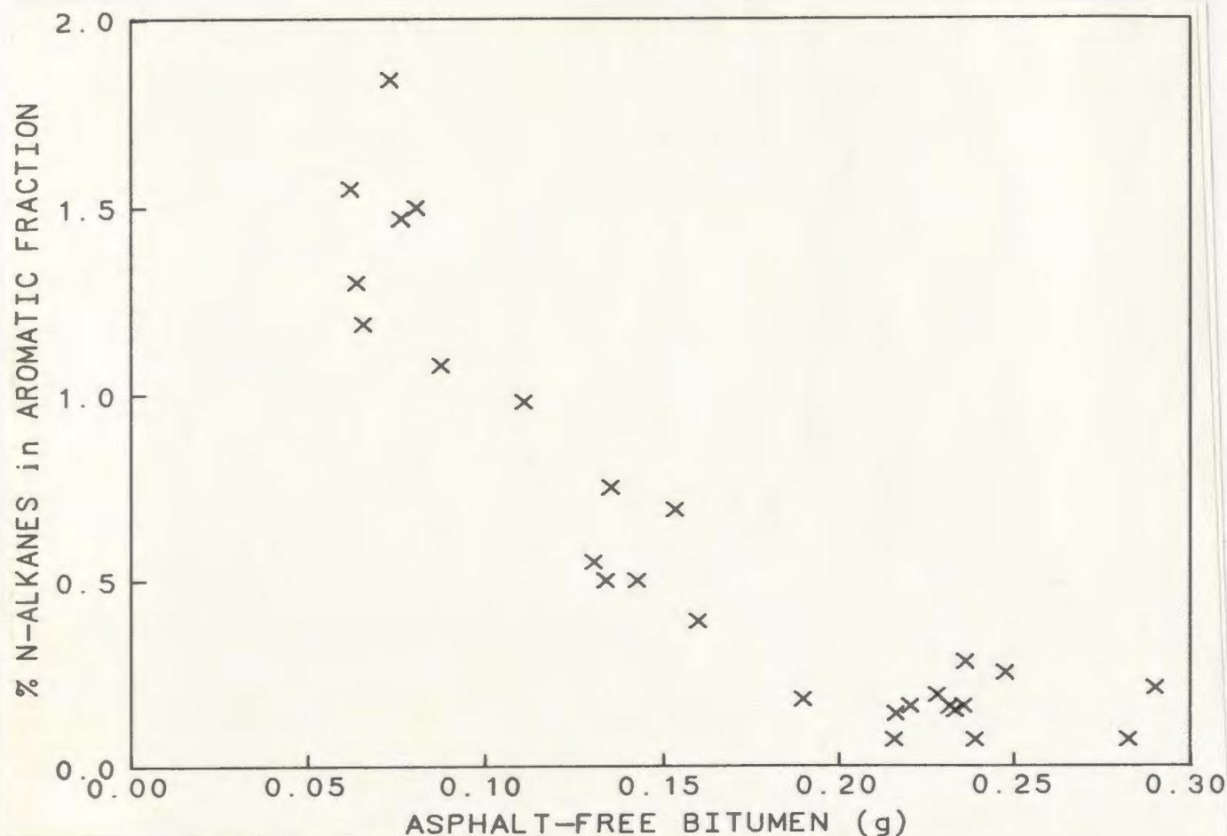
Figure 5-8: Cross-contamination vs. column feed
