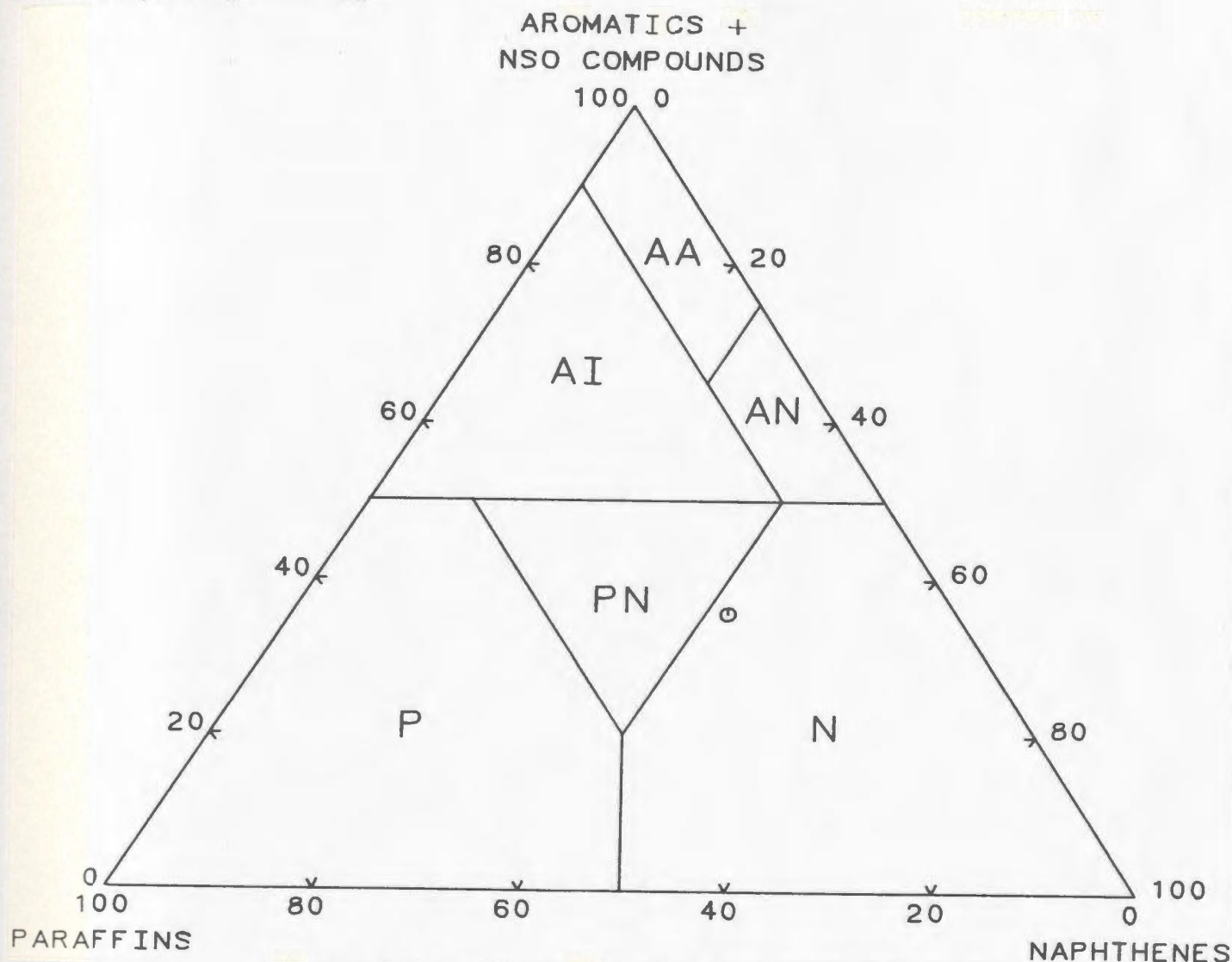
Figure 5-14: Oil classification by compound type
