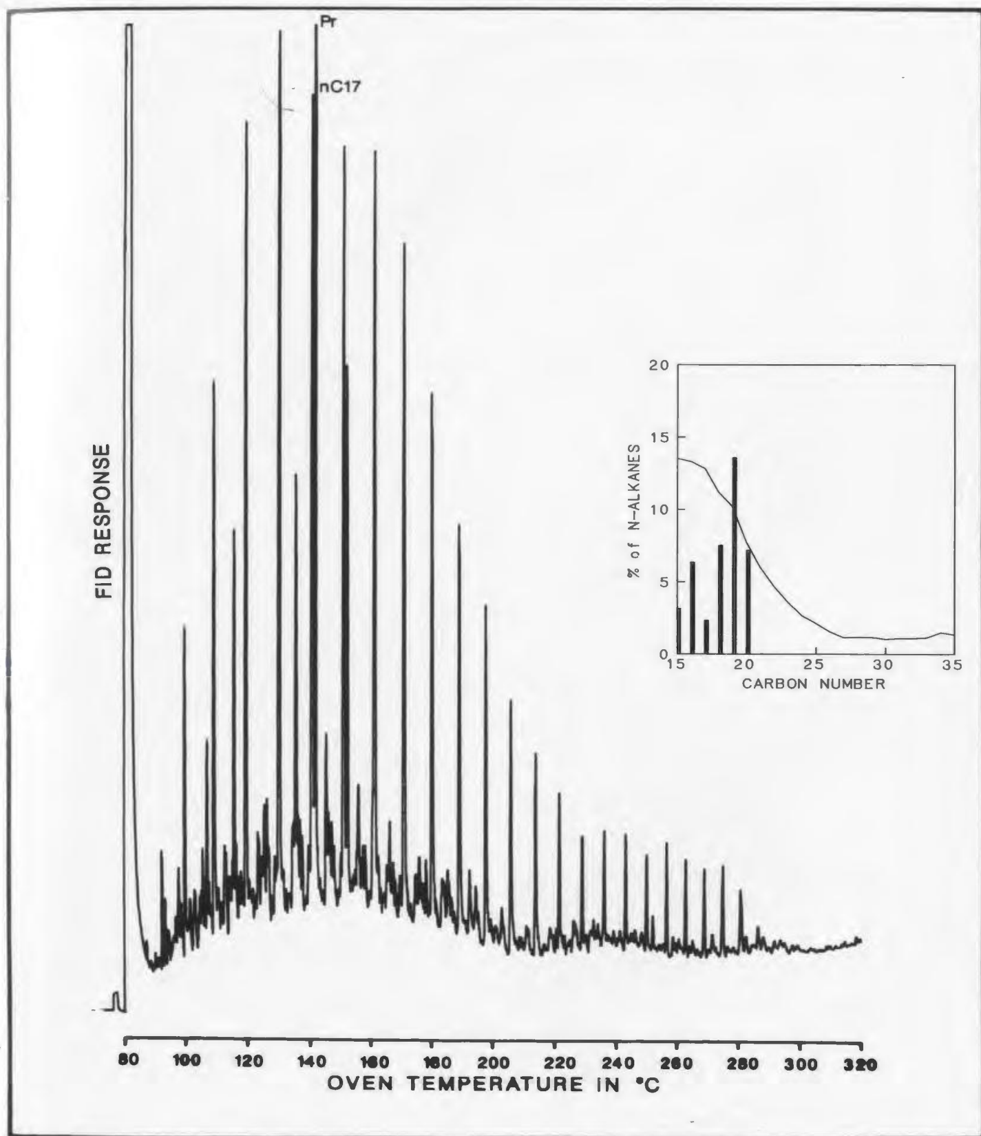
Figure C-10: Saturates, 43.1m
