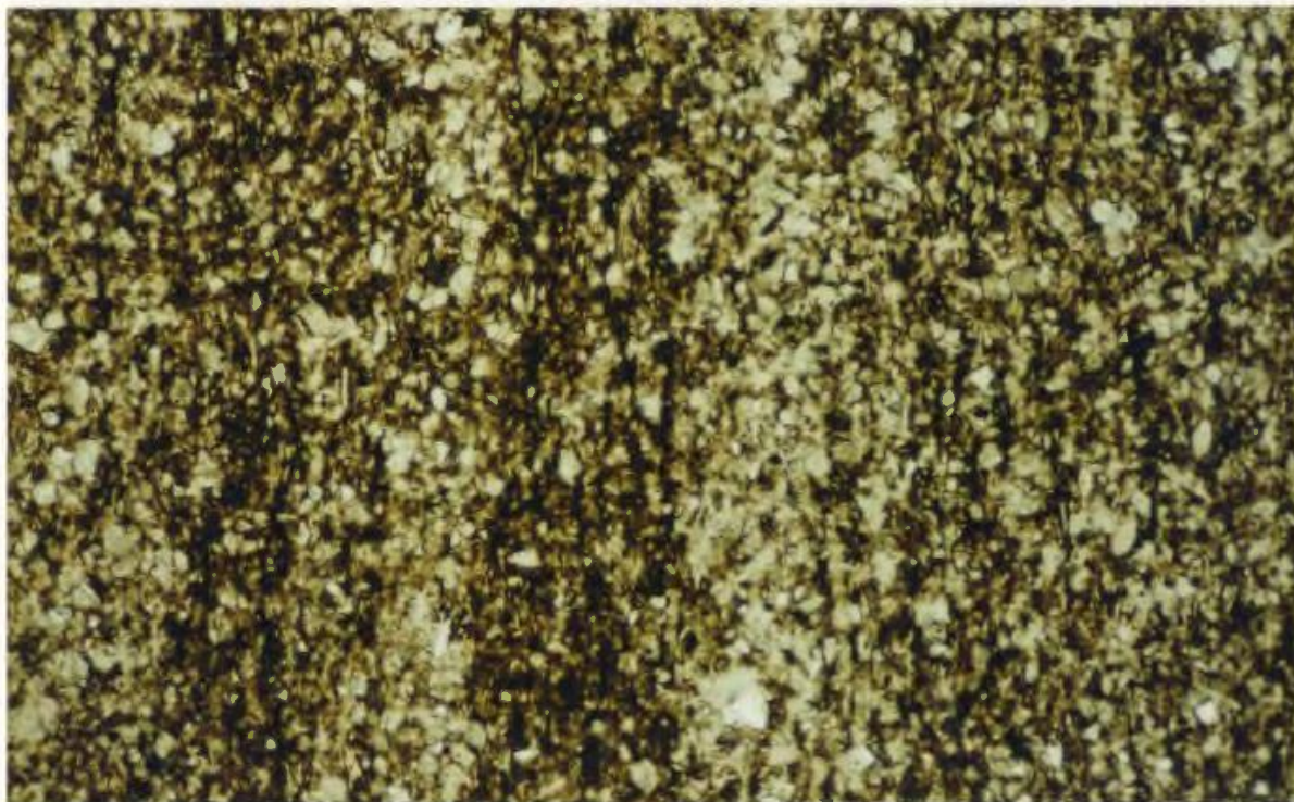
Figure 4-4: Laminated siltstone, 43.1m (x30)
