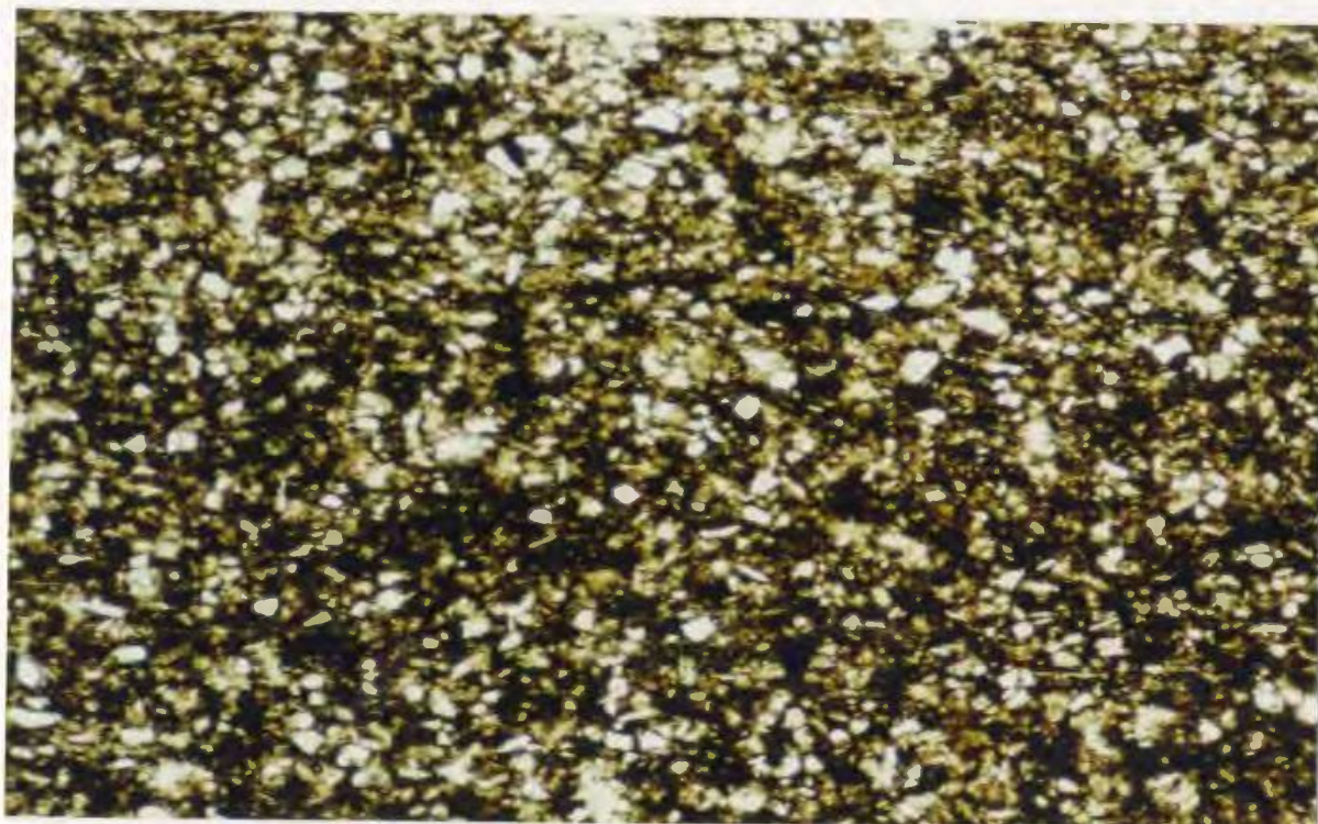
Figure 4-8: Massive siltstone, 3.2m (x30)
