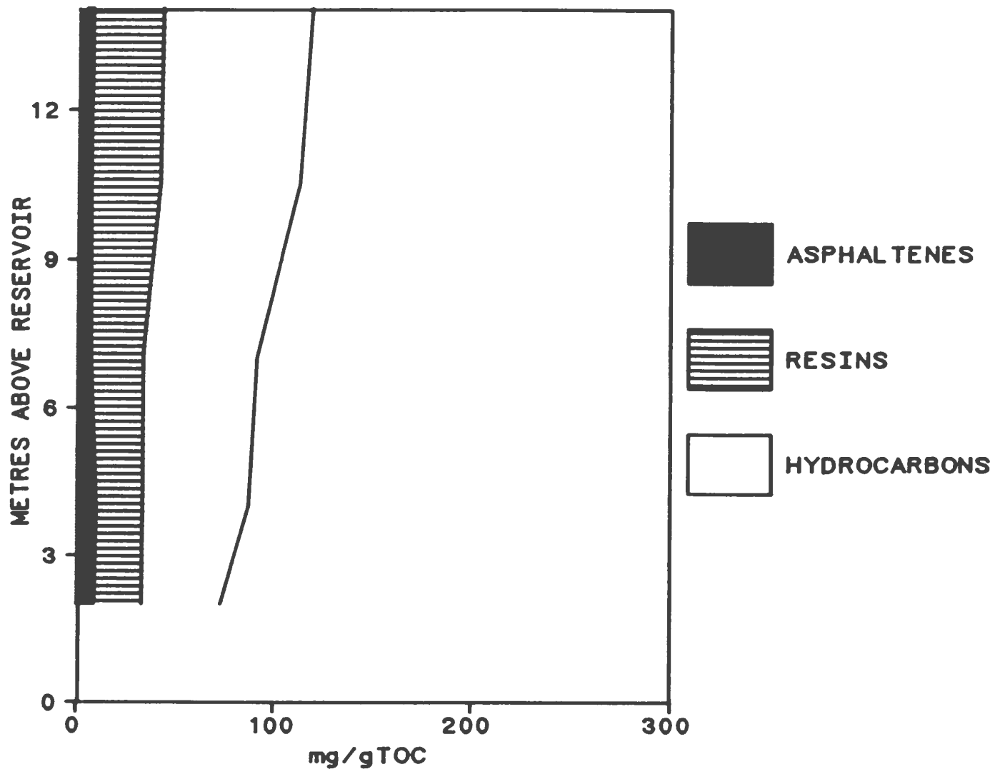
Figure 2-2: Carbon-normalized bitumen profile, U. Devonian, Algeria
