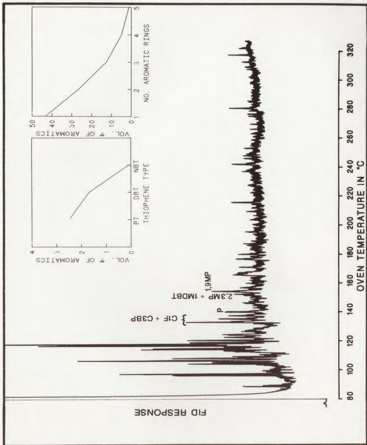
Figure C-34: Aromatics, 66.4m
