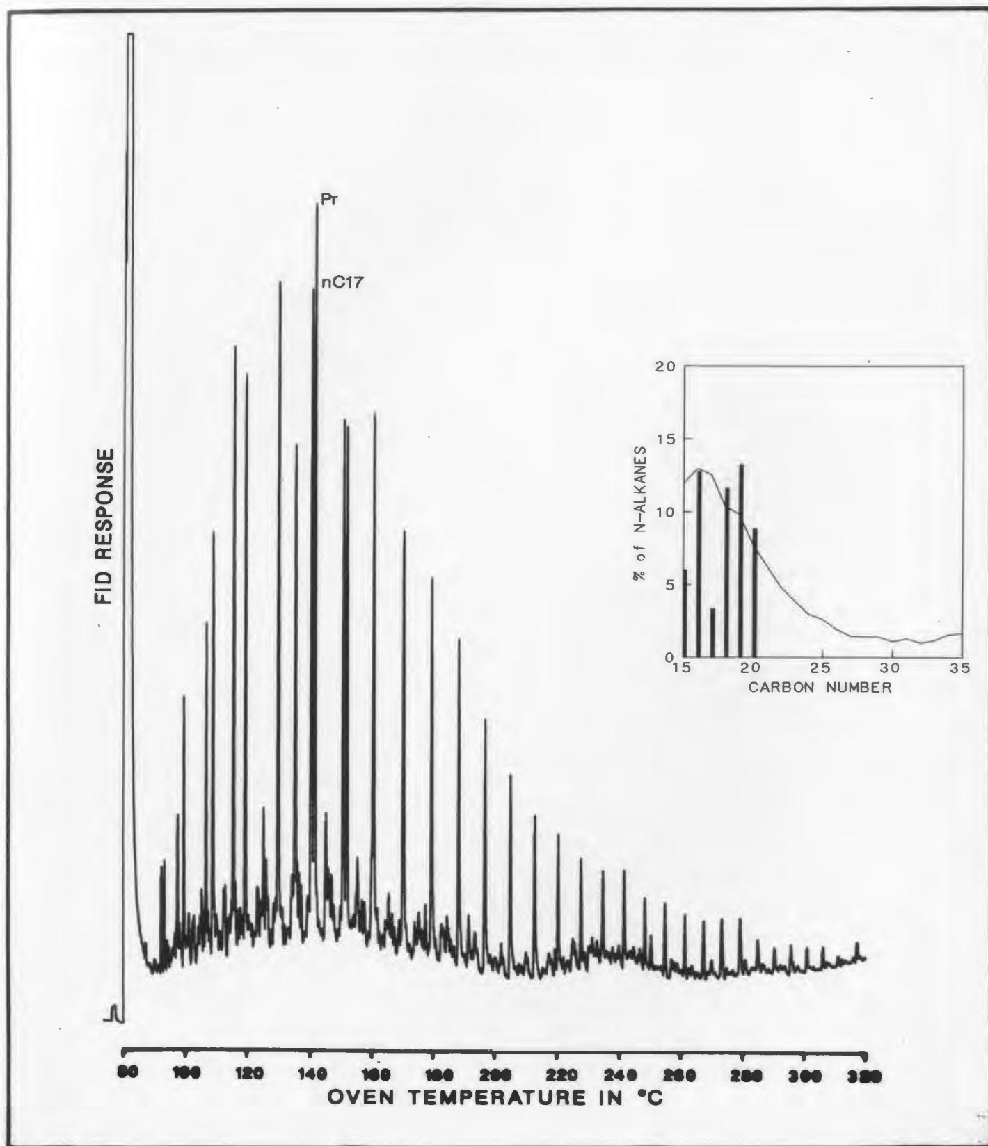
Figure C-7: Saturates, 60.2m
