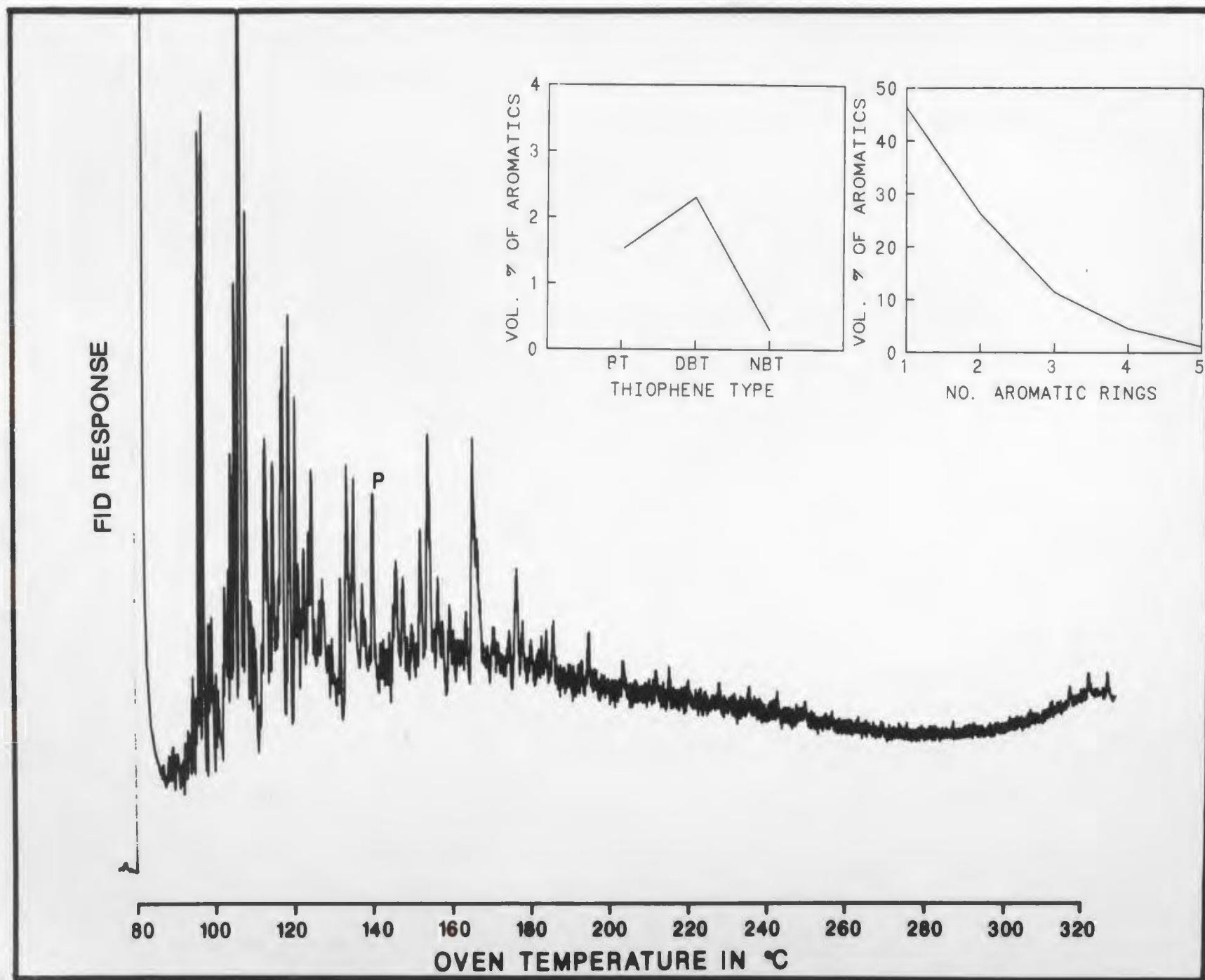
Figure C-56: Aromatics, oil
