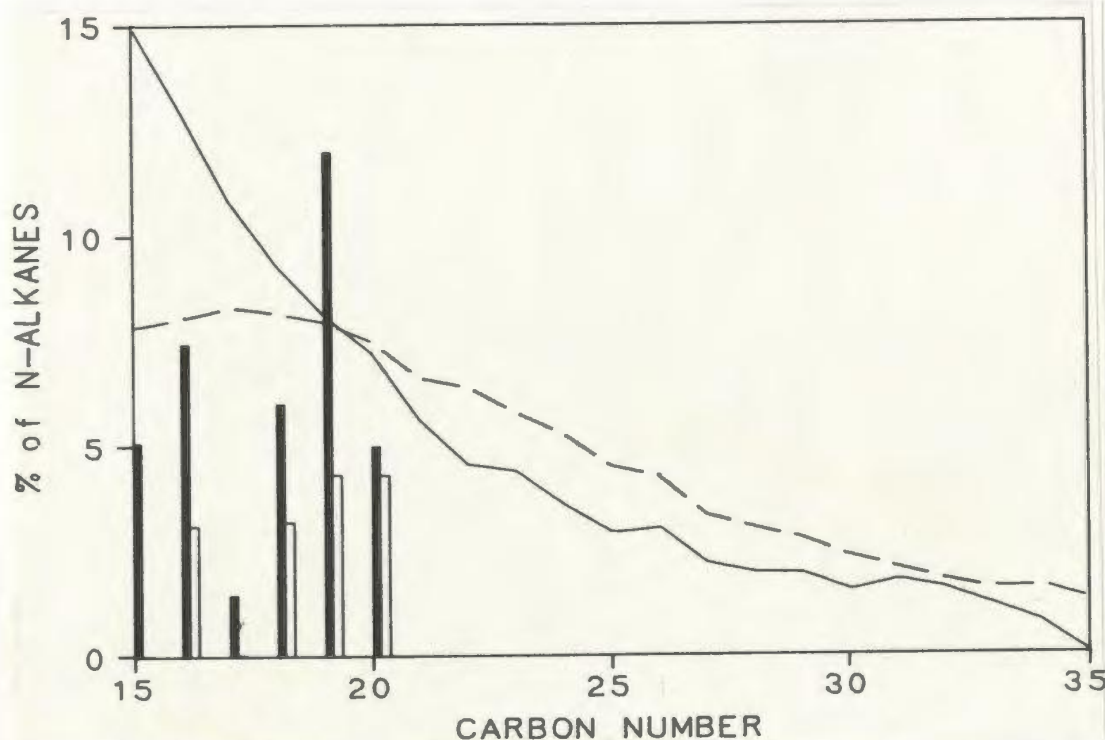
Figure 5-23: Distribution of expelled n-alkanes, 12.4m (dashed line, open bars = reservoir oil)
