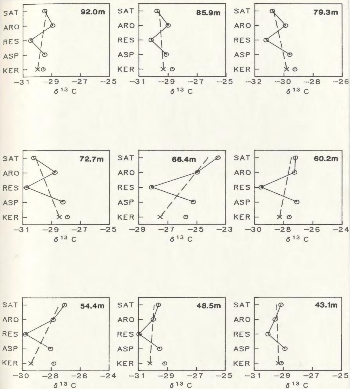
Figure 6-3: Isotopic type-curves (after Stahl, 1978)
