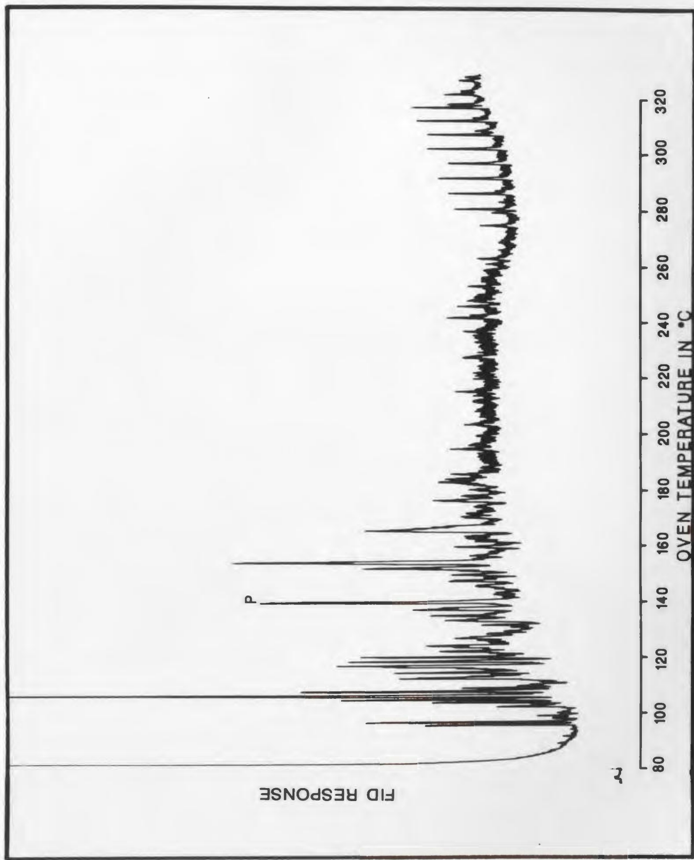
Figure C-51: Aromatics, 6.2m
