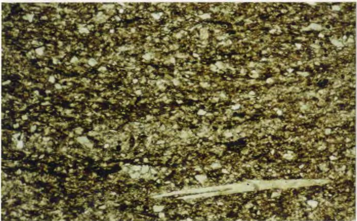
Figure 4-6: Weakly laminated siltstone, 25.5m (x30)
