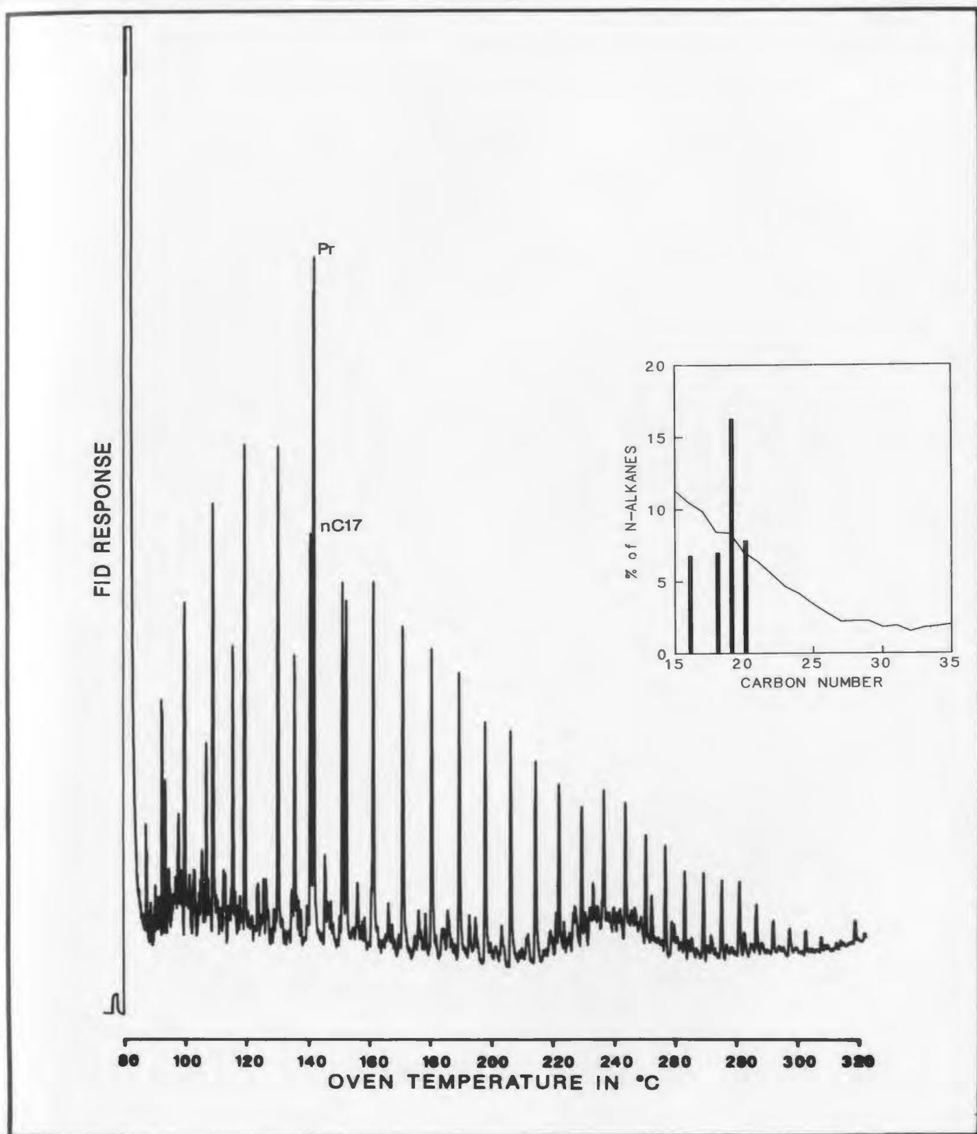
Figure C-5: Saturates, 72.7m
