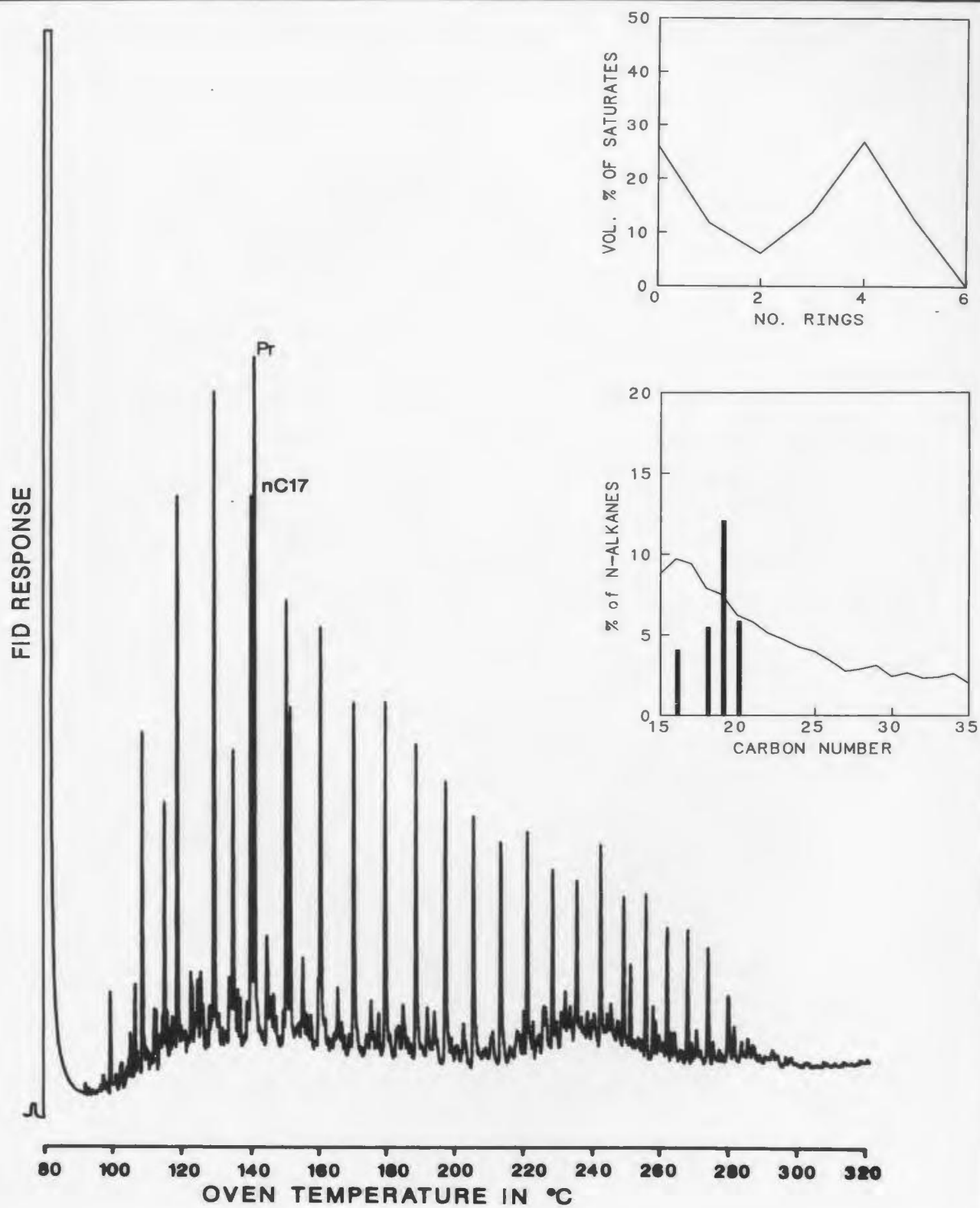
Figure C-17: Saturates, 17.9m
