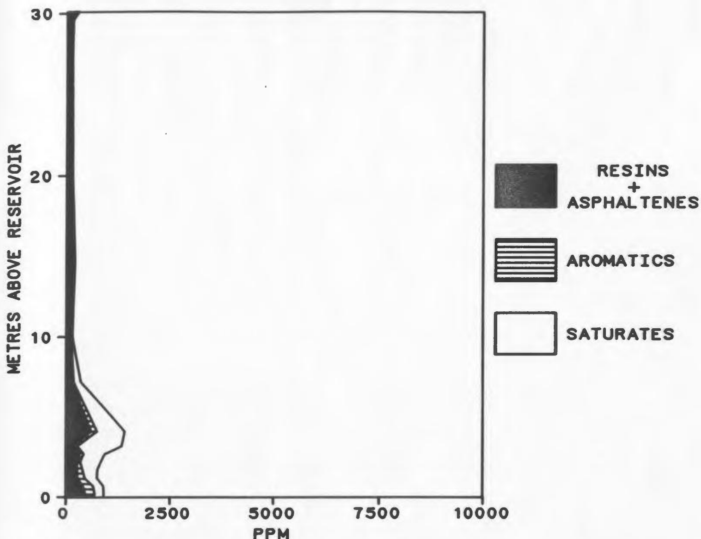
Figure 2-8: Bitumen profile, U. Carboniferous, Germany
