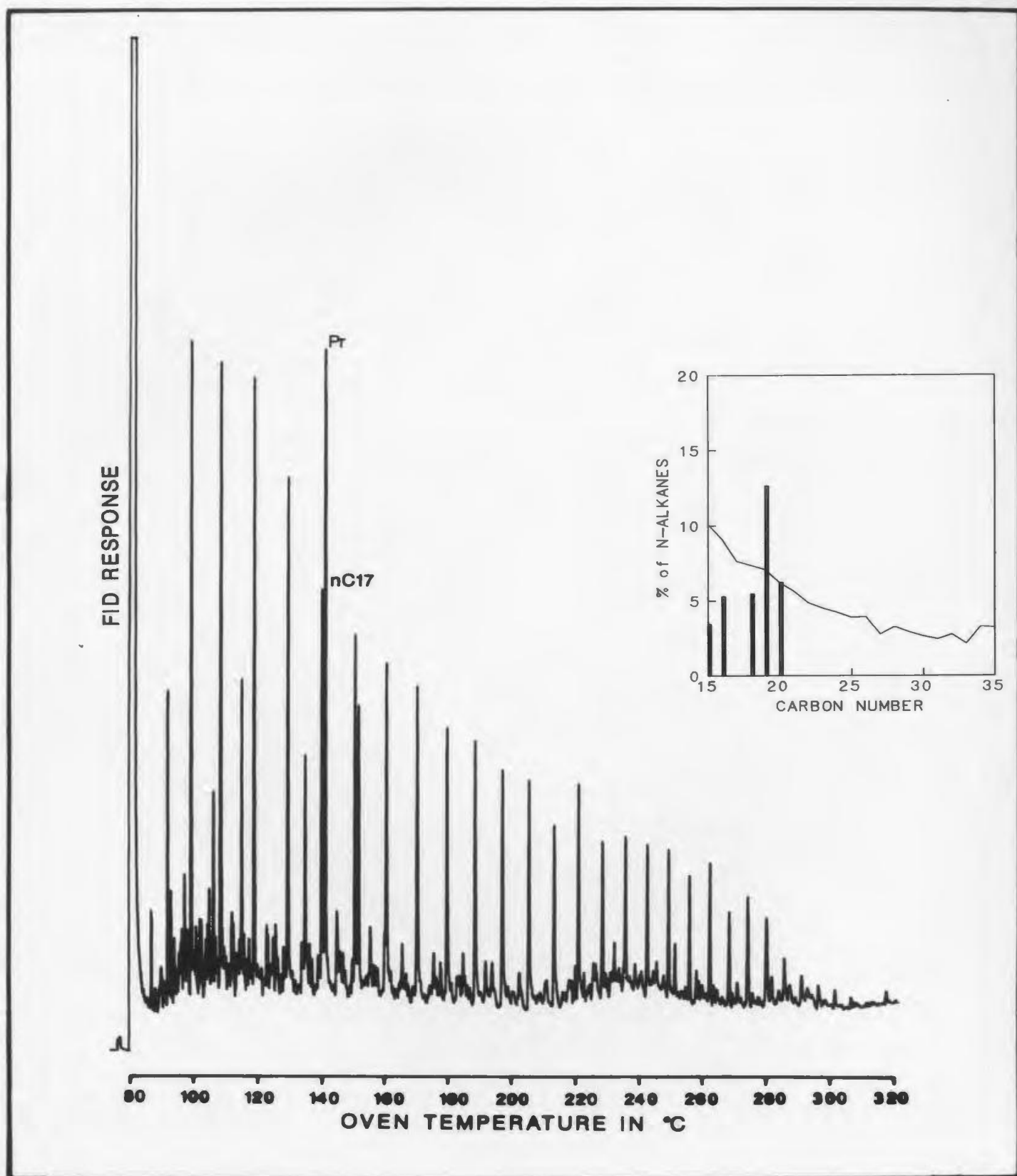
Figure C-26: Saturates, 1.4m
