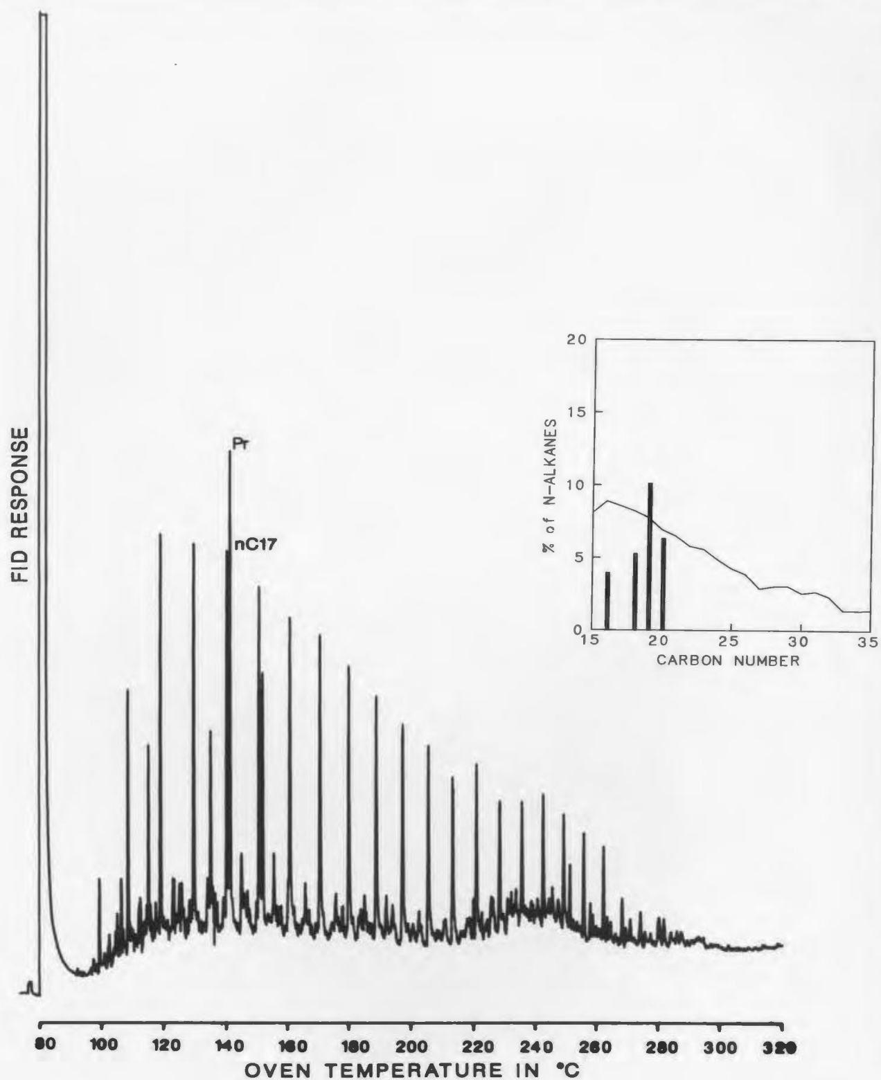
Figure C-21: Saturates, 9.2m
