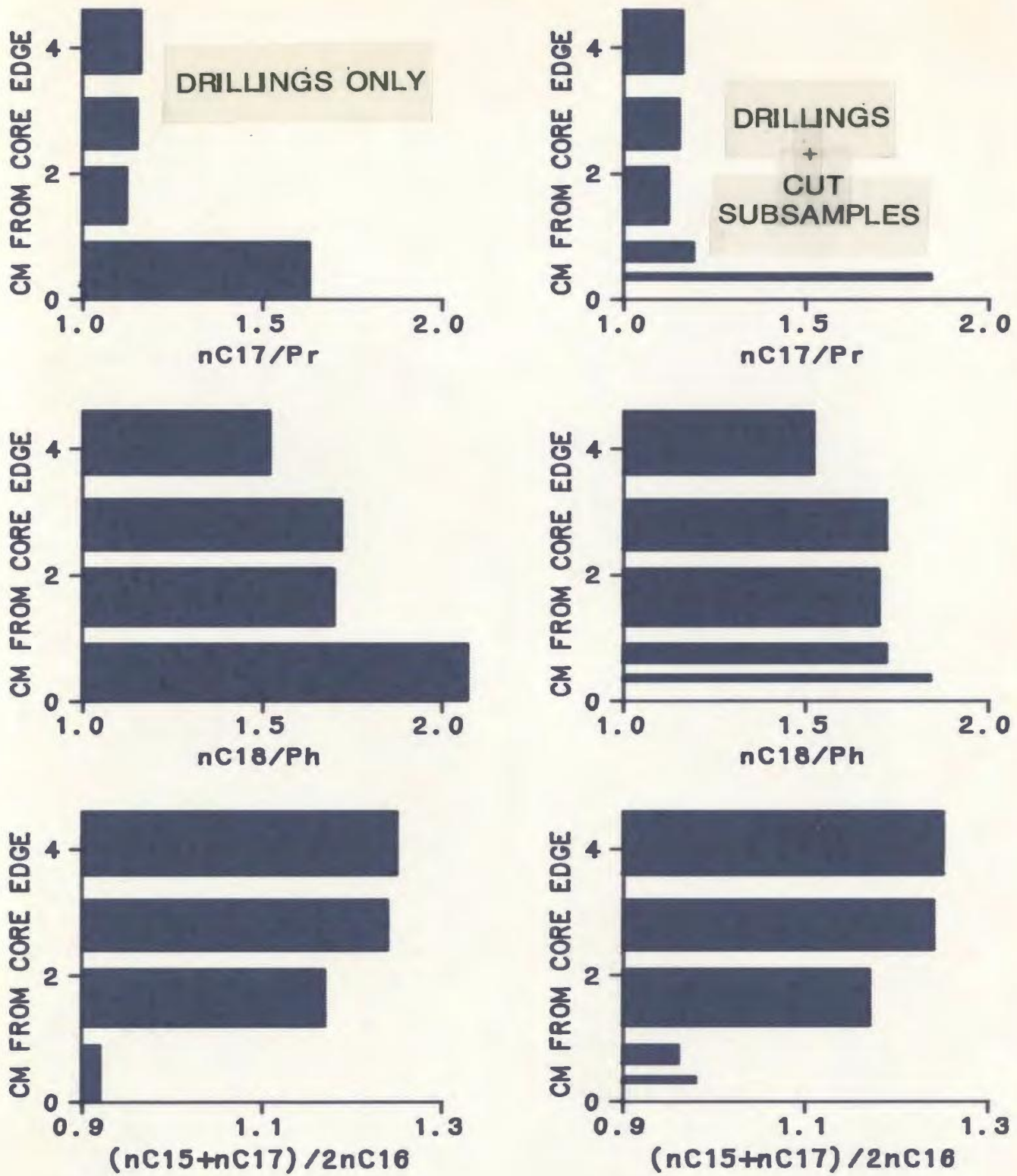
Figure A-2: Variation in component ratios across core
