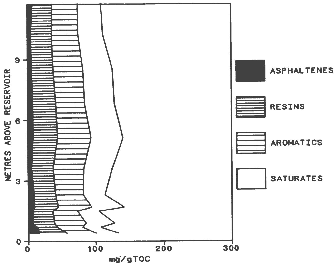
Figure 2-4: Carbon-normalized bitumen profile, L. Jurassic, France (after Vandembroucke, 1972)
