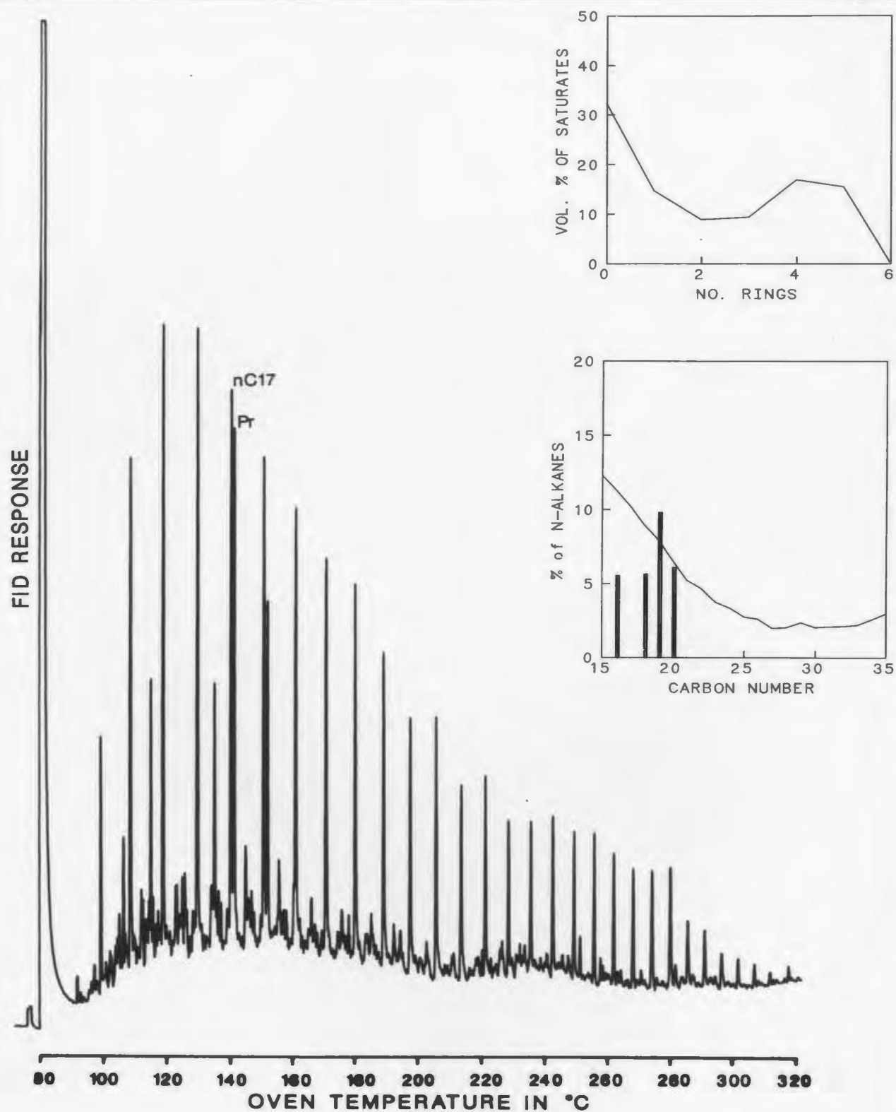
Figure C-18: Saturates, 15.8m
