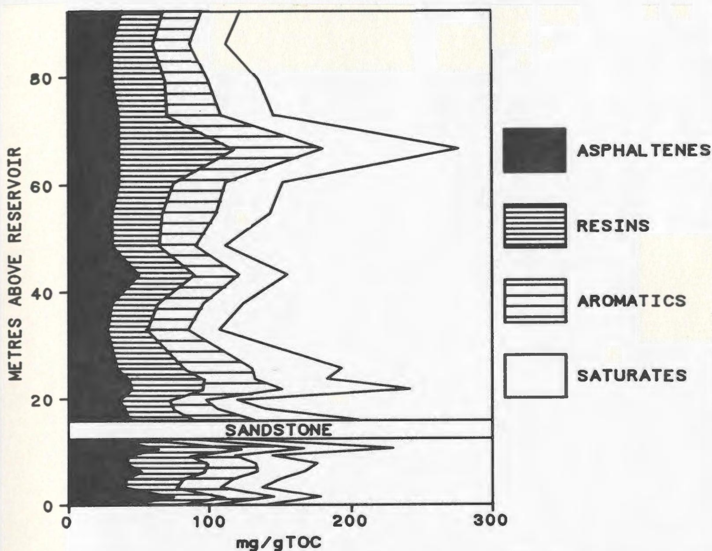
Figure 5-2: Carbon-normalized bitumen profile
