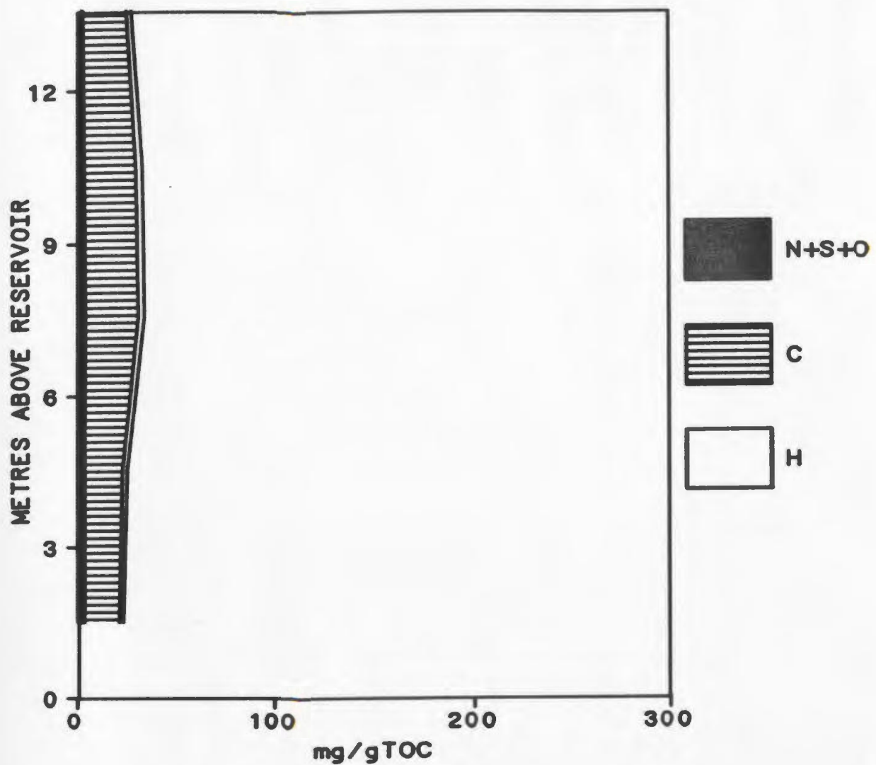
Figure 2-1: Carbon-normalized bitumen profile, M. Devonian, USSR
