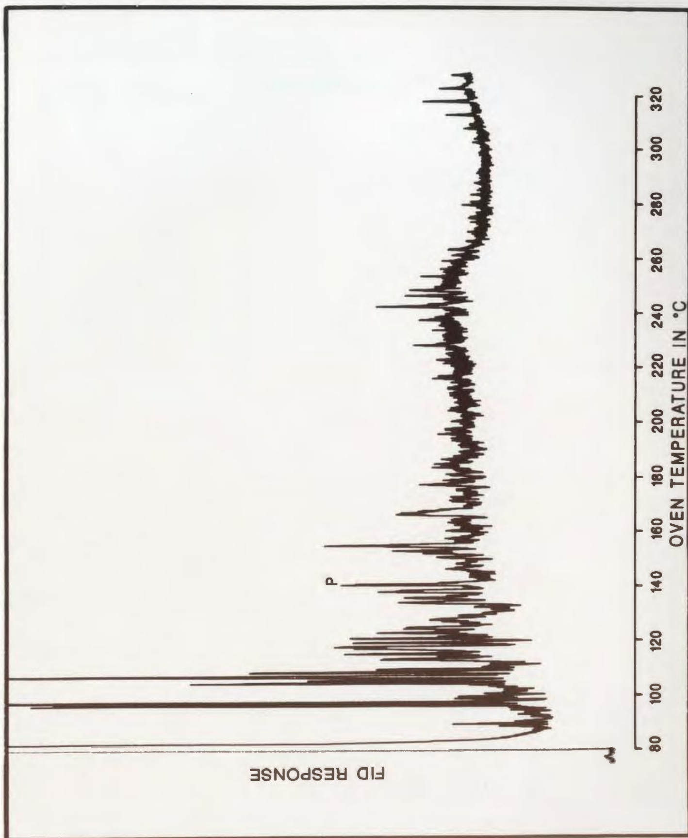
Figure C-36: Aromatics, 54.4m
