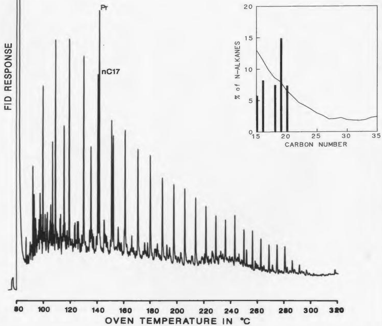
Figure C-12: Saturates, 32.8m
