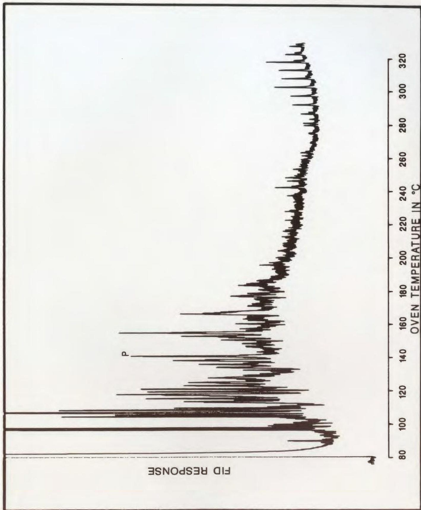
Figure C-38: Aromatics, 43.1m
