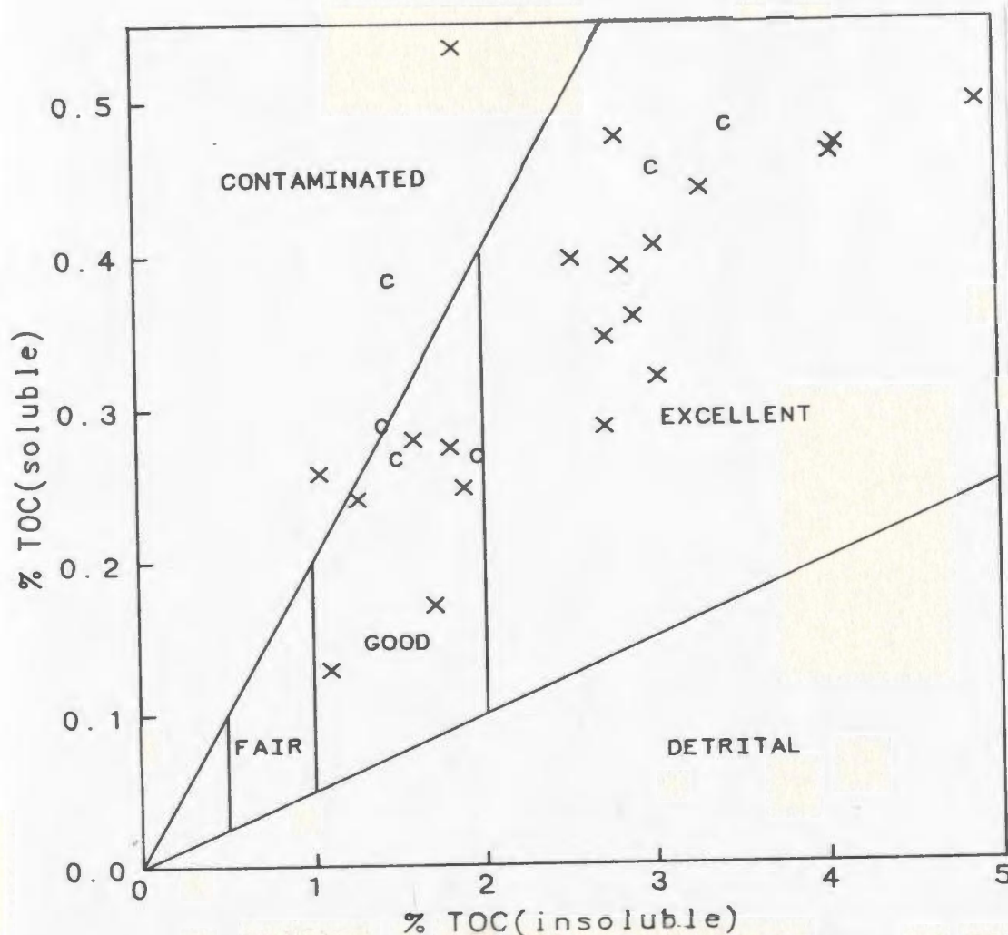
Figure 5-10: Soluble vs. insoluble organic carbon
