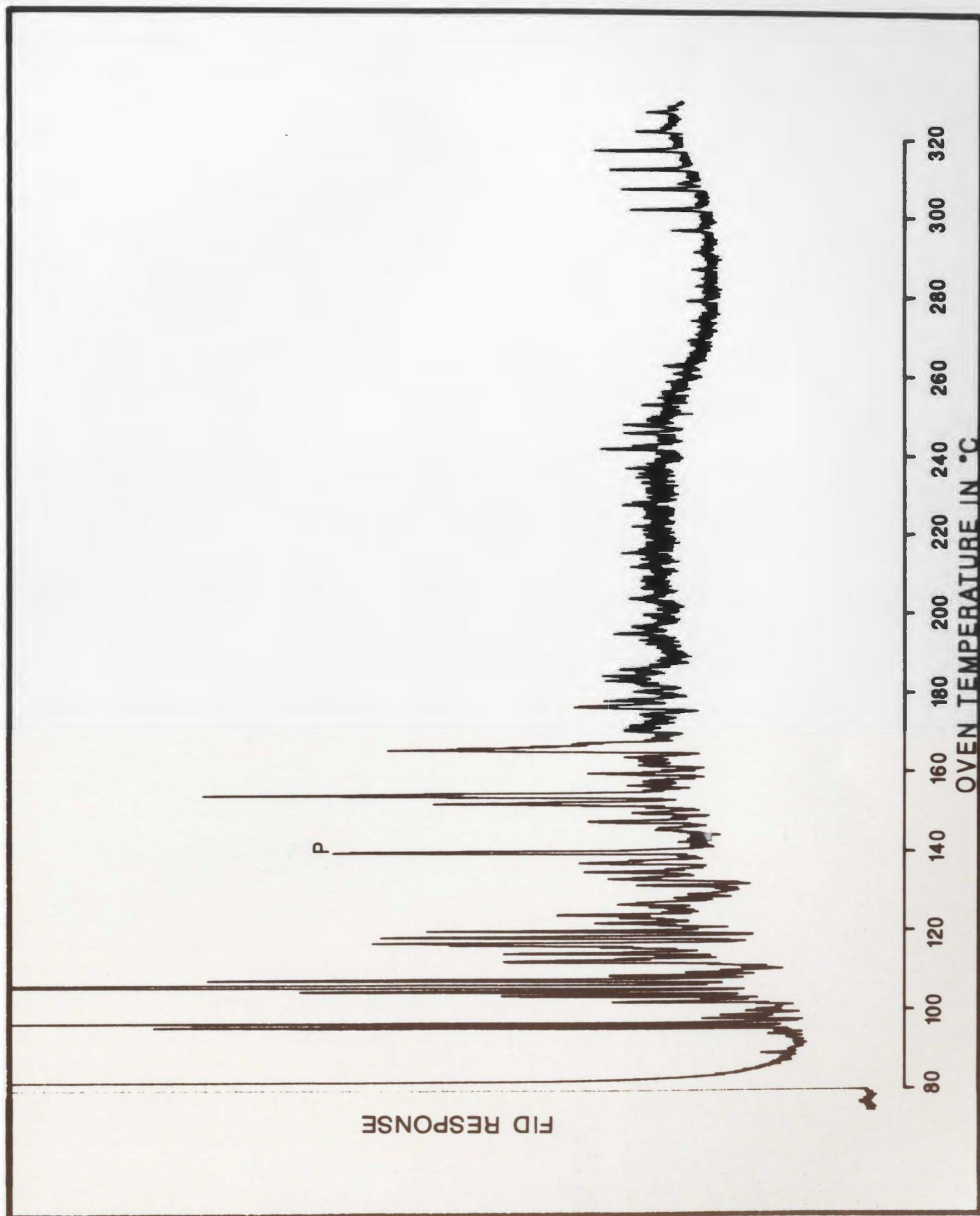
Figure C-52: Aromatics, 4.9m
