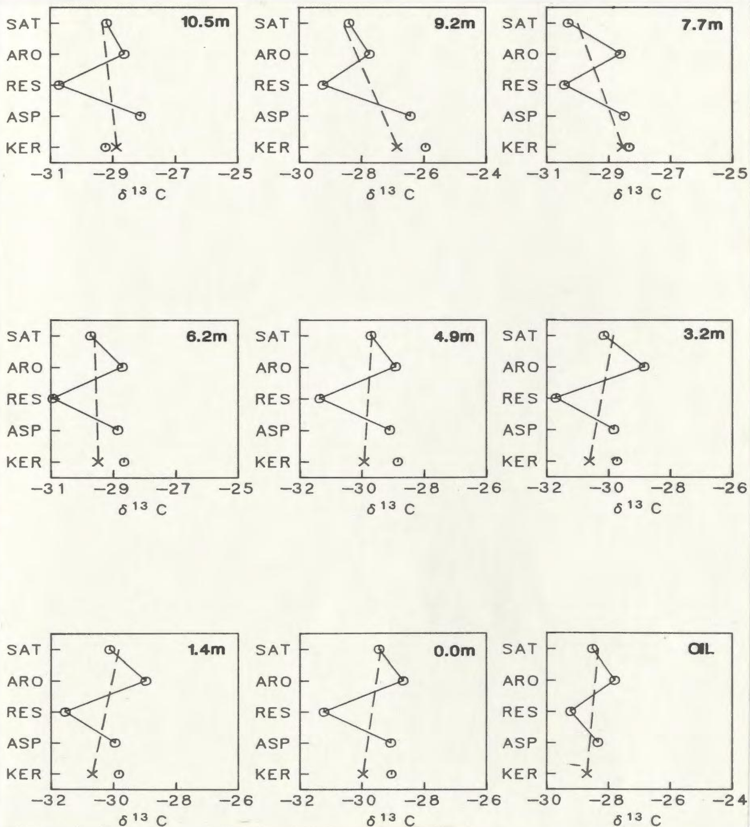
Figure 6-5: Isotopic type-curves (after Stahl, 1978)
