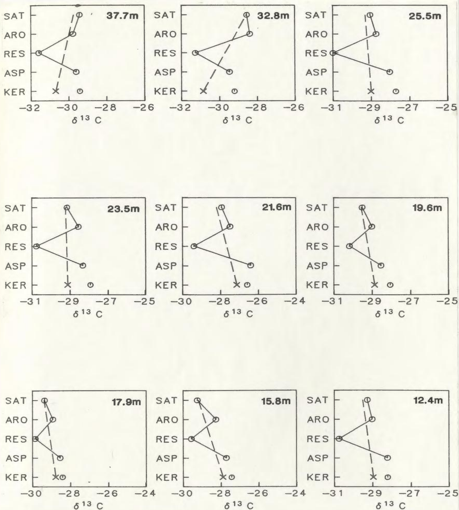
Figure 6-4: Isotopic type-curves (after Stahl, 1978)
