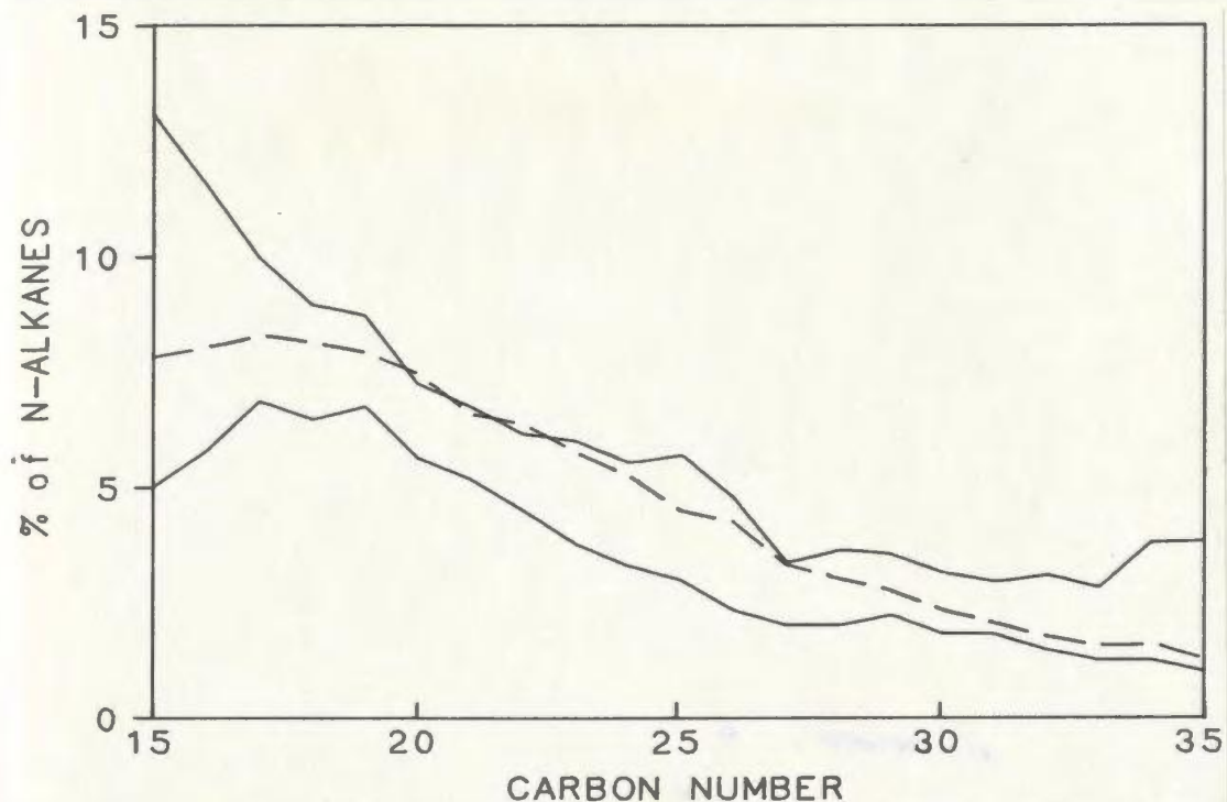
Figure 5-15: Composite n-alkane envelope: all unaltered bitumens (dashed line is reservoir oil)
