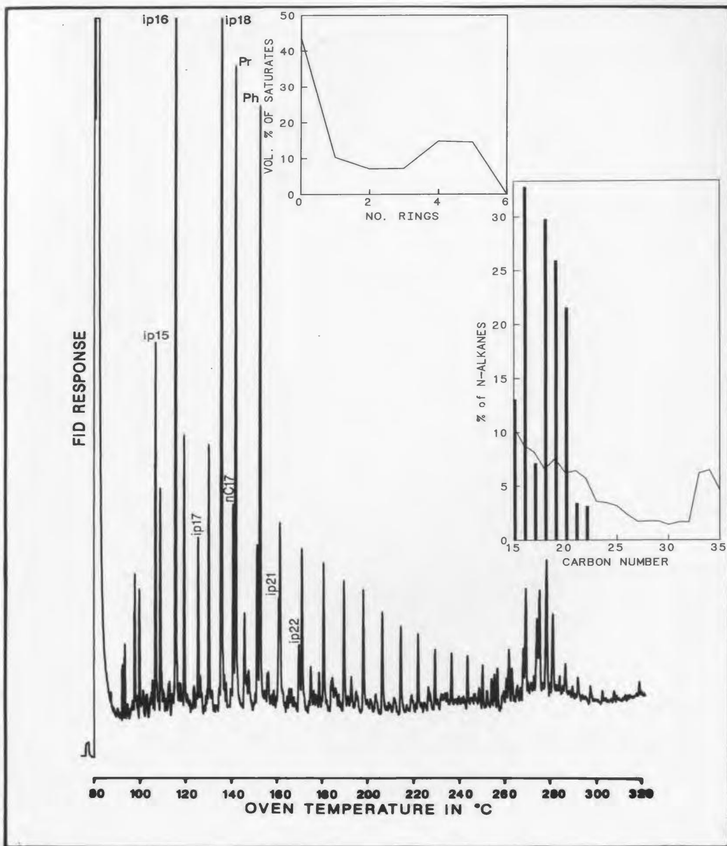
Figure C-6: Saturates, 66.4m
