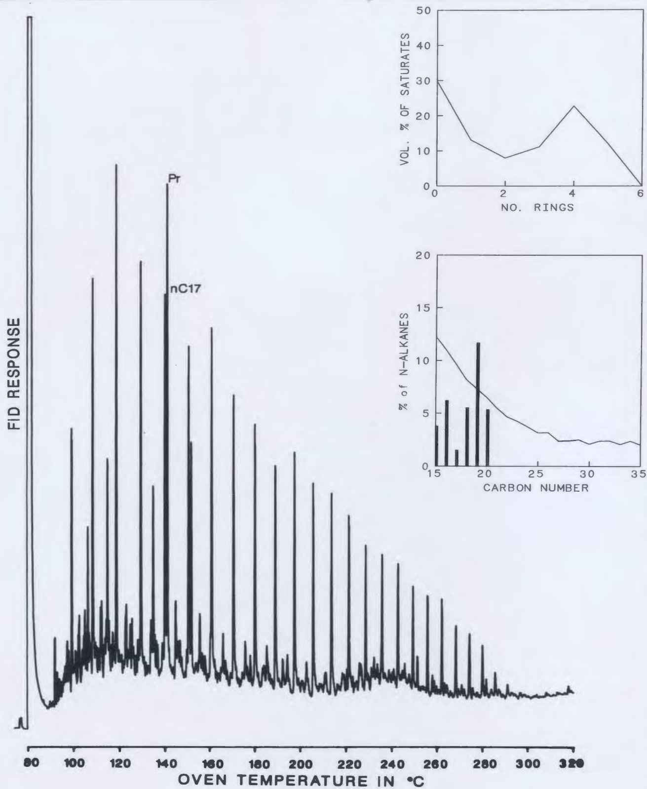
Figure C-20: Saturates, 10.5m
