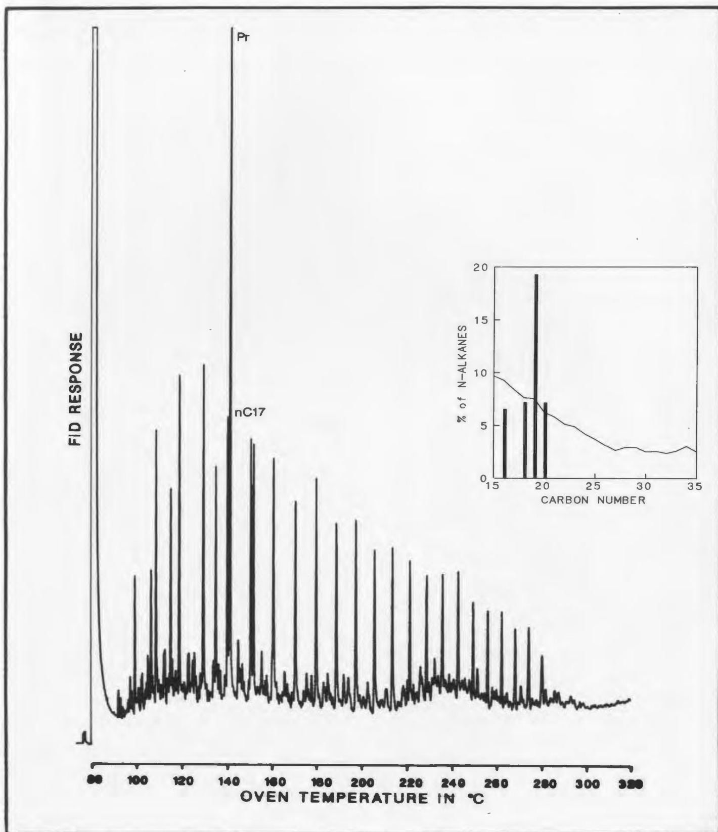
Figure C-9: Saturates, 48.5m
