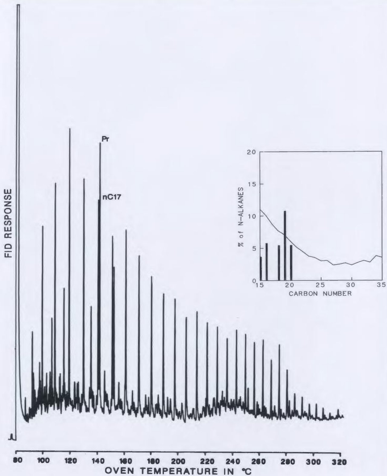
Figure C-22: Saturates, 7.7m
