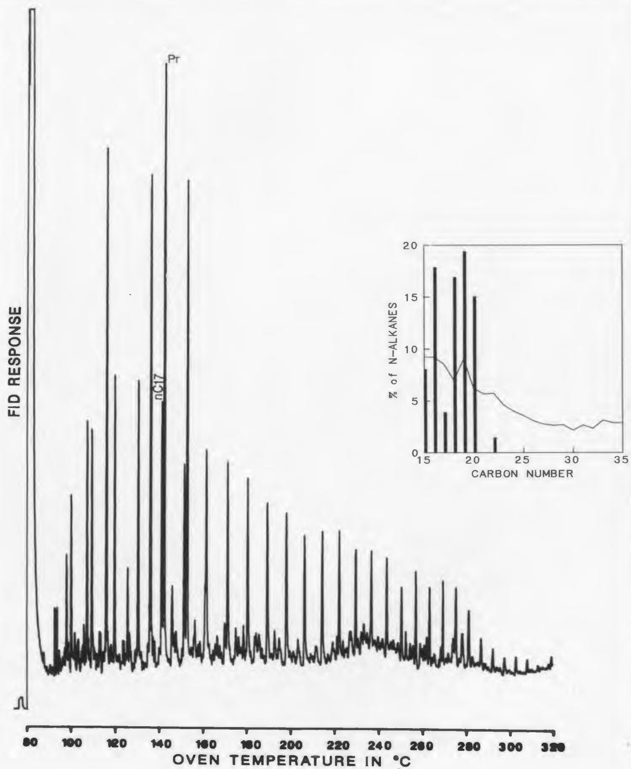
Figure C-8: Saturates, 54.4m
