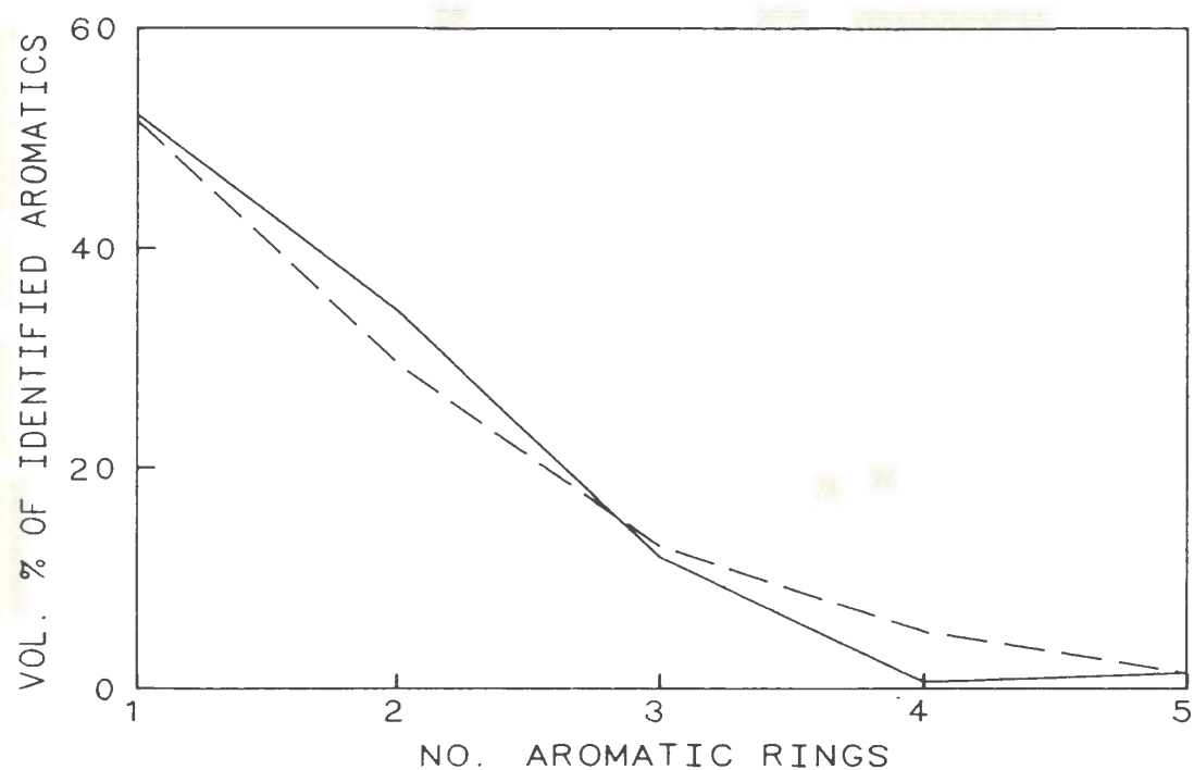
Figure 5-26: Distribution of expelled aromatics, 12.4m (dashed line is reservoir oil)
