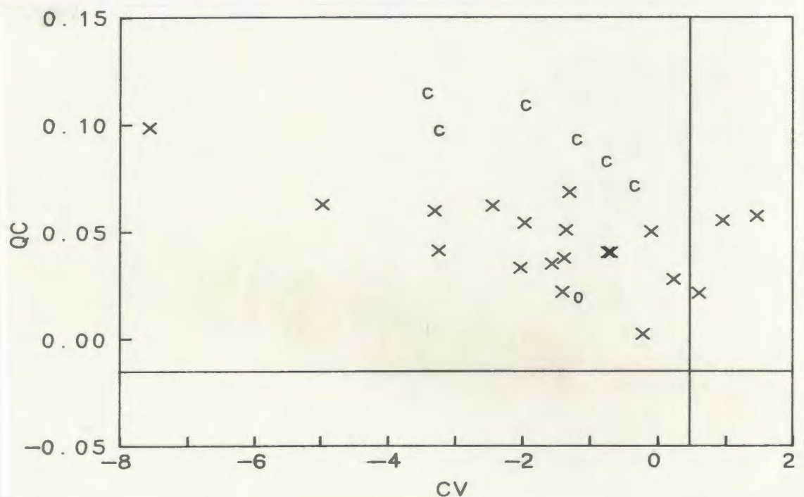
Figure 6-1: QC vs CV (after Sofer, 1984)
