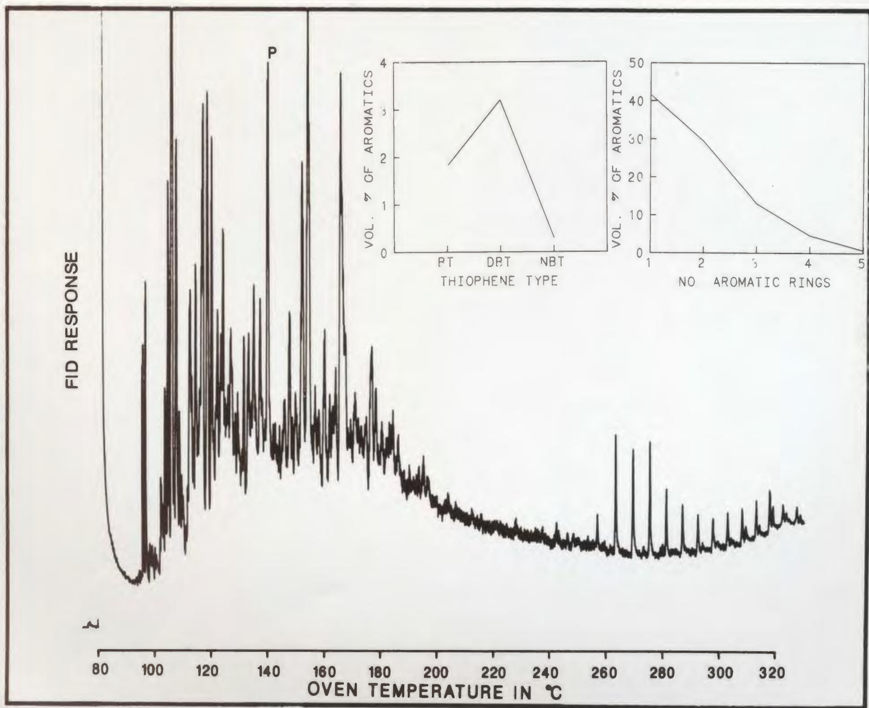
Figure C-55: Aromatics, 0.0m
