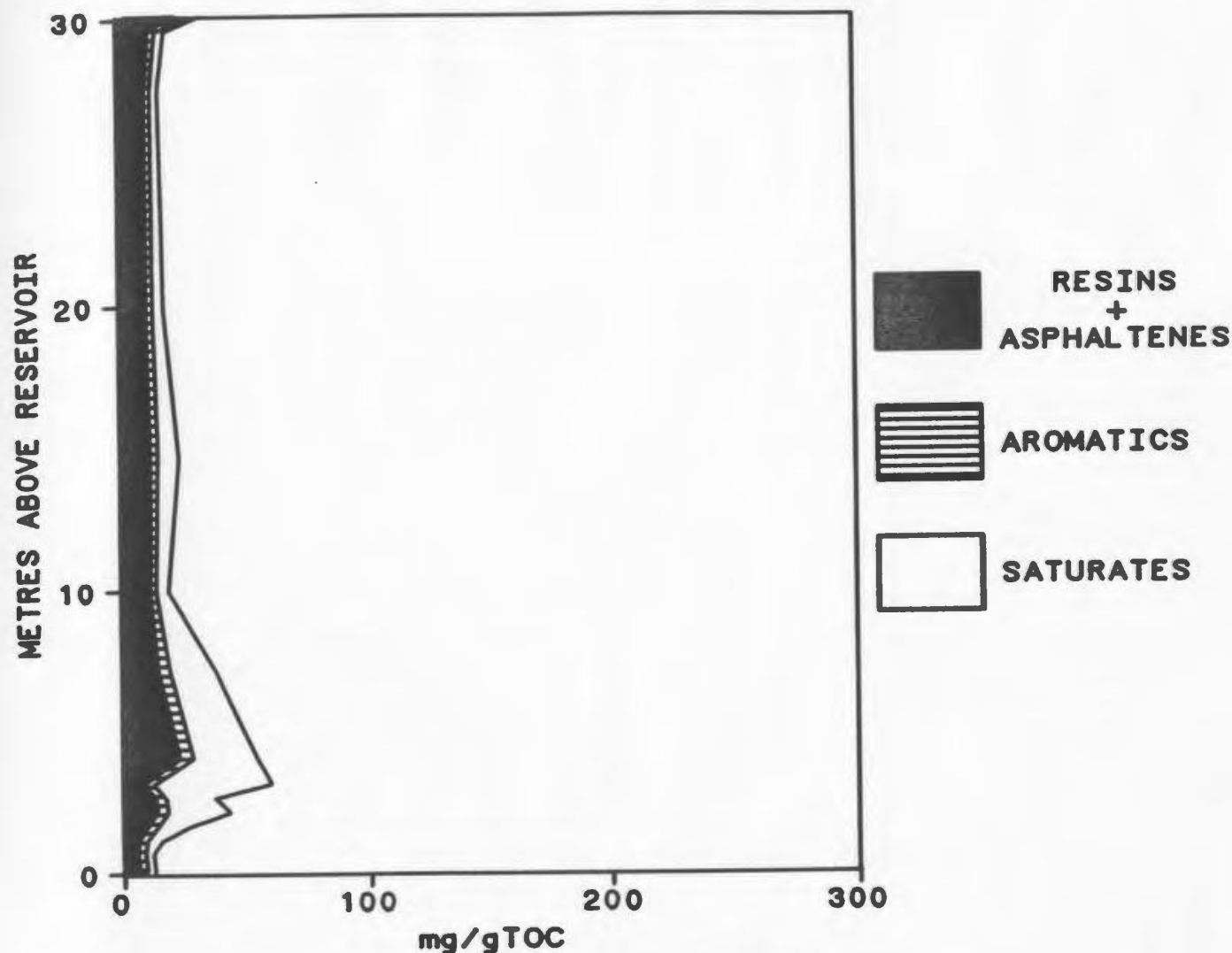
Figure 2-7: Carbon-normalized bitumen profile, U. Carboniferous, Germany (after Leythaeuser and Schaefer, 1984)
