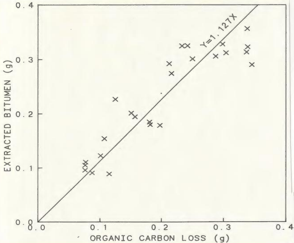
Figure 4-1: Bitumen wt. vs. carbon loss
