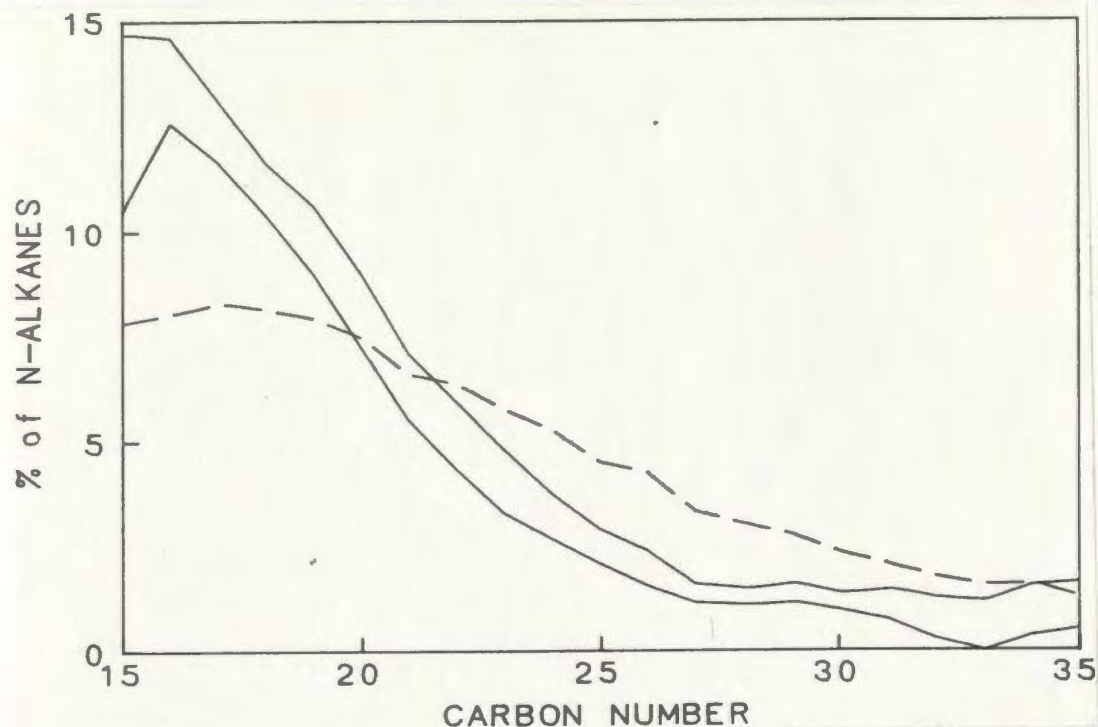
Figure 5-5: Composite n-alkane envelope - contaminated bitumens (dashed line is reservoir oil)
