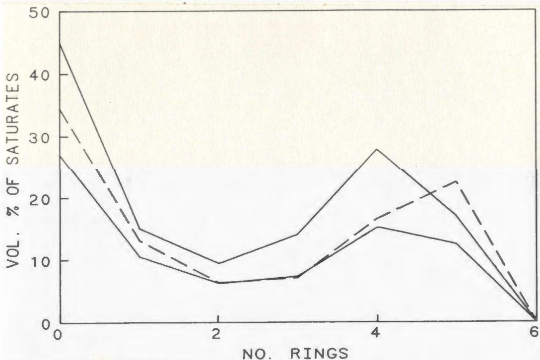
Figure 5-17: Composite saturate envelope: unaltered bitumens (dashed line is reservoir oil)
