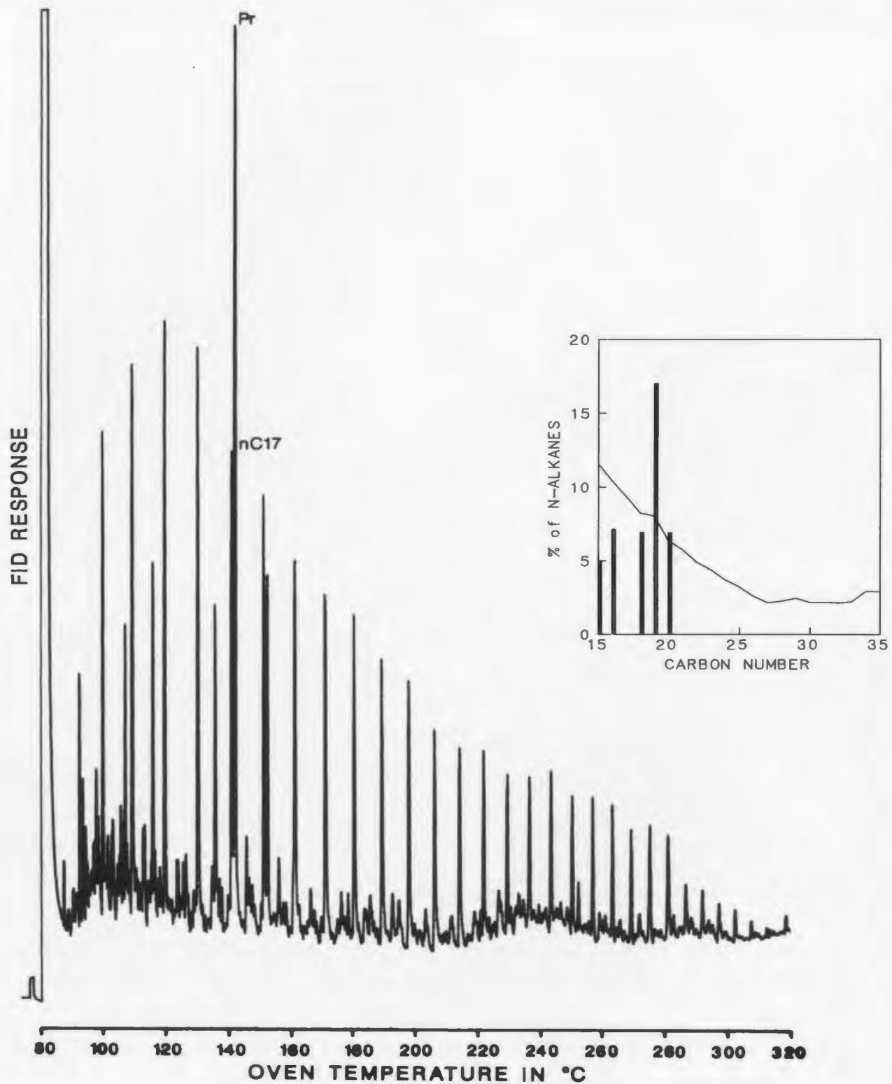
Figure C-11: Saturates, 37.7m
