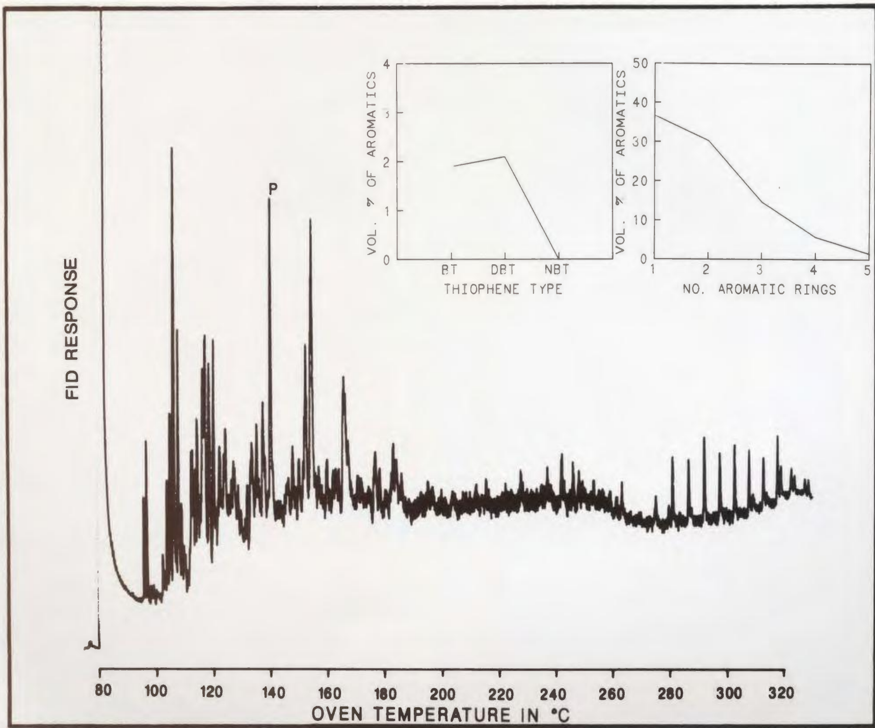
Figure C-45: Aromatics, 17.9m
