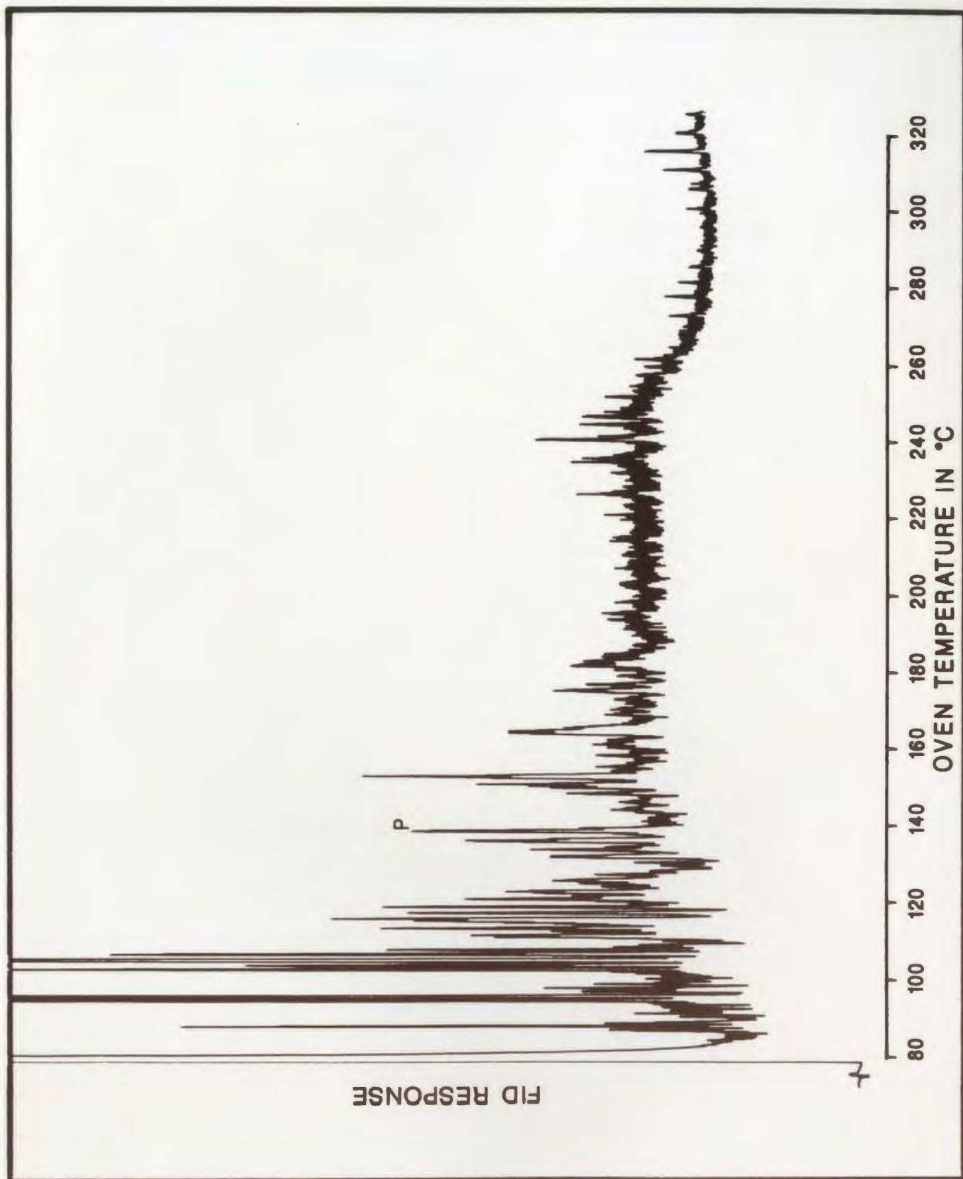
Figure C-31: Aromatics, 85.9m
