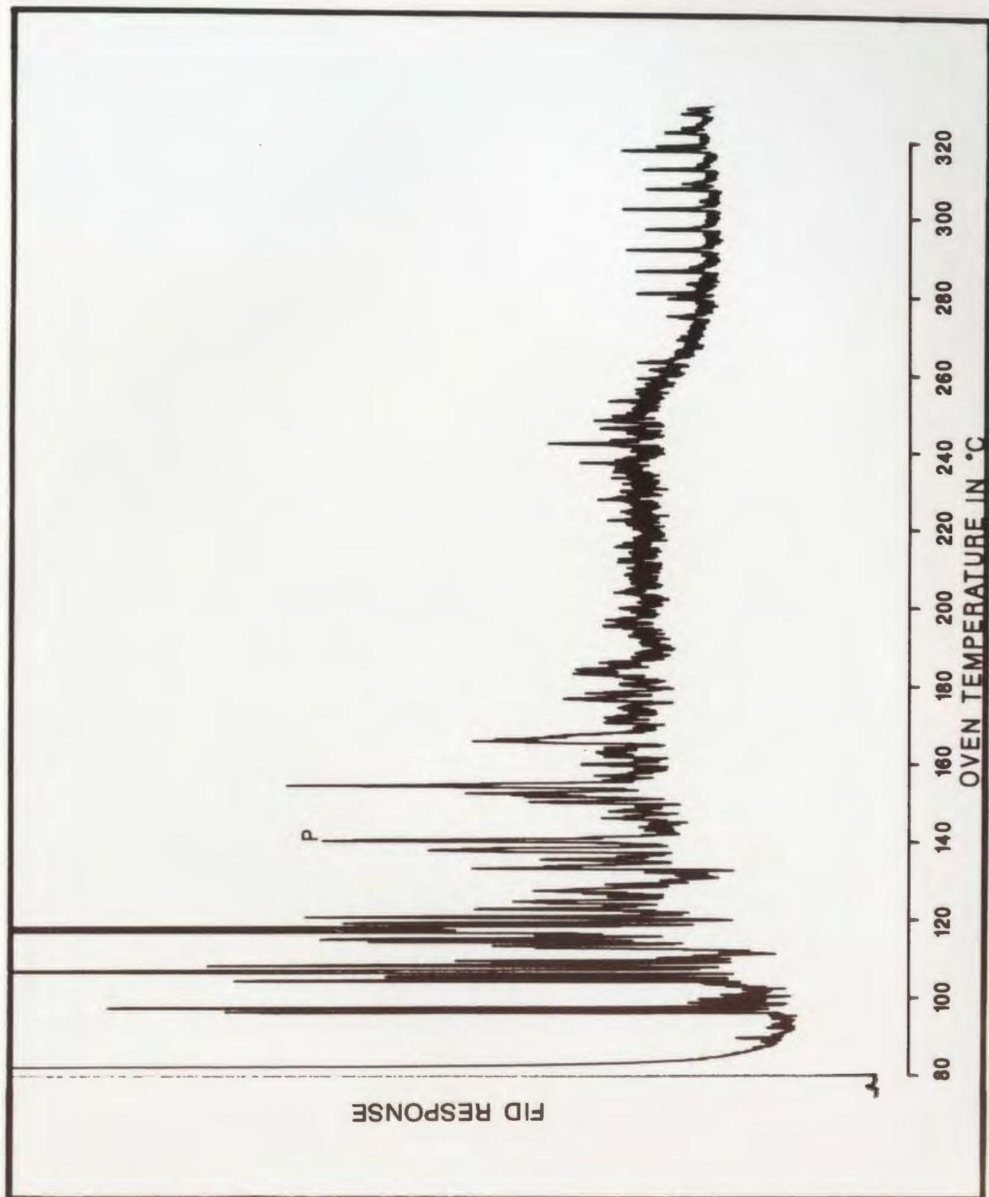
Figure C-37: Aromatics, 48.5m
