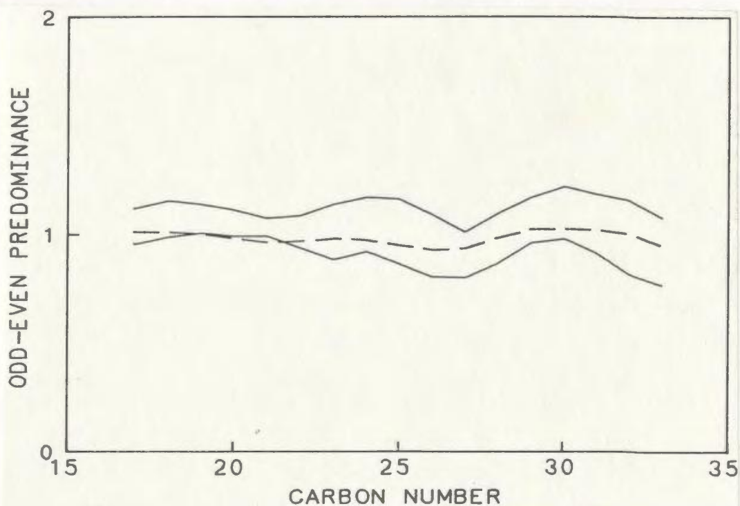
Figure 5-19: Composite OEP envelope: all unaltered bitumens (dashed line is reservoir oil)
