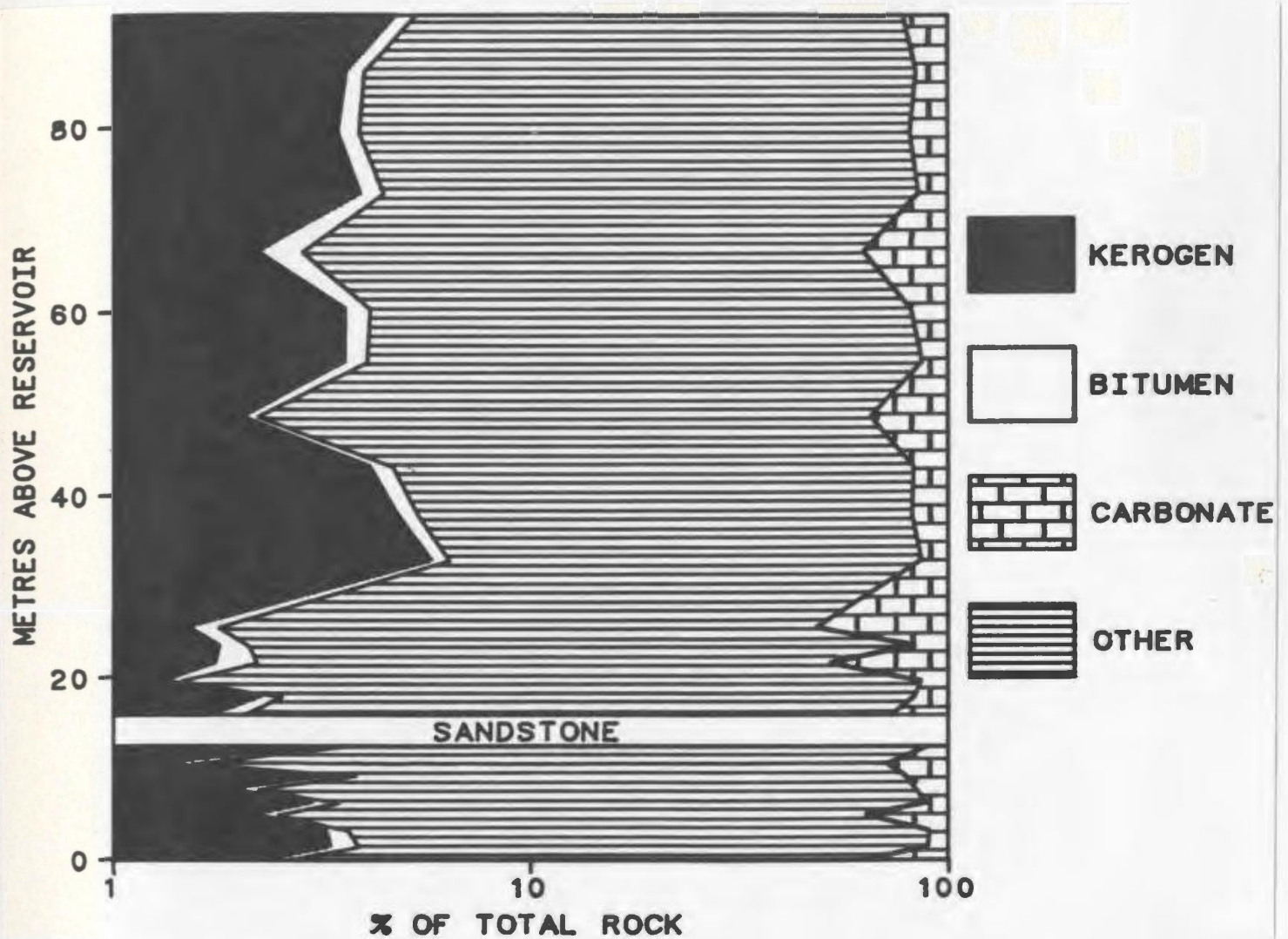
Figure 4-3: Lithological breakdown of section
