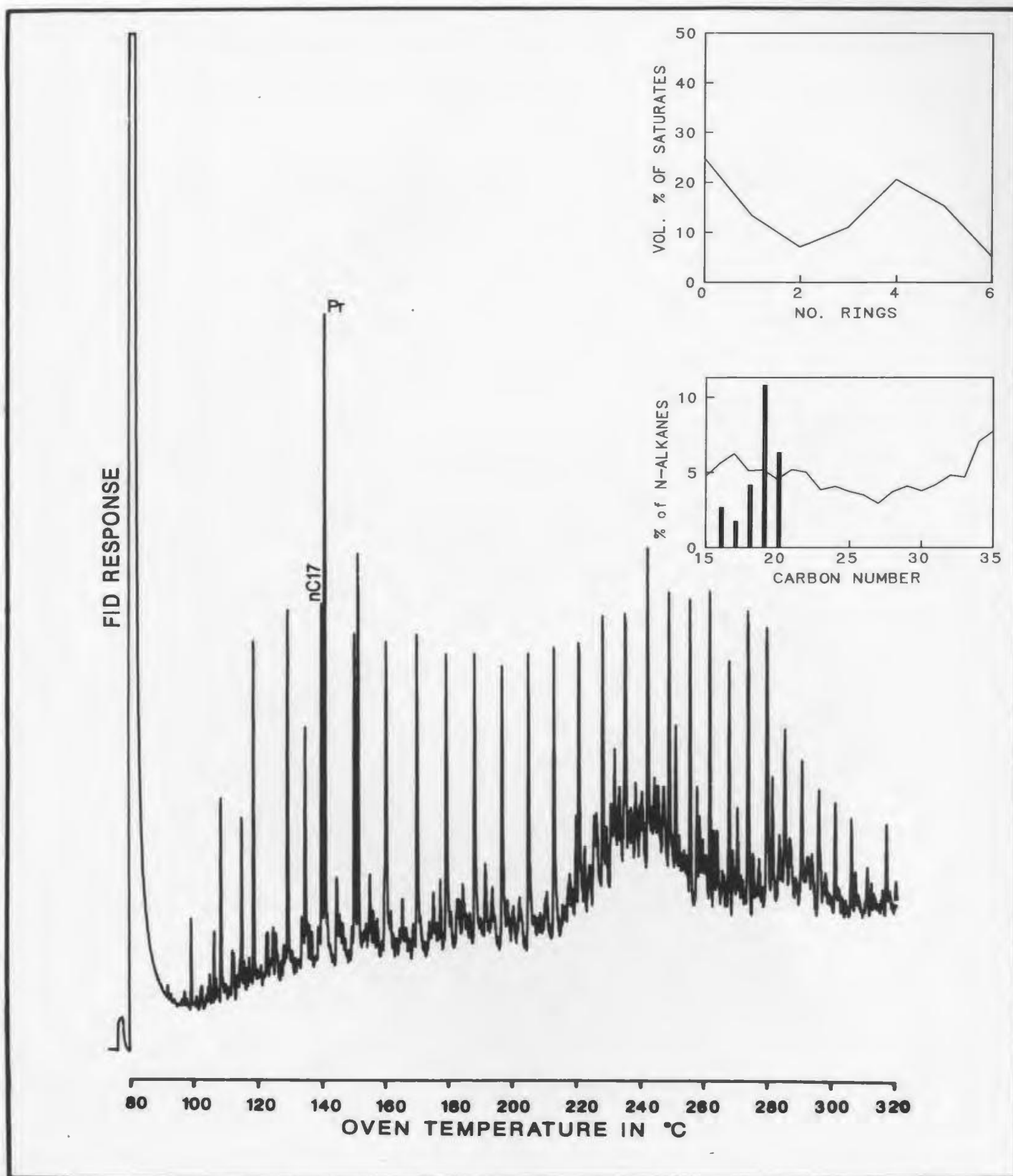
Figure C-19: Saturates, 12.4m
