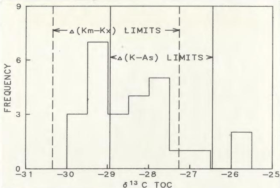
Figure 6-6: Isotopic oil-source correlation
