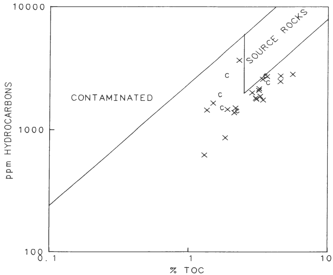
Figure 7-1: ppm Hydrocarbons vs. TOC (with cutoff)
