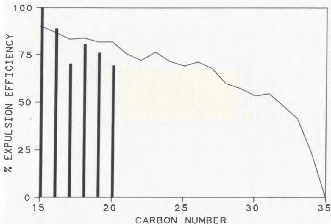
Figure 5-22: N-alkane expulsion efficiencies, 12.4m (solid bars = isoprenoids)
