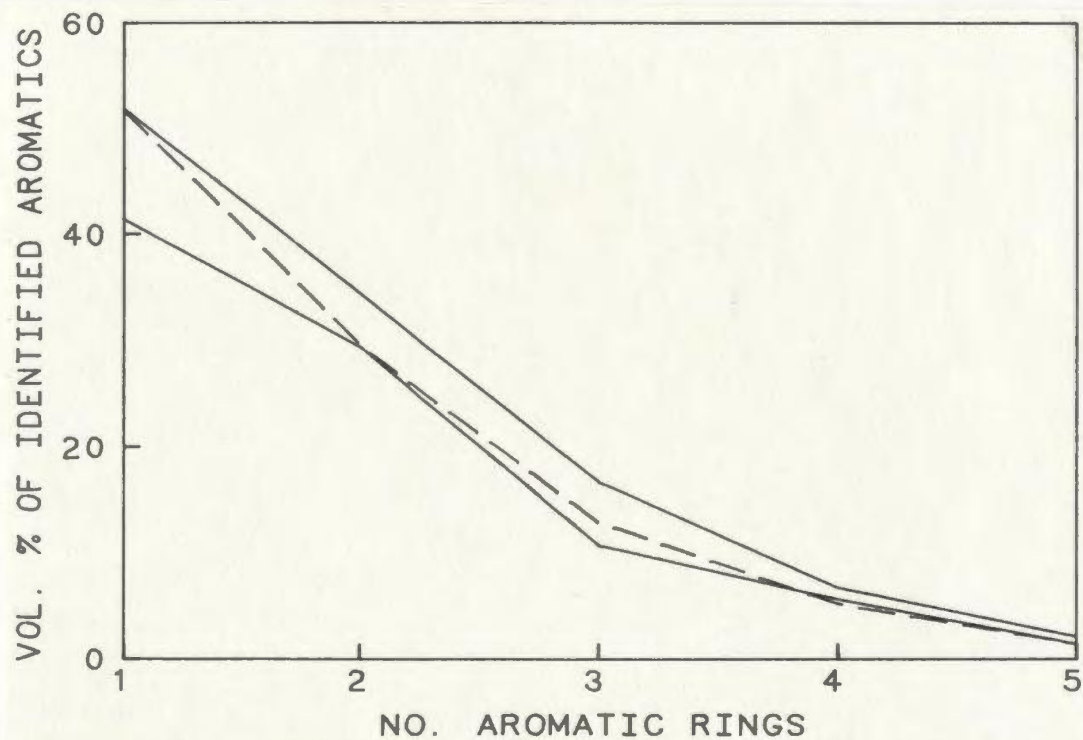
Figure 5-16: Composite aromatic envelope: unaltered bitumens (dashed line is reservoir oil)
