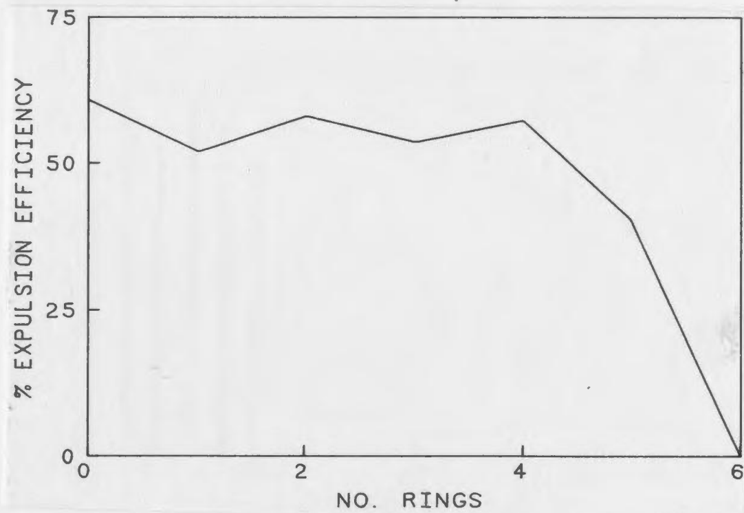
Figure 5-28: Expulsion efficiencies, saturates fraction, 12.4m
