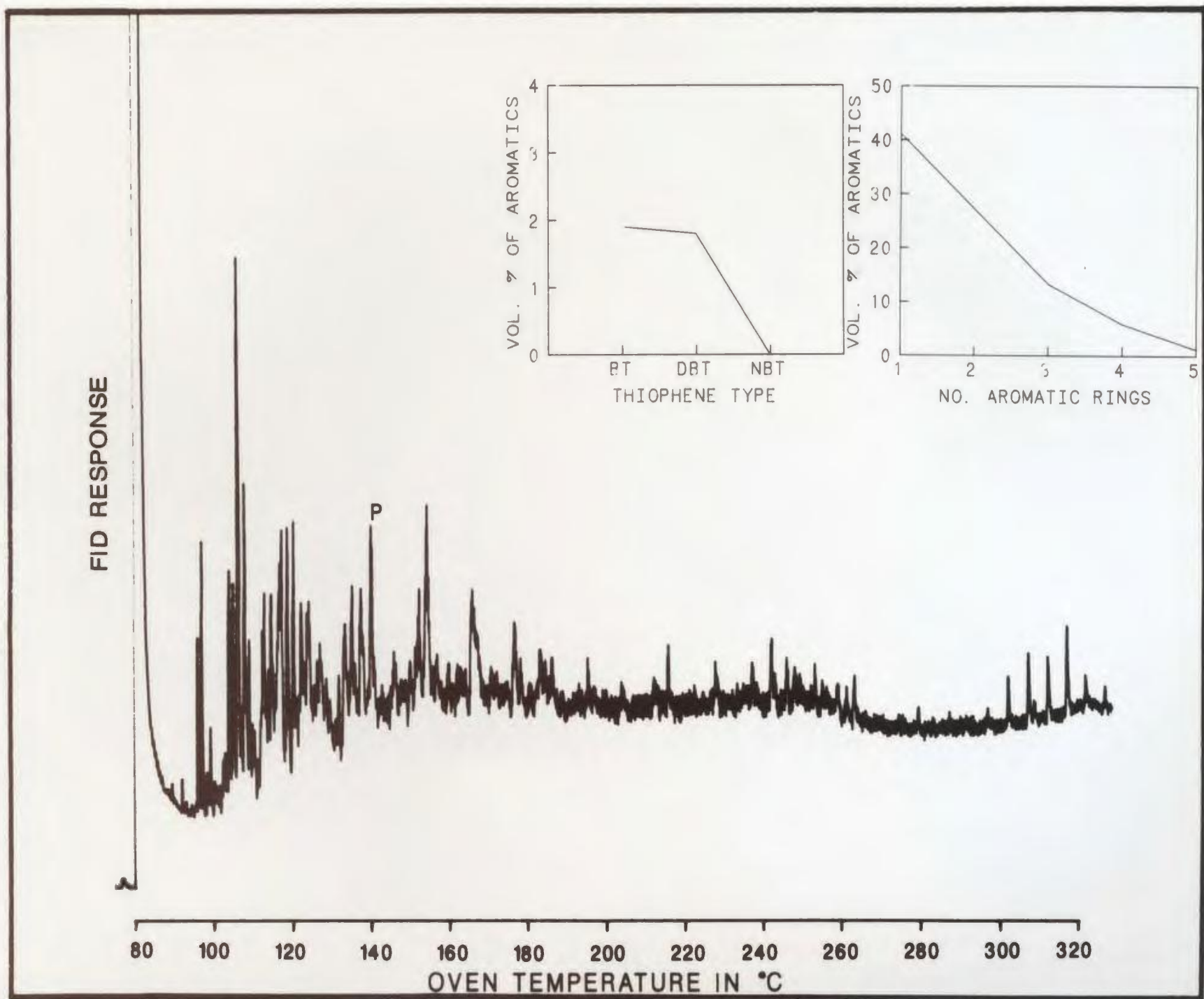
Figure C-41: Aromatics, 25.5m
