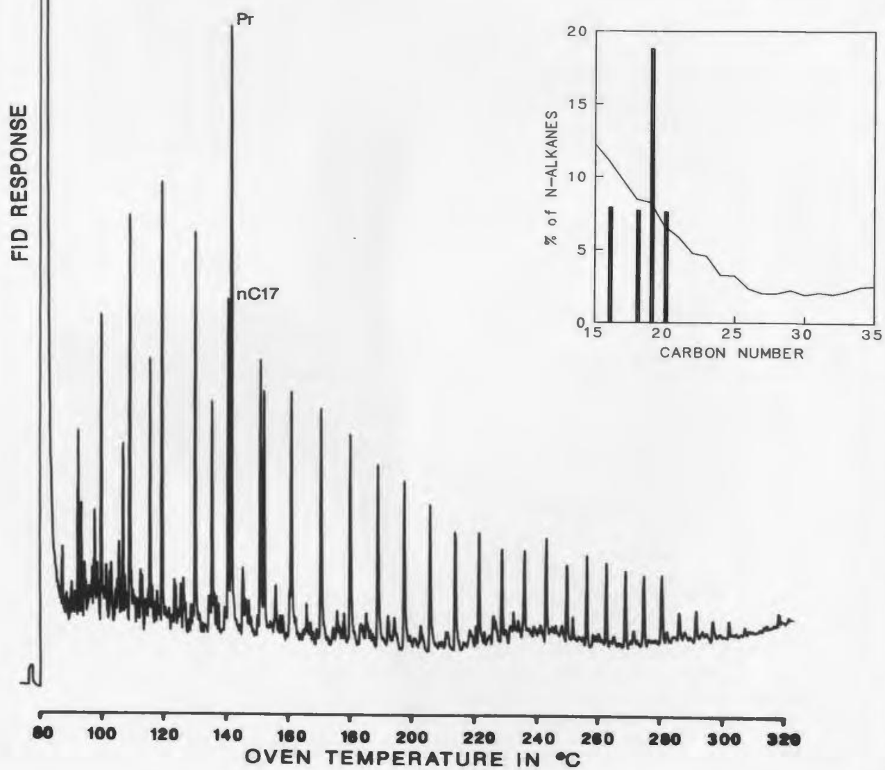
Figure C-2: Saturates, 92.0m
