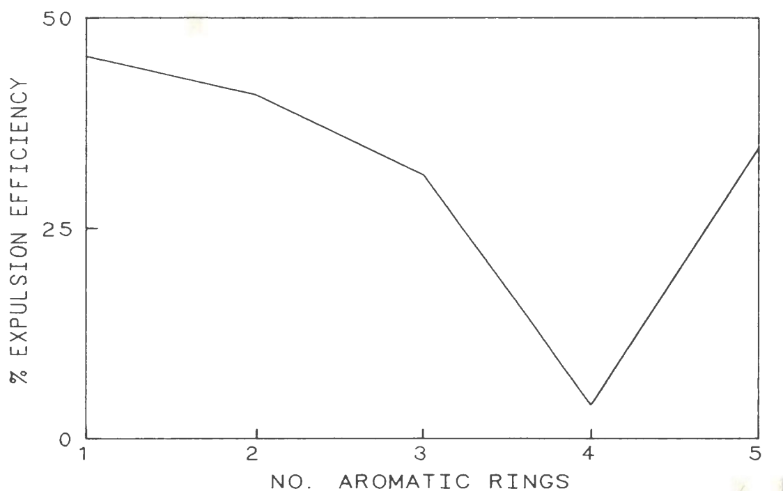
Figure 5-25: Expulsion efficiencies, aromatics fraction, 12.4m
