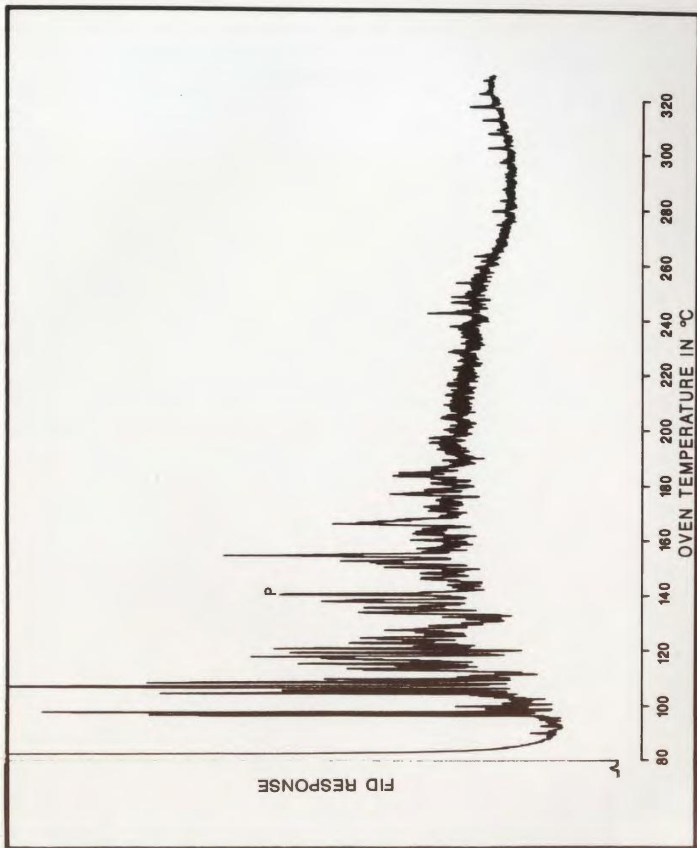
Figure C-40: Aromatics, 32.8m
