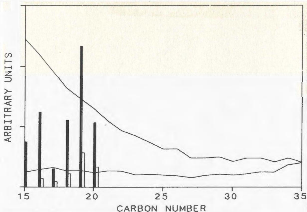
Figure 5-21: nC_{35} -normalized alkane distributions 10.5m is upper line and solid bars(isoprenoids)
