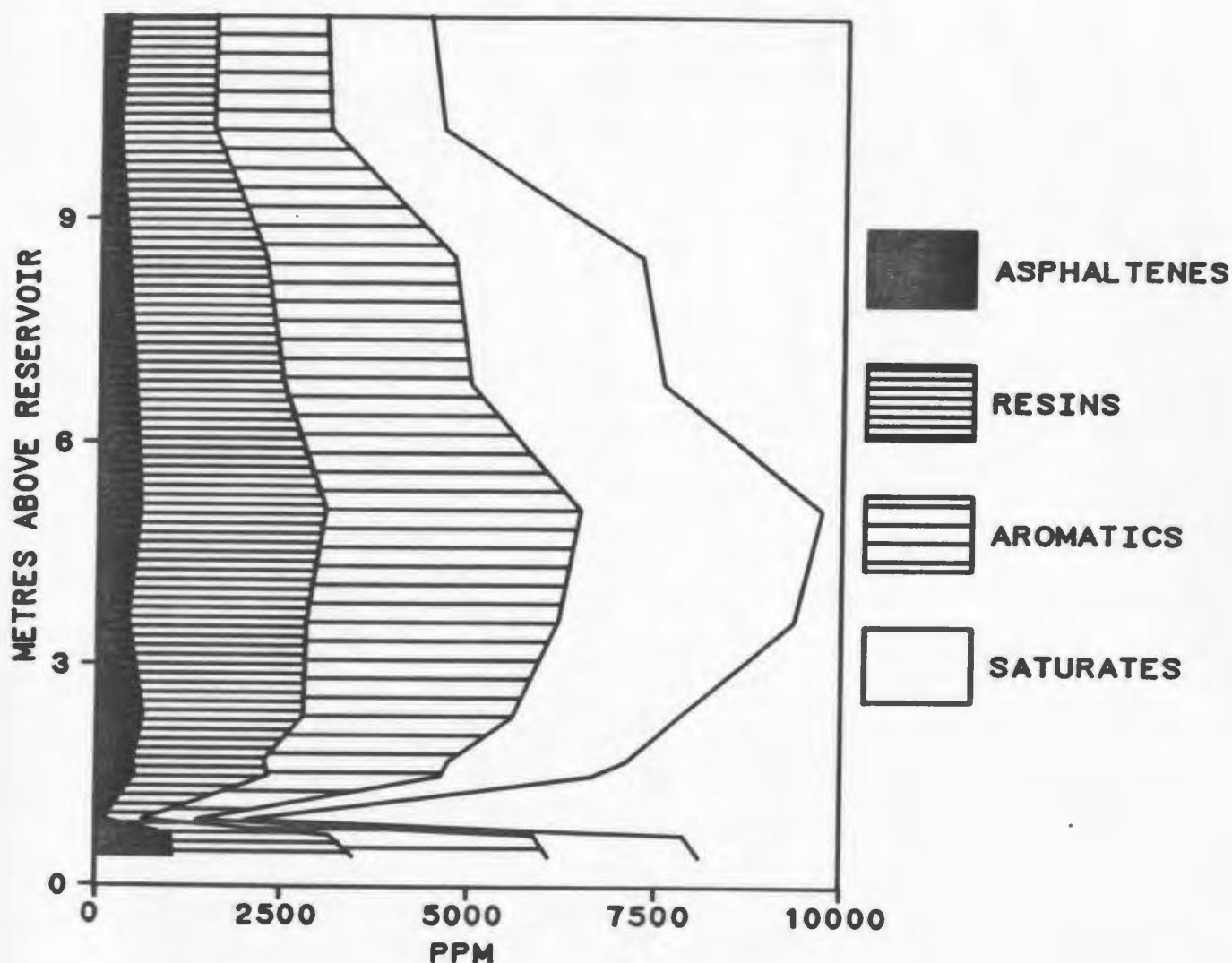
Figure 2-5: Bitumen profile, L. Jurassic, France
