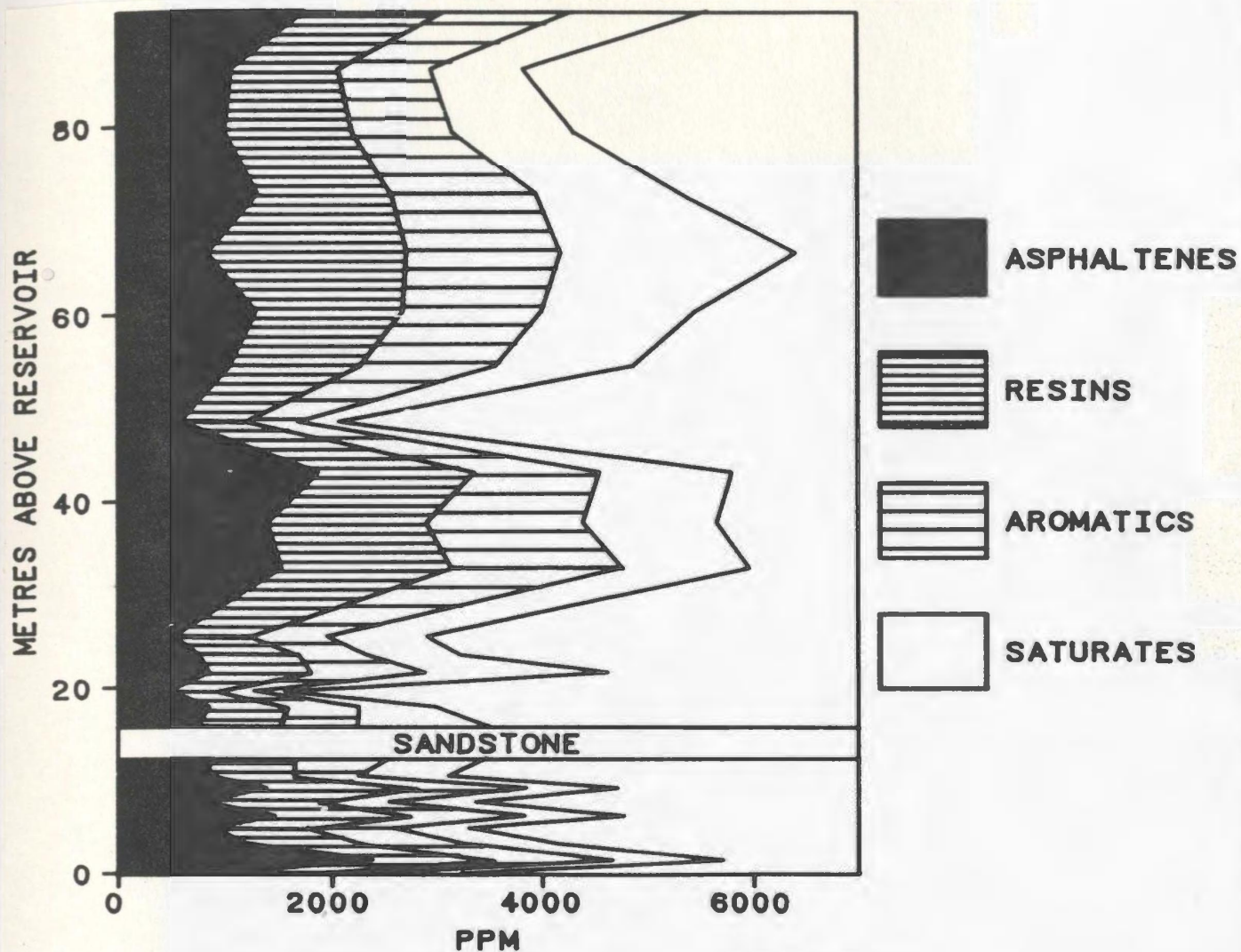
Figure 5-1: Rock-normalized bitumen profile
