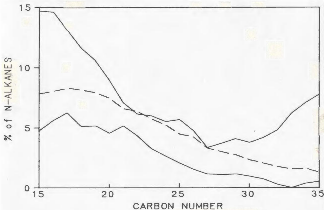
Figure 5-3: Composite n-alkane envelope - all bitumens (dashed line is reservoir oil)
