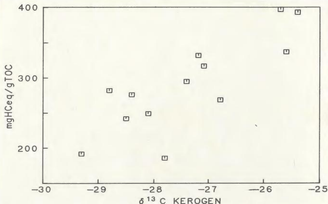
Figure 6-2: HI vs \delta^{13}\text{C} kerogen
