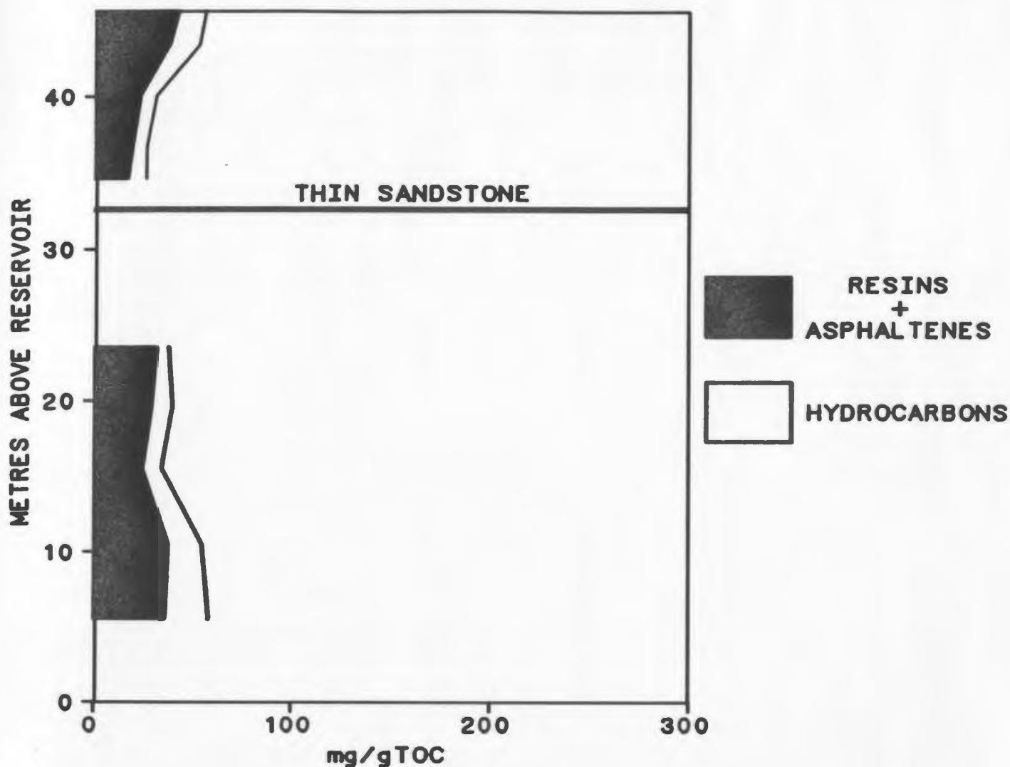
Figure 2-6: Carbon-normalized bitumen profile, Paleocene, Spitzbergen (after Leythaeuser et al. 1983)
