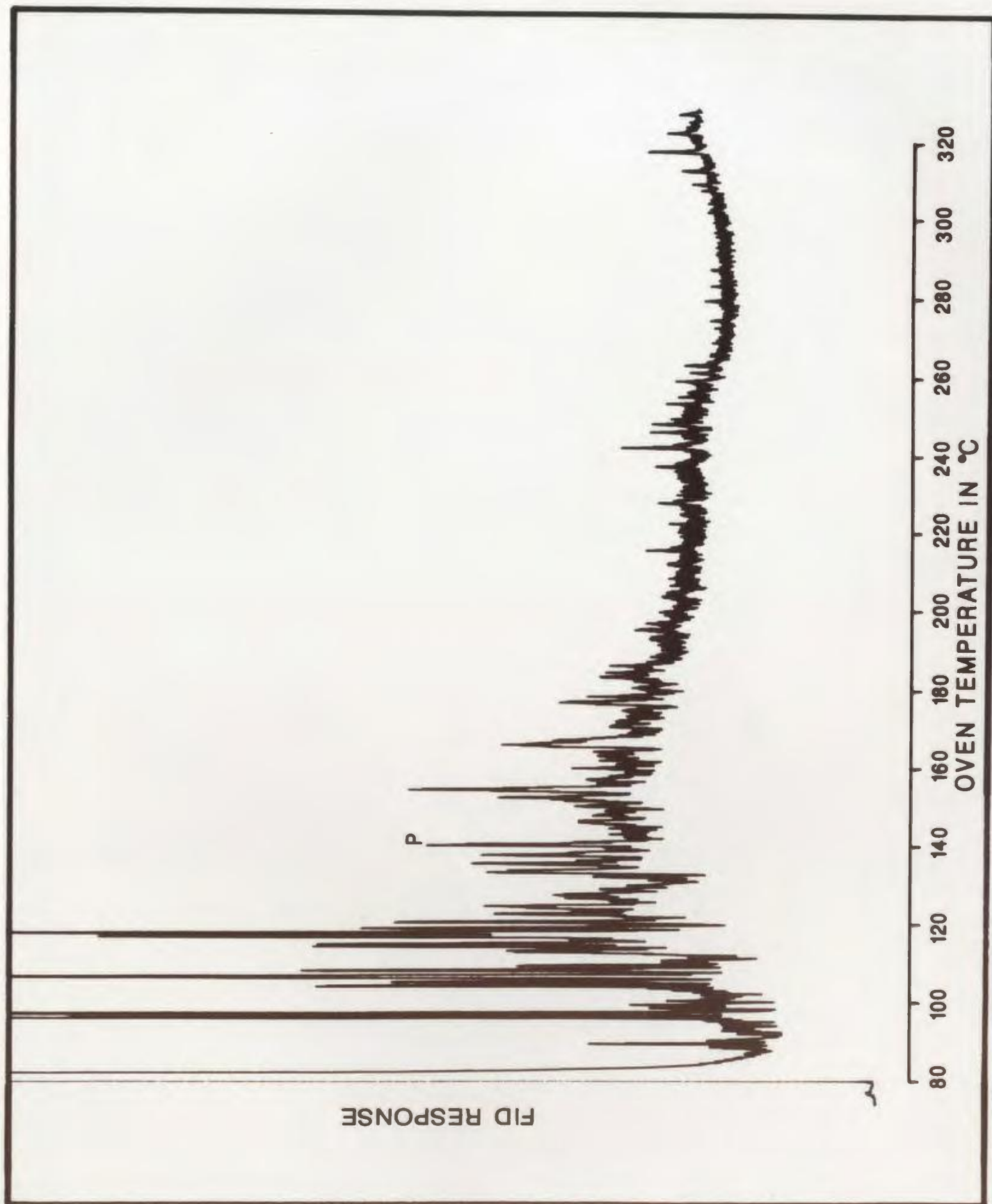
Figure C-35: Aromatics, 60.2m
