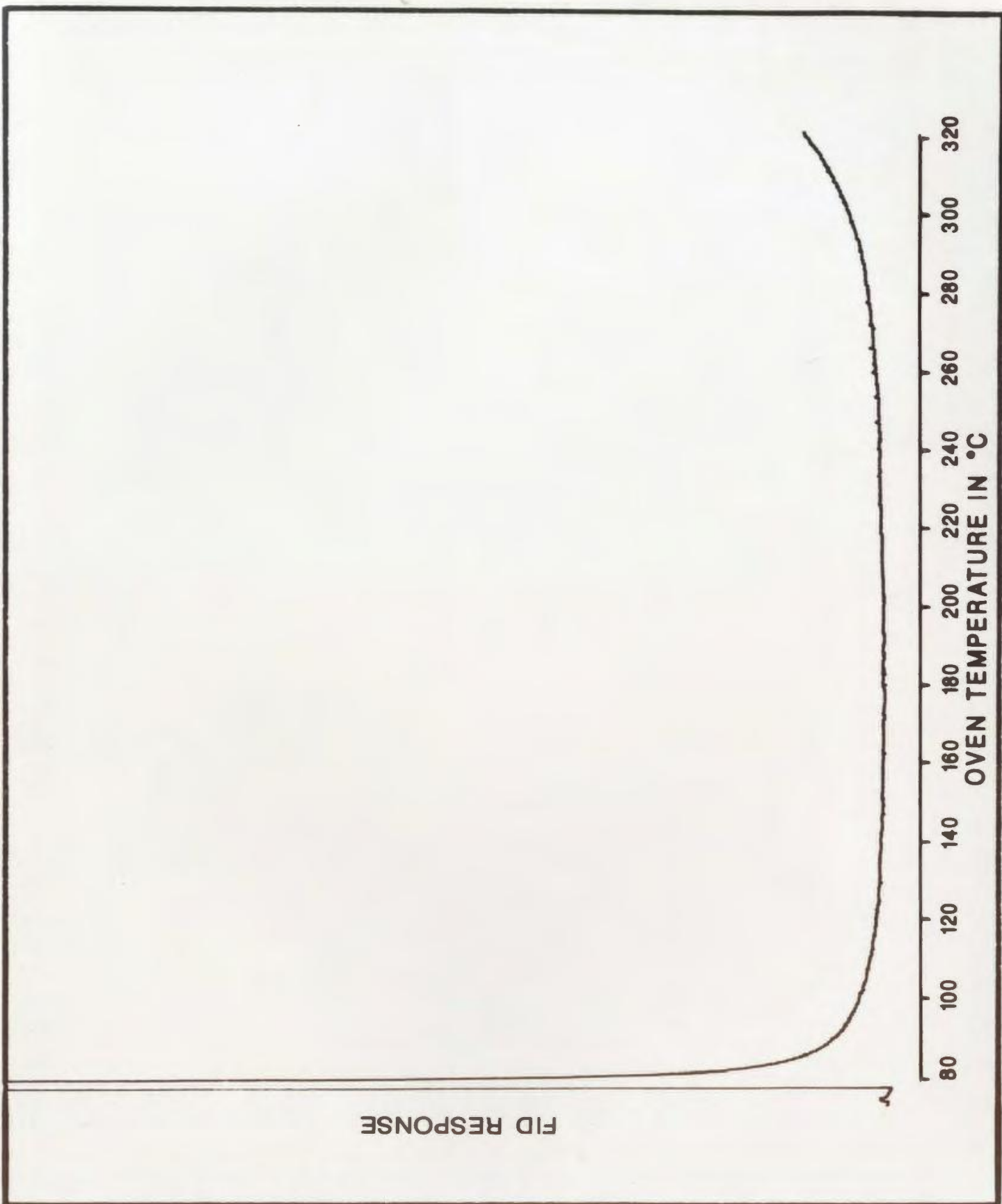
Figure C-29: Aromatics, blank
