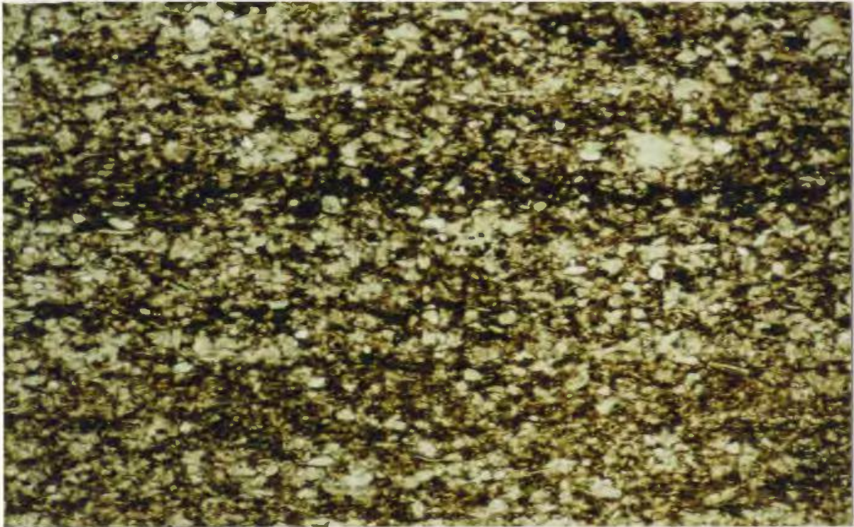
Figure 4-5: Laminated siltstone, 43.1m (x30)
