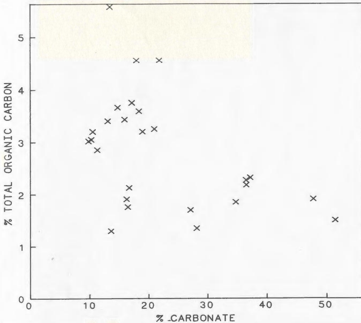
Figure 4-2: TOC vs. CO 3
