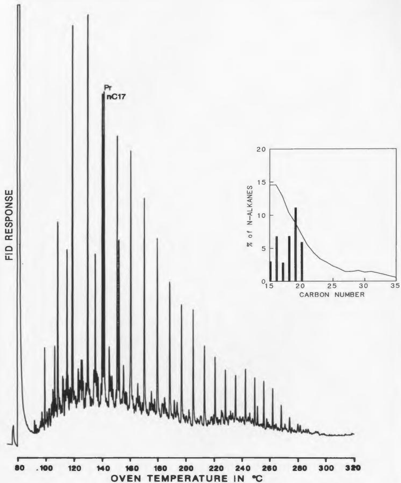
Figure C-14: Saturates, 23.5m
