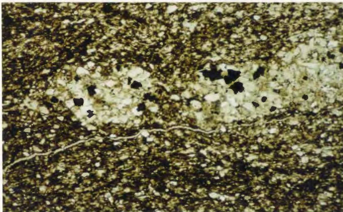
Figure 4-7: Siltstone with sandstone clasts, 7.7m (x30)
