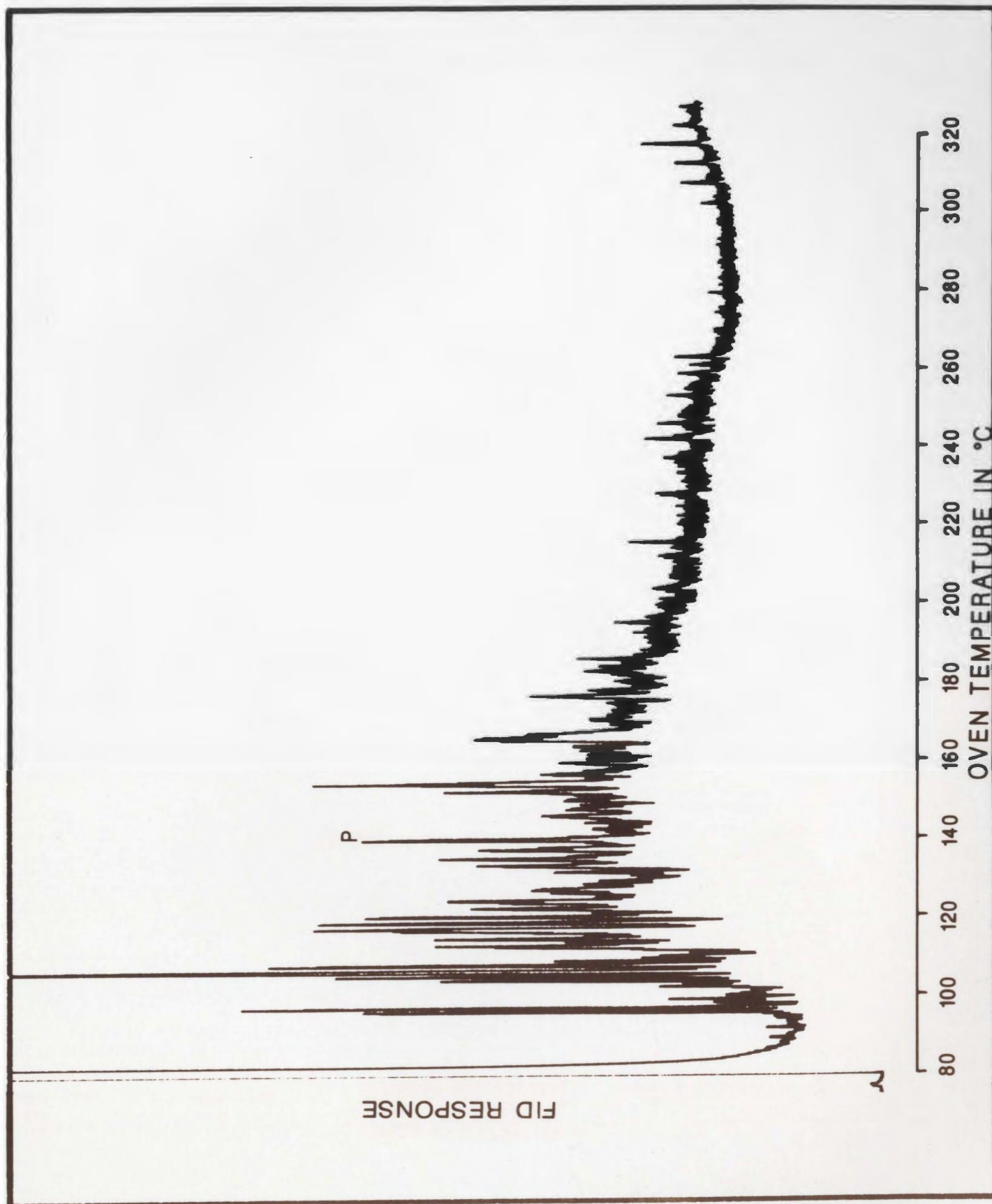
Figure C-43: Aromatics, 21.6m
