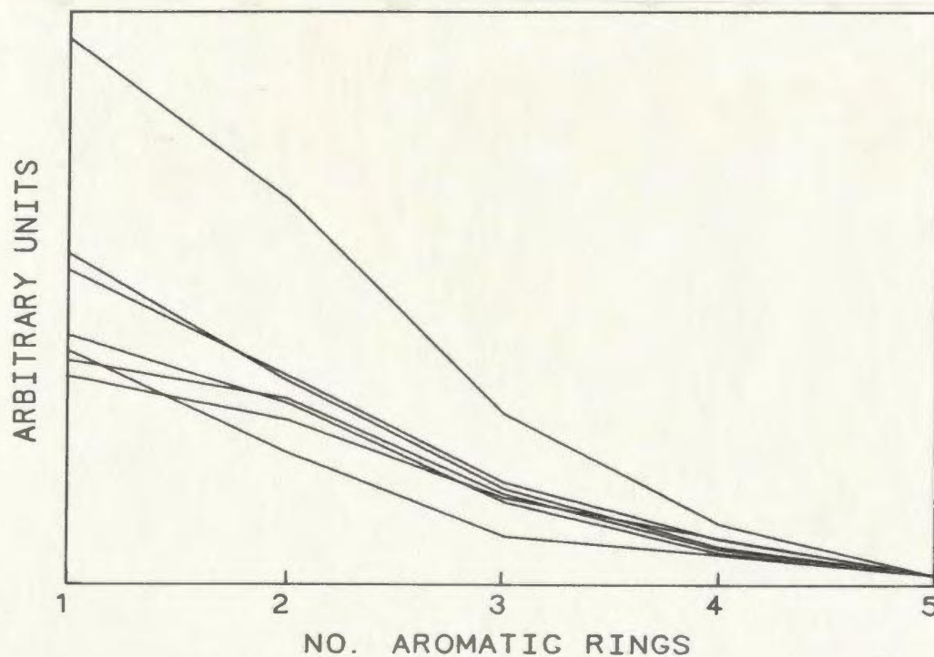
Figure 5-6: Pentaaromatic-normalized aromatic distributions
