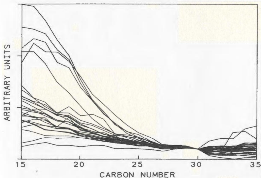
Figure 5-4: nC_{30} -normalized n-alkane distributions
