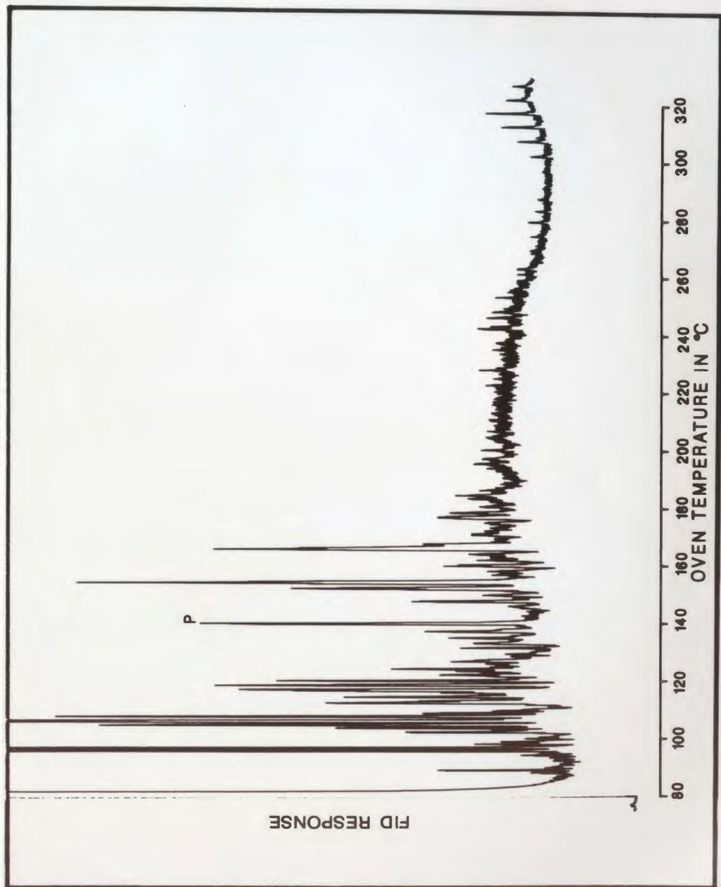
Figure C-54: Aromatics, 1.4m
