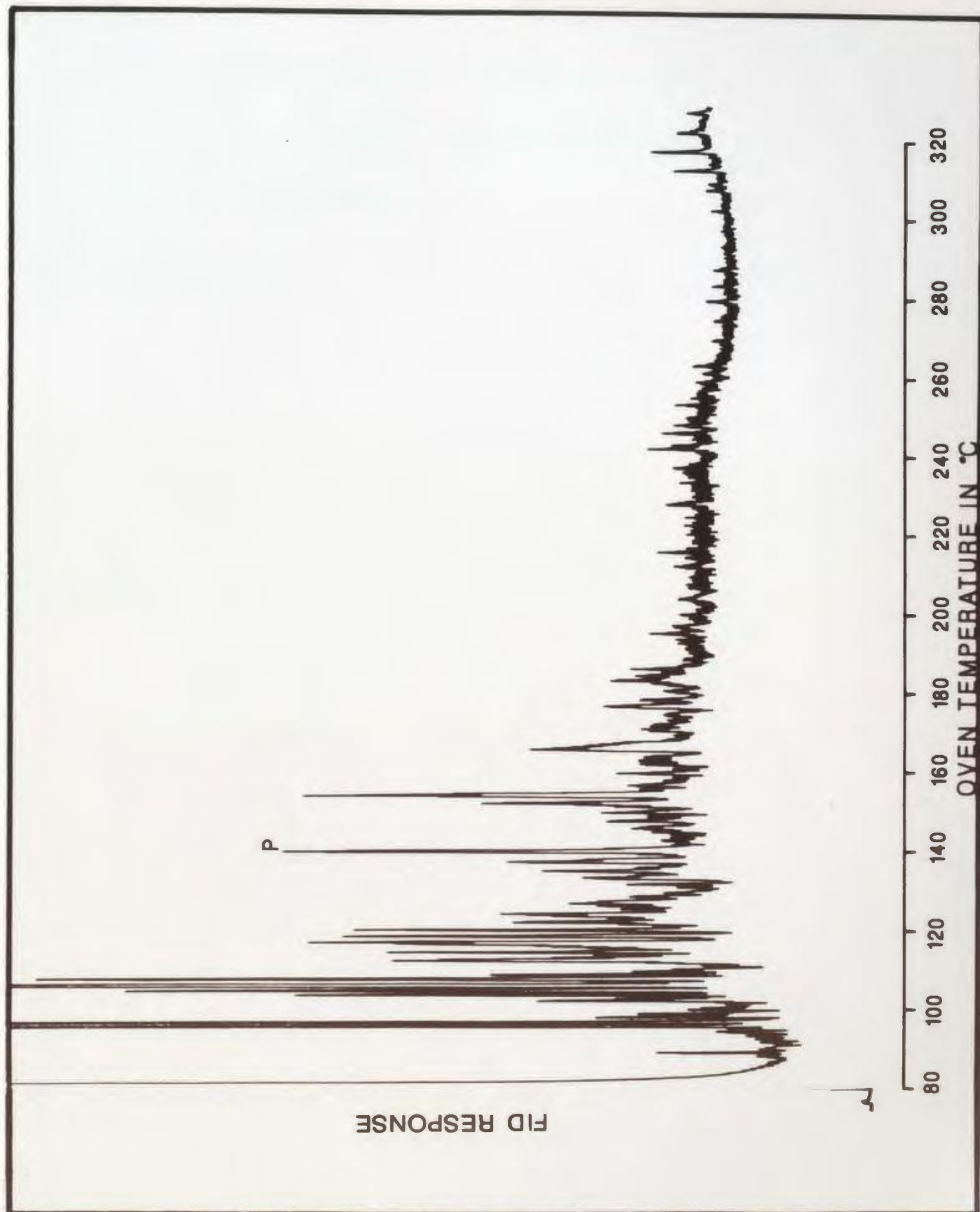
Figure C-50: Aromatics, 7.7m
