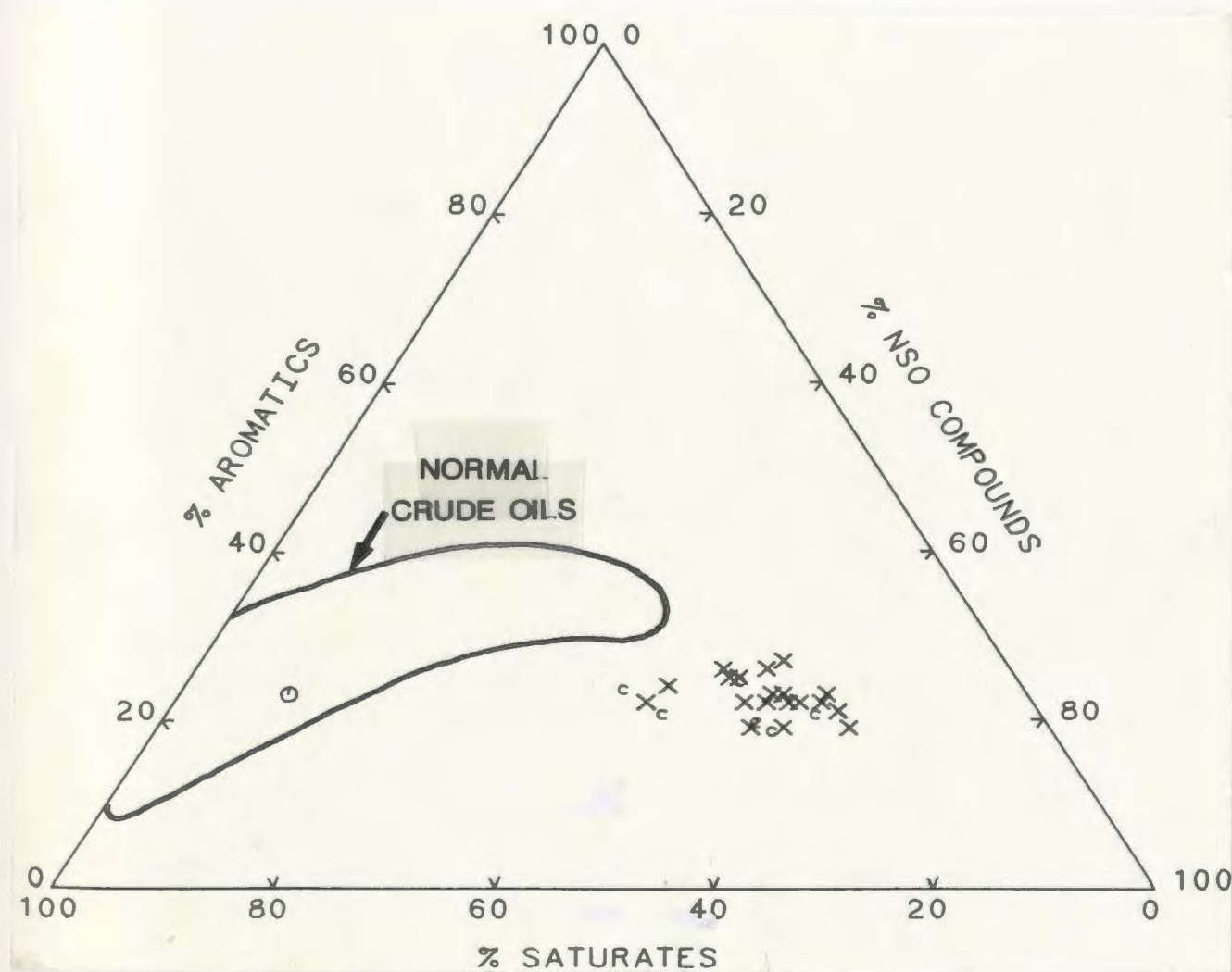
Figure 5-9: Bitumen composition by compound type
