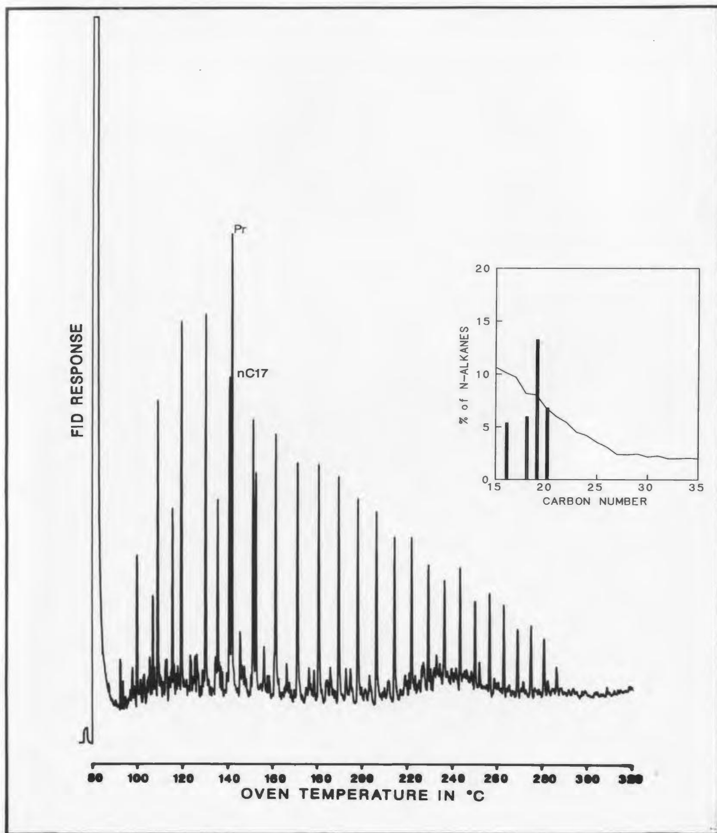
Figure C-4: Saturates, 79.3m
