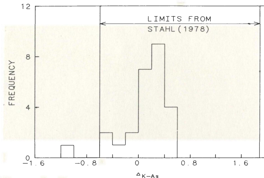
Figure 6-8: Isotopic bitumen-source correlation (using Km-As)
