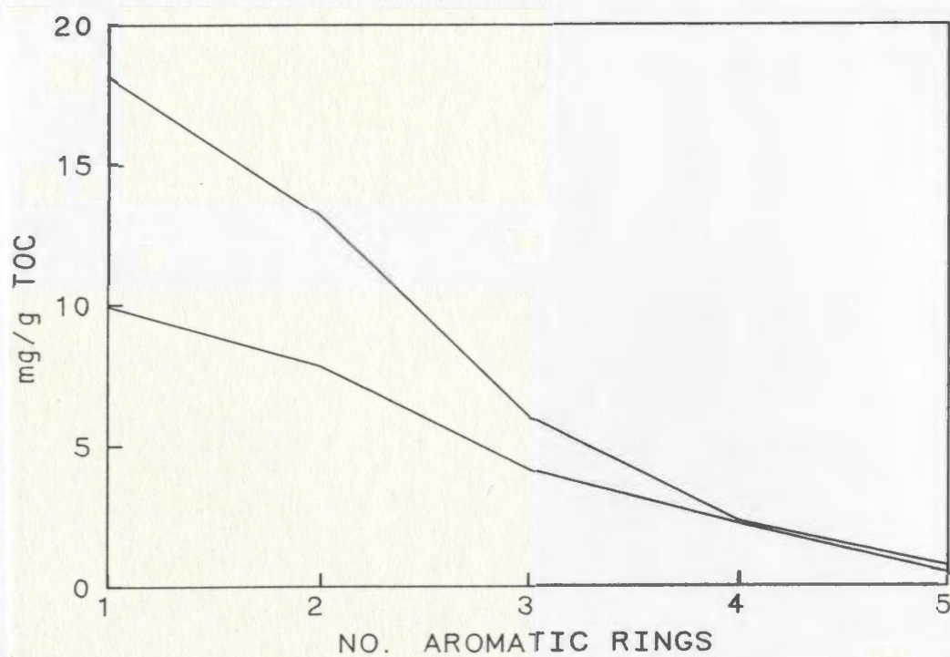
Figure 5-24: Carbon-normalized aromatics distributions (upper curve = 10.5m)
