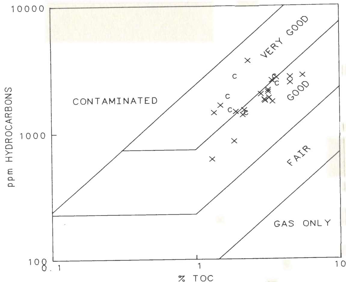
Figure 5-11: ppm Hydrocarbons vs. TOC
