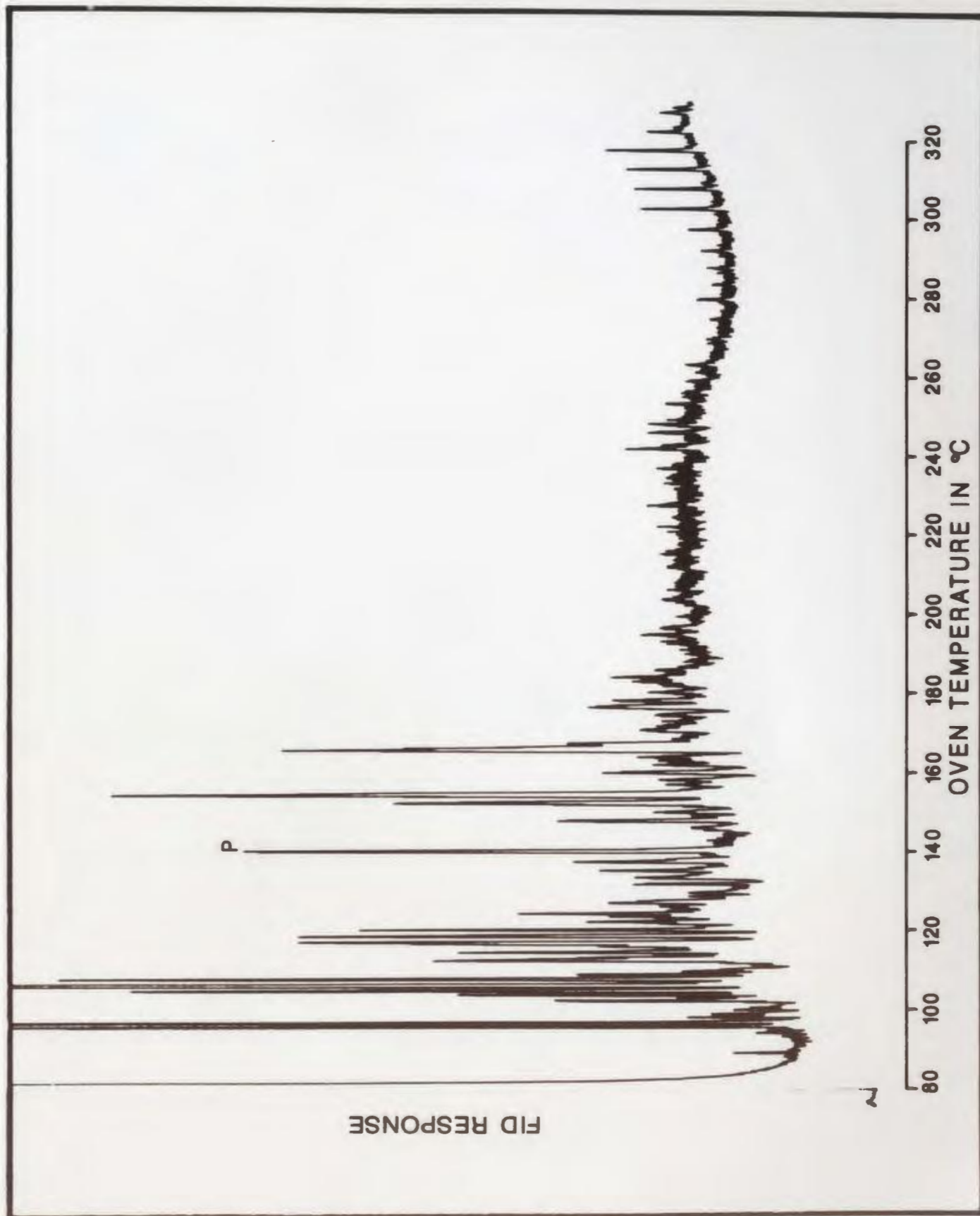
Figure C-53: Aromatics, 3.2m
