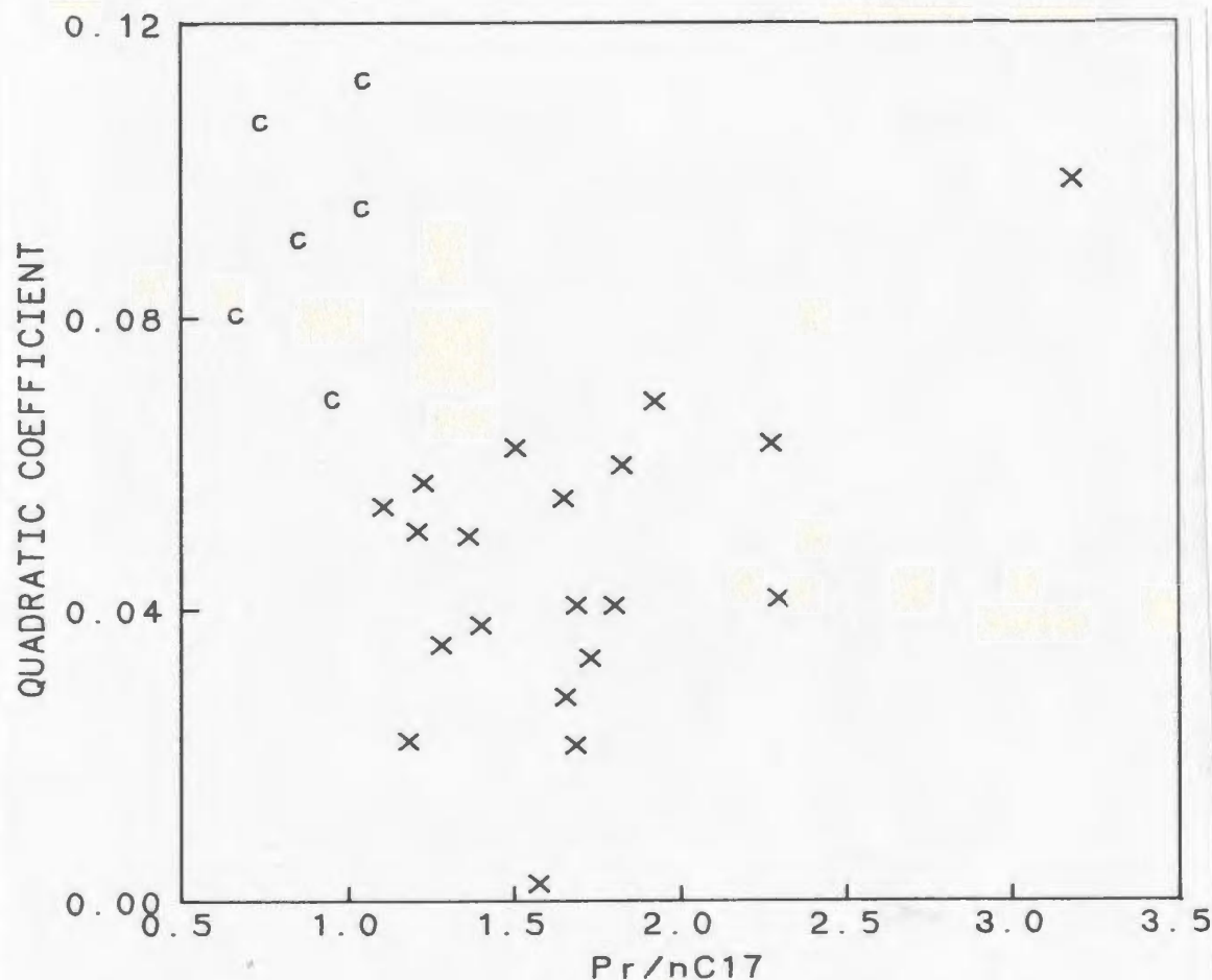
Figure 5-7: QC vs. \text{Pr}/\text{nC}_{17}
