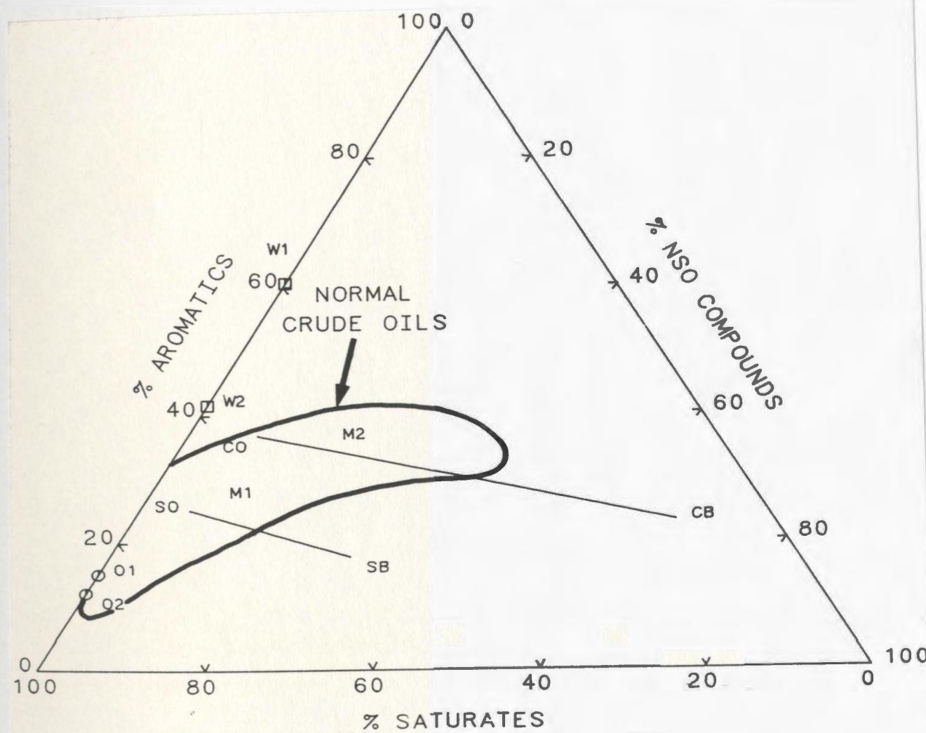
Figure 1-1: Composition of crude oils and bitumens
