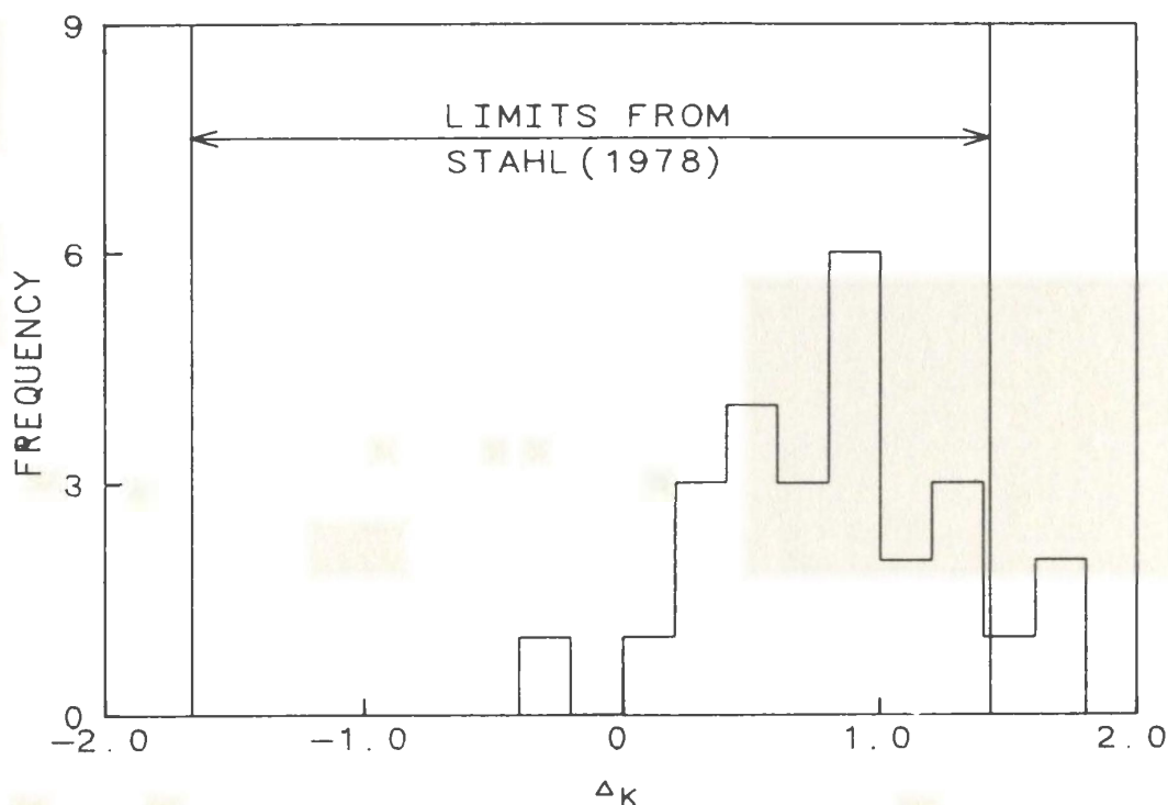
Figure 6-7: Isotopic bitumen-source correlation (using Km-Kx)
