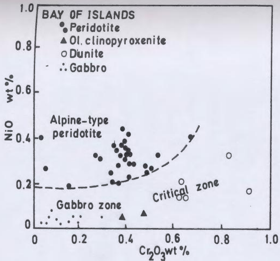
FIGURE 8: Plots showing the relative abundances of NiO and Cr 2 O 3 in peridotites from Bay of Islands (alpine-type, after Irving et al., 1972) and Baie Verte. Dashed line is used by Irving et al. to separate alpine-type peridotite from rocks of the Critical and Gabbro Zones.
