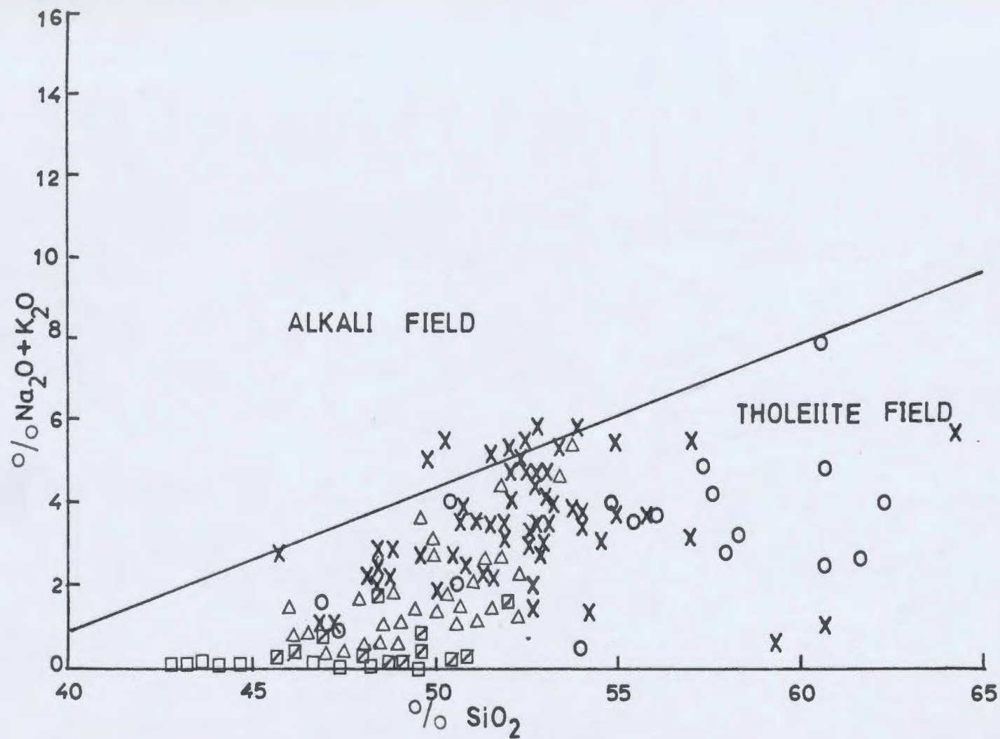
FIGURE 5: Total alkalis vs. \text{SiO}_2 variation diagram. Line separates the alkaline and tholeiitic series of the Hawaiian volcanic rocks (Macdonald and Katsura, 1964). \circ - pillow lavas; \times - sheeted dikes; \Delta - gabbro; \square - pyroxenite; \square - peridotite.
