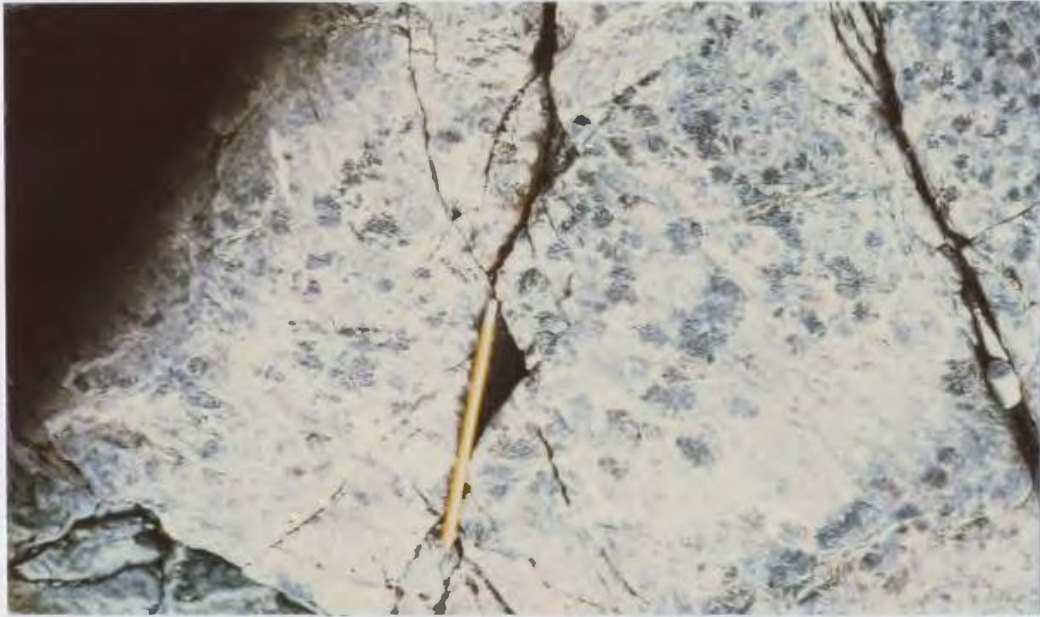
Fig. a: Poikilitic actinolite crystals in peridotite.
