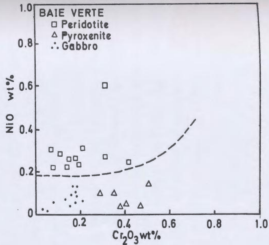
FIGURE 8: Plots showing the relative abundances of NiO and Cr 2 O 3 in peridotites from Bay of Islands (alpine-type, after Irving et al., 1972) and Baie Verte. Dashed line is used by Irving et al. to separate alpine-type peridotite from rocks of the Critical and Gabbro Zones.
