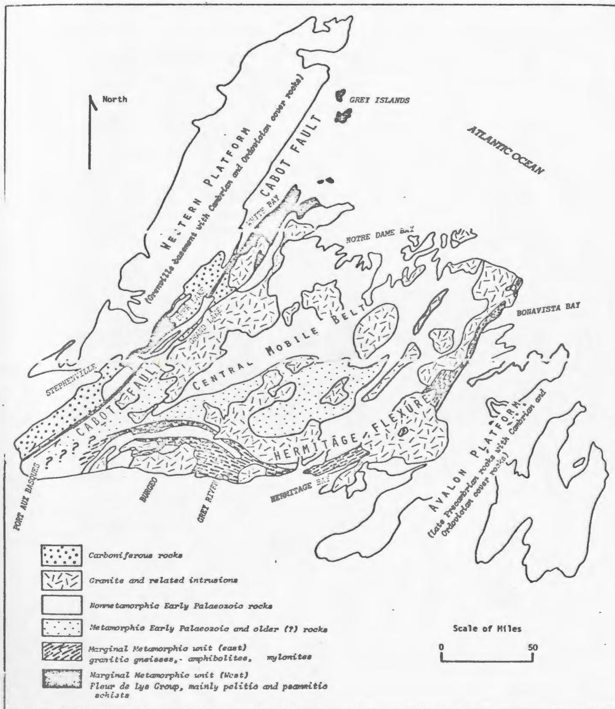
Figure 1-1. General geology and major structural subdivisions of the Newfoundland Central Mobile Belt. (AFTER Williams et al, 1970)
