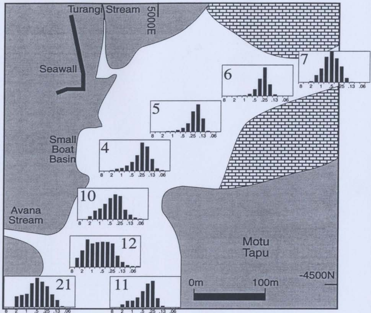
Figure 5.3 Grain-size distributions of selected samples from Ngatangia Harbour and the northern part of the channel. Grain size in millimetres.
