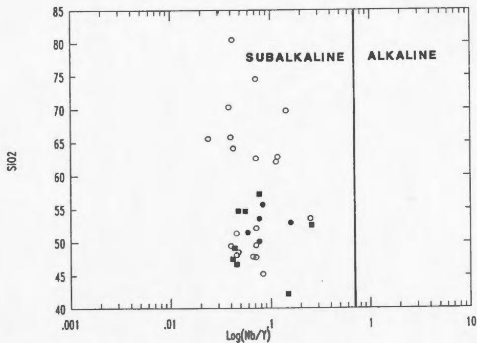
Figure 3.6. Nb/Y vs. SiO 2 diagram displaying the subalkaline and alkaline fields (adapted from Winchester and Floyd, 1977). The mafic to intermediate samples are subalkaline in character and variably silicified. Symbols as in Figure 3.1.
