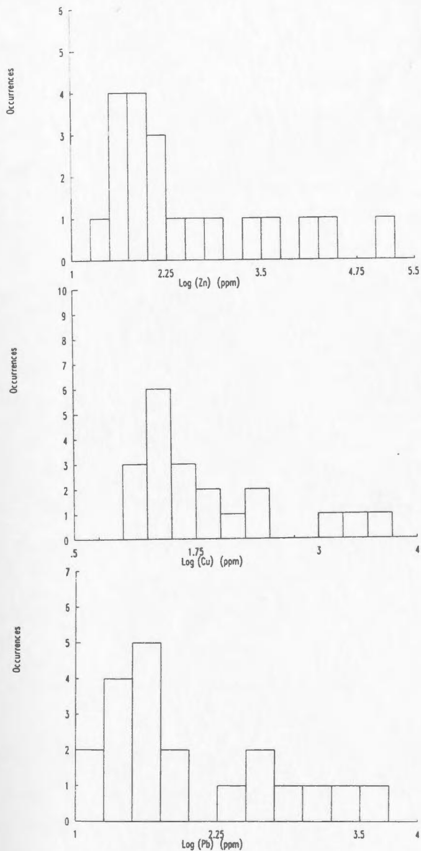
Figure 5.3. Histograms of Zn, Cu, and Pb for mineralized Tickle Point Fm. samples. Each histogram has a total of 20 samples.
