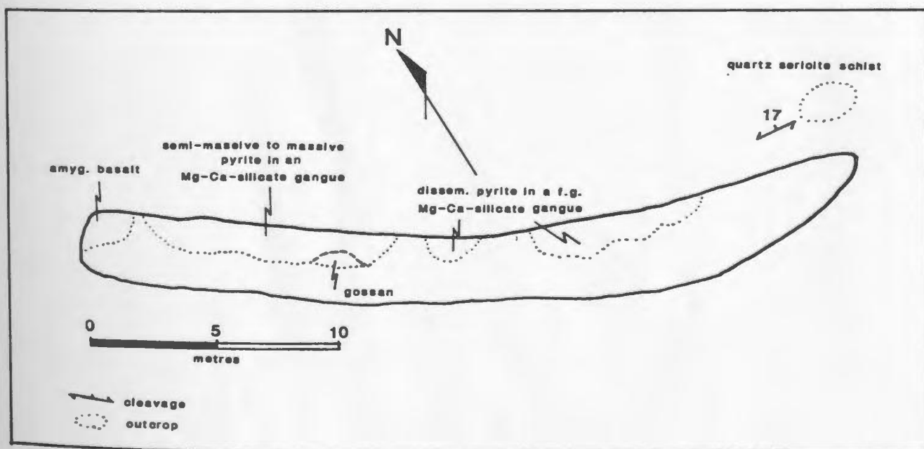
Figure 4.7. Trench geology at Winter Hill East.
