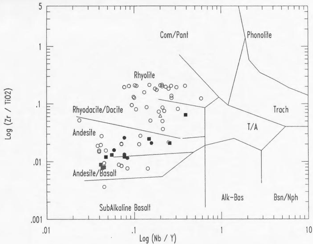
Figure 3.1. Nb/Y vs. Zr/Ti diagram from Winchester and Floyd (1977), with the 66 relatively unaltered volcanic rock samples plotted. Open circles = Tickle Pt. Fm., filled squares = Sam Head Fm., filled circles = Doughball Pt. Fm., and the open triangle = Down's Pt. Fm.
