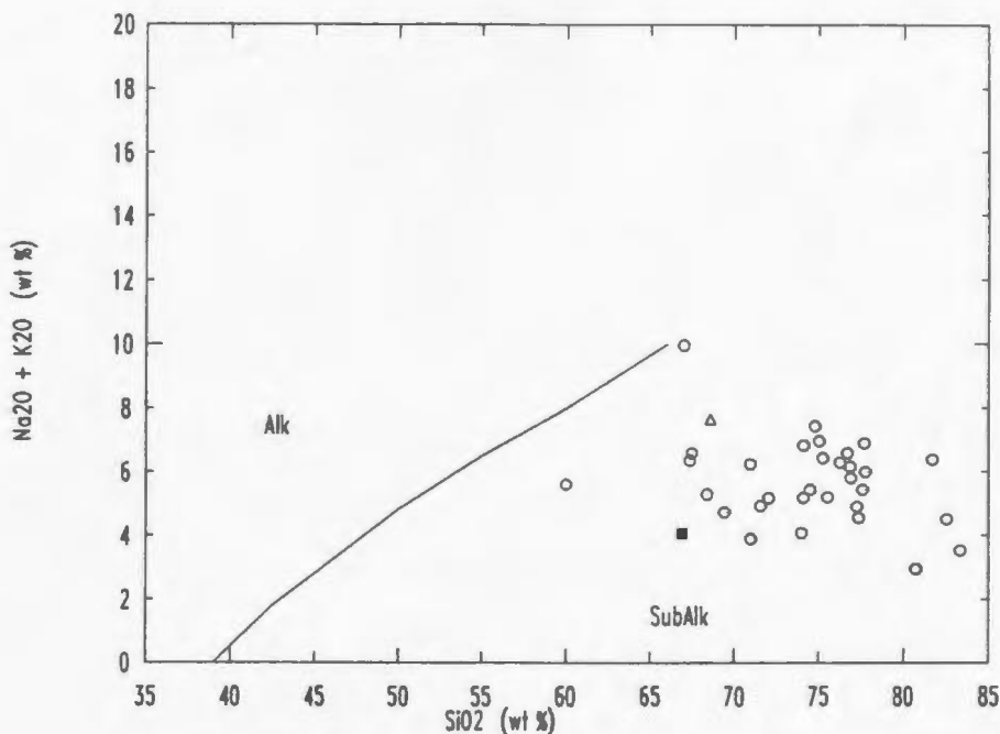
Figure 3.13. \text{SiO}_2 vs. alkalis diagram and the respective alkaline and subalkaline fields (taken from Irvine and Baragar, 1971). The dacitic to felsic rocks display a strong subalkaline character. Symbols as in Figure 3.1.
