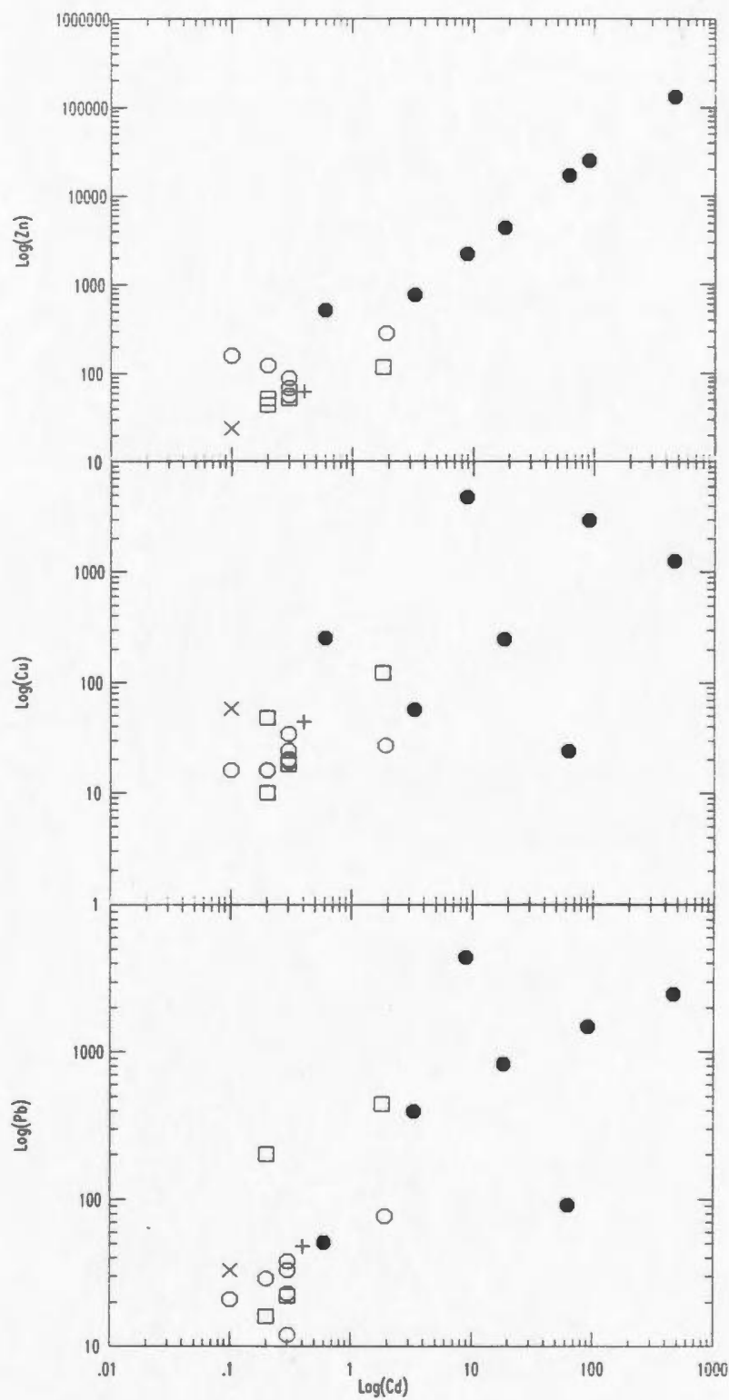
Figure 5.4. Variation diagram of Cd vs. the base-metals. Symbols as in Figure 5.1.
