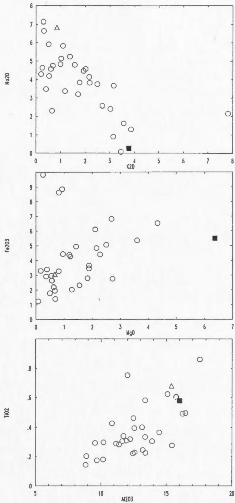
Figure 3.11. Major element variation plots. Symbols as in Figure 3.1.
