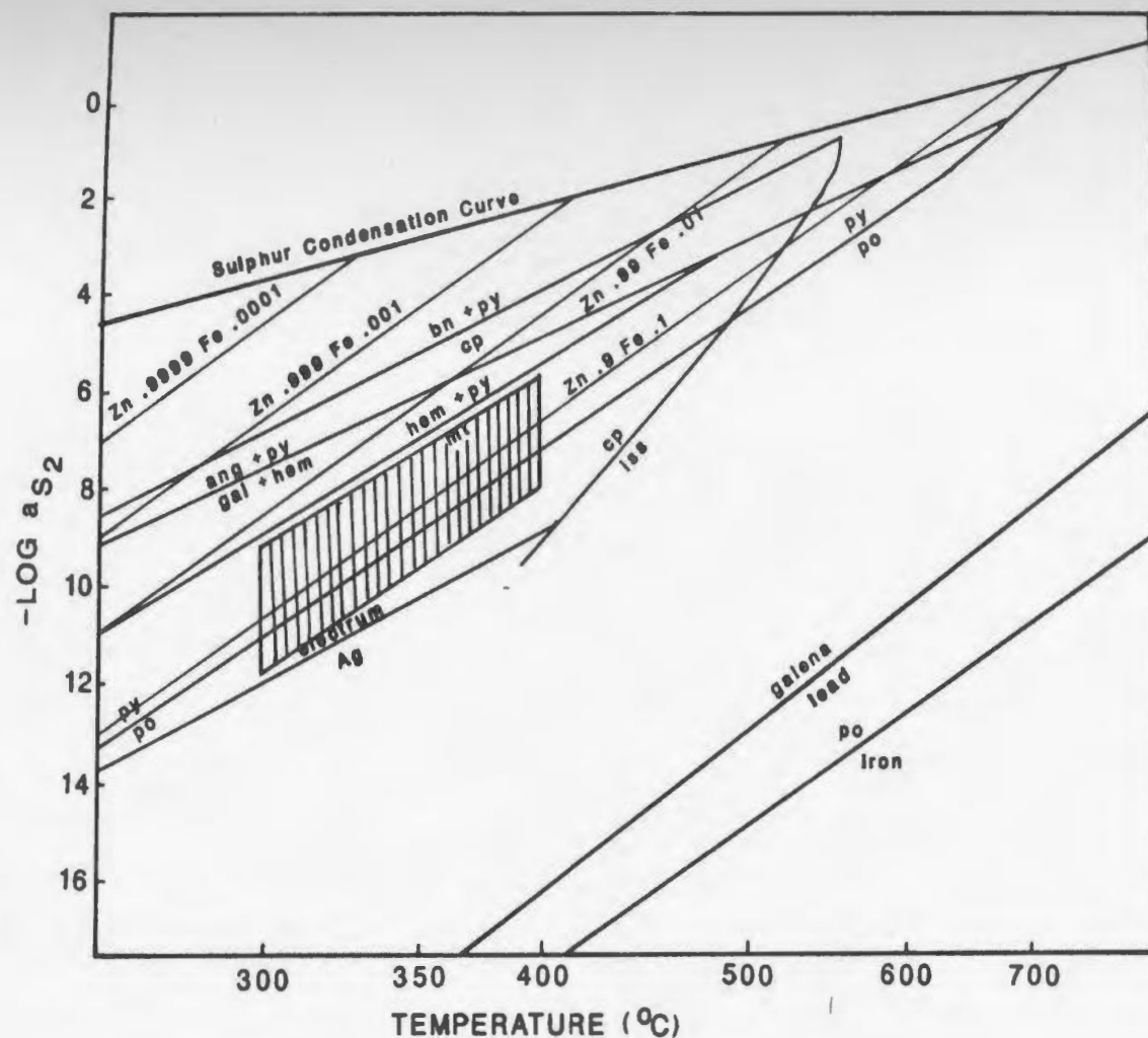
Figure 4.10. Temperature vs. -\log a_{\text{S}_2} for various sulphidation reactions from Barton and Skinner (1979), with added sphalerite compositions in equilibrium with pyrite and pyrrhotite (from Barton and Toumlin, 1966). Ruled box outlines the probable conditions during mineralization at Winter Hill based upon mineral assemblages and sphalerite compositions.
