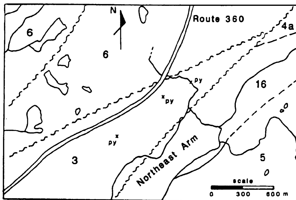
Figure 4.3. Location of the three massive pyrite outcrops constituting the Selco Showings. The map is redrawn from MacKenzie (1984) with geology from Greene and O'Driscoll (1976). The numbered lithological units are the same as in Figure 2.5. (Unit 4a = argillite)
