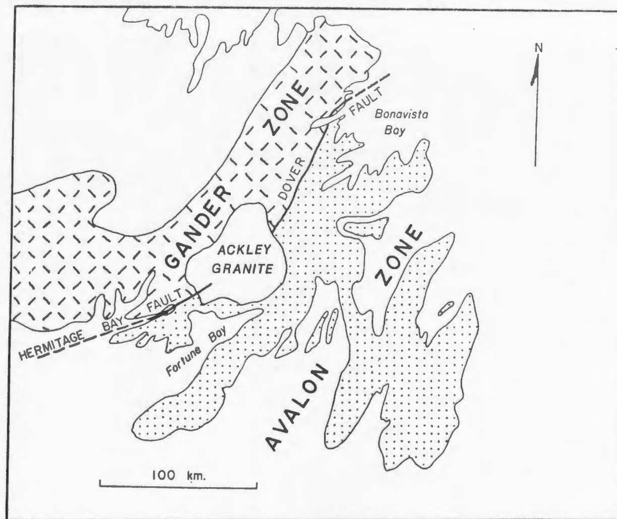
Figure 2.2. The Avalon-Gander Zone boundary and the respective positions of the Dover Fault, Hermitage Bay Fault, and the Ackley Granite. Modified from O'Driscoll (1977).
