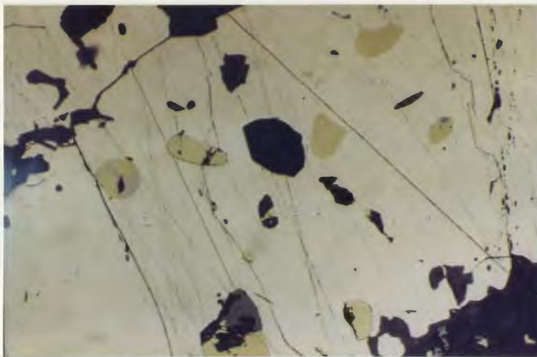
Plate 4.8. Large pyrite crystals with rounded inclusions of chalcopyrite (yellow) and pyrrhotite (light gray to light brown). Sample SS88-032 (584013), mag.= 200X, fov = 0.5 mm, reflected light.
