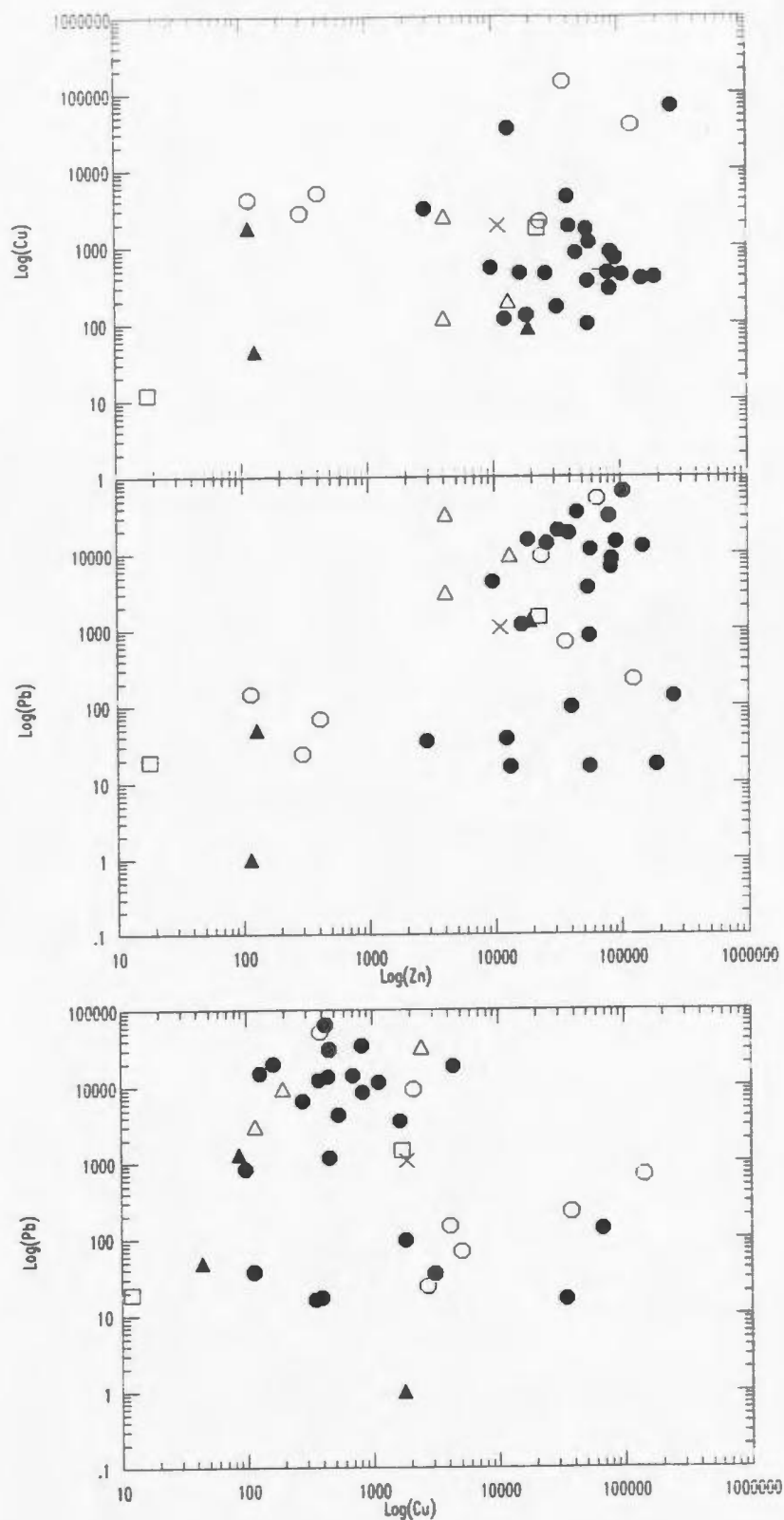
Figure 5.12. Base-metal variation plots for samples from the Sam Head Fm. Open circles = Winter Hill (lower zone), filled circles = Winter Hill (upper zone), open triangles = Winter Hill East, filled triangles = Winter Hill West, X = Winter Hill North, and open squares = Prospect #5.
