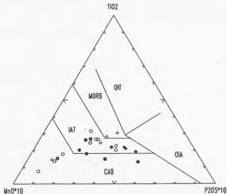
Figure 3.36. MnO - TiO 2 - P 2 O 5 ternary plot for mafic samples containing between 45 and 54 wt.% SiO 2 (taken from Mullen, 1983). CAB = calcalkaline basalt, IAT = island arc tholeiite, MORB = mid-ocean ridge basalt, OIT = ocean island tholeiite, and OIA = ocean island alkali basalt. Symbols as in Figures 3.1 and 3.18.
