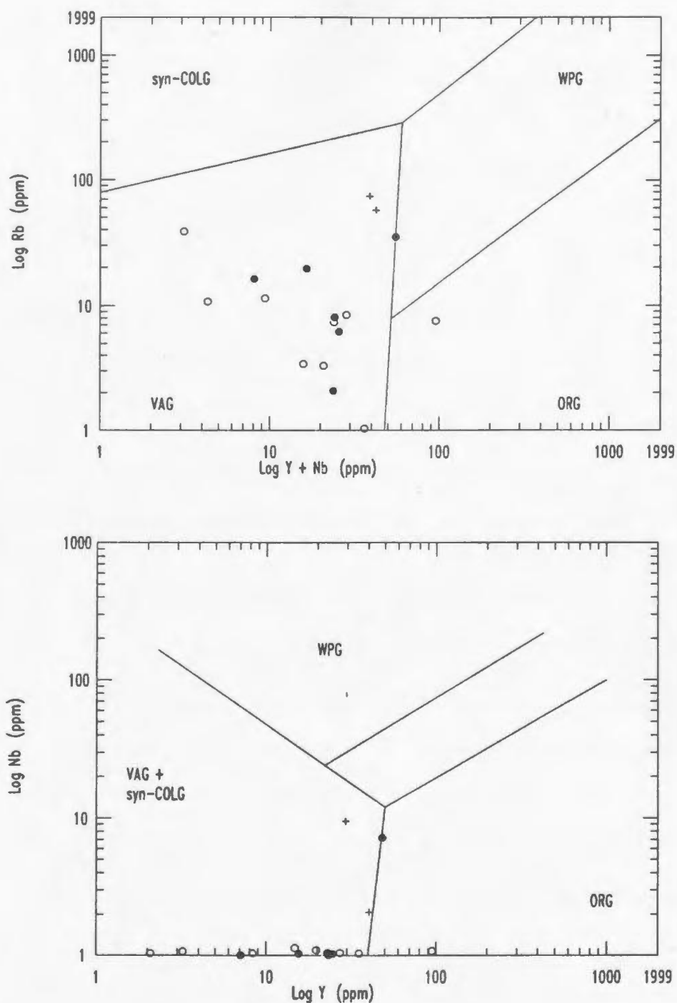
Figure 3.17. Y+Nb vs. Rb and Y vs. Nb plots, and the respective tectonic fields (from Pearce et al. , 1984). All samples but one plot in the volcanic arc granite field. Crosses = samples of the Straddling Granite, while the open and closed circles represent samples from the Simmons Brook Batholith and the Grole Diorite, respectively. WPG = within-plate granite, VAG = volcanic arc granite, syn-COLG = syn-collisional granite, and ORG = orogenic granite.
