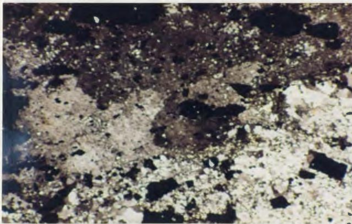
Plate 4.14. Cordierite (light gray to dark brown - near extinction) associated with fine-grained quartz (whitish, small, polygonal crystals). Sample SS88-037, mag.= 32X, fov = 3.3 mm, X-nicols.
