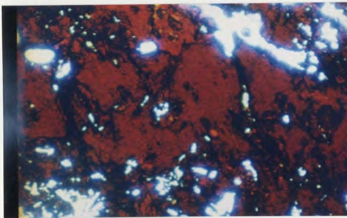
Plate 4.12. Fe-rich sphalerite from the upper zone at the Winter Hill Showing. Sample SS88-057, mag.= 32X, fov = 3.3 mm, PPL.
