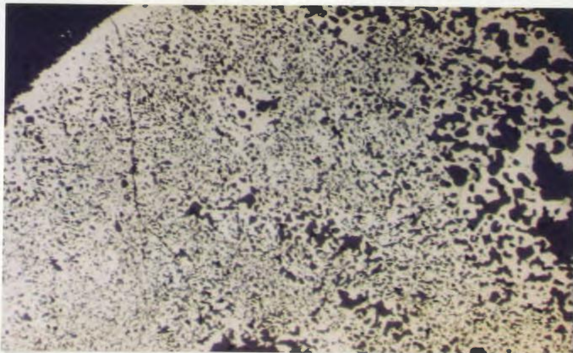
Plate 4.25. Large pyrite crystal from Winter Hill East containing numerous, rounded, calc-silicate inclusions. Sample SS88-121 (584076), mag.= 32X, fov = 3.3.mm, reflected light.
