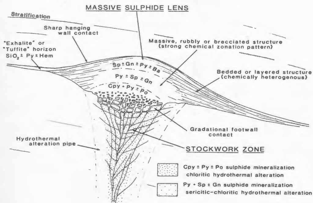
Figure 4.8. Schematic cross-section through an idealized volcanogenic massive sulphide deposit illustrating the more important lithological and mineralogical associations. Taken from Lydon (1984).
