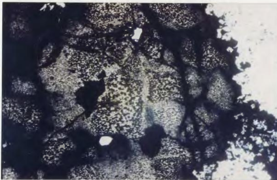
Plate 4.4. "Watermelon texture" consisting of dark, fine-grained chalcopyrite inclusions in a clear to light gray sphalerite crystal. sample SS88-414 (584196), mag.= 100X, fov = 1 mm, plane polarized light (PPL).
