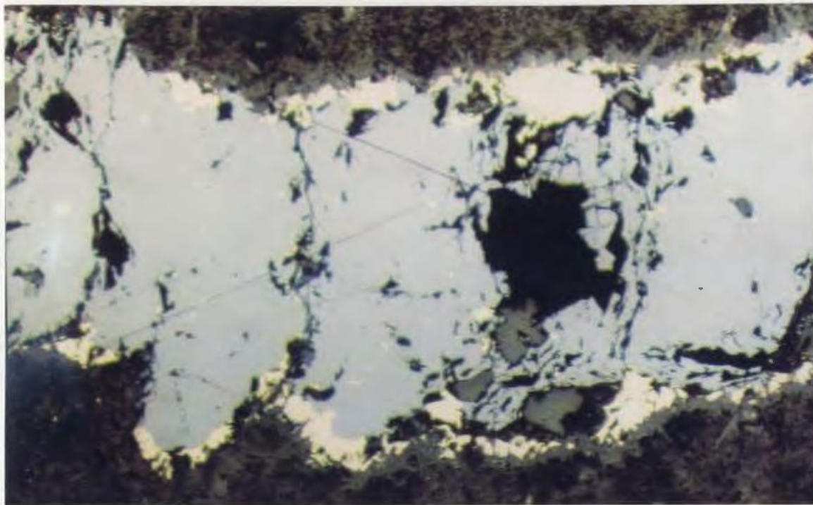
Plate 4.11. Large sphalerite crystal (gray) rimmed by chalcopyrite (whitish-yellow) near the lower zone - upper zone transition at Winter Hill. Sample SS88-039 (584016), mag.= 32X, fov = 3.3 mm, reflected light.
