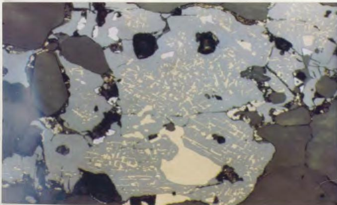
Plate 4.26. Chalcopryrite lamellae (?) and blebs (yellow) in a sphalerite crystal (medium gray) from the Winter Hill East Showing. Sample SS88-121 (584076), mag.= 200X, fov = 0.5 mm, reflected light.
