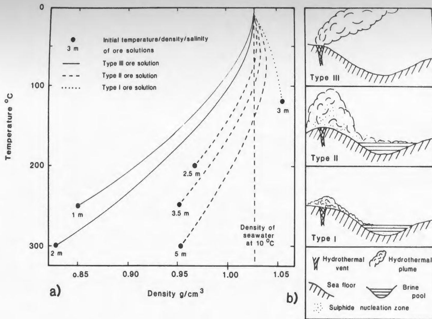
Figure 4.12 a) Density - temperature diagram illustrating the cooling trends of the three types of hydrothermal fluids when hot saline solutions mix with seawater at 10°C (after Sato (1972)). b) Schematic diagrams displaying the buoyancy of precipitating sulphides from Sato's (1972) different types of hydrothermal solutions.
