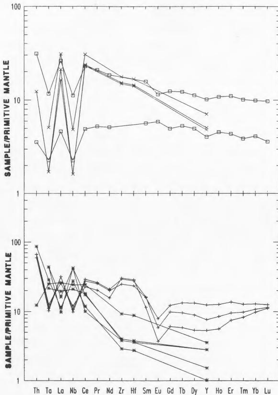
Figure 3.28. Extended REE profiles for mafic and felsic dykes cutting rocks of the Connaiyre Bay Group. Upper diagram: open squares = older mafic dykes; X = younger mafic dykes. Lower diagram: + = older felsic dykes; * = younger felsic dykes.
