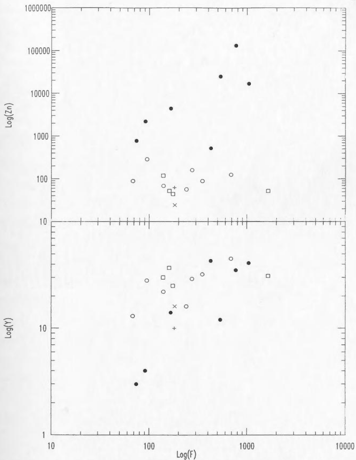
Figure 5.9. F vs. Zn and Y for samples from the Tickle Point Fm. Symbols as in Figure 5.1.
