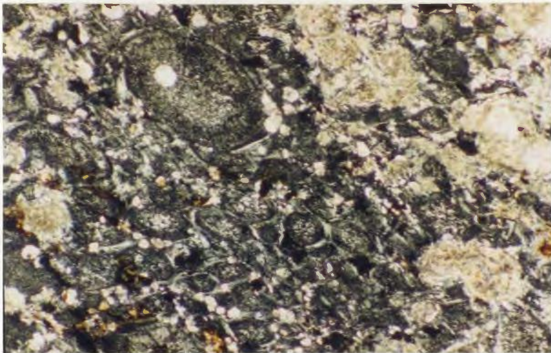
Plate 4.3. Relict spherulites (amygdules ?) in a carbonate-chlorite alteration zone at Frenchman Head. Sample SS88-407 (584193), mag.= 32X, fov = 3.3 mm, X-nicols.
