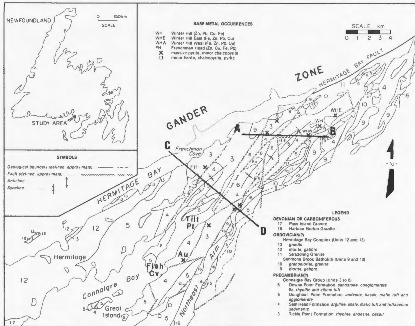
Figure 2.5. Geology of the Hermitage Peninsula with mineralized localities. Adapted from Sears and O'Driscoll (1989) after Greene and O'Driscoll (1976).
