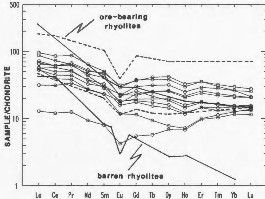
Figure 3.32. Chondrite-normalized REE profiles presenting the patterns for dacitic to felsic rocks from the Tickle Pt. Fm., and the superimposed ranges for ore-bearing and barren rhyolites, as defined by Campbell et al. (1982).
