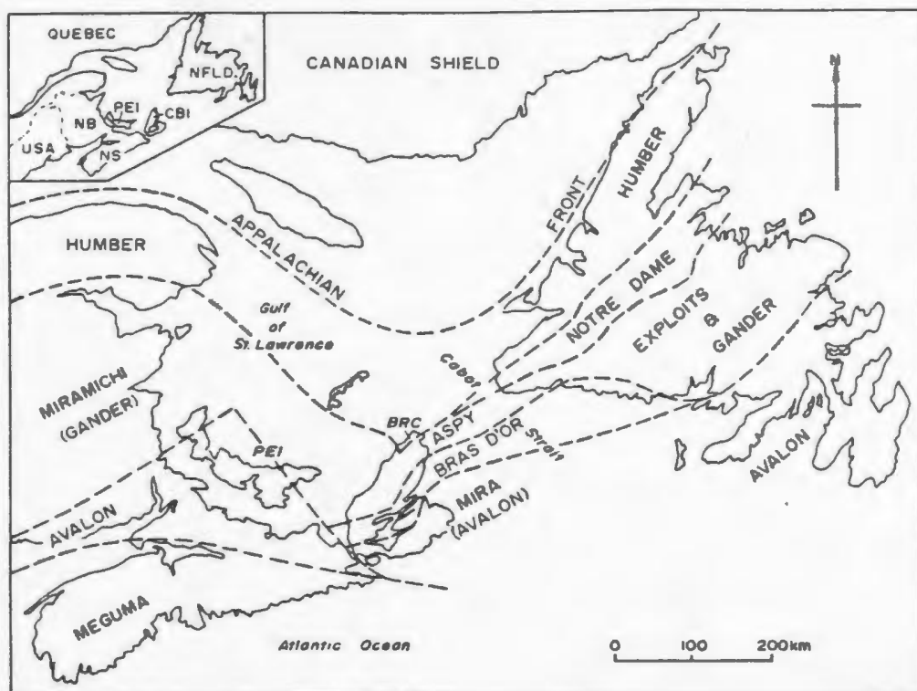
Figure 2.3. Tectonostratigraphic terrane map of Nova Scotia and Newfoundland and the inferred correlation. Taken from Barr and Raeside (1989).
