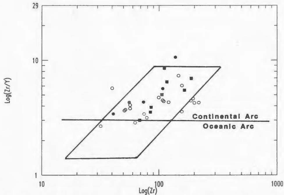
Figure 3.37. Plot of Zr vs. Zr/Y (from Pearce, 1983) displaying a dividing line between continental arc volcanic rocks and oceanic arc volcanic rocks. The field above the line represents average compositions for continental arc basalts and the field below the line represents average compositions for oceanic arc basalts. Symbols as in Figures 3.1 and 3.18.
