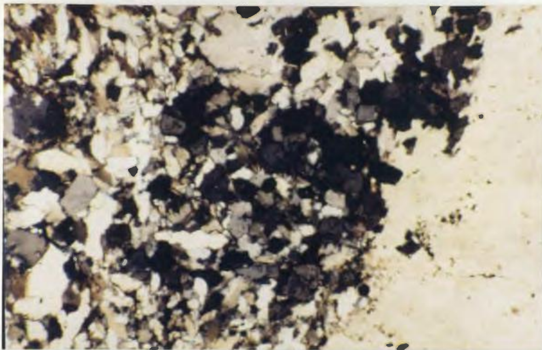
Plate 4.1. Small, dark gray, equant andalusite crystals (centre of photo) from a mineralized sample from Frenchman Head. Sample SS88-390 (584186), mag.= 32X, fov = 3.3 mm, X-nicols.
