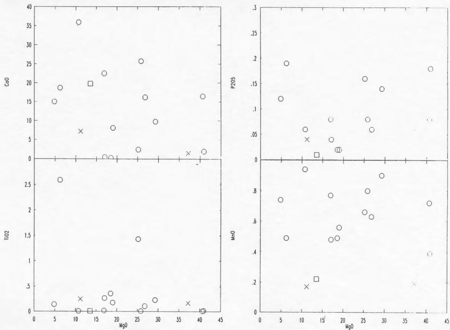
Figure 5.22. MgO vs. other major elements for the carbonate/Ca-Mg-silicate samples from the Winter Hill area. Symbols as in Figure 5.21.
