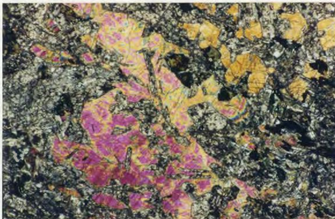
Plate 2.12. Ophitic to subophitic texture in a gabbroic phase of the Hermitage Bay Complex. Sample SS88-264 (584138), mag.= 17.5X, fov = 6.2 mm, X-nicols.
