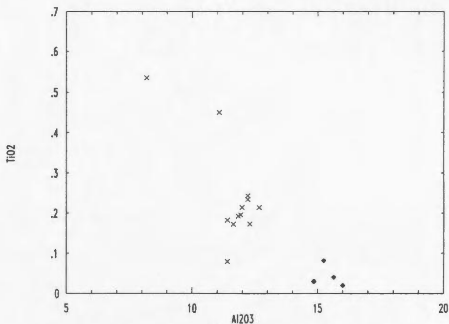
Figure 3.25. Al_2O_3 vs. TiO_2 variation diagram. The younger dyke suite is distinguished from the older suite by higher Al_2O_3 and lower TiO_2 . Symbols as in Figure 3.21.
