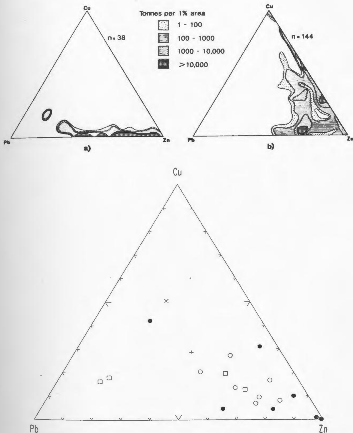
Figure 5.2. Pb-Cu-Zn ternary diagram for mineralized samples from the Tickle Point Formation. Ternary diagrams (a) and (b) represent bulk compositions for sediment-hosted stratiform Pb-Zn deposits (a) and VMS deposits of the Abitibi Belt, the New Brunswick area, Norwegian Caledonides, and the Green Tuff Belt of Japan (b) (taken from Lydon, 1983). Contours are total tonnes of ore metals per 1% area of the diagram. Symbols as in Figure 5.1.
