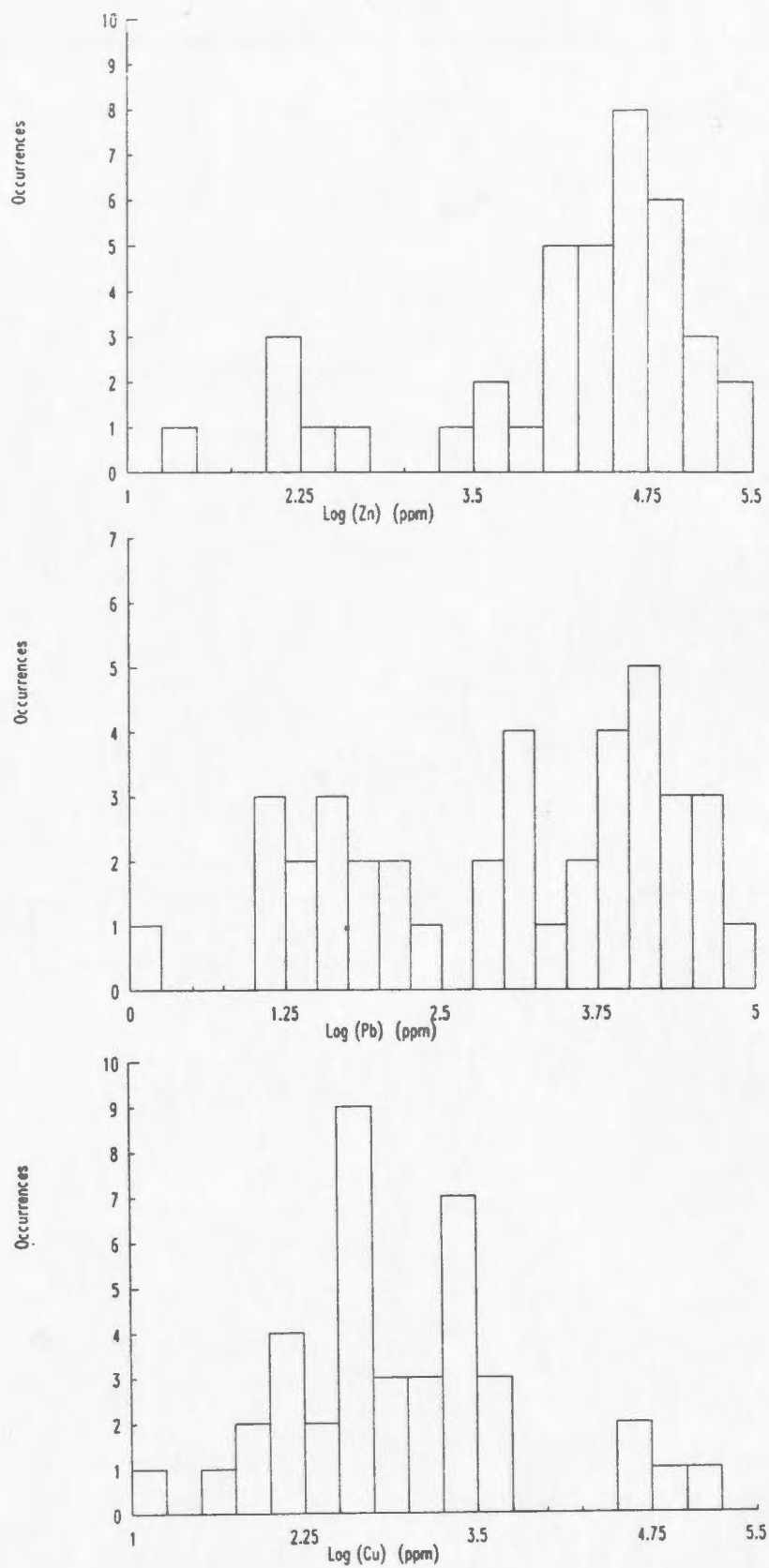
Figure 5.13. Histograms of Zn, Cu, and Pb for mineralized samples from the Sam Head Fm. Each histogram has a total of 39 samples.
