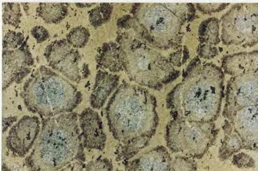
Plate 2.8. Relict spherulite containing fine-grained quartz-rich cores, inner sericitic mantles, and outer sericite-and opaque-rich mantles, in a very fine-grained sericite groundmass. Sample SS88-515, mag.= 8X, fov = 13.2 mm, X-nicols.
