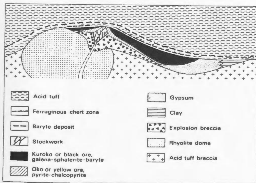
Figure 4.9. Schematic cross-section through an idealized Kuroko deposit. Taken from Evans (1980) after Sato (1977).
