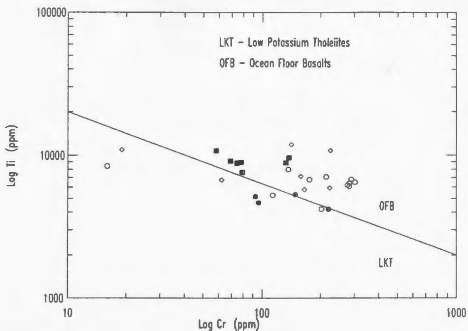
Figure 3.33. Cr vs. Ti plot defining LKT (low potassium tholeiite) and OFB (ocean floor basalt) fields, taken from Pearce (1975). Symbols as in Figures 3.1 and 3.18.
