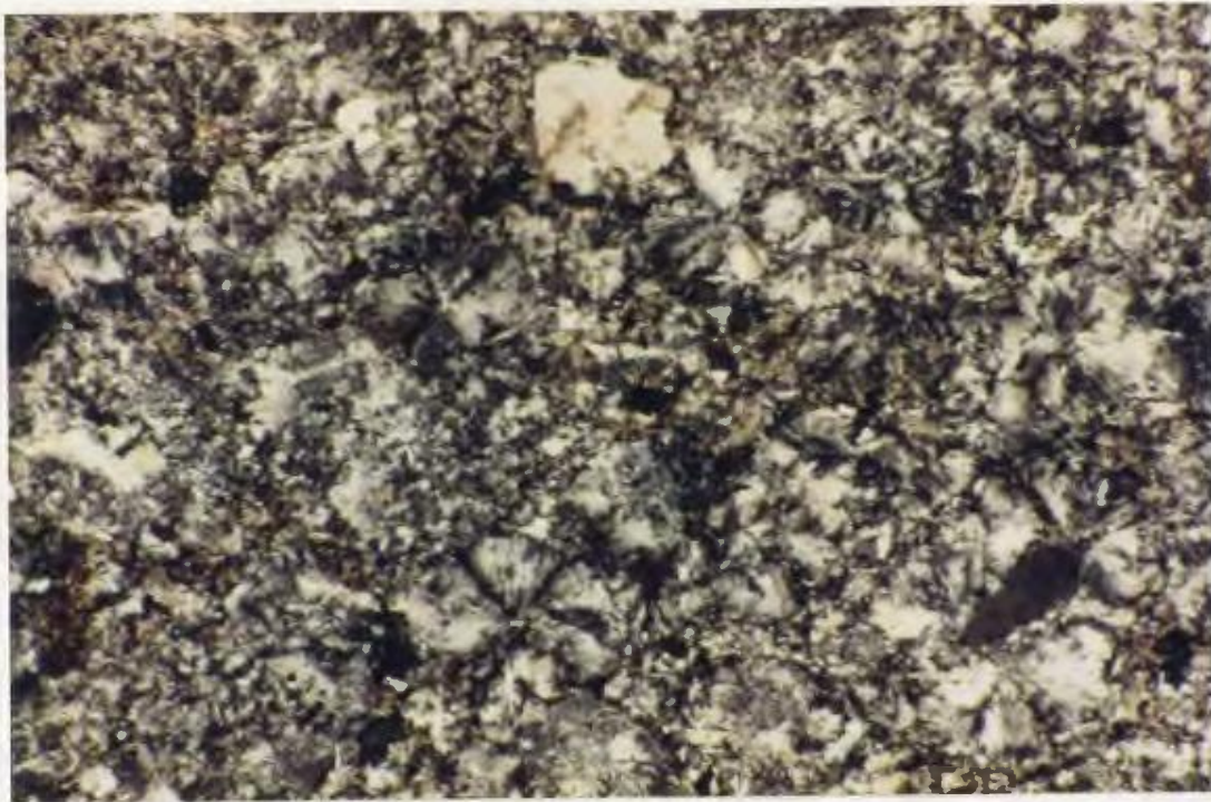
Plate 2.15. Spherulites in a rhyolite dyke. Sample SS88-502, mag.= 20X, fov = 5.3 mm, X-nicols.
