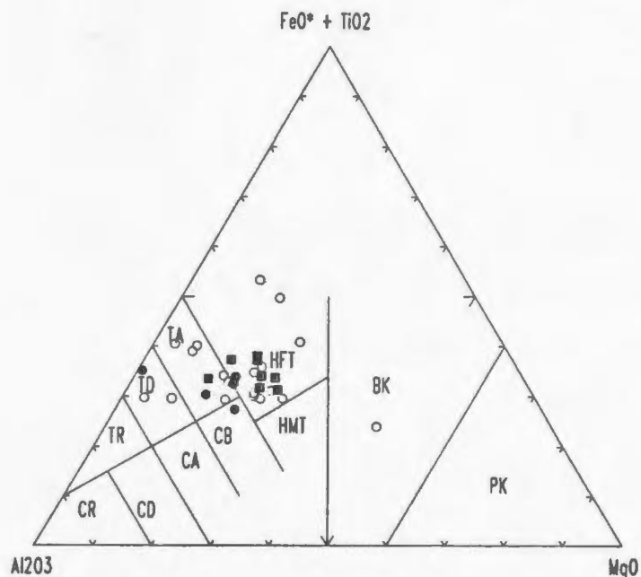
Figure 3.7. \text{Al}_2\text{O}_3 - \text{FeO}^* ( \text{Fe} total) + \text{TiO}_2 - \text{MgO} ternary diagram after Jensen (1976). This plot illustrates the tholeiitic nature of the mafic to intermediate rocks. Symbols as in Figure 3.1. CR, CD, CA, CB = calcalkaline rhyolite, dacite, andesite, basalt; TR, TD, TA = tholeiitic rhyolite, dacite, andesite; HFT = high Fe tholeiite; HMT = high Mg tholeiite; BK = basaltic komatiite; PK = picritic komatiite.
