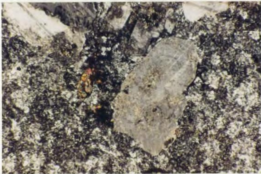
Plate 2.2. Oscillatory zoned plagioclase crystal with albite twins from rhyolite belonging to the Tickle Point Formation. Sample SS88-422 (584199), magnification (mag.) = 26X, field of view (fov) = 4.0 mm (long dimension), X-nicols.
