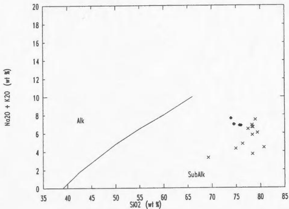
Figure 3.22. \text{SiO}_2 vs. alkalis diagram. Both felsic dyke suites have are subalkaline in character. Symbols as in Figure 3.21.
