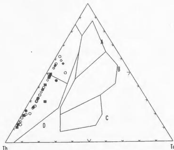
Figure 3.29. Th - Hf - Ta ternary diagram (from Wood, 1980). The mafic to intermediate samples all plot in the destructive plate margin field. A = N (normal)-type MORB; B = E (enriched)-type MORB and tholeiitic within-plate basalts and differentiates; C = alkaline within-plate basalts and differentiates; D = destructive plate margin basalts and differentiates. The arrowed line ( i.e. where Hf/Th = 3 ) within the D-field separates calcalkaline samples (below line) from tholeiitic samples (above line). Symbols as in Figures 3.1 and 3.18.
