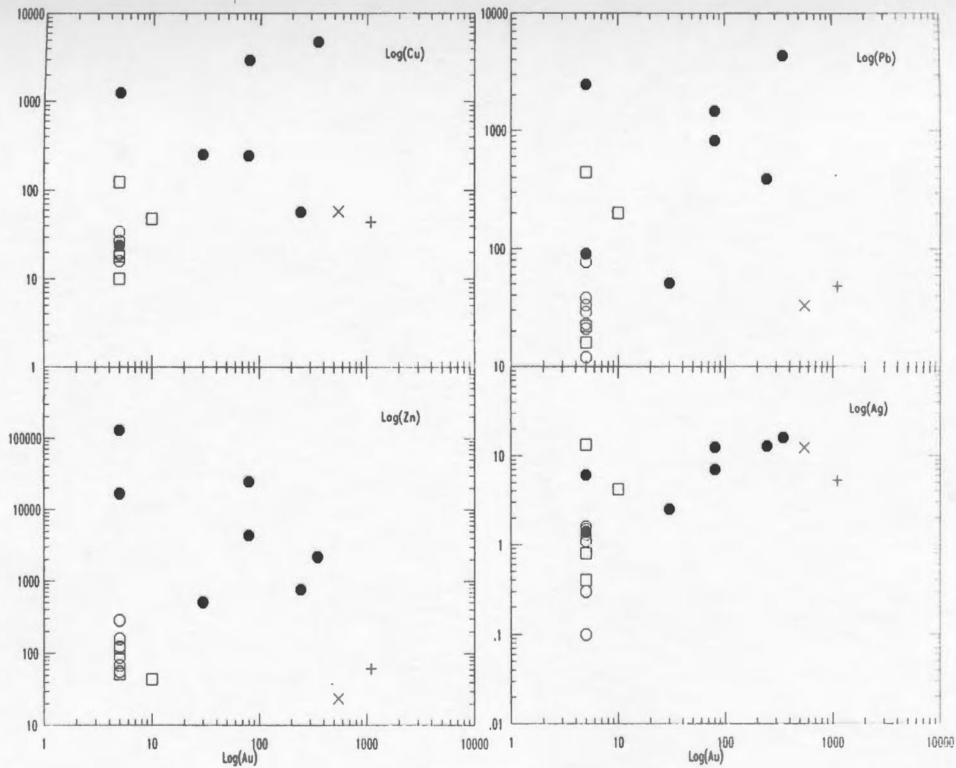
Figure 5.5. Variation diagrams involving Au (ppb) and Ag vs. the base-metals. Symbols as in Figure 5.1.
