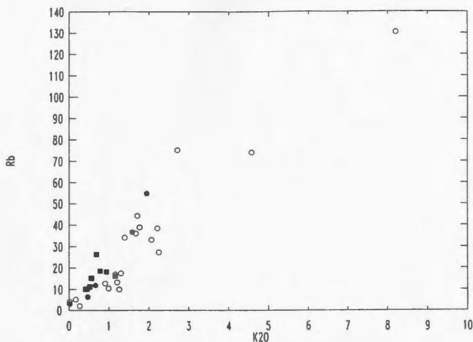
Figure 3.5. Plot of K 2 O vs. Rb displaying a positive linear relationship. Symbols as in Figure 3.1.
