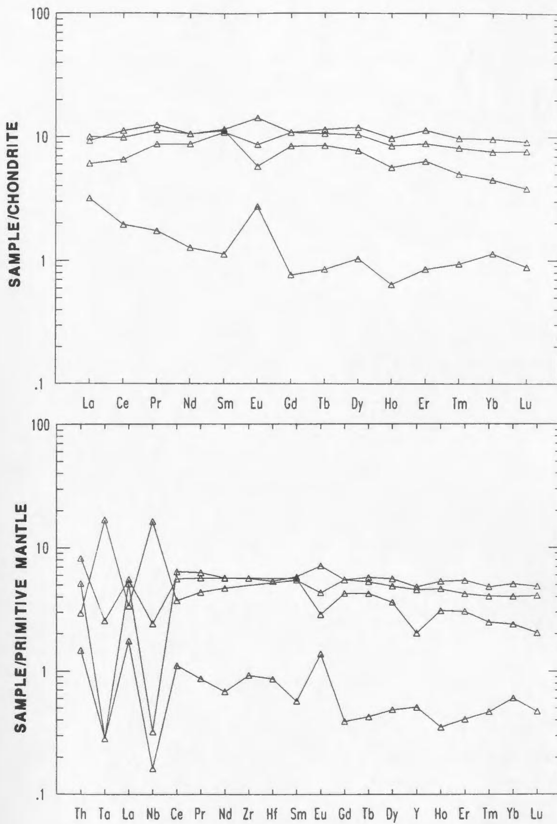
Figure 5.19. REE and extended REE profiles for mineralized samples from the Winter Hill East Showing.
