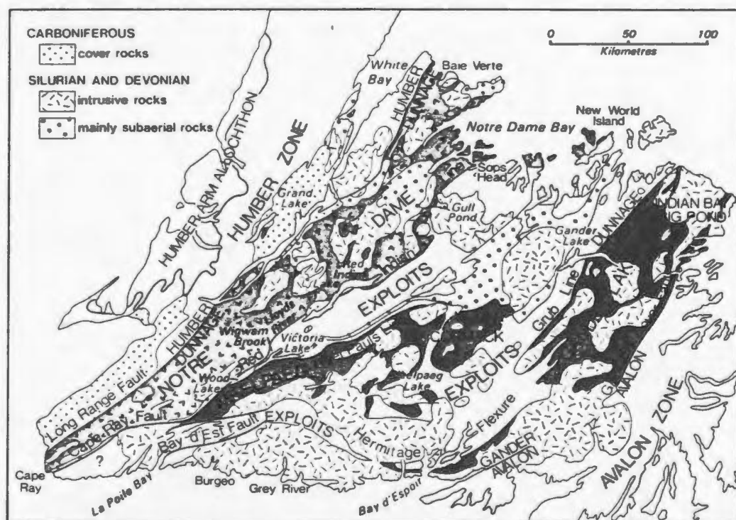
Figure 2.4. Dunnage and Gander Zone subdivisions in Newfoundland, from Williams et al. (1988).
