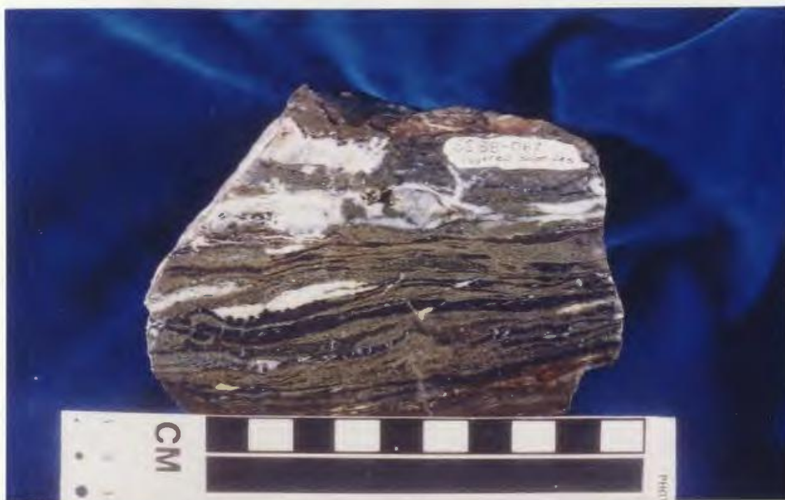
Plate 4.19. Layered pyrite (yellow-brown), sphalerite (dark brown), and lesser galena (bluish gray - below sample caption) with a quartz-carbonate gangue from the Winter Hill Showing. Sample SS88-067.
