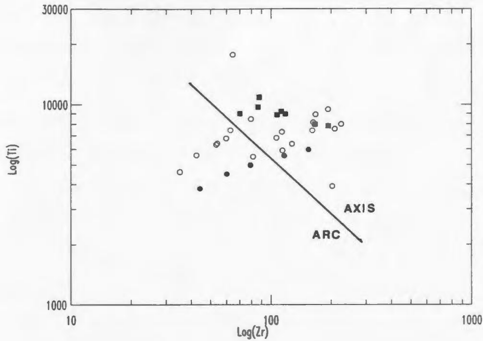
Figure 3.35. Zr vs. Ti diagram illustrating the arc/axis dividing line (after Pearce et al. , 1981), and the transitional nature of the mafic rocks. Symbols as in Figures 3.1 and 3.18.
