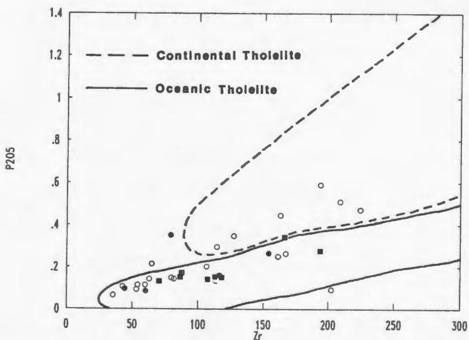
Figure 3.8. Plot of \text{Zr} vs. \text{P}_2\text{O}_5 and the respective fields for oceanic and continental tholeiites. The mafic to intermediate rocks have a strong oceanic character. Symbols as in Figure 3.1.
