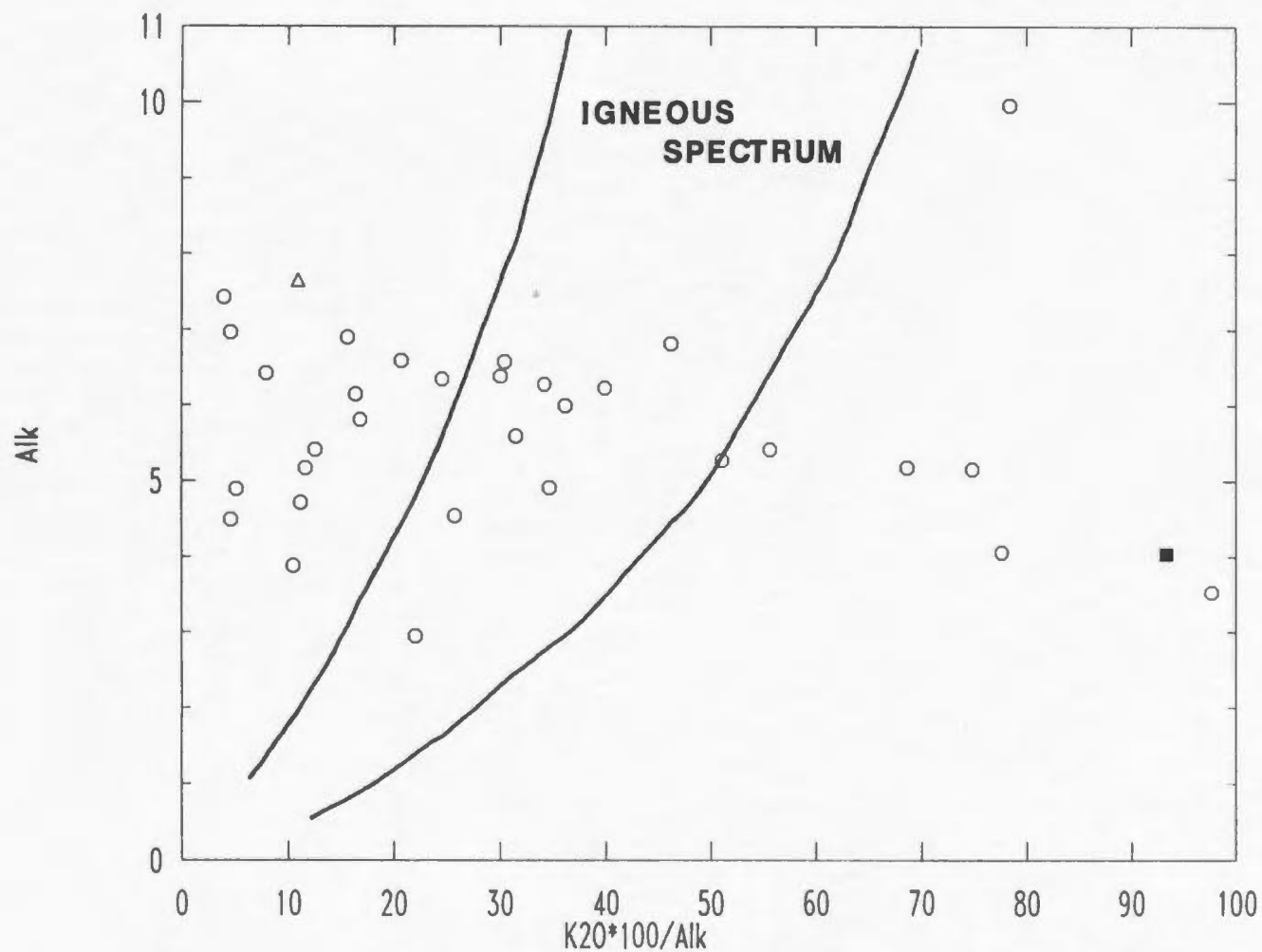
Figure 3.9. An "igneous spectrum" diagram taken from Hughes (1973). The felsic rocks are generally altered with respect to the K_2O and Na_2O , but the overall alkali content remains fairly constant between 4 and 7 wt.%. Symbols as in Figure 3.1.
