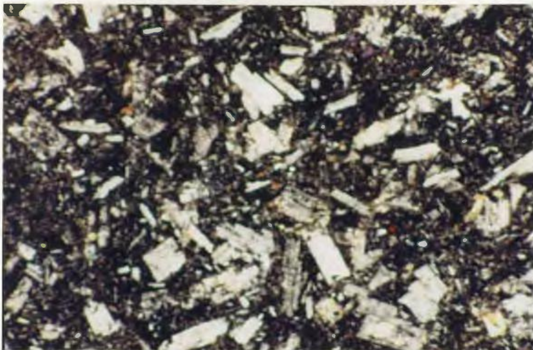
Plate 2.9. Mafic volcanic rock from the Doughball Point Formation containing plagioclase laths and small pyroxene crystals in a glassy matrix. Sample SS88-469 (584211), mag.= 20X, fov = 5.3 mm, X-nicols.
