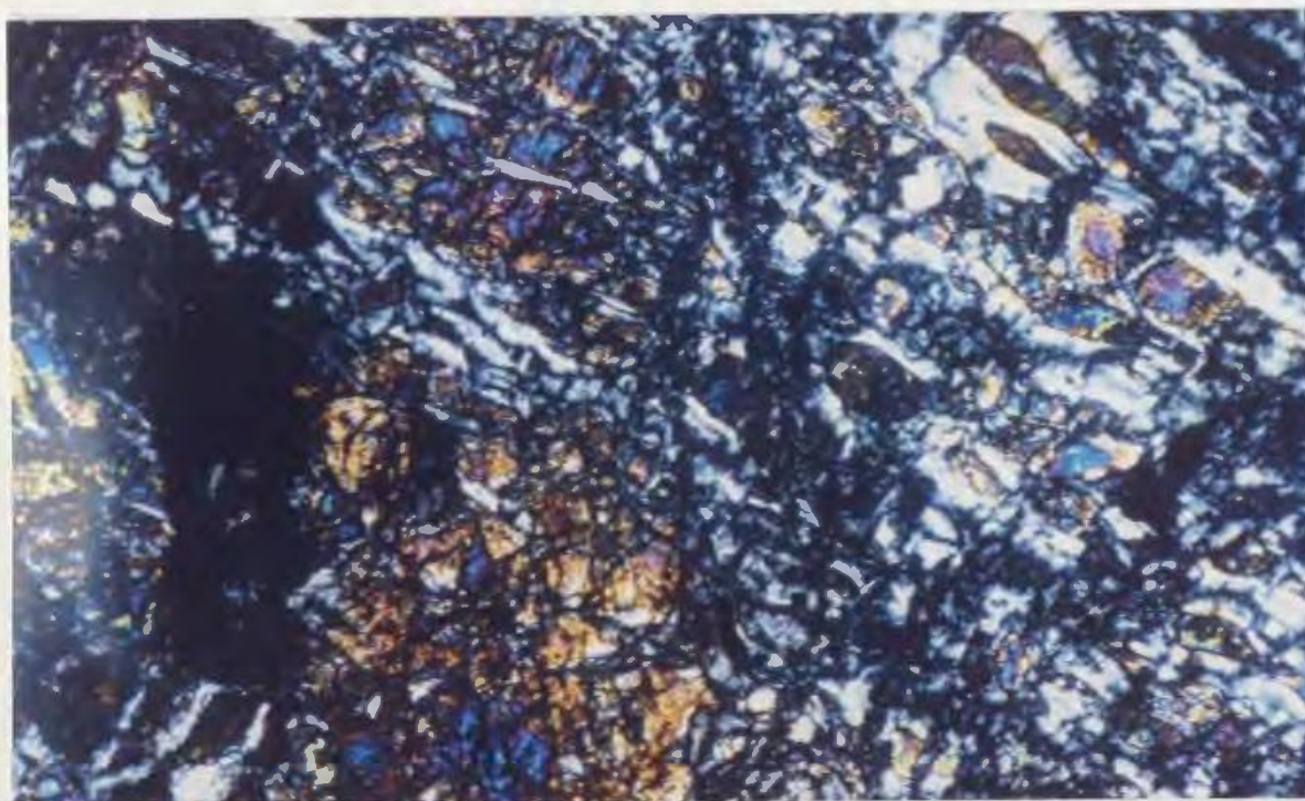
Plate 4.16. Serpentized olivines in an alteration zone at the base of the carbonate/calc-silicate lens at Winter Hill. Sample SS88-048 (584024), mag.= 100X, fov = 1 mm, X-nicols.
