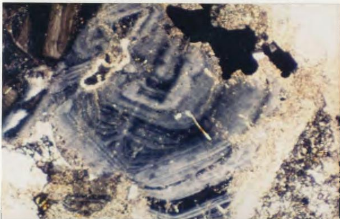
Plate 4.2. Oscillatory zoned plagioclase in andesitic rock from Frenchman head. Sample SS88-356 (584174), mag.= 22.5X, fov = 4.8 mm, X-nicols.
