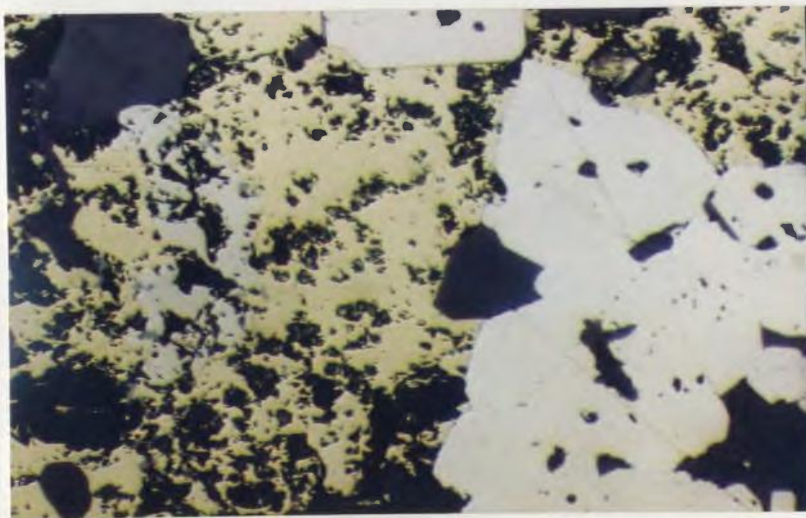
Plate 4.10. Crystals of chalcopyrite (yellow) associated with pyrite (white) in thin stringers from the lower zone at Winter Hill. Sample SS88-512, mag.= 100X, fov = 1 mm, reflected light.
