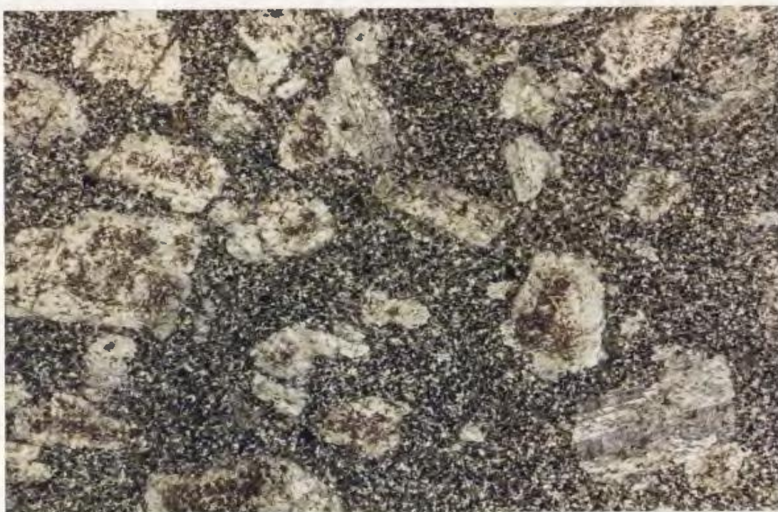
Plate 2.17. Altered plagioclase crystals with relict albite twins from the younger mafic dyke set. Sample SS88-366 (584177), mag.= 6.3X, fov = 17.0 mm, X-nicols.
