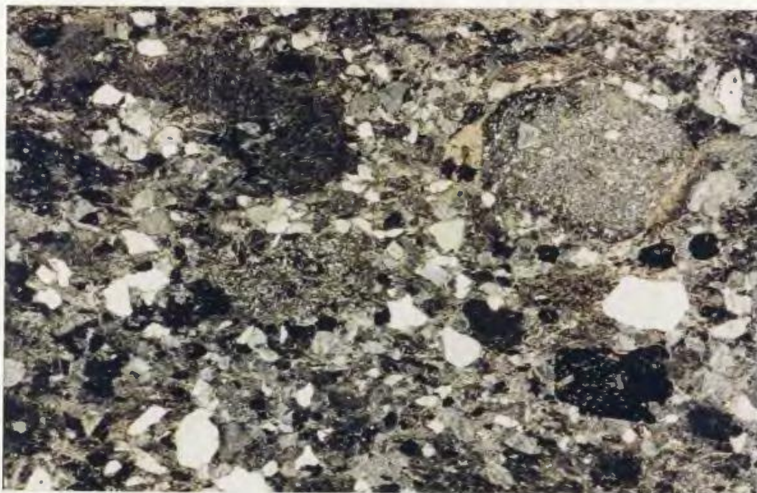
Plate 2.10. Lithic and crystal fragments in a lithic arkose from the Down's Point Formation. Sample SS88-458 (584208), mag.= 7X, fov = 15.0 mm, X-nicols.
