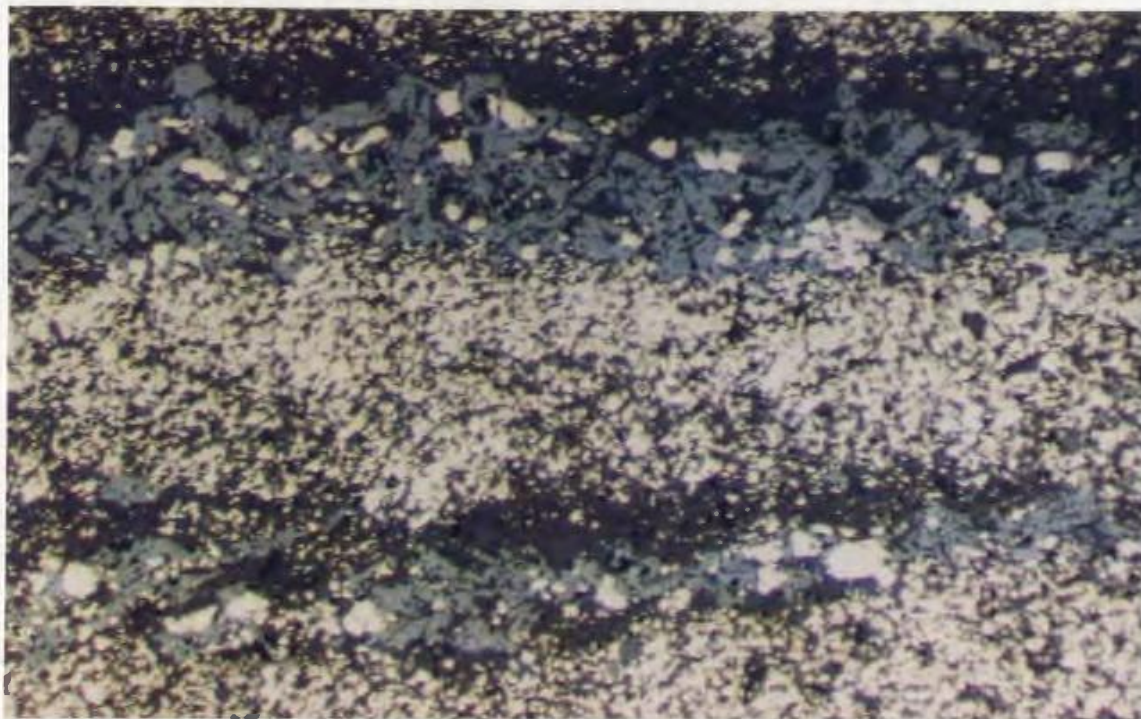
Plate 4.5. Alternating layers of pyrite (whitish) and magnetite (dark gray) from the Selco Showings. Sample SS88-141 (584086), mag.= 32X, fov = 3.3 mm, reflected light.
