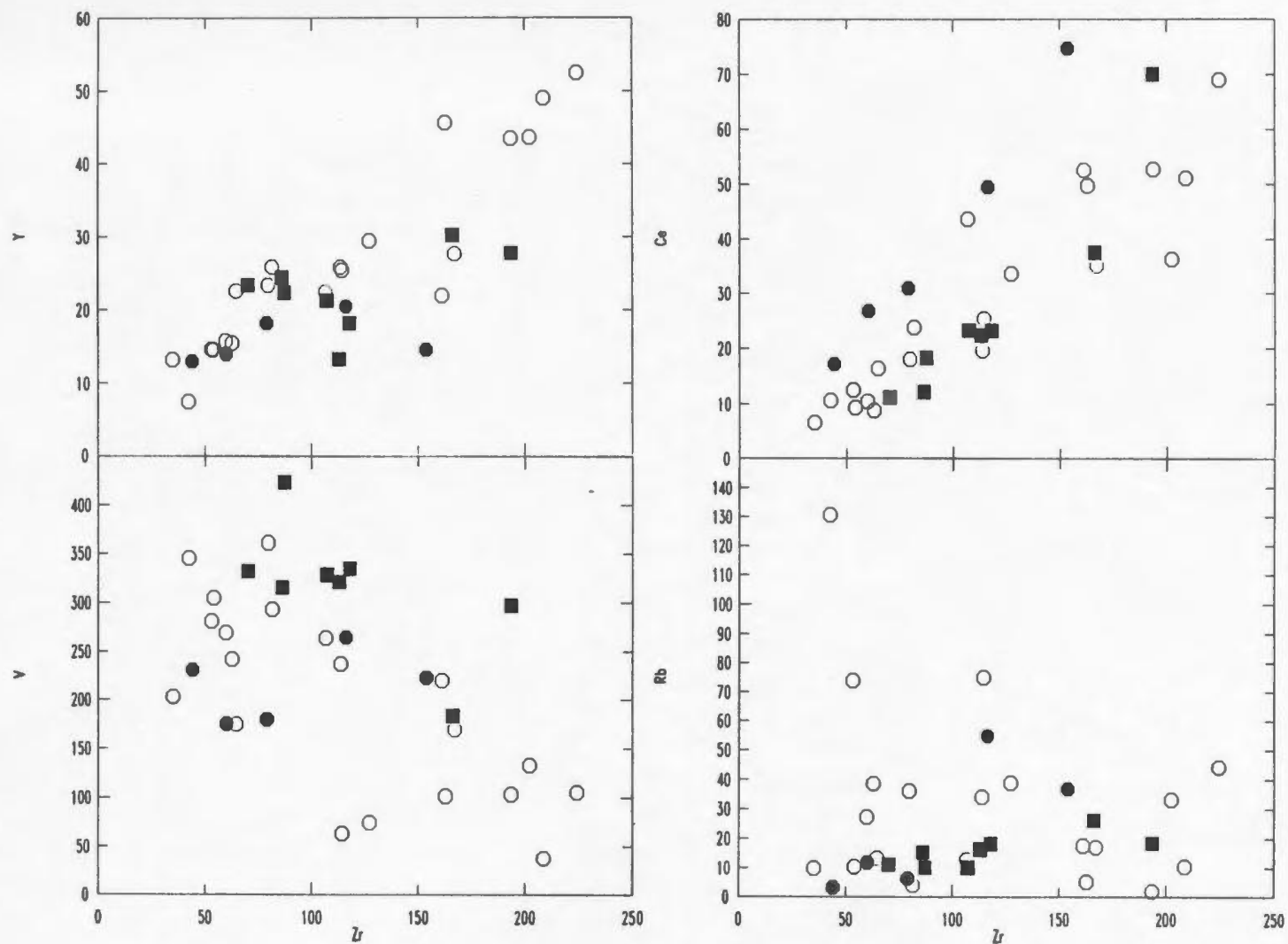
Figure 3.3. Variation diagrams of Zr vs. selected trace elements. Symbols as in Figure 3.1.
