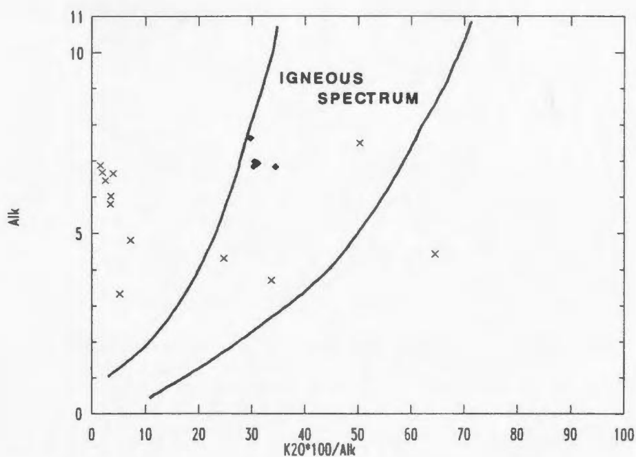
Figure 3.24. An "igneous spectrum" plot illustrating the apparently altered younger felsic dykes and the apparently Na-altered older felsic dyke suite. Symbols as in Figure 3.21.
