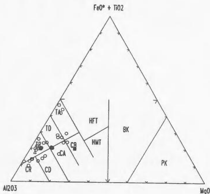
Figure 3.14. \text{Al}_2\text{O}_3 - \text{FeO}^* (Fe total) + \text{TiO}_2 - \text{MgO} ternary diagram for the dacitic to felsic rocks. The rocks have an apparent transitional tholeiitic-calcalkaline character. Symbols as in Figure 3.1 and the fields are the same as in Figure 3.7.
