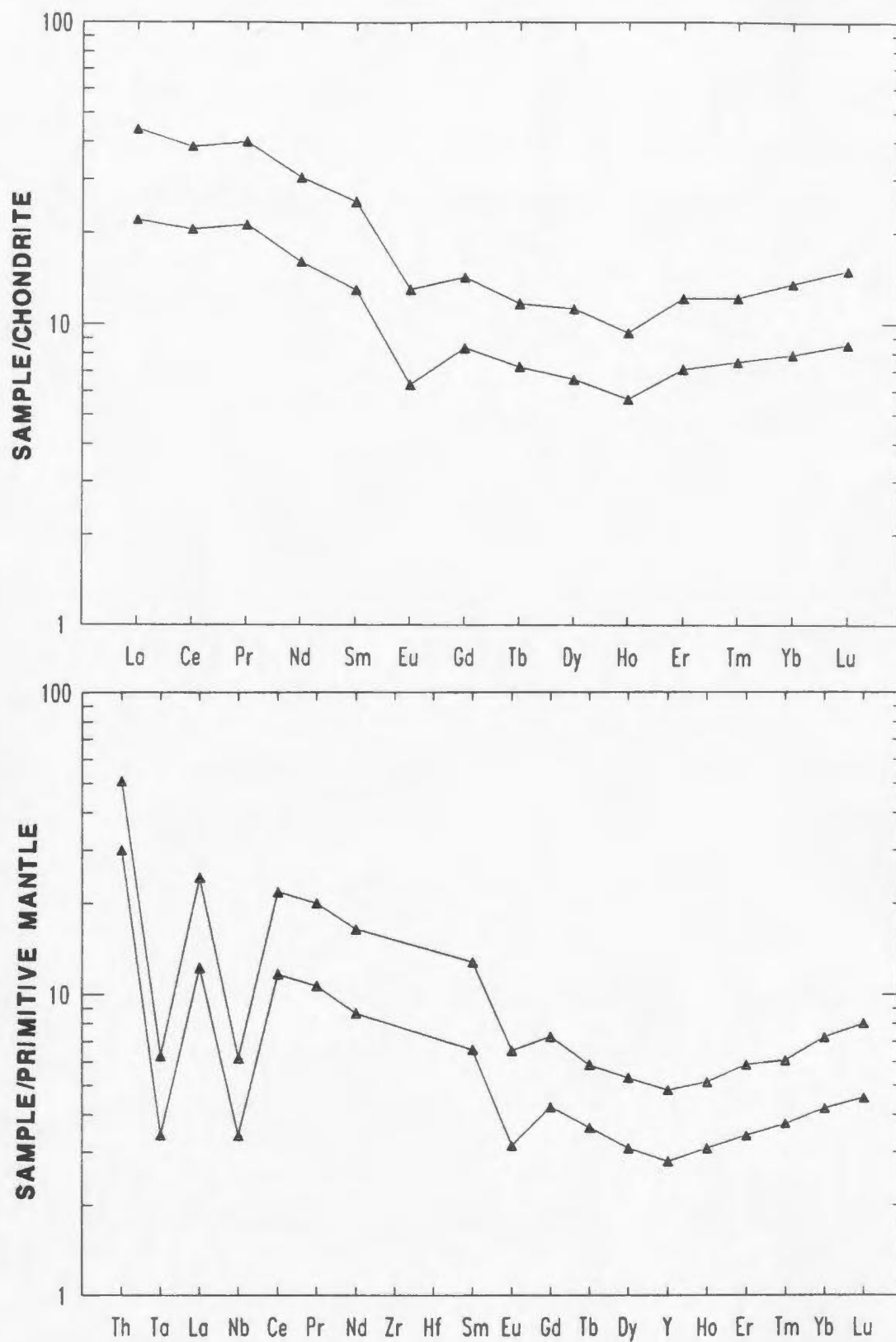
Figure 5.20. REE and extended REE patterns for samples from the Winter Hill West Showing.
