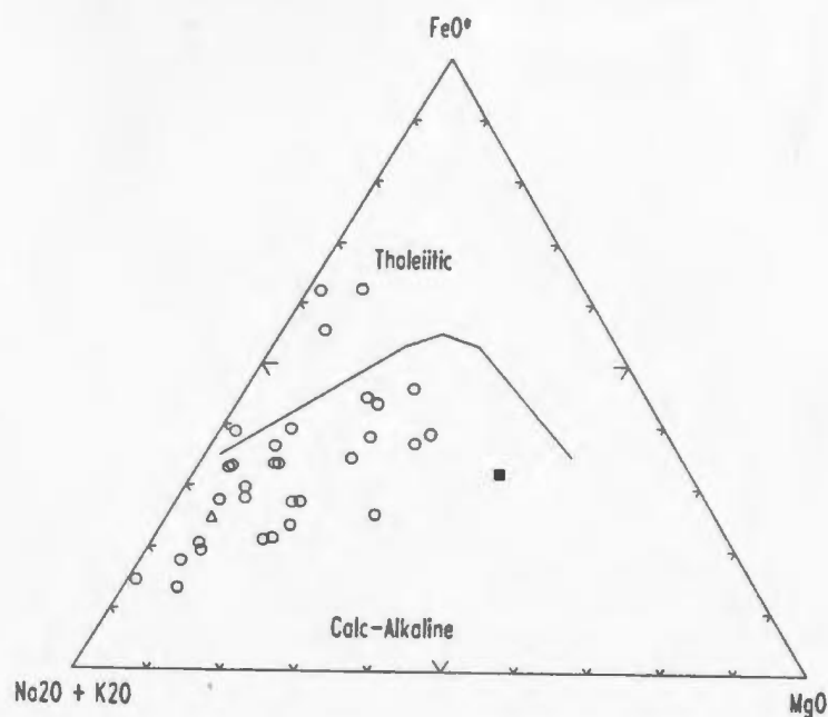
Figure 3.15. AFM diagram after Irvine and Baragar (1971). The dacitic to felsic samples display calcalkaline affinities. Symbols as in Figure 3.1. ( \text{FeO}^* = \text{Fe total} ).
