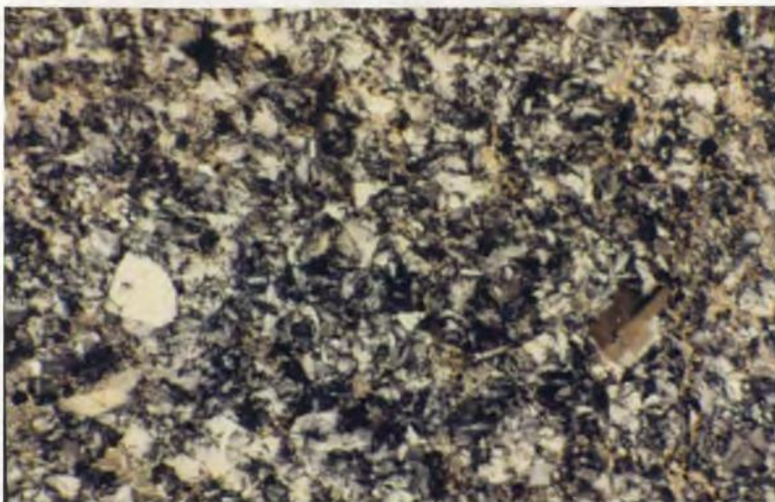
Plate 2.3. Spherulites in rhyolite from the Tickle Point Formation. Sample SS88-197 (584109), mag.= 8X, fov = 13.2 mm, X-nicols.
