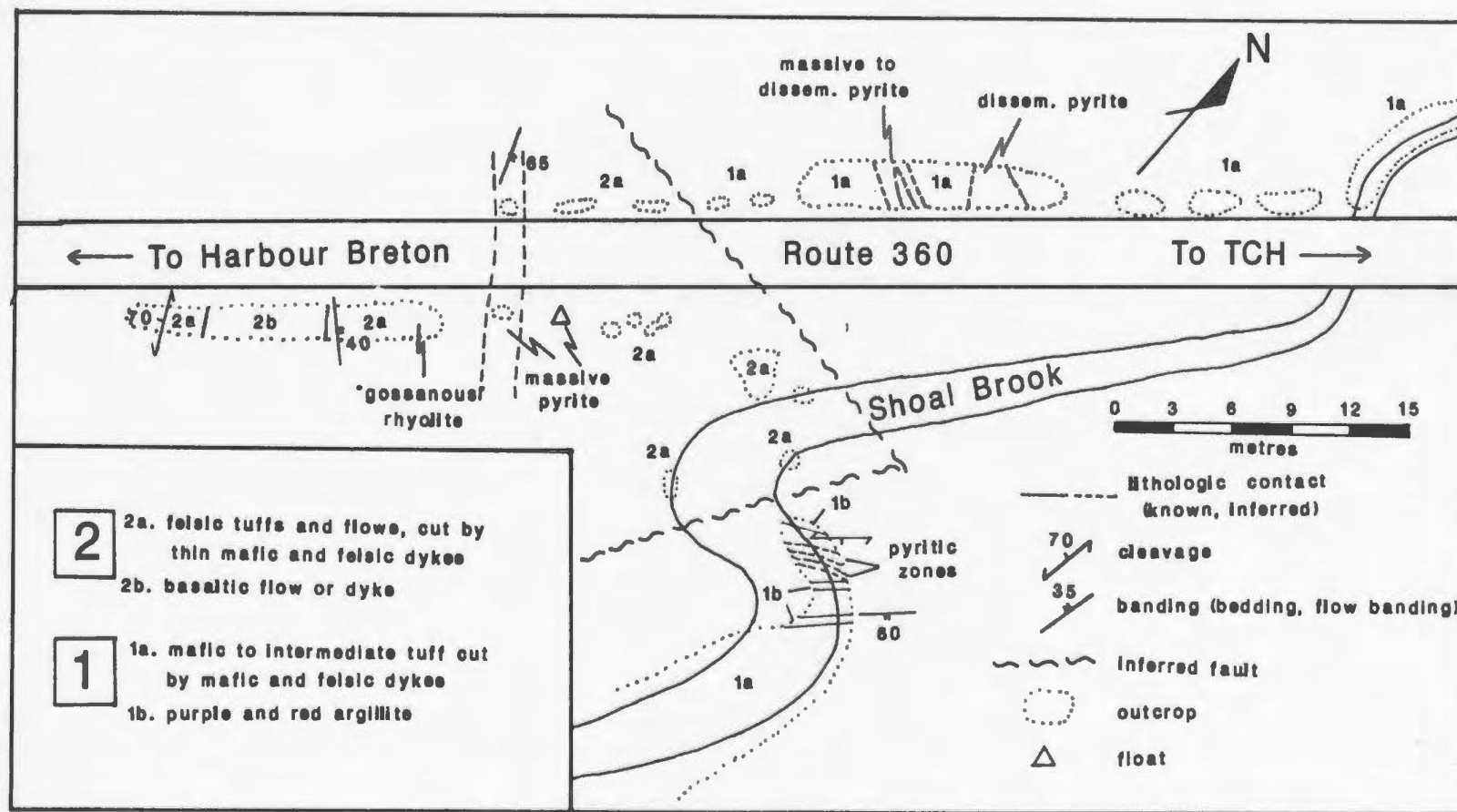
Figure 4.2. Detailed geology of the Shoal Brook Showing.
