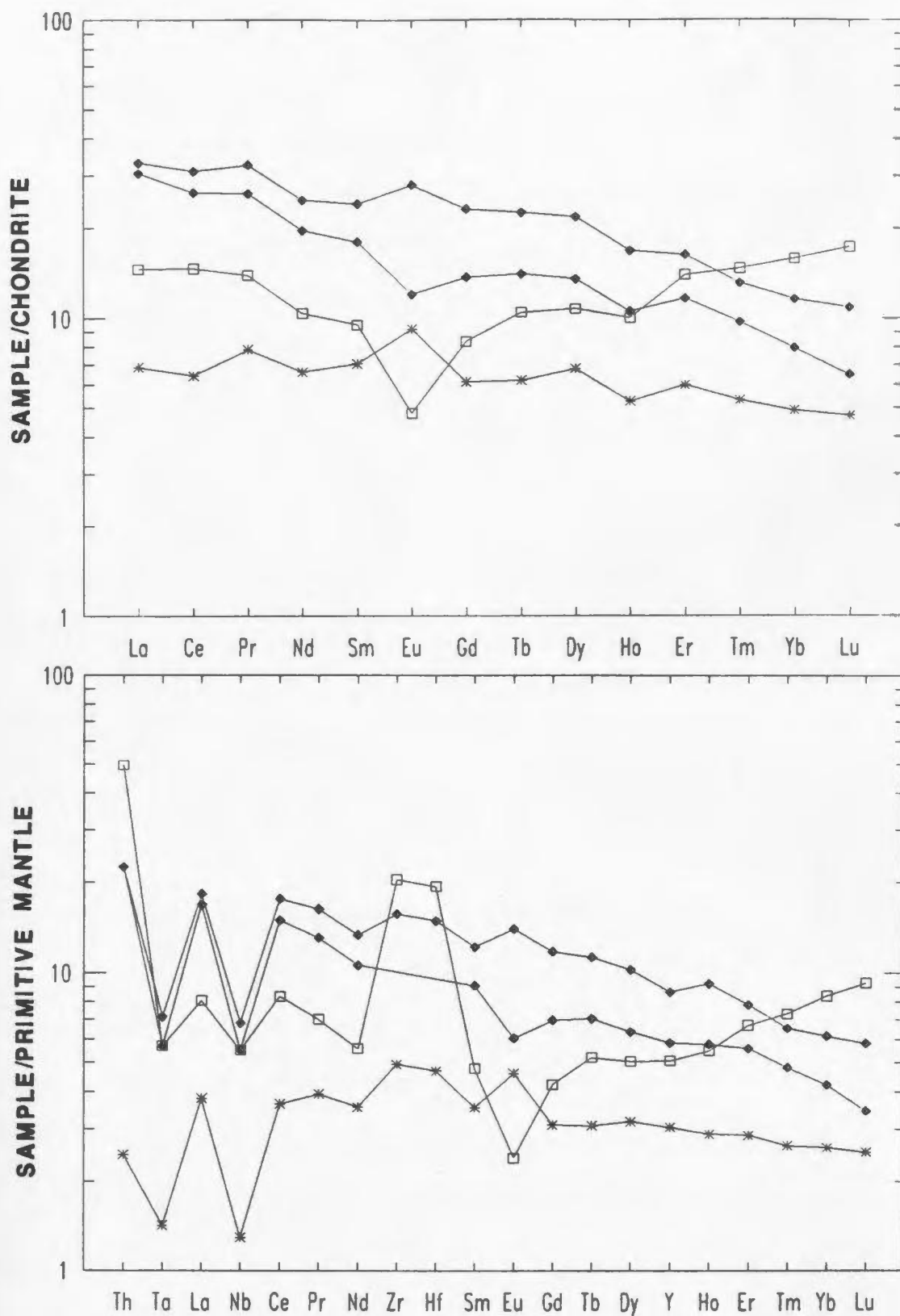
Figure 5.11. REE and extended REE patterns for samples from Shoal Brook (filled diamonds), Frenchman Head (asterisk), and Tilt Point (open squares).
