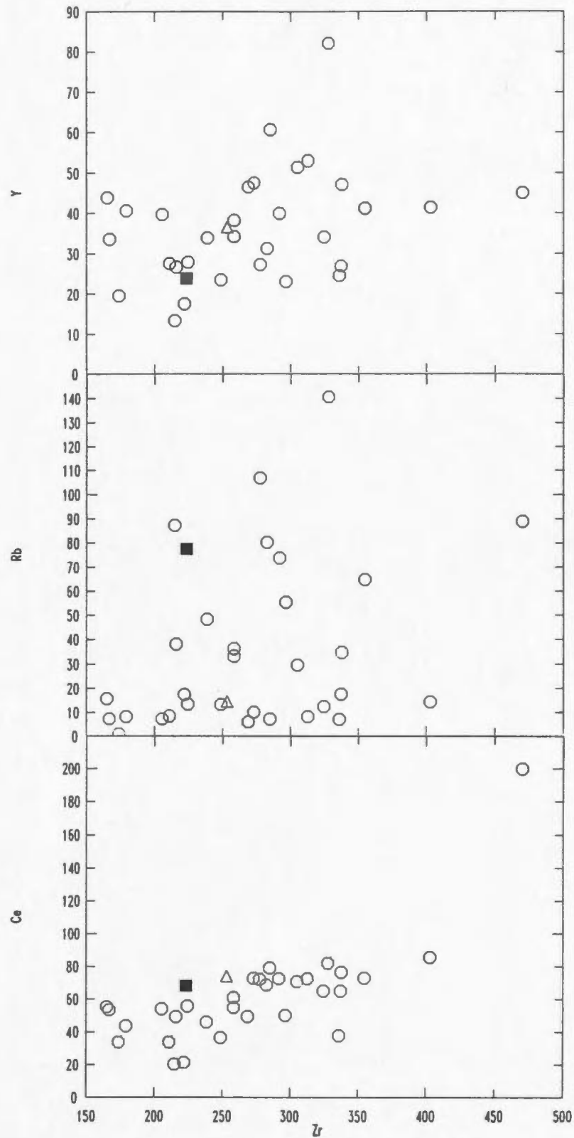
Figure 3.12. Trace element variation diagrams involving Zr and other selected elements. Symbols as in Figure 3.1.
