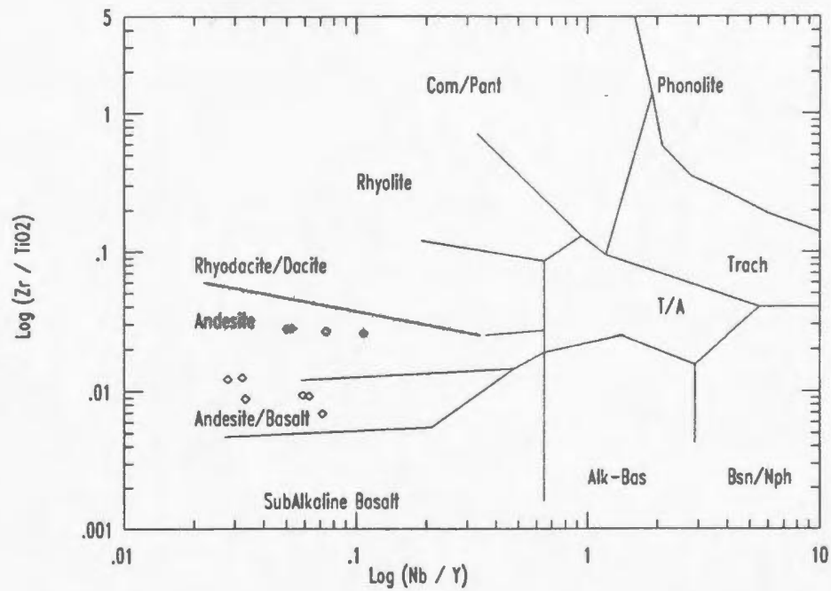
Figure 3.18. Nb/Y vs. Zr/Ti diagram illustrating the compositions of the older (open diamonds) and younger (filled diamonds) mafic dykes.
