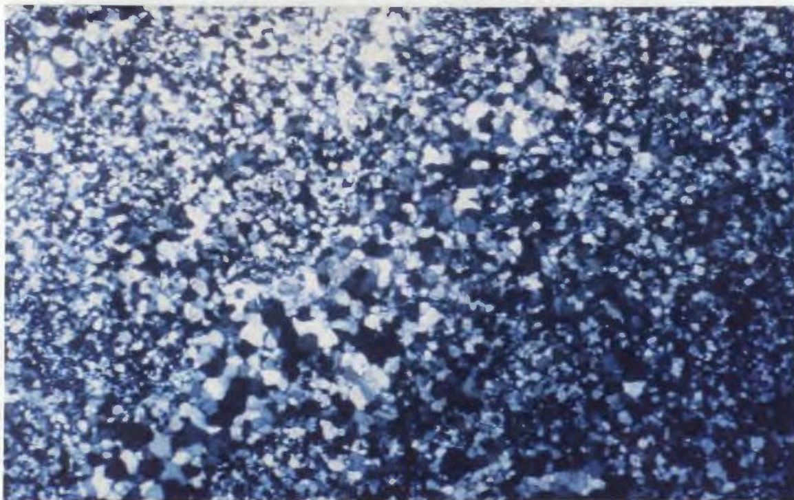
Plate 4.13. Fine-grained recrystallized quartz from the lower zone at the Winter Hill Showing. Sample SS88-103 (584066), mag.= 100X, fov = 1 mm, X-nicols.
