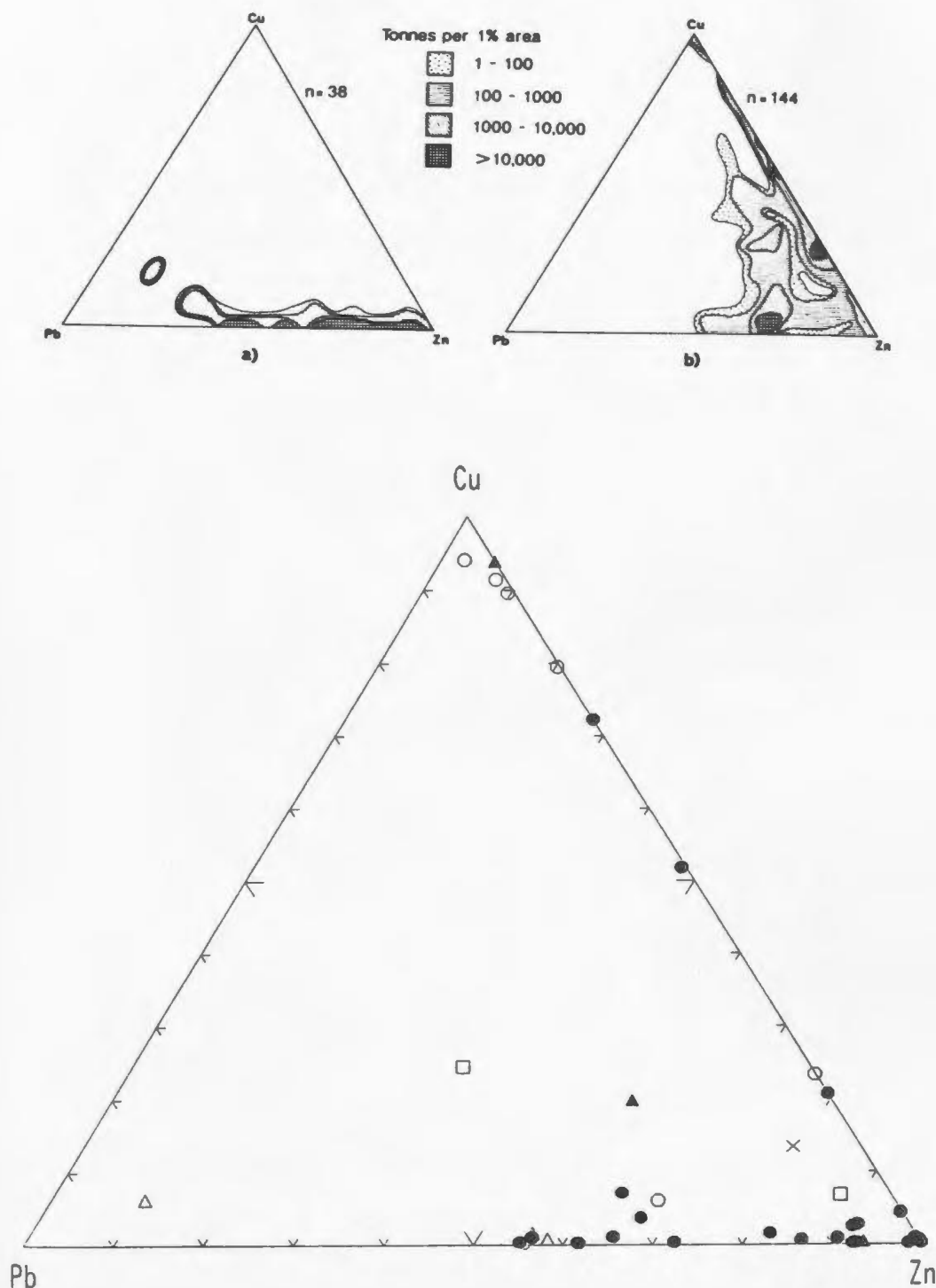
Figure 5.14. Pb-Cu-Zn ternary diagram for mineralized Sam Head Fm. samples. Ternary diagrams (a) and (b) represent bulk compositions for sediment-hosted stratiform Pb-Zn deposits (a) and VMS deposits of the Abitibi Belt, the New Brunswick area, Norwegian Caledonides, and the Green Tuff Belt of Japan (b) (taken from Lydon, 1983). Contours are total tonnes of ore metals per 1% area of the diagram. Symbols as in Figure 5.12.
