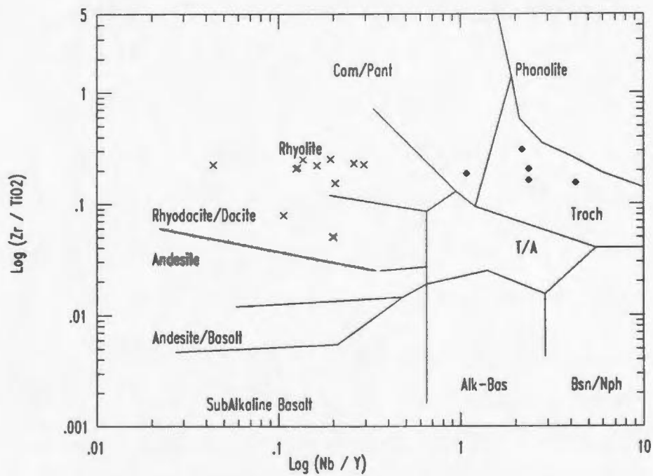
Figure 3.21. Nb/Y vs. Zr/Ti plot illustrating the distinct chemical signatures between the older felsic dykes (X's) and the younger felsic dykes (filled diamonds).
