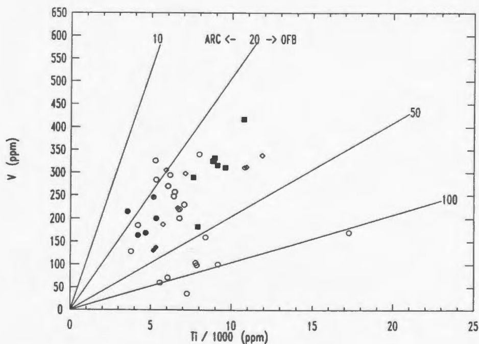
Figure 3.34. Plot of Ti vs. V displaying the volcanic arc (ARC) field and the ocean floor basalt (OFB) field, as defined by Shervais (1982). Symbols as in Figures 3.1 and 3.18.
