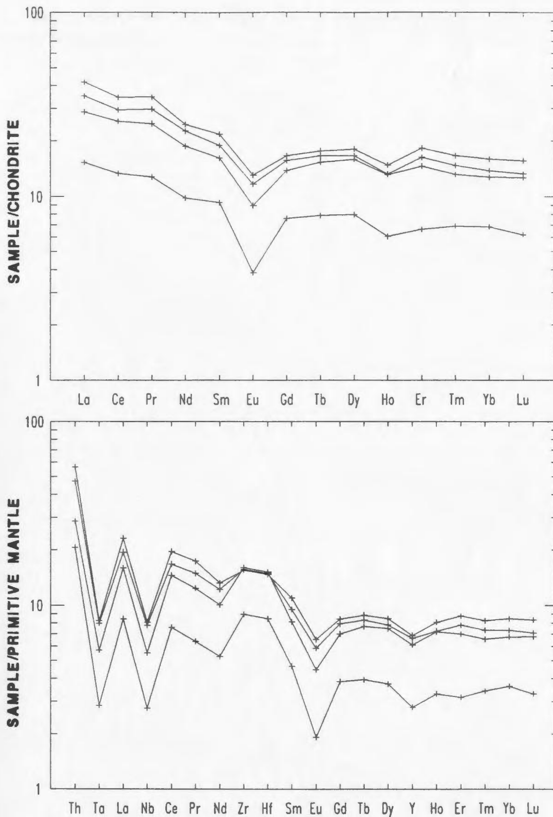
Figure 5.10. Chondrite-normalized REE and primitive mantle-normalized extended REE profiles for mineralized samples from the Selco Showings.
