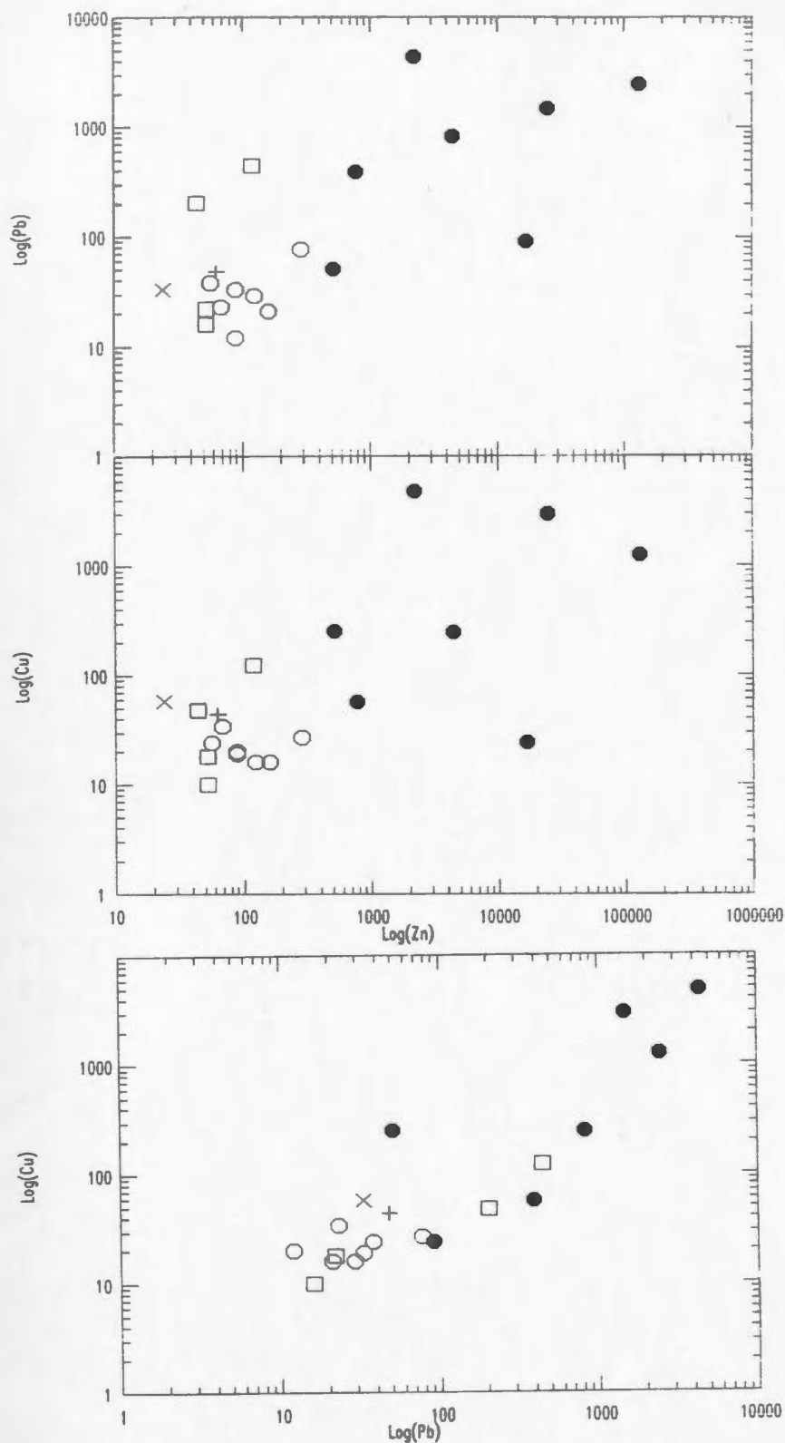
Figure 5.1. Base-metal variation diagrams for samples from the Tickle Point Formation. Closed circles = Frenchman Head Showing, open circles = Selco Showings, open squares = Shoal Brook Showing, X = Tilt Point, and cross = Fish Cove (Au occurrence).
