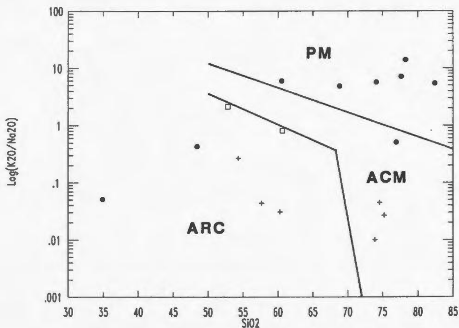
Figure 3.16. \text{SiO}_2 vs. \text{K}_2\text{O}/\text{Na}_2\text{O} plot taken from Roser and Korsch (1986), with the fields for passive margin (PM), active continental margin (ACM), and oceanic island arc (ARC) sedimentation. Closed circles = sedimentary rocks from the Sam Head Fm., crosses = sedimentary samples from the Tickle Pt. Fm., open squares = Doughball Pt. Fm. sedimentary rock samples.
