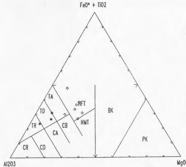
Figure 3.20. \text{Al}_2\text{O}_3 - \text{FeO}^* (Fe total) + \text{TiO}_2 - \text{MgO} diagram displaying the tholeiitic nature of both mafic dyke sets. Symbols as in Figure 3.18 and fields as in Figure 3.7.
