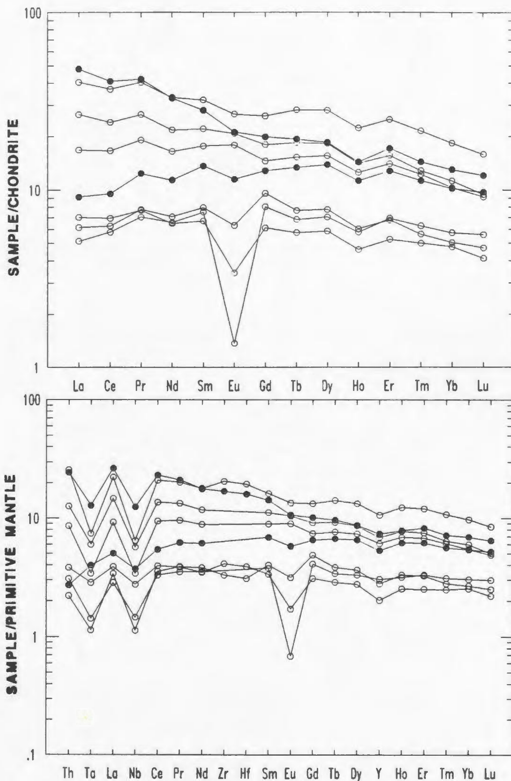
Figure 3.26. Chondrite-normalized REE and primitive mantle-normalized extended REE patterns for selected mafic to intermediate rock samples from the Tickle Pt. Fm. (open circles) and the Sam Head Fm. (filled circles).
