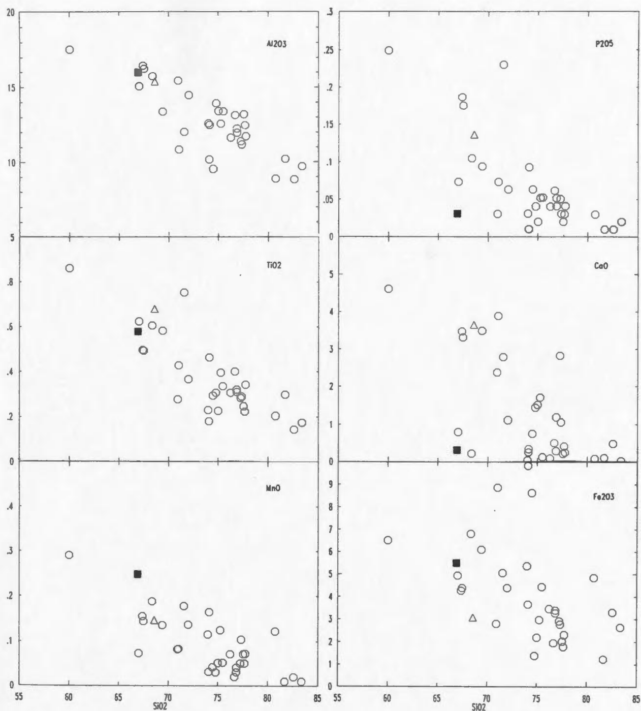
Figure 3.10. Variation diagrams involving \text{SiO}_2 vs. other major elements for the dacitic to felsic rock samples. Symbols as in Figure 3.1.
