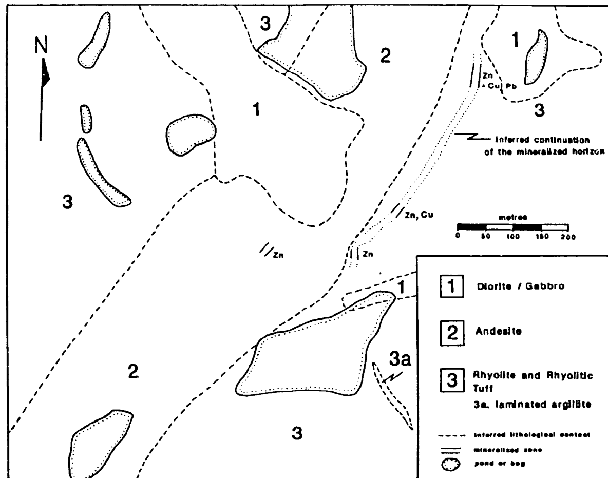
Figure 4.1. Geology of the Frenchman Head Showing.
