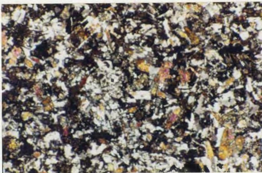
Plate 2.16. Equigranular texture from the older mafic dyke suite. Sample SS88-284 (584145), mag.=32X, fov = 3.3 mm, X-nicols.
