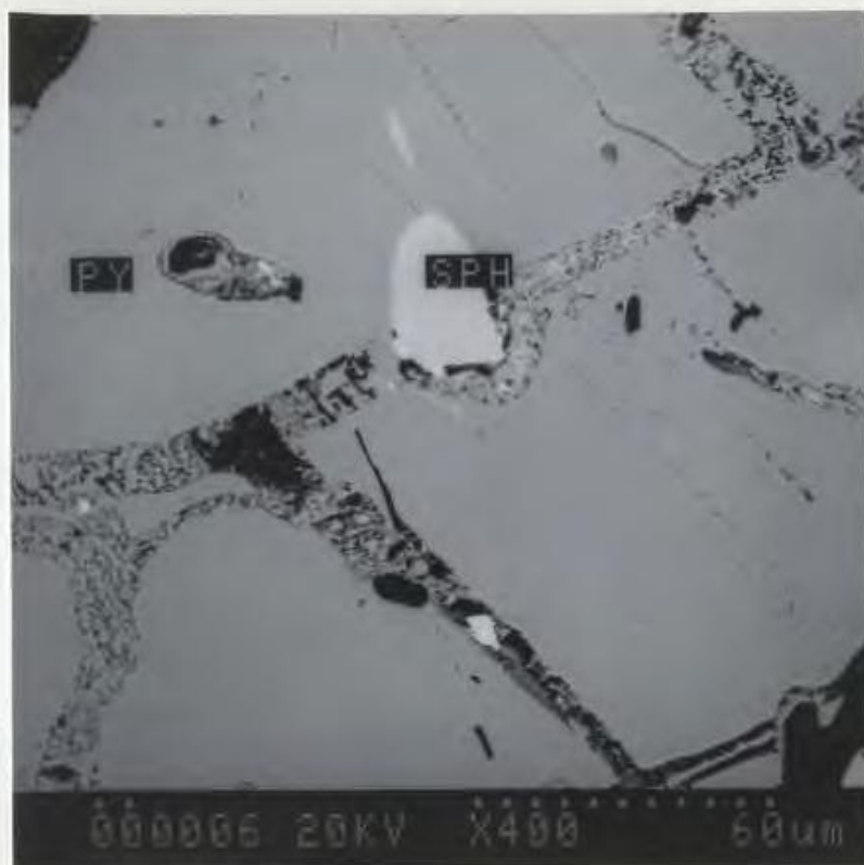
Plate 4.9. Scanning electron microscope (SEM) back scatter photograph of brecciated channels within pyrite grains. PY = pyrite, SPH = sphalerite. Sample SS88-039 (584016), mag.= 400X.
