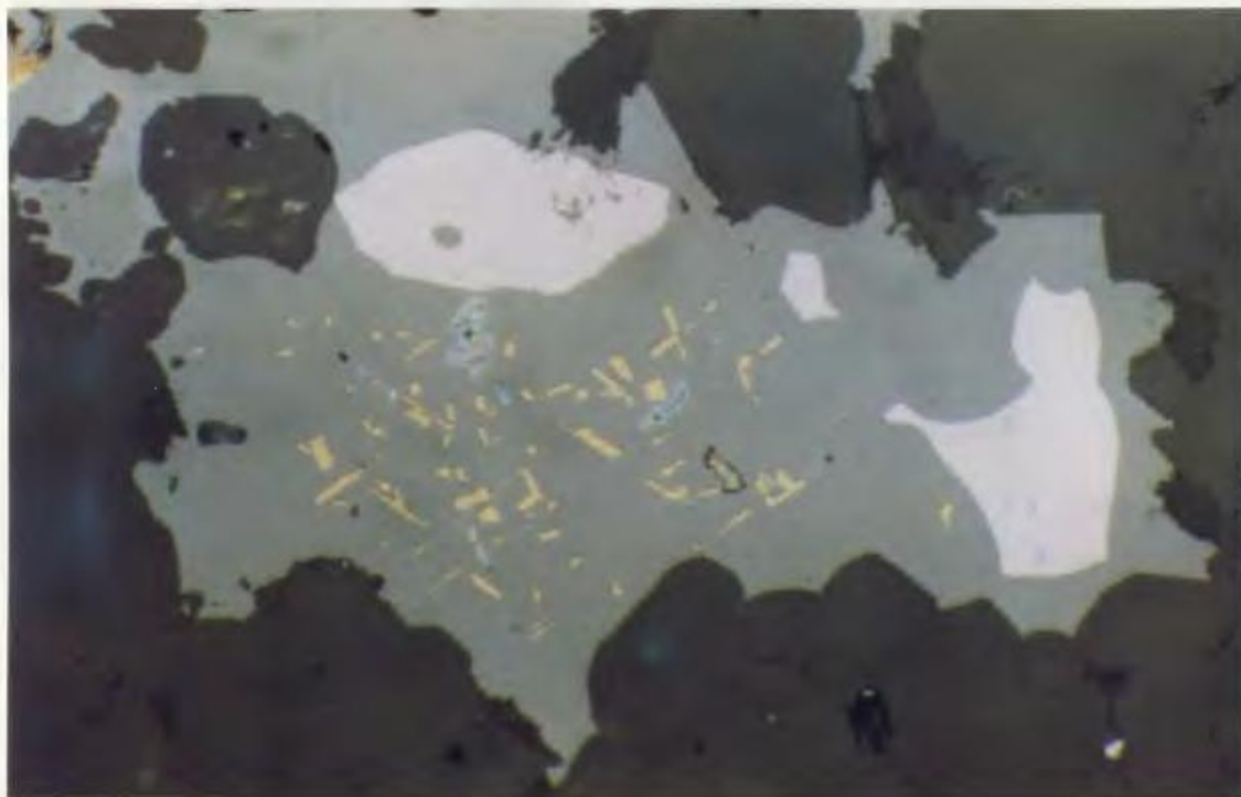
Plate 4.21. Elongate chalcopyrite crystals (yellow) along crystal boundaries in sphalerite (medium to dark gray). White crystals are galena. Sample SS88-101 (584065), mag.= 200X, fov = 0.5 mm, reflected light.
