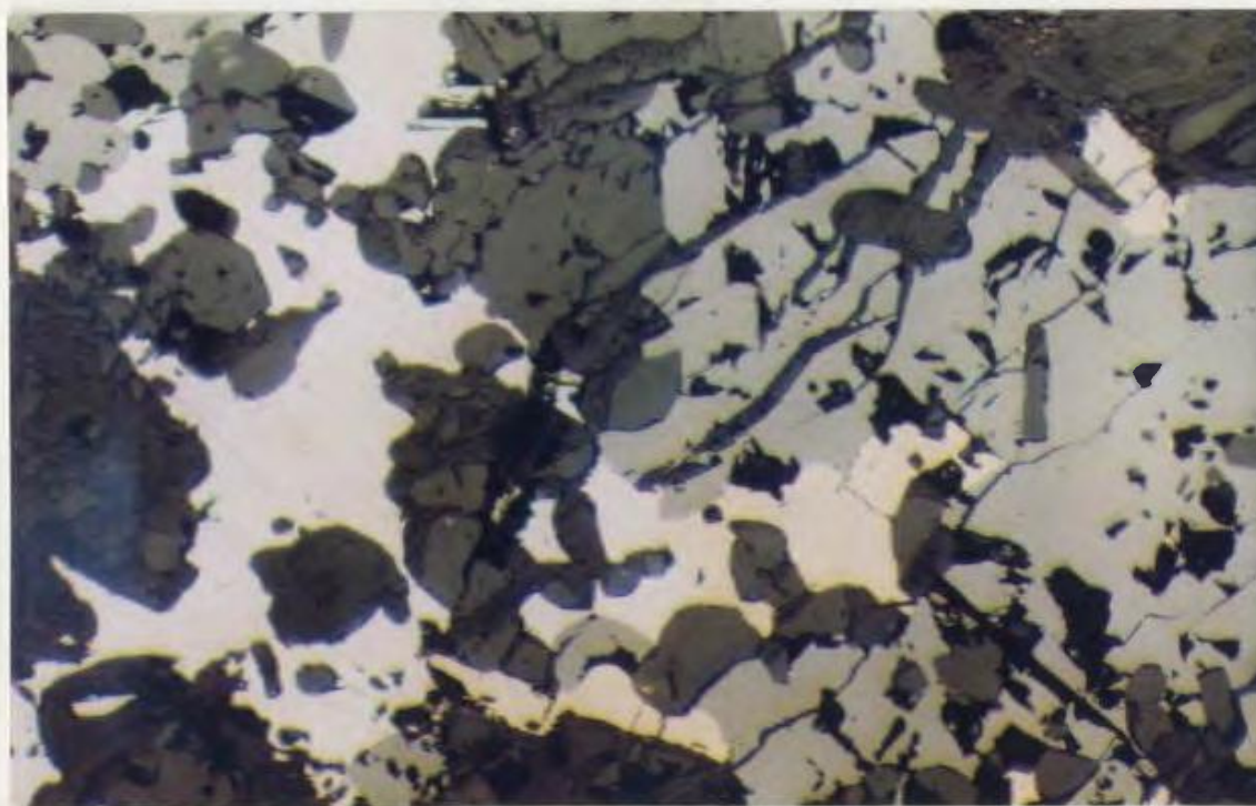
Plate 4.22. Sphalerite (medium gray), galena (white), and pyrrhotite (creamy brown) mineralization within the Winter Hill Showing. Sample SS88-089 (584055), mag.= 100X, fov = 1 mm, reflected light.
