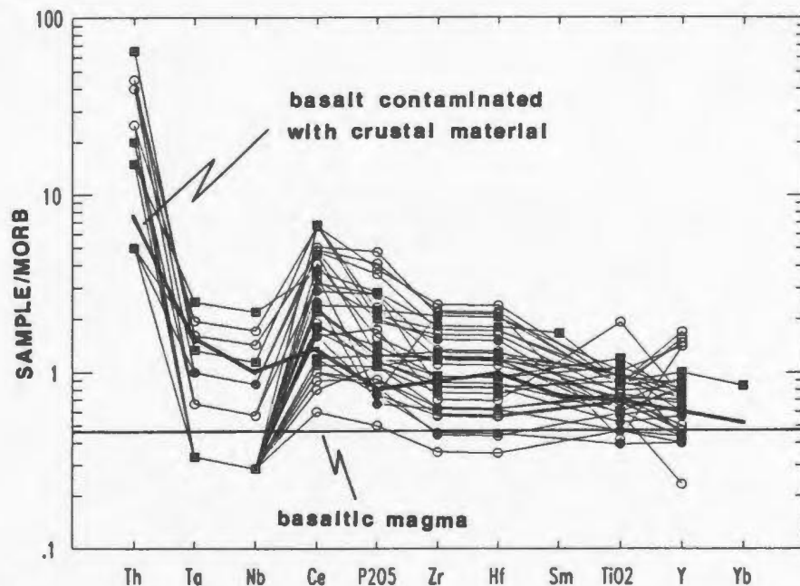
Figure 3.38. MORB-normalized spidergram adapted from Pearce (1983). The straight line (at approximately 0.5 MORB) represents a basalt magma and the above pattern represents a basalt contaminated by crustal material ( i.e. graywacke). The Connaigre Bay Group mafic to intermediate rocks may have been contaminated by a highly enriched crustal source. Symbols as in Figure 3.1.
