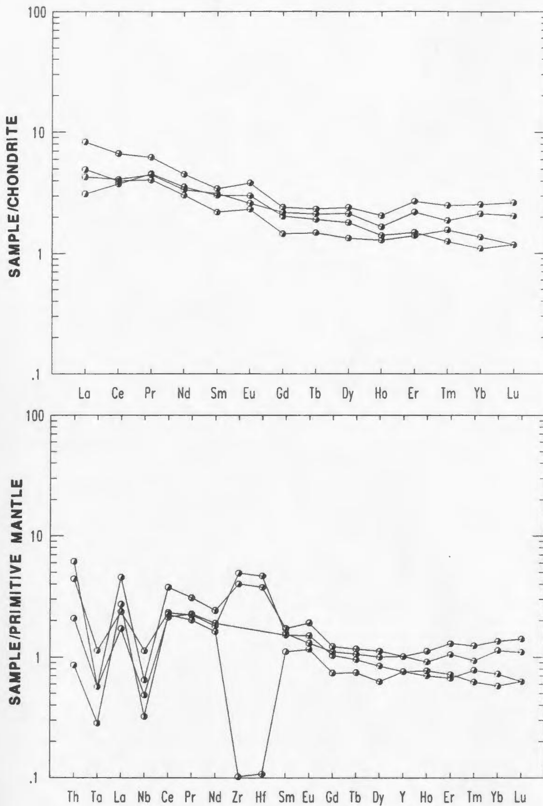
Figure 5.18. Chondrite-normalized REE and primitive mantle-normalized extended REE patterns for mineralized samples from the Winter Hill Showing.
