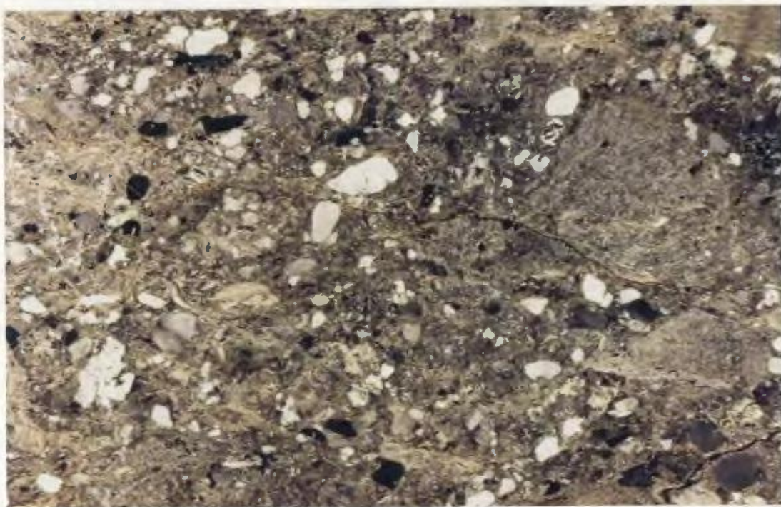
Plate 2.4. Lithic- and crystal-rich rhyolitic tuff from the Tickle Point Formation. Sample SS88-237 (584126), mag.= 6.3X, fov = 17.0 mm, X-nicols.
