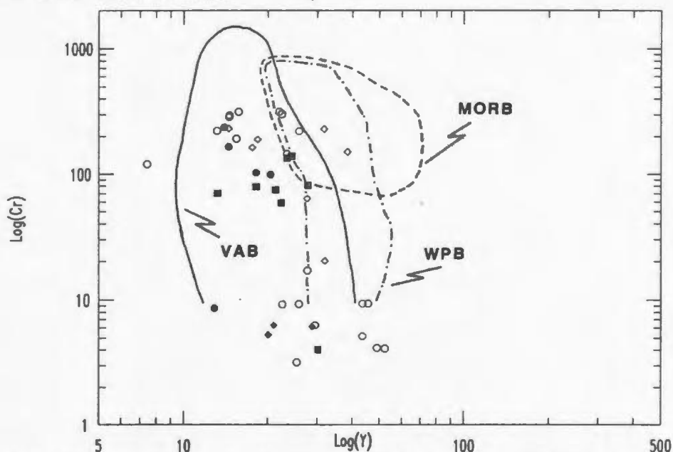
Figure 3.30. Y vs. Cr diagram with the respective tectonic fields (from Pearce et al. , 1981). The mafic to intermediate rocks and the mafic dykes plot mainly in the VAB field but some overlap into the WPB and MORB fields. VAB = volcanic arc basalt, MORB = mid-ocean ridge basalt, and WPB = within-plate basalt. Symbols as in Figures 3.1 and 3.18.
