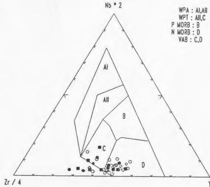
Figure 3.31. Zr - Nb - Y diagram taken from Meschede (1986) Most samples plot in fields C and D, whereas some plot outside the C-field toward the Zr axis. WPA = within-plate alkali basalt, WPT = within-plate tholeiite, P-MORB = plume influenced mid-ocean ridge basalt, N-MORB = normal mid-ocean ridge basalt, and VAB = volcanic arc basalt. Symbols as in Figures 3.1 and 3.18.
