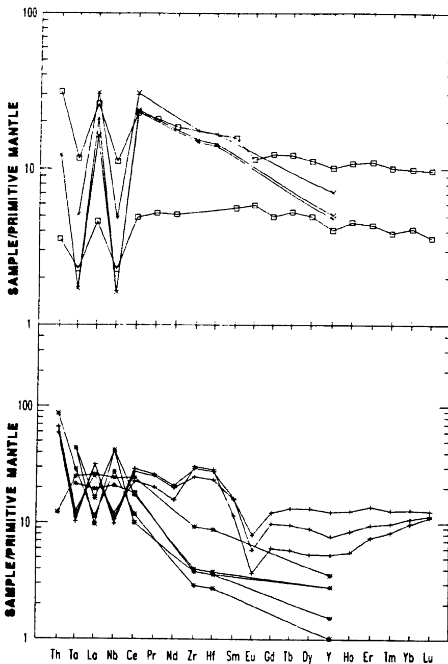
Figure 3.28. Extended REE profiles for mafic and felsic dykes cutting rocks of the Connaigre Bay Group. Upper diagram: open squares = older mafic dykes; X = younger mafic dykes. Lower diagram: + = older felsic dykes; * = younger felsic dykes.
