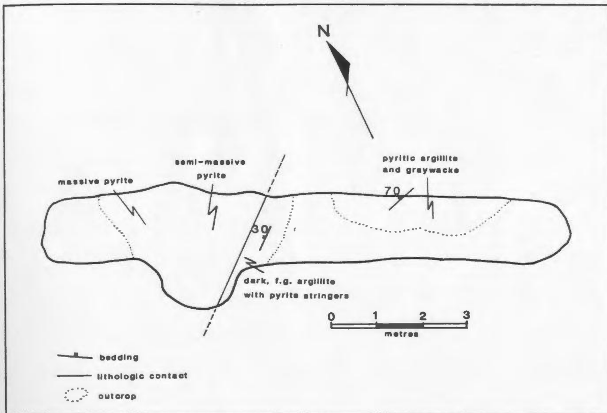
Figure 4.6. Geology of the main trench at Winter Hill West.
