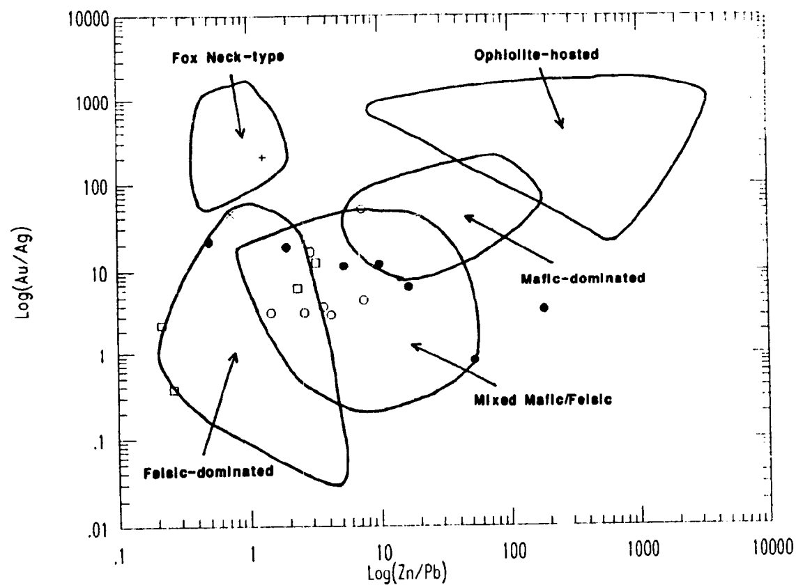
Figure 5.6. Zn/Pb vs. Au/Ag diagram taken from Swinden and Kean (1988). The plot displays the increasing Zn/Pb and Au/Ag ratios as the host rocks become more basic. The Tickle Point Fm. samples plot mainly in the felsic-dominated and mixed mafic-felsic fields. Symbols as in Figure 5.1.
