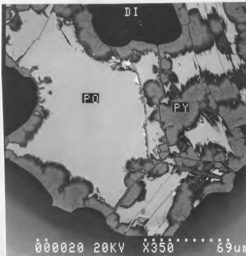
Plate 4.23. SEM back scatter photograph of a pyrrhotite (PO) crystal being replaced by pyrite (PY). Also present is a diopside (DI) inclusion. SS88-082 (584052), mag.= 350X.
