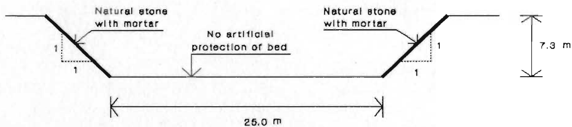
Figure 1.3. Typical cross-section of the proposed diversion channel.
