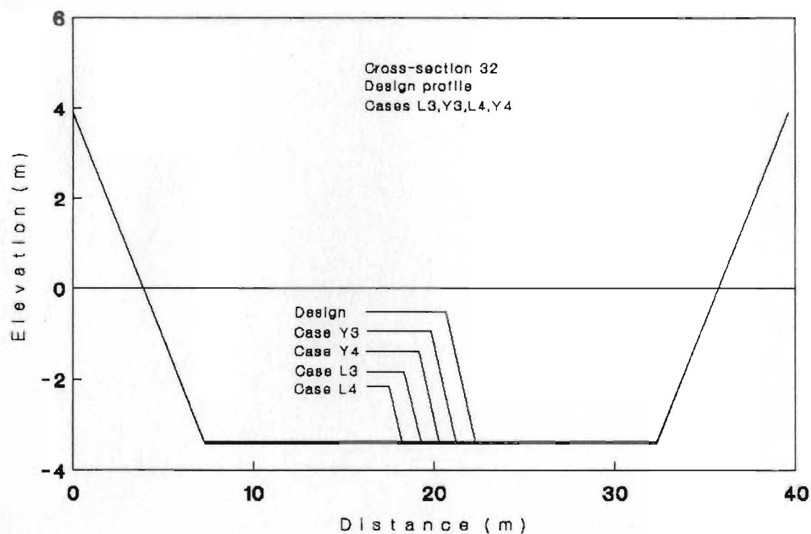
Figure C.6. Estimated changes in cross-section 32.
