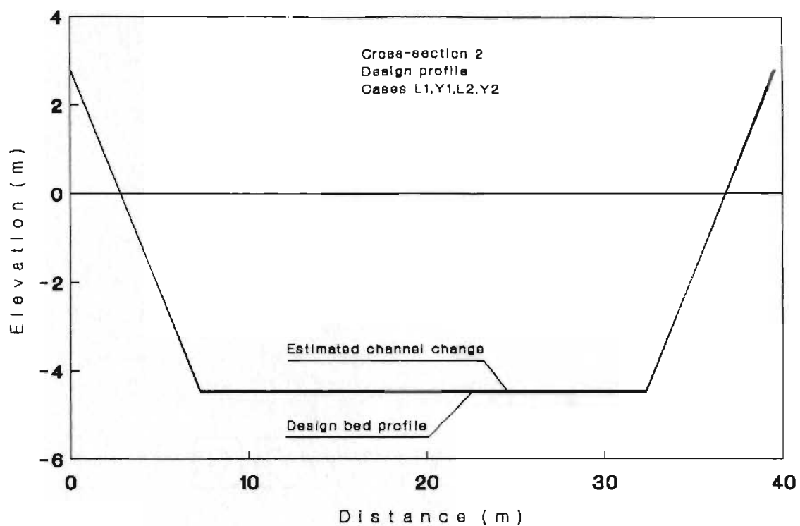
Figure C.1. Estimated changes in cross-section 2.
