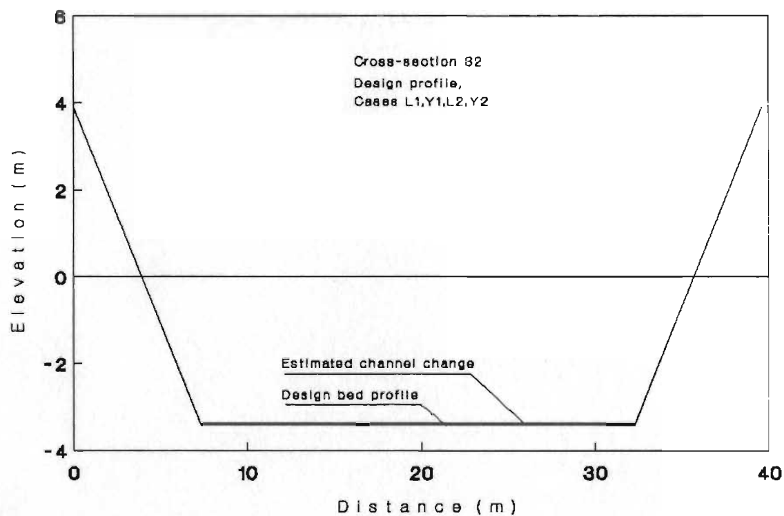
Figure C.2. Estimated changes in cross-section 32.
