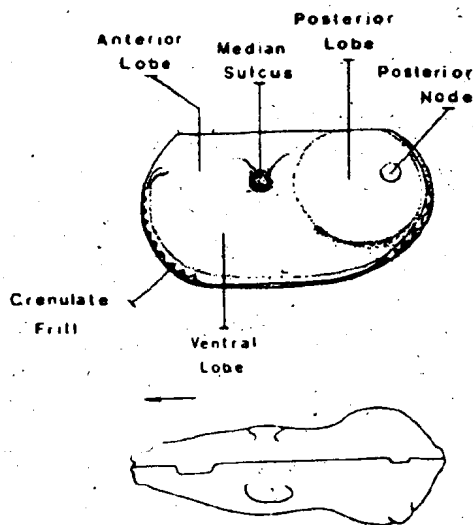
Text-fig. 6.17 : Morphology of Beyrichiopsis cornuta .
