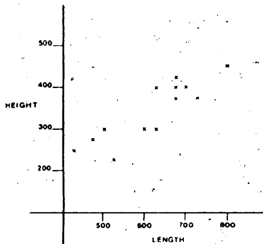
Text-fig. 6.16 : Morphology and growth sequence of Geisina sp. from Assemblage V.
