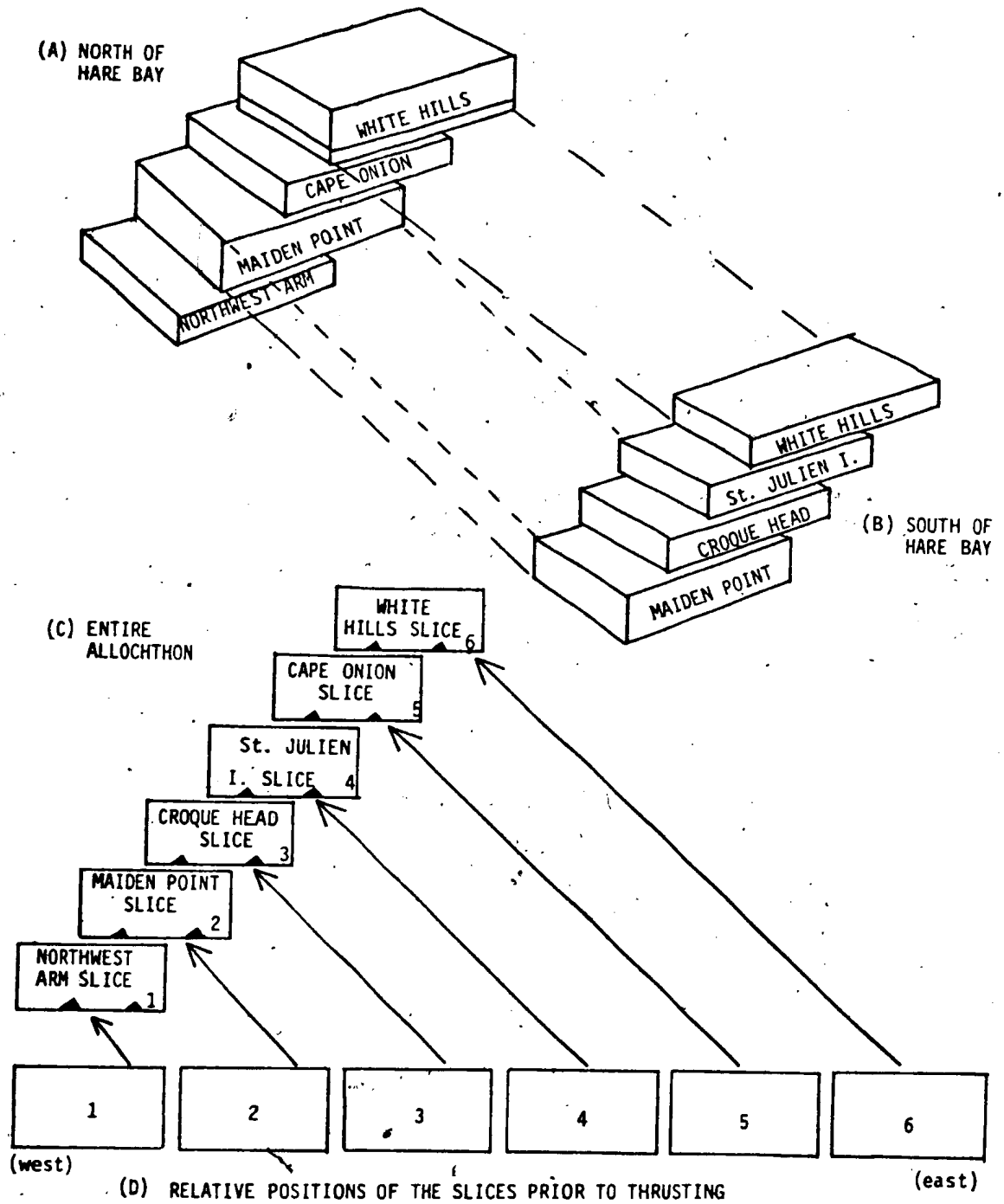
Fig 2i: Palinspastic reconstruction of the thrust slices shown schematically. (A) Structural stacking order of the slices north of Hare Bay. (B) Structural stacking order of the slices south of Hare Bay. (C) Structural stacking order of the slices of the entire Hare Bay Allochthon. (D) Palinspastic reconstruction of the slices to the relative positions they had before emplacement, using the assumption that the higher slices originated farther from the continental margin in the west.
