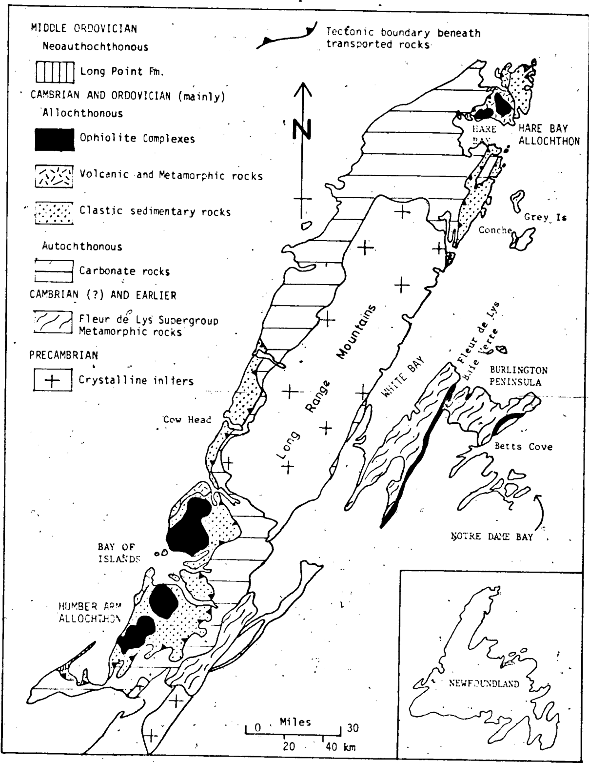
Figure 1. Major tectonic elements of western Newfoundland
