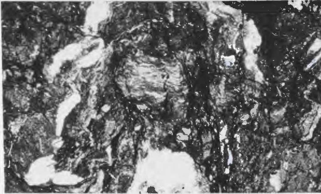
Fig. a: Photomicrograph of Mélange. Note how the emplacement schistosity ( S_1 ) is cut by an upright crenulation ( S_2 ) cleavage. Basal mélangé to the Croque Head Slice, Cobblers Cove.
