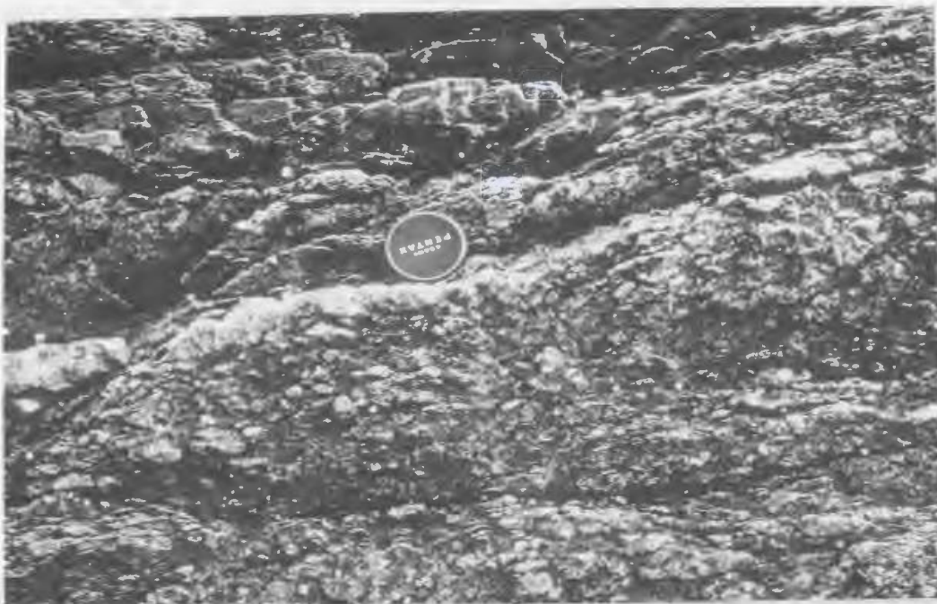
b: Highly deformed, schistose granite, Sugarloaf Slide Zone. The schistosity ( S_1 ) is defined by thin zones of phyllonite that form augen around relict phenocrysts of feldspar and quartz. Southwest of Sugarloaf Cove.
