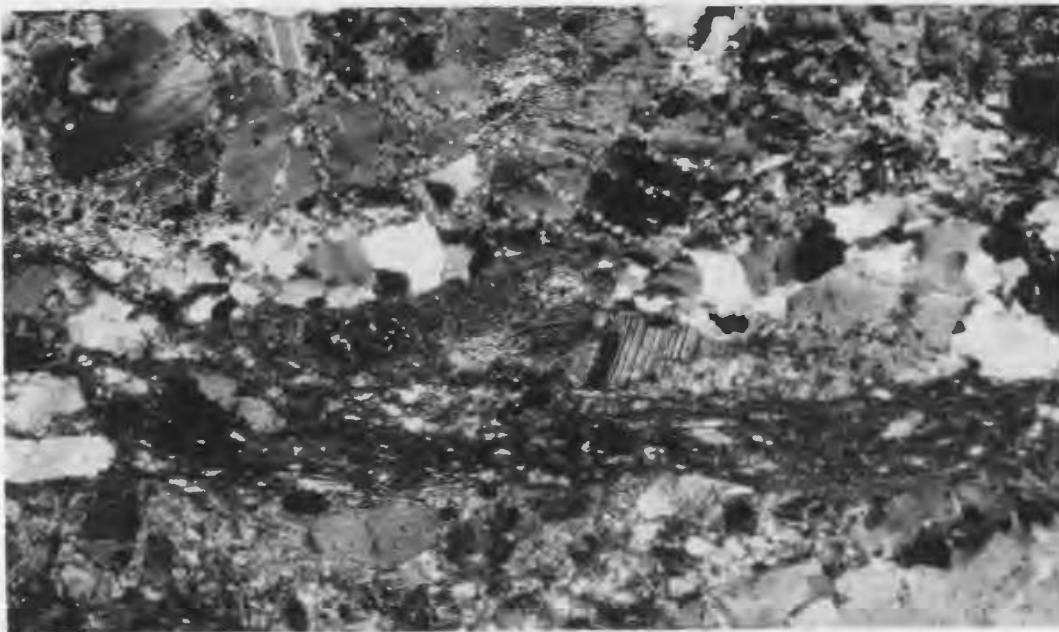
b: Photomicrograph of Phyllonitized granite, Sugarloaf Slide Zone. Note parallel zones of granulated and schistose matrix. Crossed nicols.
