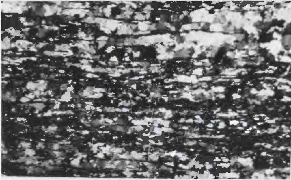
Fig.a: Foliated gneiss clast, St. Julien Island Formation. Note alternating quartz and mafic (dark) foliae. St. Julien Island. Crossed nicols.
