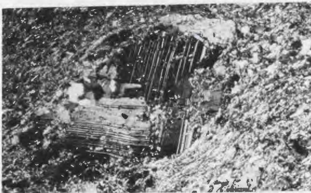
b: Relict Plagioclase Porphyroblast enclosed in highly crushed and granulated matrix. Sugarloaf Slide Zone. Shore, south of Sugarloaf Cove. Crossed nicols.
