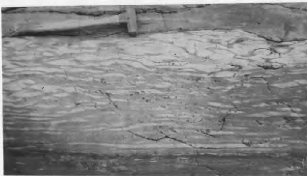
b: Slumped bedding in greywackes, Maiden Point Formation. Mare Cove.
