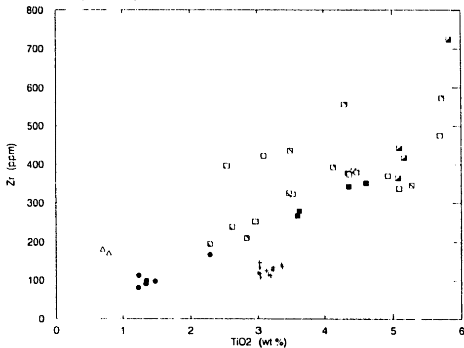
FIGURE 4.2i (TiO 2 VS Zr)
