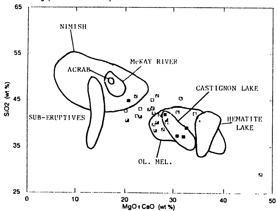
FIGURE 5.1g (MGO+CAO VS \text{SiO}_2 )
