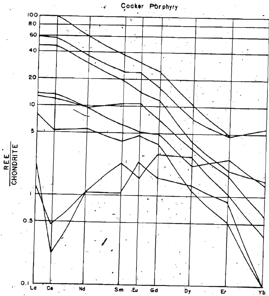
Figure 6.8 REE/Chondrite: Coaker Porphyry
