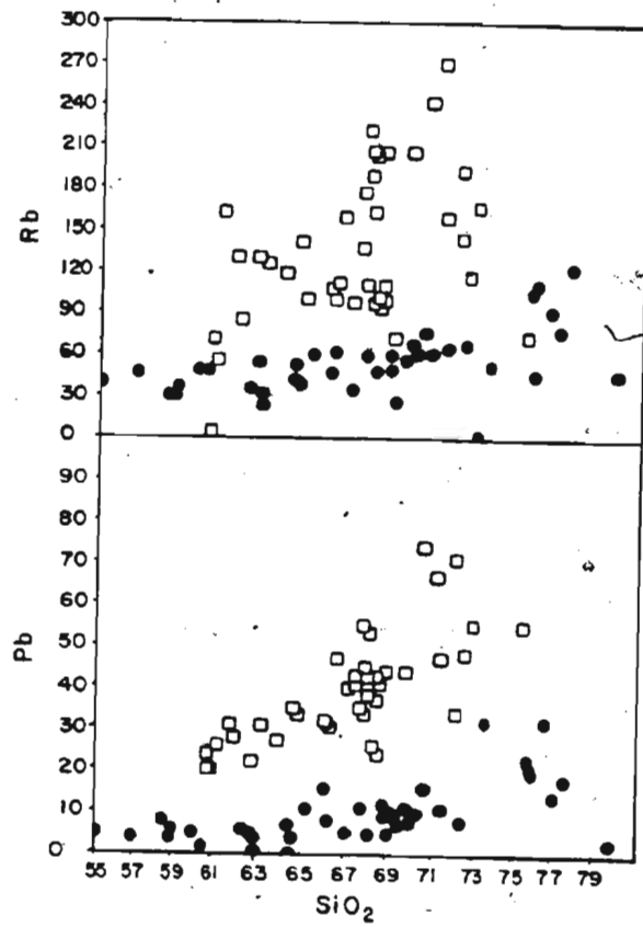
Figure 7.10 A comparison between Coaker Porphyry (□) and Loon Bay/Dildo Porphyry (●) contents of Rb and Pb versus SiO 2 .
