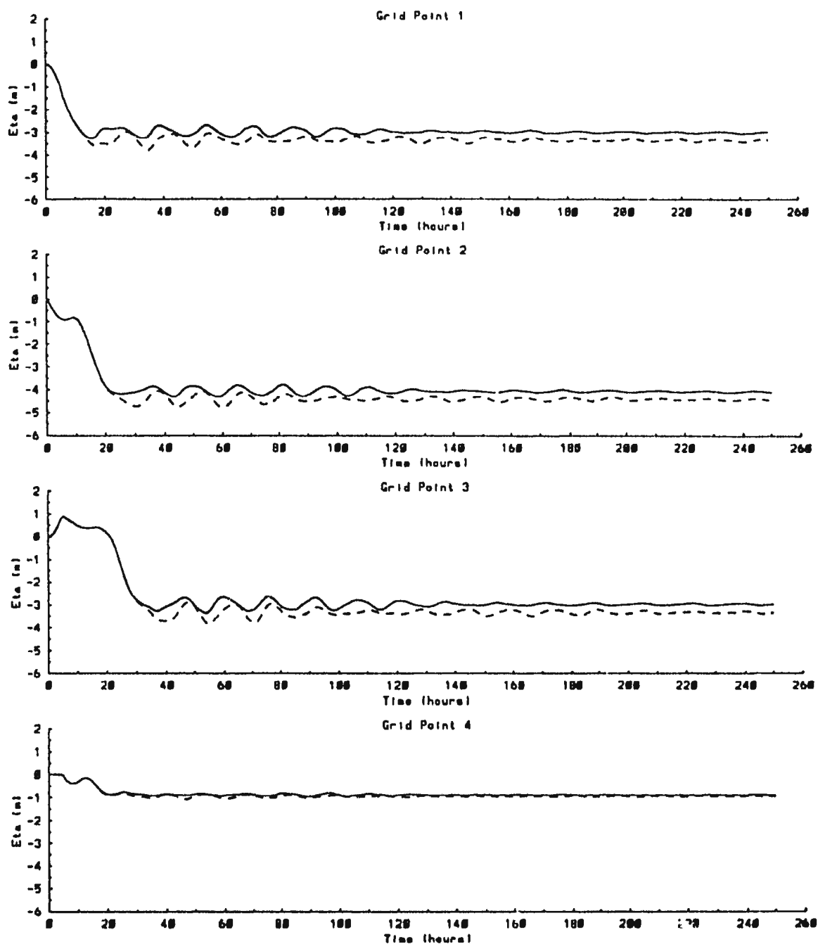
Figure 3.10a Time series of the interface displacement (in meters) at the grid points numbered in Figure 3.8 following the sudden application at t = 0 of a uniform, steady, northward wind. The solid lines represent the case using the smaller domain in Figure 3.8. The dashed lines are obtained using the domain shown in Figure 3.7.
