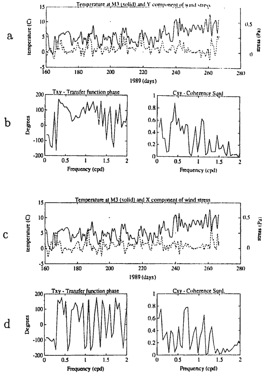
Figure 4.4 (a) Temperature (in ^{\circ}\text{C} ) at \sim 25 meters at M3 and the y -component of wind stress (in Pa). (b) Cross-spectrum between temperature and y -component of wind stress. (c) Temperature (in ^{\circ}\text{C} ) at \sim 25 meters at M3 and the x -component of wind stress (in Pa). (d) Cross-spectrum between temperature and x -component of wind stress. Spectra have ten degrees of freedom, and values of (\text{coherence})^2 greater than 0.59 are significant at the 90% confidence level.
