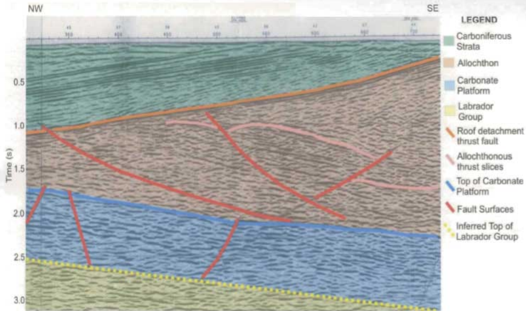
Figure 2.3b. Seismic line 91-1561, a typical seismic expression of the Triangle zone. In comparison to 5.3a the above figure gives a wider picture of the Taconic allochthon and its internal structure of thrust sheets (see figure 2.6 for location).
