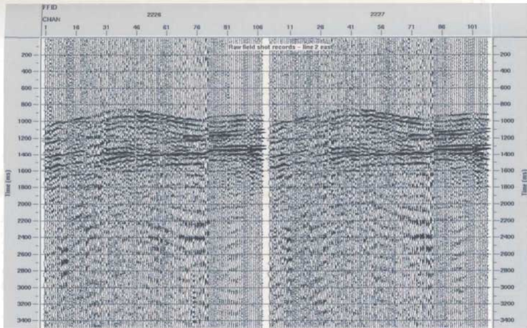
Figure 3.7b. Sample unfiltered/unscaled shot records for line 2 east of the marine 3D survey.
