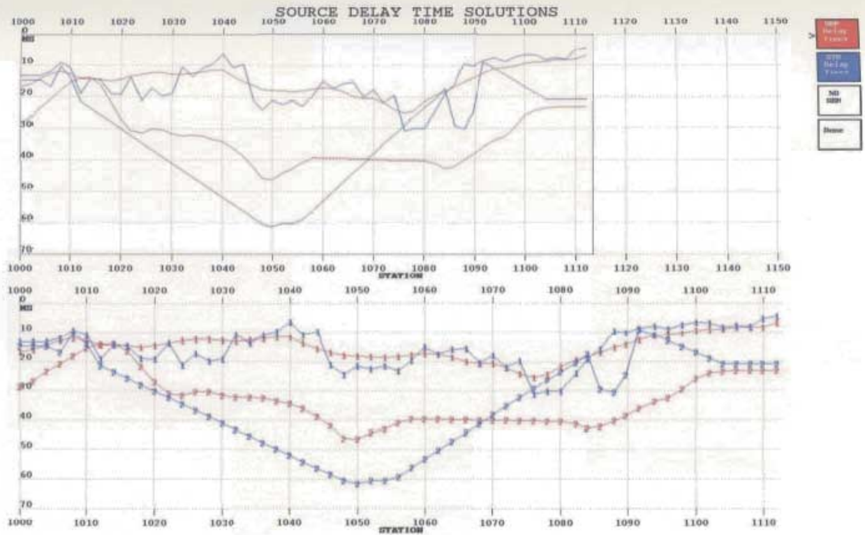
Figure 4.9d. Diagram of source static shifts calculated from the velocity and depth models, again the DRM values are in red.
