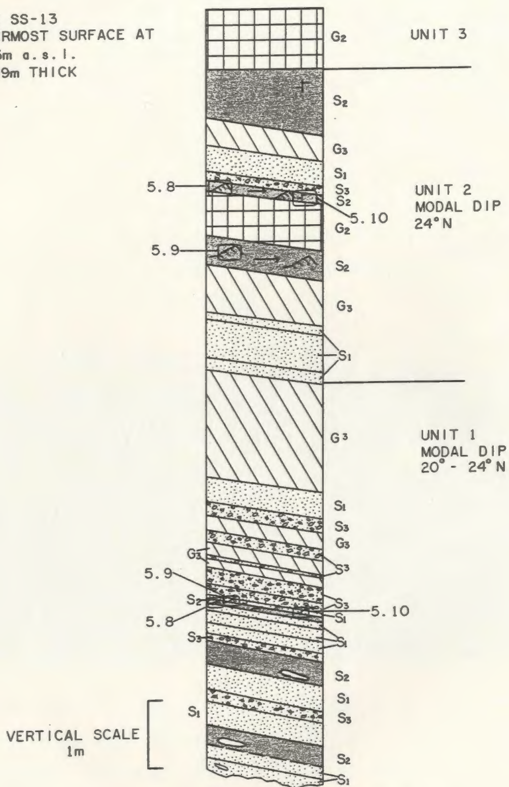
Figure 5.6: Sedimentary column of Site SS-13. See Figure 5.2 for Legend.
