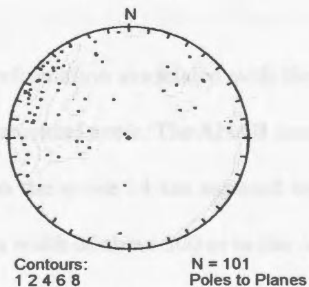
C. Foliation
