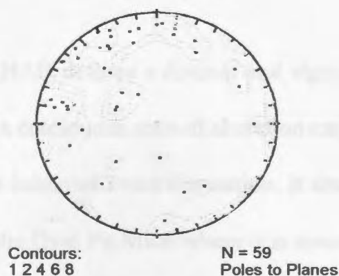
D. Cleavage
