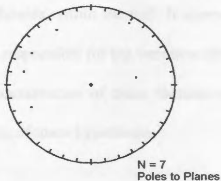
A. Eutaxitic Foliation
