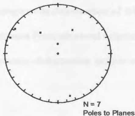
B. Layering in Unwelded Tuffs
