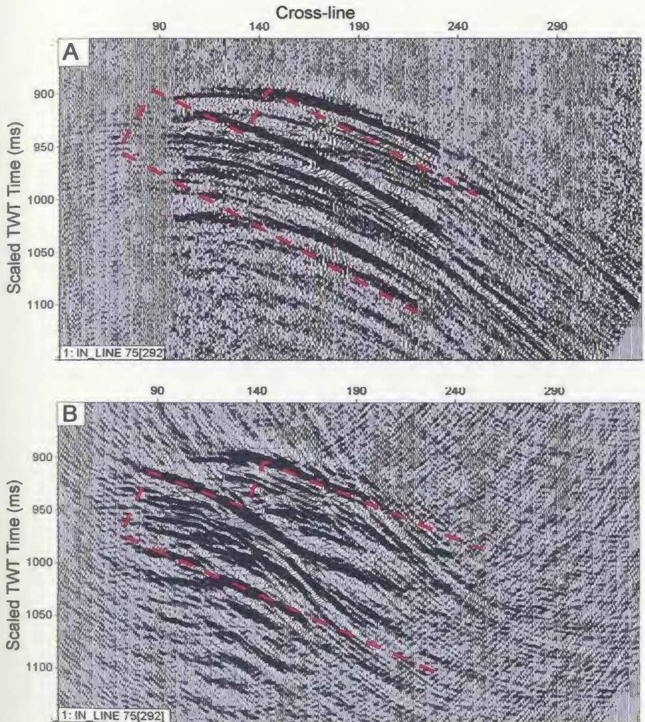
Figure 4.2.2-8: In-line stacks through the cylinder-shaped model dipping at 35° before (A) and after (B) post-stack 3D F-K time migration. A simplified cross-section of the model is overlain to facilitate interpretation.
