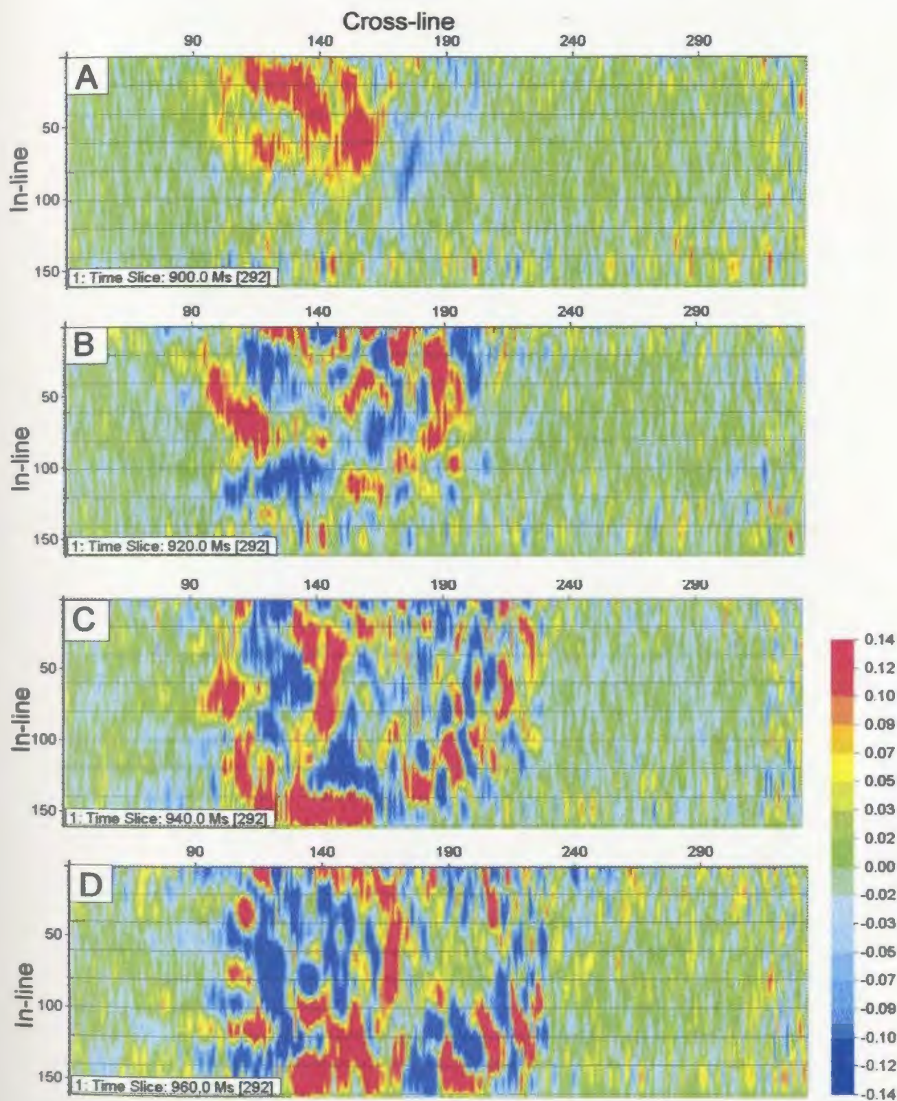
Figure 4.2.2-9: Time slices through the cylinder-shaped model dipping 35^\circ before 3D F-K time migration. Note that the diffraction pattern is roughly circular but discontinuous because of the rugged surface relief.
