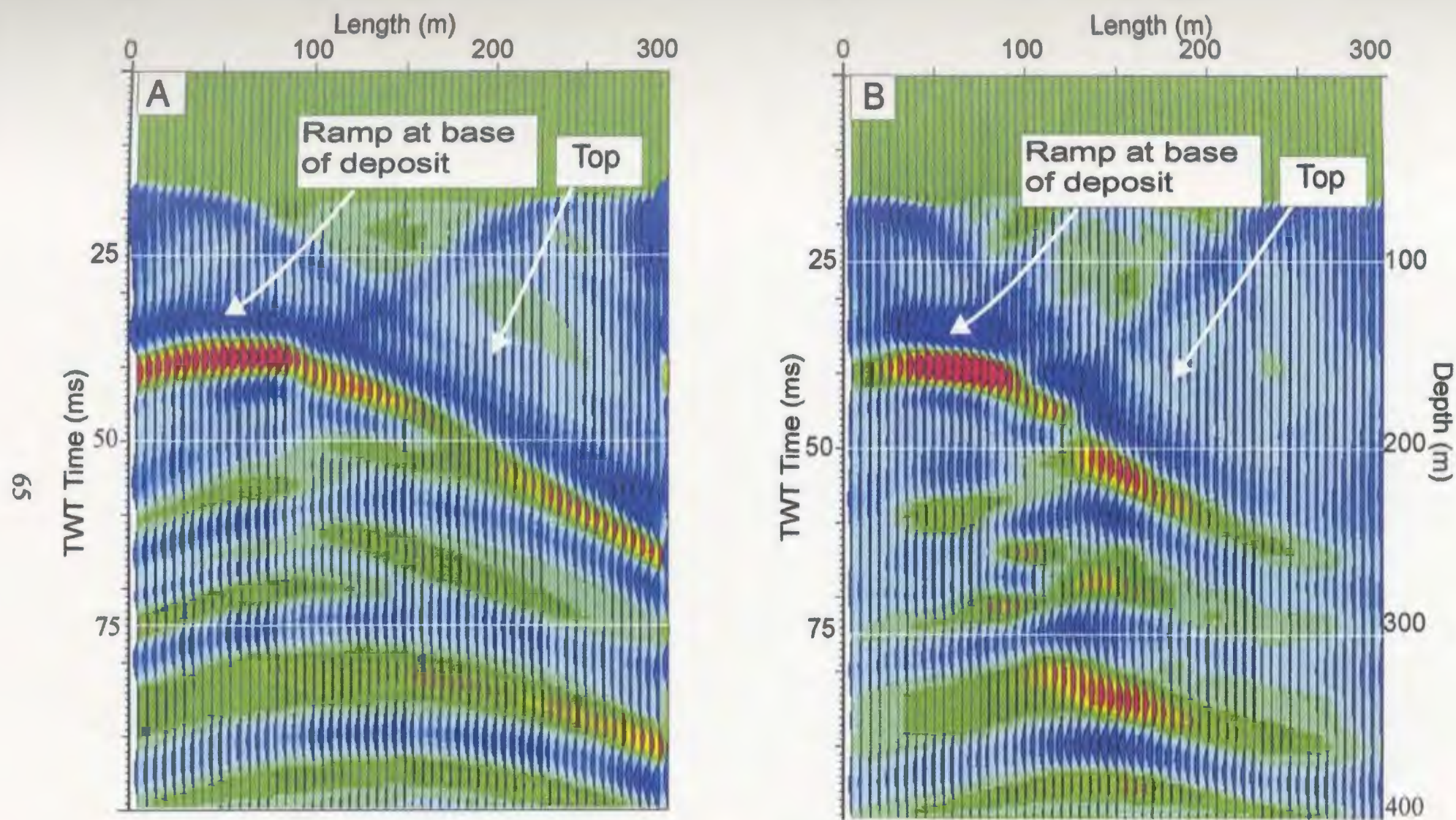
Figure 3.2-12: Synthetic profiles for the Flin-Flon Zn-Pb-Cu deposit (MN) (A) before migration, and (B) after migration. The diffraction pattern clearly shows that the deposit is steeply dipping to the right.
