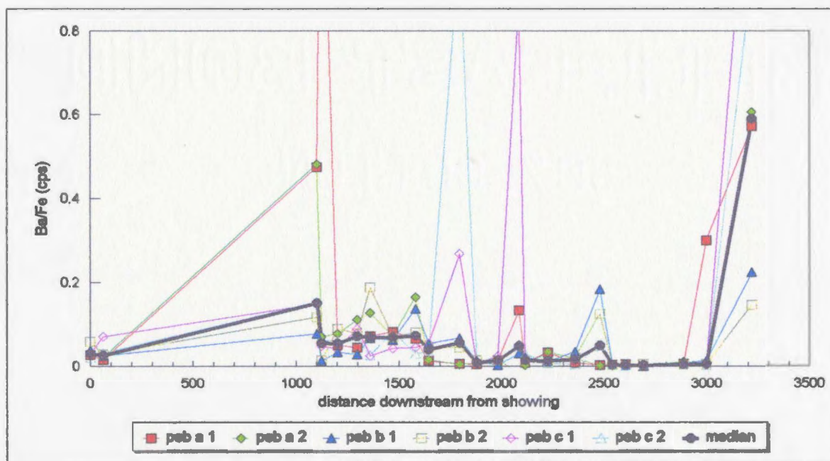
Figure 4.17: Ba determined in the oxide pebble coatings collected from Country Brook; Winter Hill VMS prospect is located at distance zero. (a) Ba/Fe (ppm) results from partial dissolutions of Mn-Fe-oxide coatings and (b) Ba/Fe (cps) results from laser ablation of the Mn-Fe-oxide pebble coatings.
