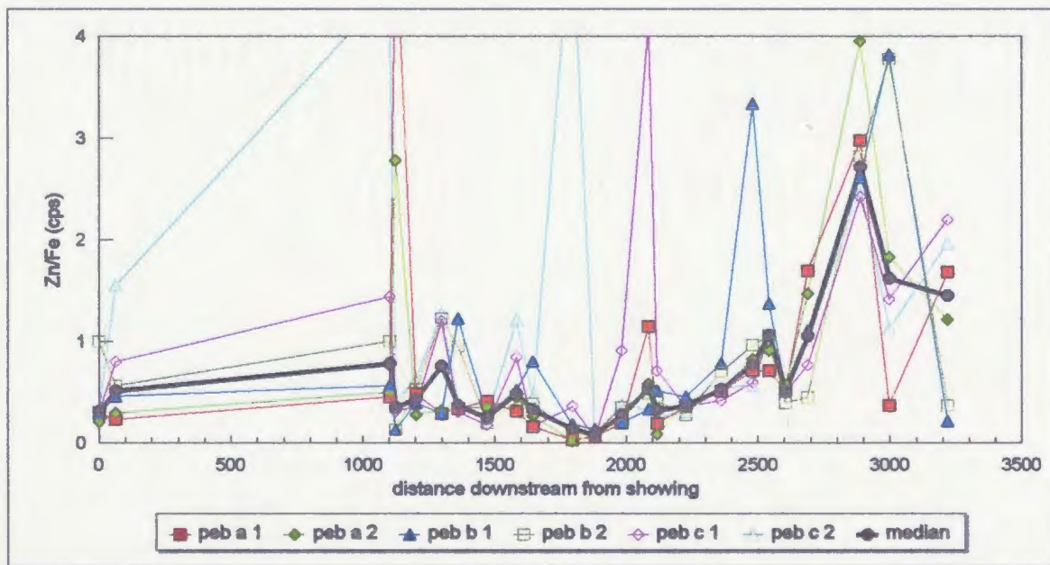
Figure 4.15: Zn determined in the oxide pebble coatings collected from Country Brook; Winter Hill VMS prospect is located at distance zero. (a) Zn/Fe (ppm) results from partial dissolutions of Mn-Fe-oxide coatings and (b) Zn/Fe (cps) results from the laser ablation of Mn-Fe-oxide pebble coatings.
