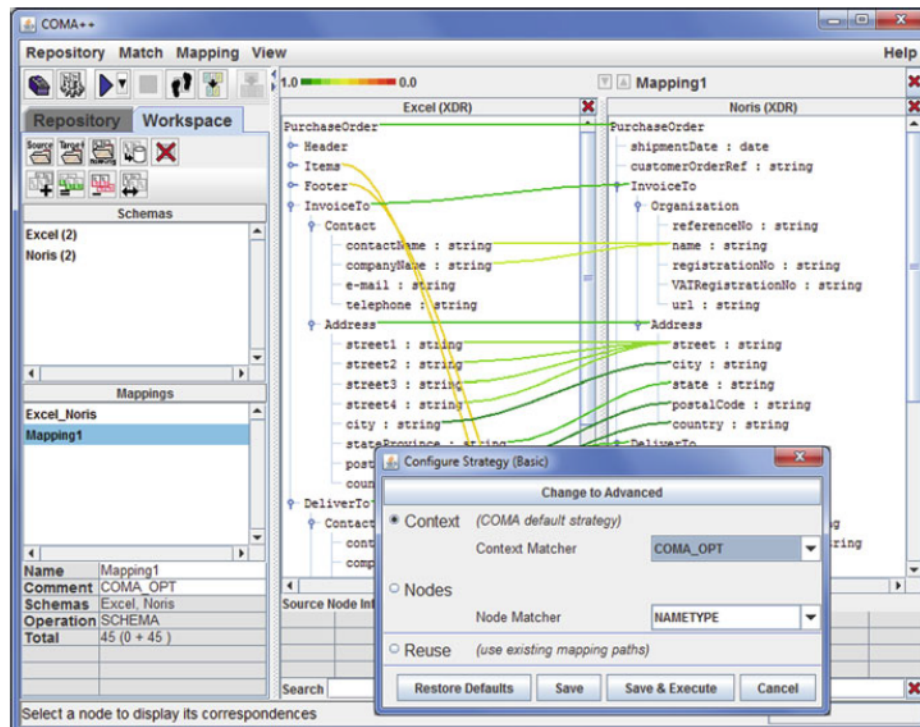
Figure 2.4: Screenshot of the interface of the COMA++ system [28]
